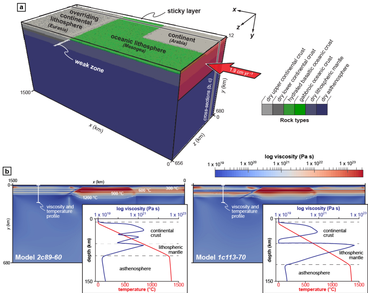
Figure 5.6: initial model setup. (a) 3D model domain with colors representing the different rock types. Air and sea water phases (composing the sticky layer) are cut off for clarity. (b) x - y viscosity cross-sections of the initial model domain with a two-layer (left panel) and one-layer (right panel) continental crust. White lines represent 300, 600, 900 and 1200 °C isotherms. Vertical viscosity (blue) and temperature (red) profiles are shown as inset for each model.
