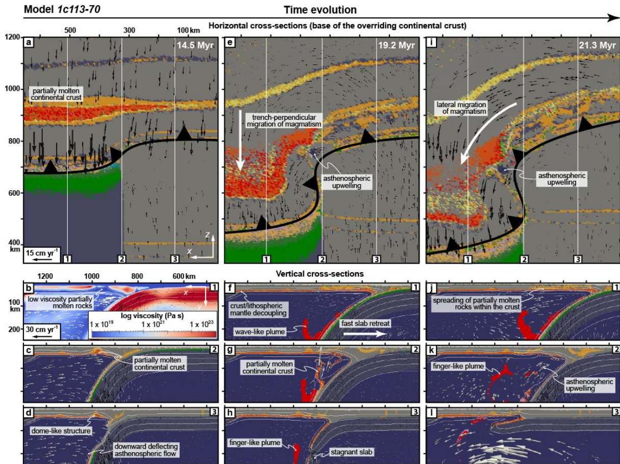
Figure 5.15: evolution of magmatism in model 1c113-70 . x - z plan views (a, e, i) and x - y cross-sections (b, c, d, f, g, h, j, k, l) of the subduction zone for selected time steps. Colors represent the different rock types (see figure 5.7 for detailed legend), except for cross-section (b) where the viscosity is mapped. Black and white arrows represent velocity vectors in the continental crust (top panels) or lithospheric mantle (bottom panels) and the asthenosphere, respectively. Scale of velocity vectors is twice larger in top panels than in bottom panels. White lines (bottom panels) represent 300, 600, 900 and 1200 °C isotherms.
