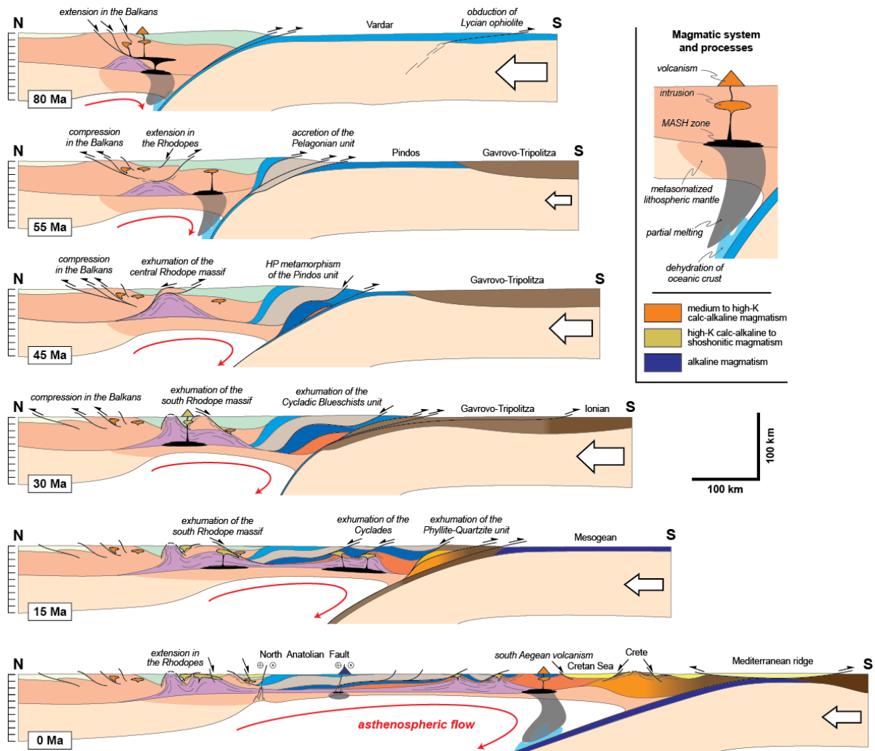
Figure 2.10: reconstructed cross-sections of the Aegean region highlighting the different magma genesis processes. MASH zone : Melting Assimilation Storage and Homogenization zone. See figure 2.5 for detailed legend.
