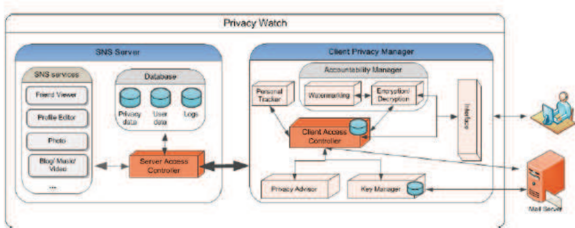
Figure 2.4 – PrivacyWatch's architecture
