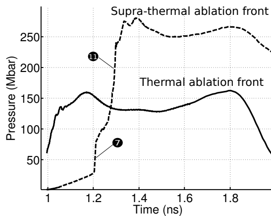
Figure 6.22: Pressure evolution at the laser driven and hot electron driven ablation fronts. The hot electrons parameters in this simulation are \eta_{he} = 15\% and \rho_{he} = 10 \text{ mg}\cdot\text{cm}^{-2} .
