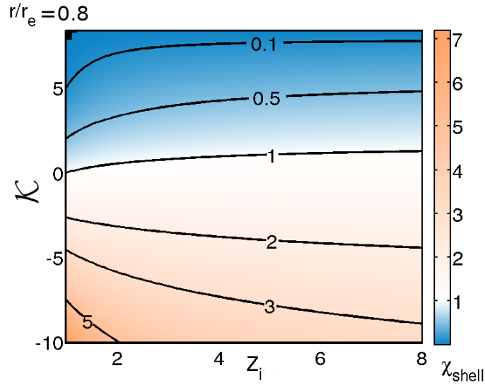
Figure 5.8: Shock pressure amplification \mathcal{X}_{\text{shell}} = \tilde{p}_{s_f}/\tilde{p}_{s_i} in the shell comoving frame as a function of (\mathcal{K}, Z_i) for a fixed value r_{in}/r_{out} = 0.8 .
