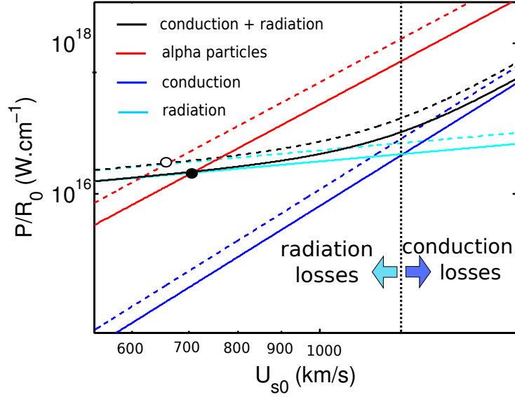
Figure 4.17: Powers of losses and gain in the hot-spot divided by the initial hot-spot radius. The initial areal density is \rho_0 R_0 = 50 \text{ mg.cm}^{-2} . The results for M_{s_0} = \infty are represented with dashed line, and for M_{s_0} = 5 with full lines.
