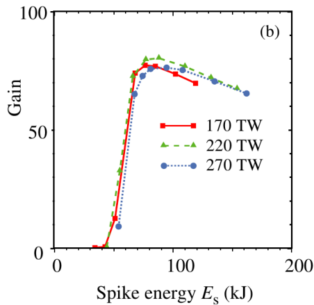
Figure 1.18: Gain versus the spike energy for three spike powers [Atzeni et al., 2011] for the HiPER baseline target SI implosions.
