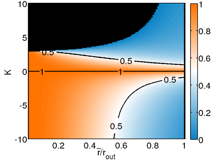
Figure 5.5: Contribution of the geometrical effect in the shock strengthening: |\mathcal{S}_r d \ln \tilde{R}_s| / (|\mathcal{S}_\rho d \ln \tilde{\rho}_0| + |\mathcal{S}_p d \ln \tilde{p}_0| + |\mathcal{S}_r d \ln \tilde{R}_s|) .
