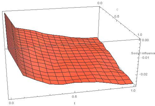
FIGURE 3.15 – Social Influence : Average of a_i^* - \hat{a}_i
