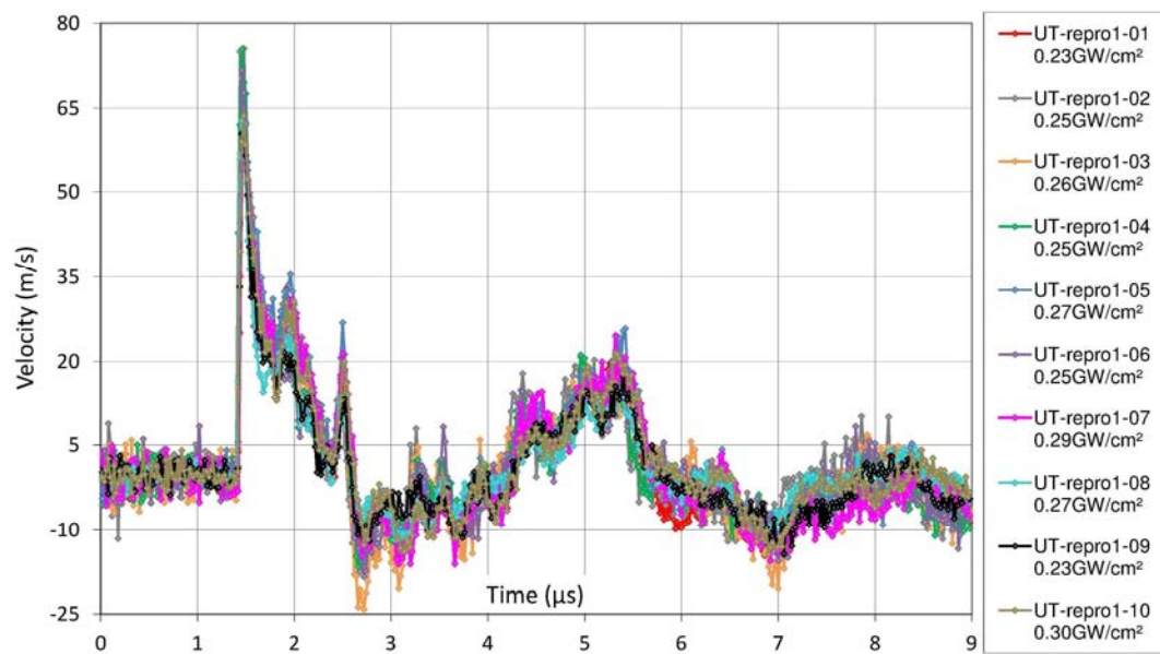
Figure 6.2, 10 successive VISAR measurements of the laser shocks performed on the same UT superposed to show the good reproducibility from one shock to the following
