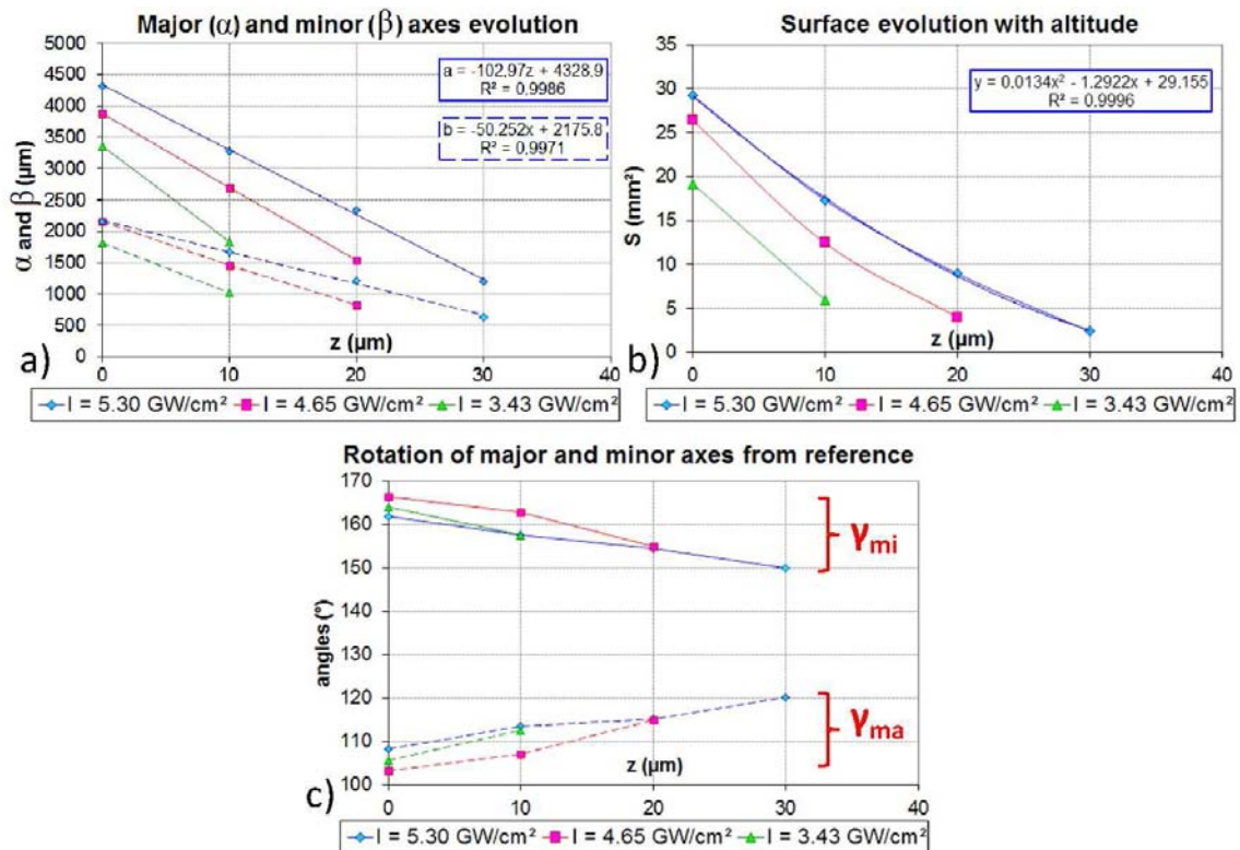
Figure 3.26, Analysis of the back face blister on T800/M21 samples: a) Evolution of the semi-minor (dash line) and semi-major axes (plain line) lengths versus the height of the contour line with the associated correlations, for the different laser intensities, b) Evolution of the in-plane deformation surface defined by the contour line versus the height level of the contour line with the associated correlation, for the different laser intensities, c) Evolution of the angles between the major and minor axes and the horizontal axis versus the height of the contour line, for the different laser intensities
