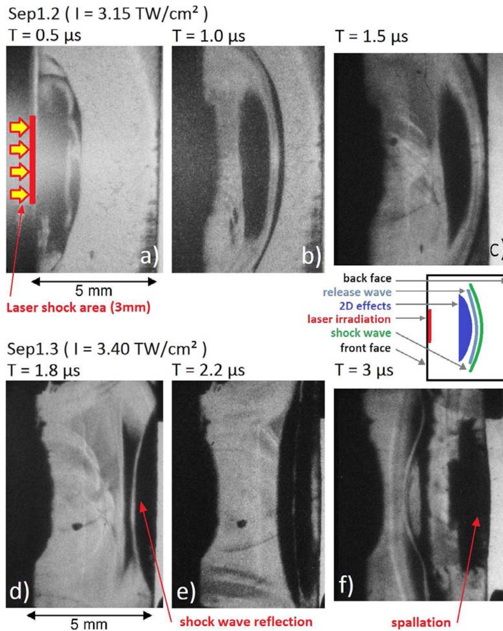
Figure 3.4 Laser shock wave propagation history obtained by shadowgraphy in epoxy resin:
