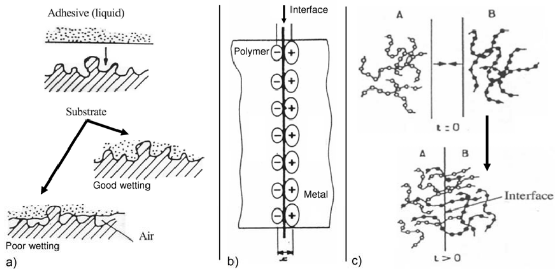
Figure 1.26 Adhesion mechanisms principle from G. Fourche [174], a) Sketch of the mechanical interlocking model in both good wetting and poor wetting cases, b) Sketch of the electrical model principle, c) Sketch of the diffusion model principle
