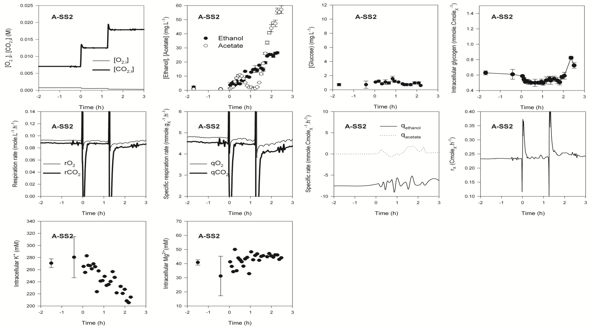
Figure 35. Overview of the yeast transient response to the 5.34 and 5.27 mM successive CO 2 shift-up. The shift-ups were performed at t = 0h and t = 1.28h respectively.
