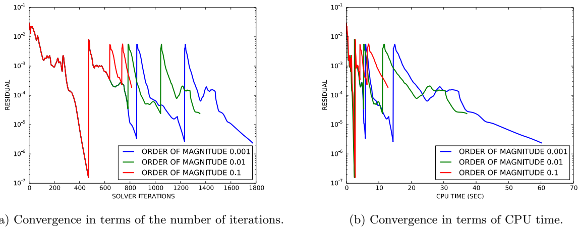
Figure 6.5: Comparison of the residual convergence for some input orders of magnitude.
