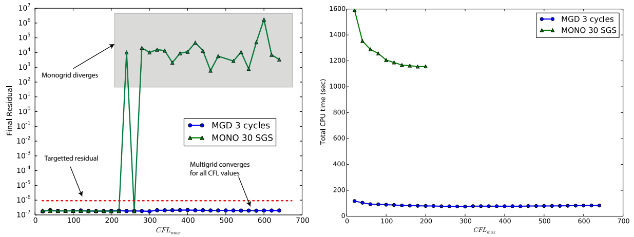
(a) Final residual wrt CFL_{max} . The targeted final residual was set to 10^{-6} . (b) Final CPU comparison wrt CFL_{max} . NB: the single-grid CPU is not plotted for CFL_{max} > 220 , as it failed converging.
