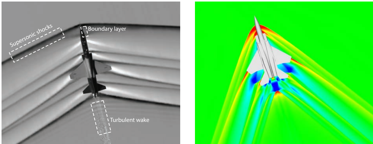
(a) A recent schlieren photograph of a T-38C flying at Mach 1.09 (Credit: NASA).
