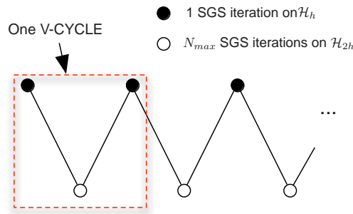
Figure 5.1: Bigrid V-cycle
