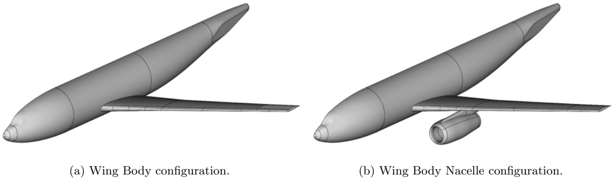
Figure 4.18: DPW2 geometries.
