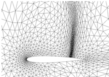
(d) Adapted mesh obtained after 3 stages of Algorithm 1 (2200 vertices).
