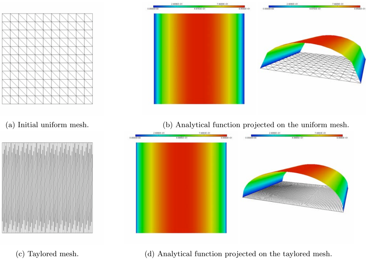
Figure 1.1: Simple analytical example that illustrates the minimization of the interpolation error using manual mesh modification.
