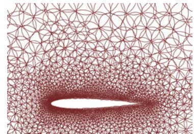
(c) Metric \mathcal{M}_{L^2,0} computed according to an error estimation of (\mathcal{H}_0, \mathcal{S}_0) .
