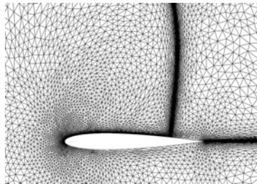
(e) After 10 stages (22000 vertices).
