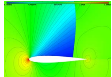
(f) Corresponding final solution at stage 10.
