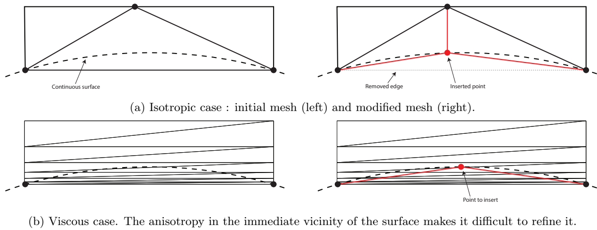
Figure 7.10: Illustration of one difficulty of surface reprojection when boundary layer meshes are involved.
