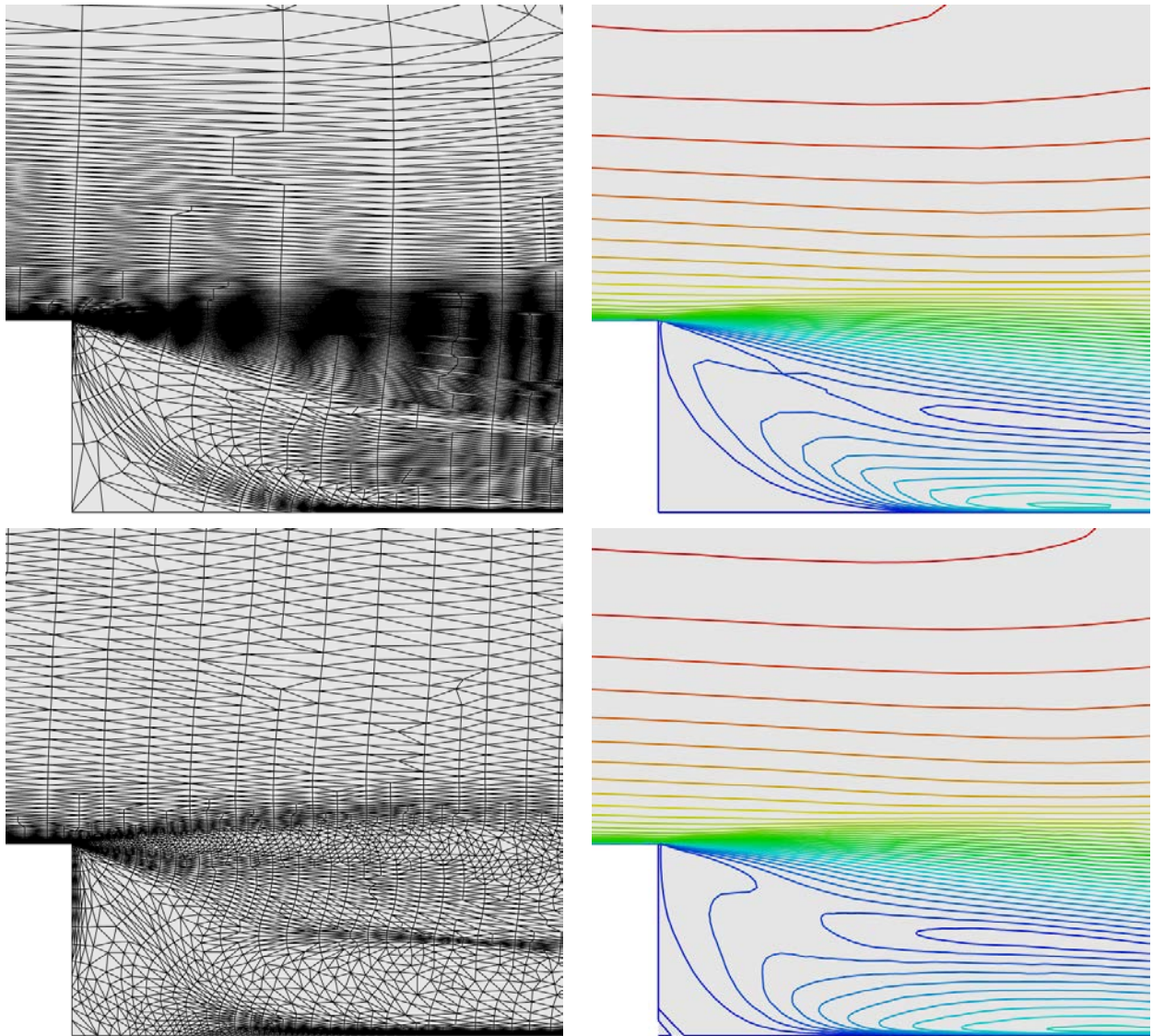
Figure 7.6: Backward facing step: Left, comparison of the meshes generated from \mathcal{M}_G (top) and \mathcal{M}_{LP} (bottom) near the corner at complexity 24 000. Right, iso-values of the norm of the velocity.
