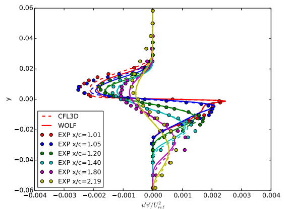
Figure 4.14: 2D airfoil near-wake.
