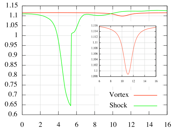
(b) Shock waves and vortices don't have the same magnitude, but must be captured altogether.
