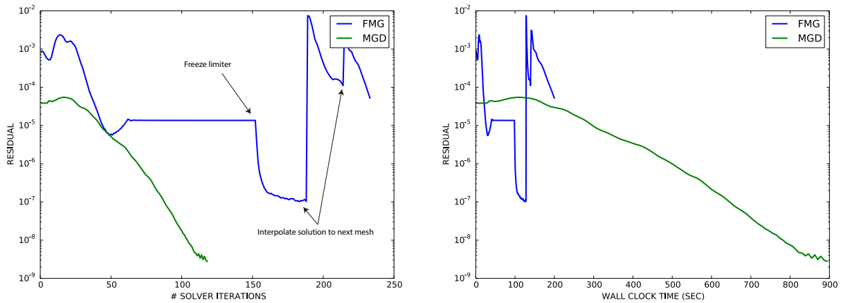
(a) Convergence in terms of the number of solver iterations.
