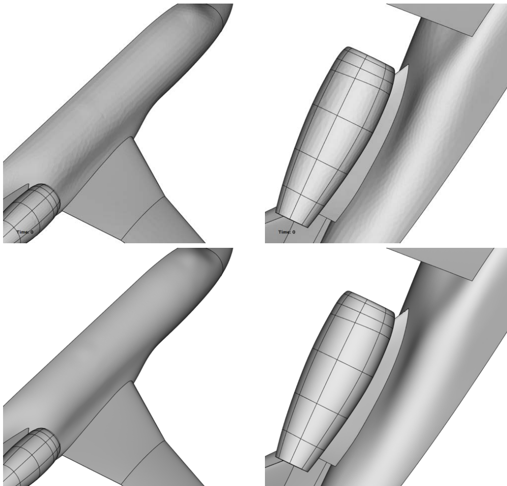
Figure 7.11: CAD projection: Falcon case: Illustration of the surface approximation without (top) and with (bottom) projecting the mesh to the CAD.
