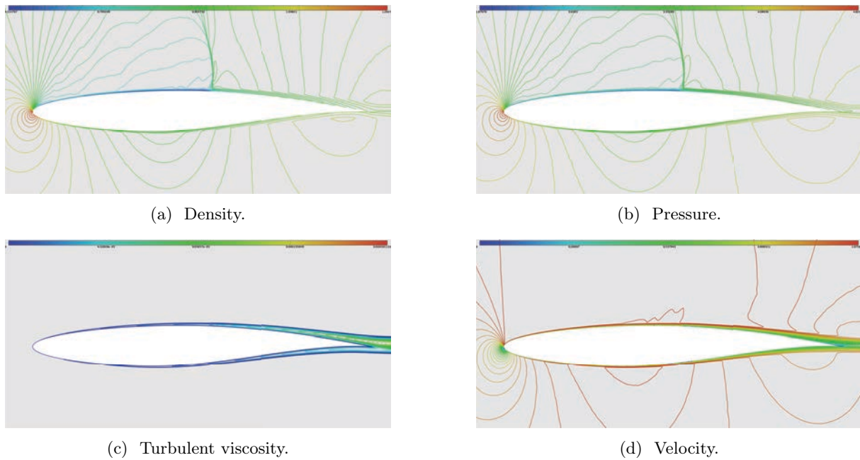
Figure 7.9: RAE 2822: isolines of the solution on the final adapted mesh.
