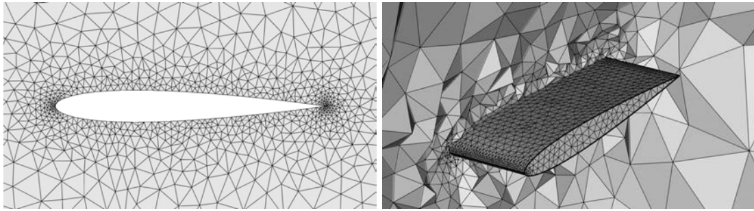
Figure 3: Examples of meshes 2D (left) and 3D (right) meshes of a NACA 0012 airfoil.
