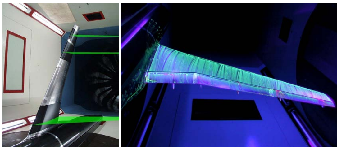
Figure 1: Wind tunnels are tube-shaped facilities, which use powerful fans to move air over a model of aircraft. It teaches a lot about the aircraft aerodynamics, and is extensively used during the design process. (Image credit: NASA).
