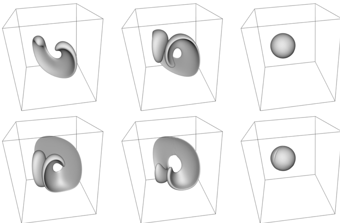
Figure A.15: Result of the final 3D mesh adaptation. The bubble's interface (iso-surface \rho = 0.95 ) at times t = \frac{T}{8}, \frac{T}{4}, \frac{T}{2}, \frac{3T}{4}, \frac{7T}{8} and T .
