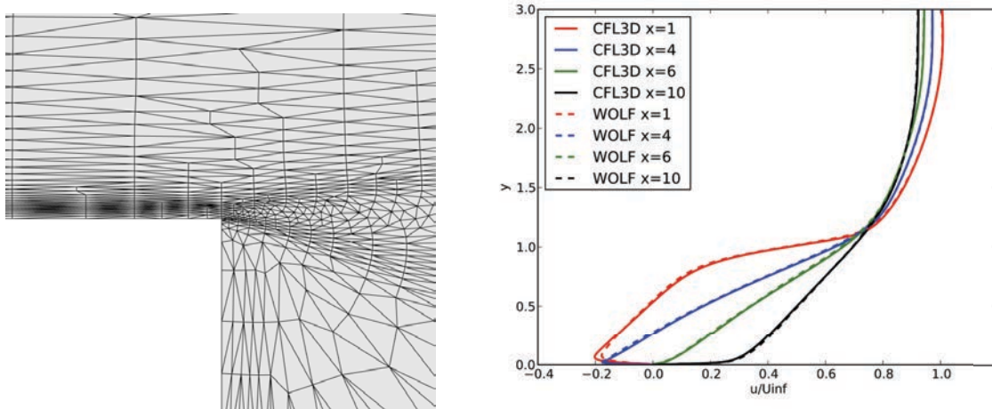
Figure 7.7: Backward facing step, metric \mathcal{M}_{Lp} : Left, mesh at complexity 24000, and comparison to CFL3D (whose solution was computed on the uniform reference mesh) of the velocity profiles.
