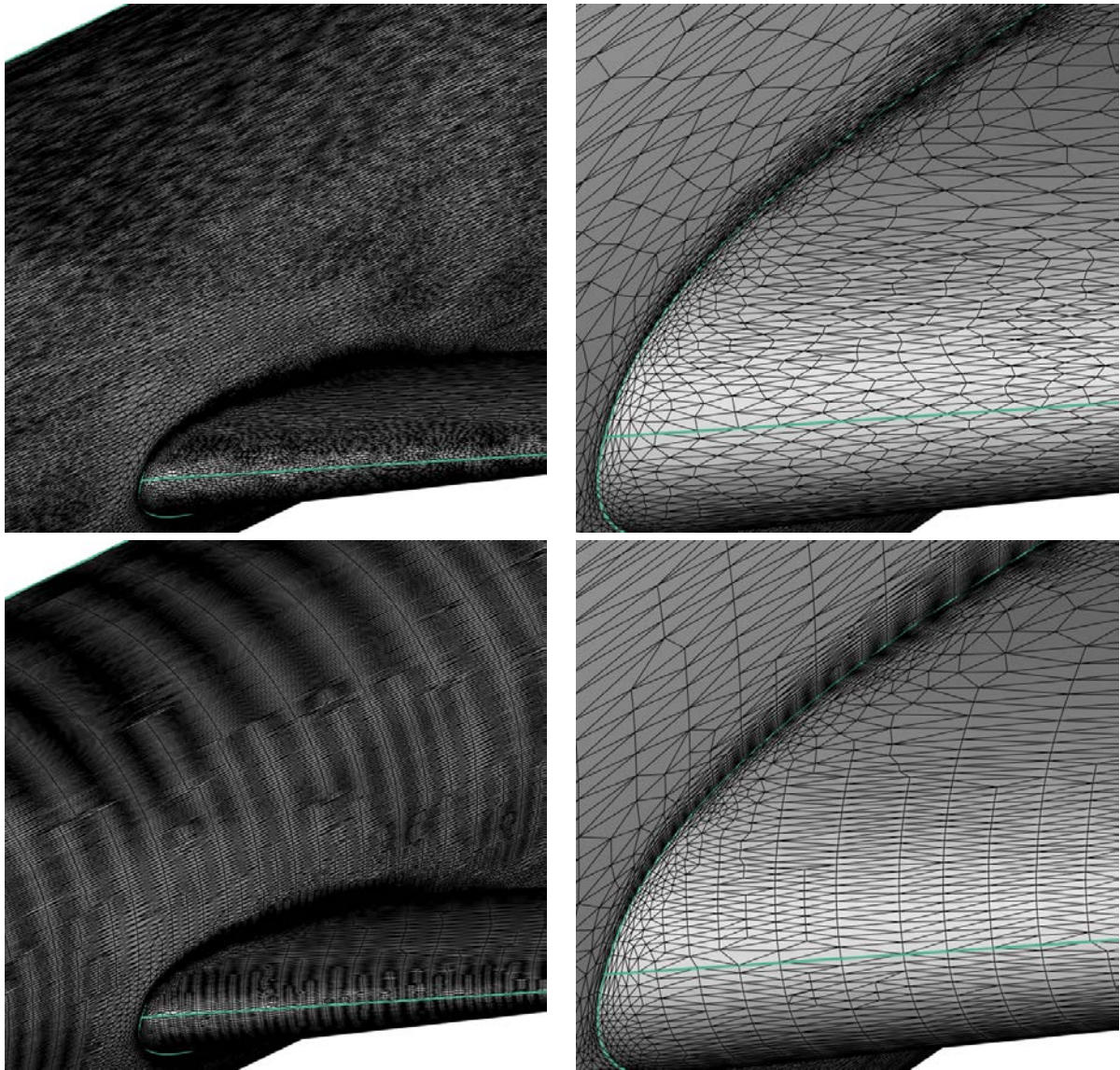
Figure 7.2: DPW2 test case: Generation of two adapted surface meshes with the standard approach (top) and the metric-aligned one (bottom).
