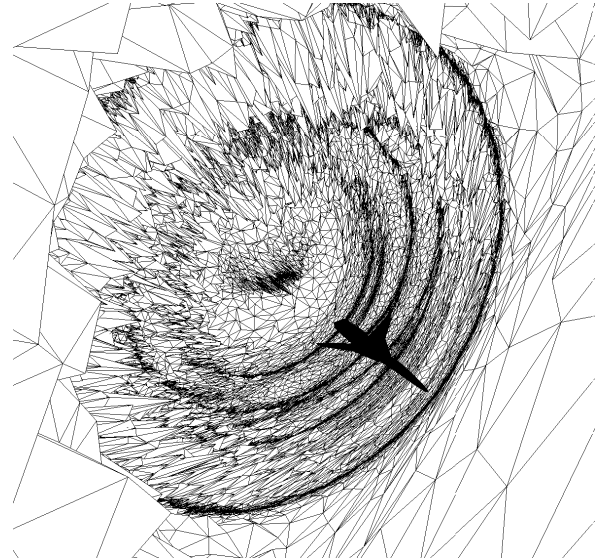
(c) Mesh adaptation result: solution (left) and adapted mesh (right).
