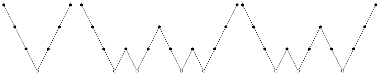
Figure 5.2: Four-grid methods : V-cycle, W-cycle and F-cycle ( \bullet : 1 smoothing SGS iteration, \circ : Several SGS iterations)
