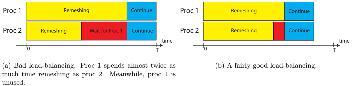
Figure 2.2: The domain partitioning step must preserve the load-balancing.
