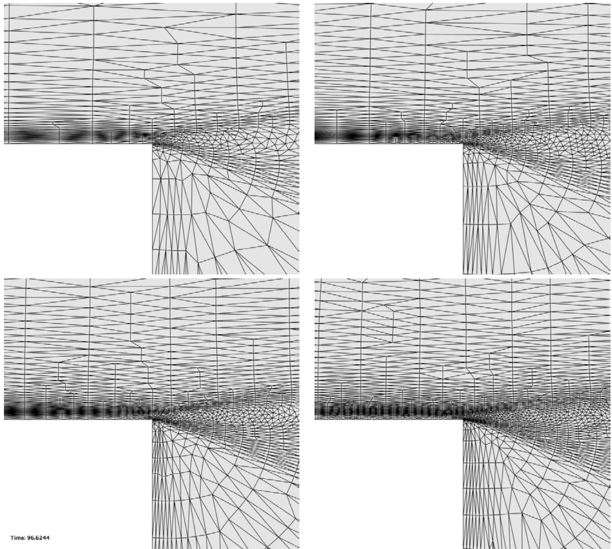
Figure 7.5: Backward facing step: mesh resolution around the corner for the complexity 24 K, to 36 K for the multi-field multi-scale metric from left to right, top to bottom.
