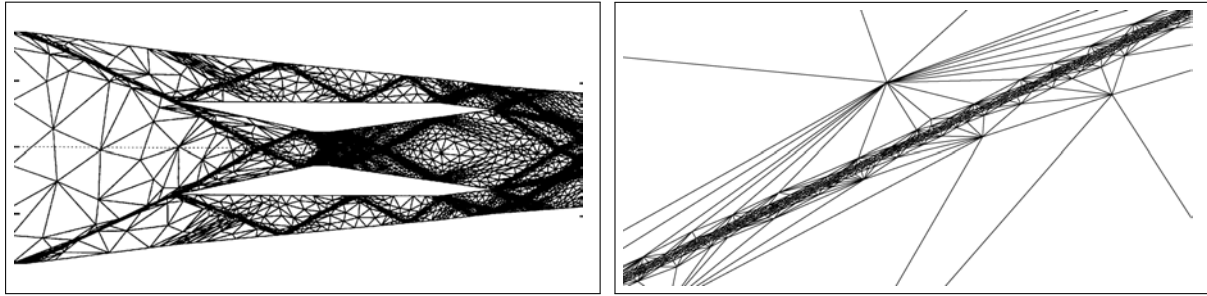
(a) Large view of the final adapted mesh.
