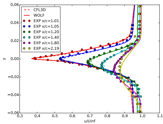
Figure 4.14: 2D airfoil near-wake.
