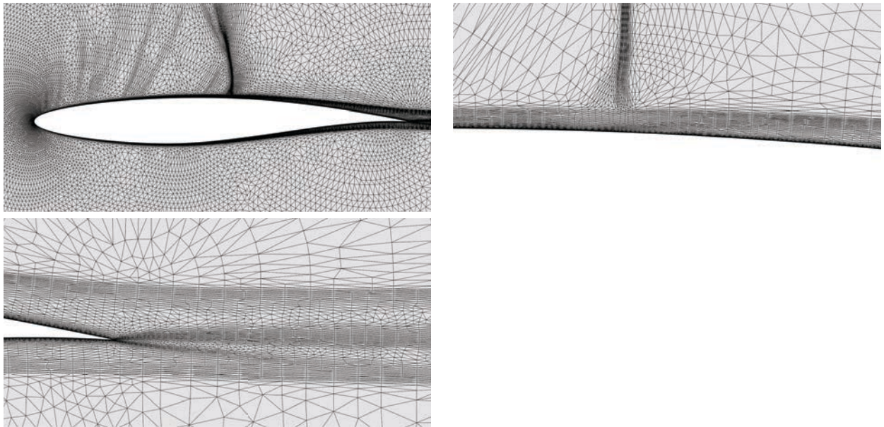
Figure 7.8: RAE 2822: Views of the final adapted mesh using the \mathcal{M}_G metric and the metric-aligned meshing method.
