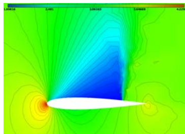
(b) Initial solution \mathcal{S}_0 .
