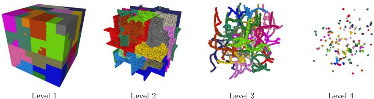
Figure 2.3: Recursive partitioning into 32 sub-domains of a cubic domain for a constant work per element. From left to right, level 1, 2, 3 and 4 of partitioning. We observe that the domain topology varies drastically with the level.
