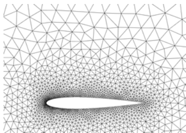
(a) Initial mesh \mathcal{H}_0 .
