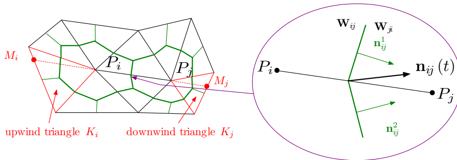
Figure 3.5: Illustration of finite volume cell construction in 2D: two neighbouring cells C_i and C_j and the upwind triangles K_i and K_j associated to edge P_i P_j .
