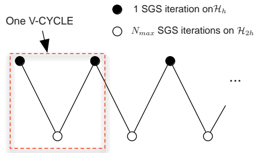
Figure 5.1: Bigrid V-cycle
