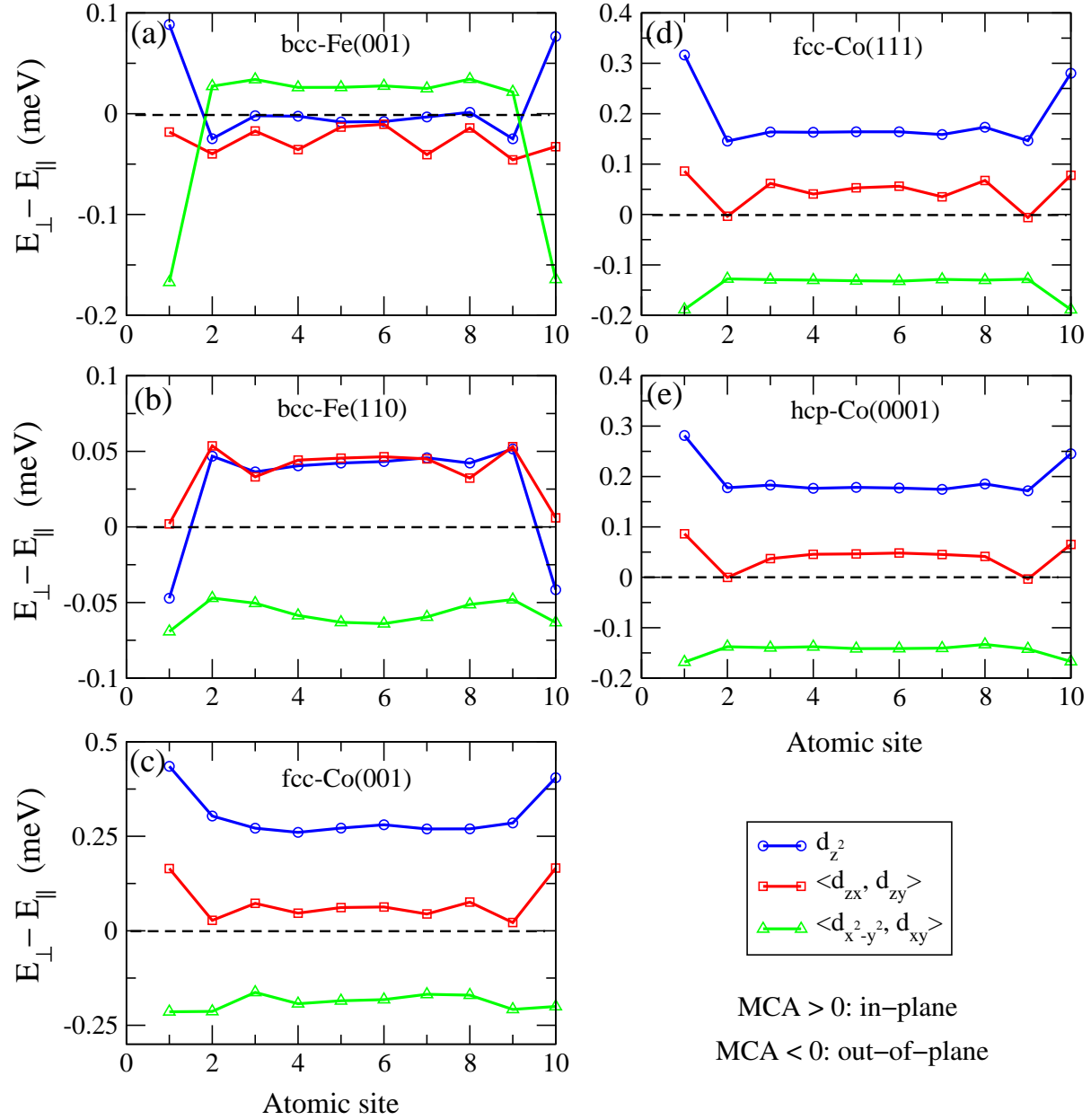
Figure 3.4: DFT results : d -orbitals decomposition of MCA for Fe and Co slabs made of 10 atomic layers : (a) bcc-Fe(001), (b) bcc-Fe(110), (c) fcc-Co(001), (d) fcc-Co(111) and (e) hcp-Co(0001). Due to symmetry, contributions from different orbitals in (d_{zx}, d_{zy}) and (d_{x^2-y^2}, d_{xy}) pairs are very similar so that their averaged values are presented for simplicity.
