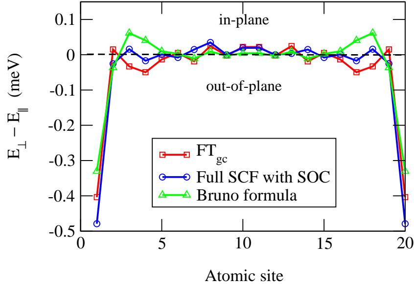
Figure 2.2: Layer-resolved MCA of the Fe(001) slab with N = 20 layers calculated using \text{FT}_{\text{gc}} approximation (red squares), full self-consistent calculation with SOC (blue circles) and the Bruno formula (green triangle ups). Note that the layer-resolved spin-projected orbital moments are obtained by self-consistent calculations.
