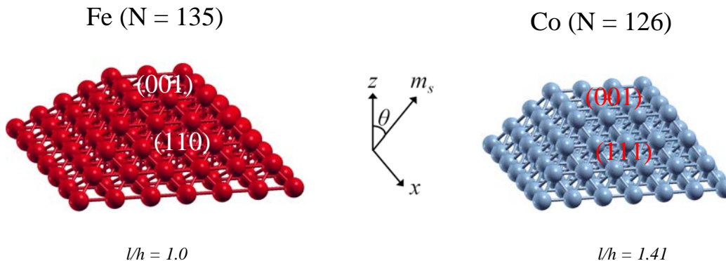
Figure 4.3: Examples of truncated-pyramid shaped Fe and Co nanocrystals studied in the present work. The crystals are made of bcc-Fe and fcc-Co with two types of facets : (001) and (110) for Fe and (001) and (111) for Co, respectively. Their possible size and shape is controlled by length-to-height ratio, l/h , kept to \sim 1.0 (Fe) and 1.41 (Co) which are close to experimental values, \sim 1.20 (Fe) [3] and \sim 1.48 (Co) [25]. The z axis was chosen to be normal to the pyramid base and the spin moment is rotated in the xz plane forming the angle \theta with the z axis.
