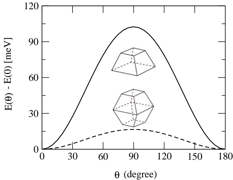
Figure 4.6: Total MCA as a function of angle \theta for a Fe truncated pyramid ( N = 620 ) and a Fe truncated bipyramid ( N = 1020 ). For the latter one the MCA is strongly reduced because of the much smaller area of (001) facets.
