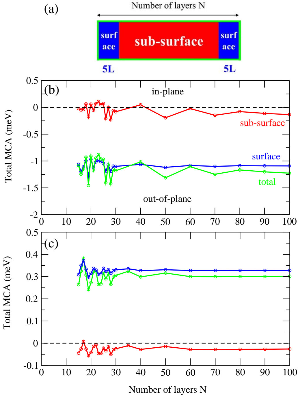
Figure 3.2: TB results : (a) Schematic presentation of N -atom slabs with surface and sub-surface contribution. The surface contribution is obtained by summing the MCA over the five outer layers of the unit cell on each side of the slab. Surface (blue), subsurface (red) and total MCA (green) per unit cell of N -atom for (b) bcc-Fe(001) and (c) bcc-Fe(110) slabs as a function of the number of atomic layers N in the slab. Positive (negative) MCA values mean in-plane (out-of-plane) easy-axis direction. The two different slabs orientations have MCA of opposite sign.
