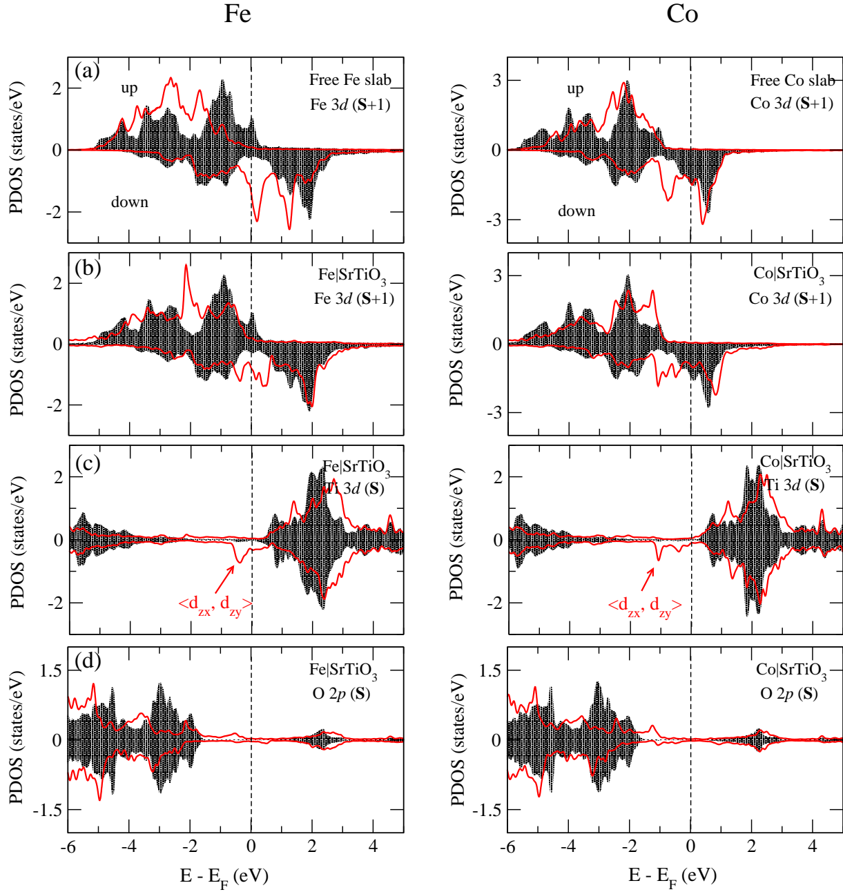
Figure 5.3: (a) Free Fe slab : Scalar-relativistic projected density of states (PDOS) of the surface Fe 3d orbitals in layer S+1 ; Fe|SrTiO 3 (001) : PDOS of (b) Fe 3d orbitals in layer S+1 , (c) Ti 3d and (d) O 2p orbitals in layer S . The shaded plots are the DOS of atoms in the central monolayer of Fe slab (a, b) or (c, d) TiO 2 in layer S-2 . Positive and negative PDOS are for spin up and spin down channels, respectively. The vertical dashed lines indicate the Fermi level ( E_F ). It is the same for Co as presented in the right panels.
