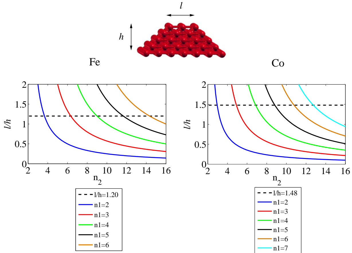
Figure B.1: The ratio of the length ( l ) of the top square to the height ( h ) of the Fe (left) and Co (right) truncated pyramids with respect to n_2 as a given n_1 . Note that n_2 \times n_2 and n_1 \times n_1 are the number of atoms in the first (bottom) and last (up) layers of the truncated pyramids. The experimental value of l/h is also indicated as a black dotted line.
