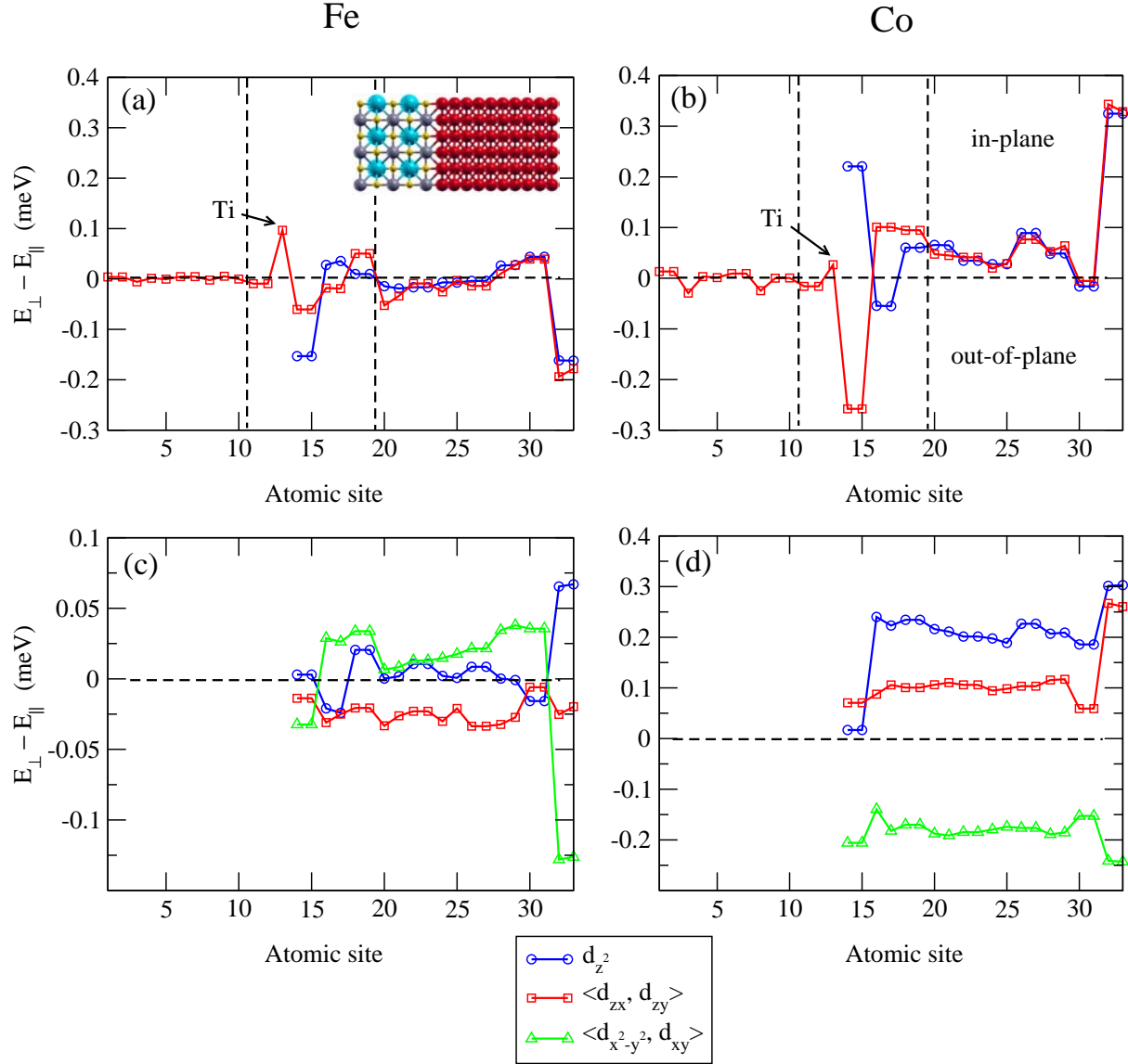
Figure 5.4: Atom-resolved MCA at Fe|SrTiO 3 (a) and Co|SrTiO 3 (b) interfaces, blue circles and red squares correspond to free slab and slab on a SrTiO 3 substrate. d -orbitals-resolved MCA for Fe (c) and Co (d) slabs on SrTiO 3 , we plot only the part of ferromagnetic slabs. Due to symmetry, contributions from different orbitals in (d_{zx}, d_{zy}) and (d_{x^2-y^2}, d_{xy}) pairs are very similar so that their averaged values are presented for simplicity. Note that positive and negative MCA represent in-plane and out-of-plane magnetization, respectively.
