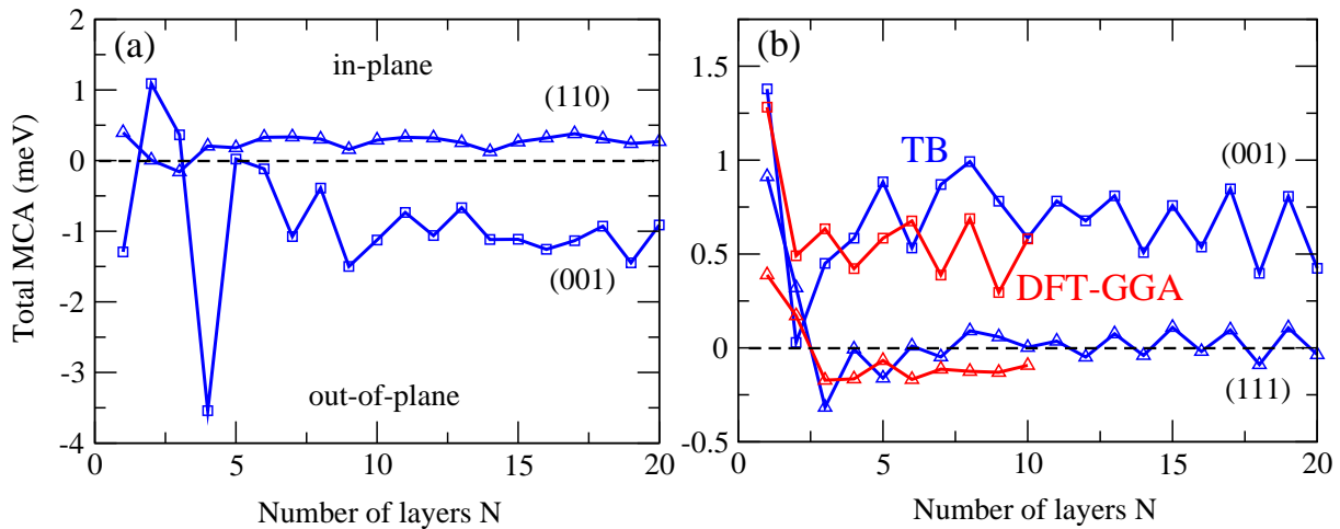
Figure 3.1: Total MCA per unit cell, E_{\perp}^{\text{band}} - E_{\parallel}^{\text{band}} , of N -atom-thick bcc-Fe and fcc-Co slabs as a function of the number of layers N . Squares and triangle ups are for two different orientations of Fe and Co slabs, respectively. In the case of fcc-Co slabs, TB calculations (blue) are compared with ab initio DFT-GGA calculations (red)
