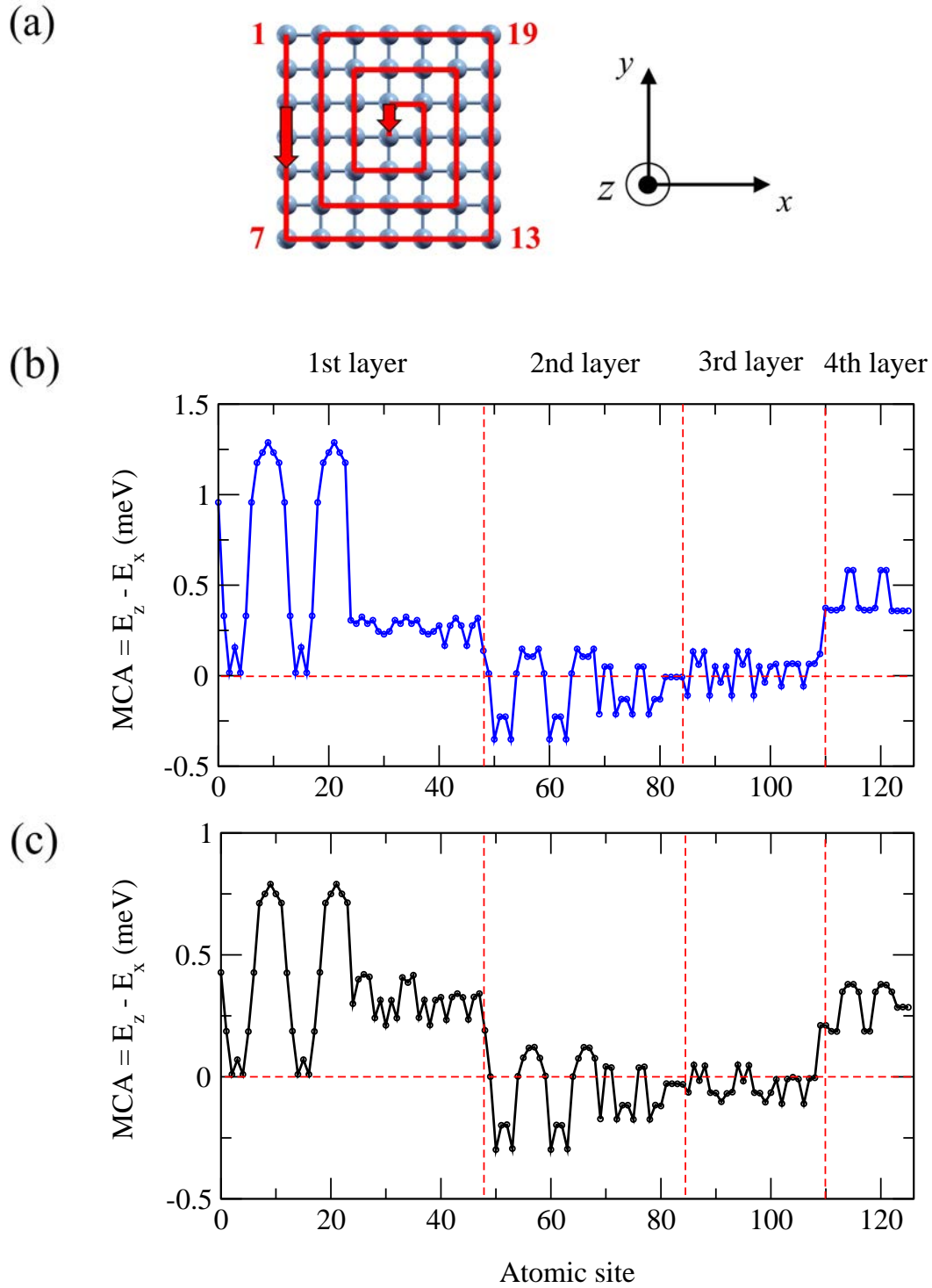
Figure 4.7: Atom-resolved MCA for Co nanocrystal made of 126 atoms : (a) trajectory for numbering the base layer atoms starting from the corner and going along the spiral to the center. The atoms of other layers are numbered in the similar way. (b) MCA per atom in meV within TB approach. (c) MCA per atom in meV from DFT-GGA calculations.
