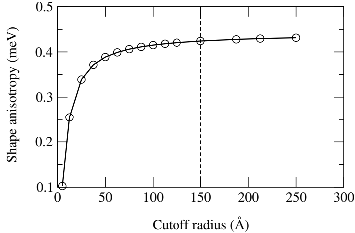
Figure C.1: Convergence test : Shape anisotropy energy with respect to the cutoff radius of a 5-layer Fe-bcc(001) slab. The cutoff radius of 150 Å is used in the following to get well-converged shape anisotropy energy.
