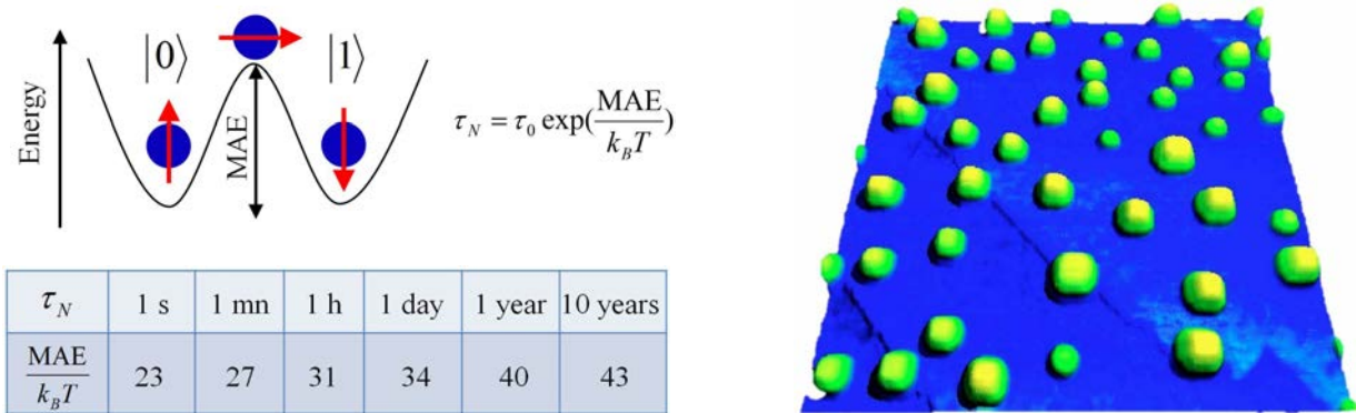
Figure 1: Left : Néel relaxation time \tau_N – a mean time between two flips of the magnetic moment – with respect to the magnetic anisotropy energy MAE (over temperature), where k_B is the Boltzmann constant, T is the temperature and \tau_0 is the attempt time (typical values of which are between 10^{-9} and 10^{-10} seconds). Right : 3D representation of scanning tunneling microscopy (STM) topography of truncated pyramid-shaped Fe nanocrystals of nanometer-size grown on \text{SrTiO}_3(001) substrate [3].
