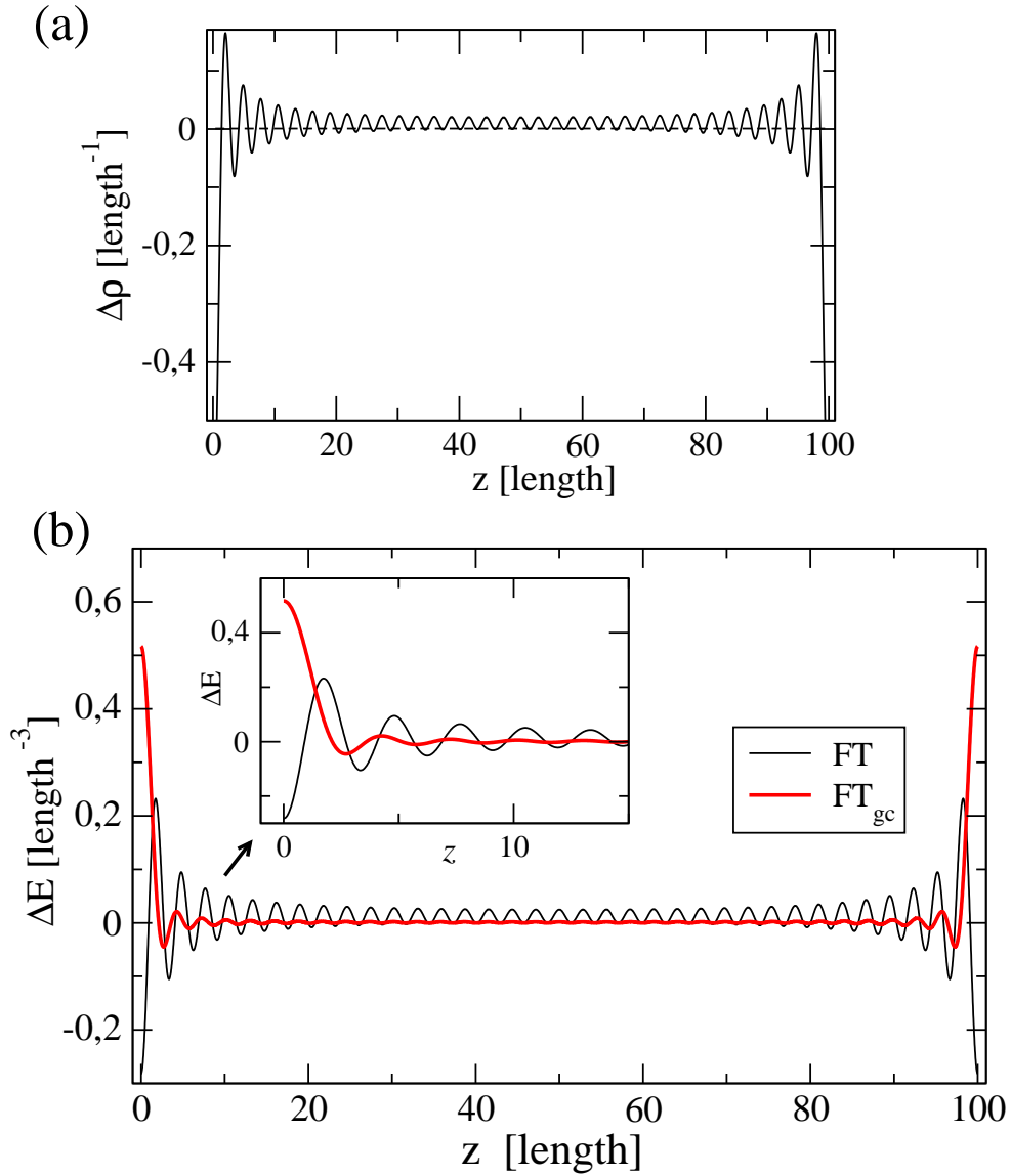
Figure A.1: Graphical representation of the functions \Delta E(z) , \Delta E_{gc}(z) , and \Delta\rho(z) for a one-dimensional electron gas confined by infinite barriers in the box of the length L . The discretized calculations were done with the parameters N = 70 (total number of electrons) and L = 100 .
