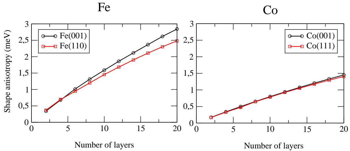
Figure C.2: Shape anisotropy energy of bcc-Fe (left) and fcc-Co (right) N -layer slabs with two different orientations. Note that the spin moments are taken from a tight binding calculation.
