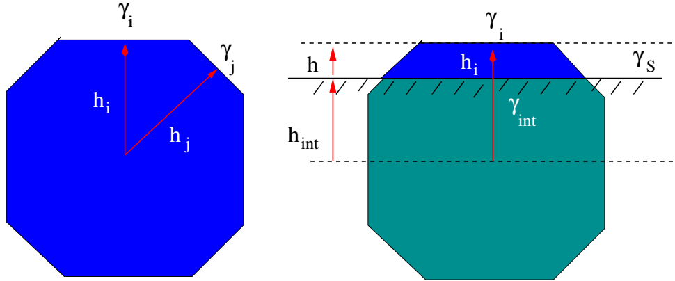
Figure 4.2: Wulff (left) and Wulff-Kaichev (right) construction to determine the equilibrium shape of a free or supported crystal.
