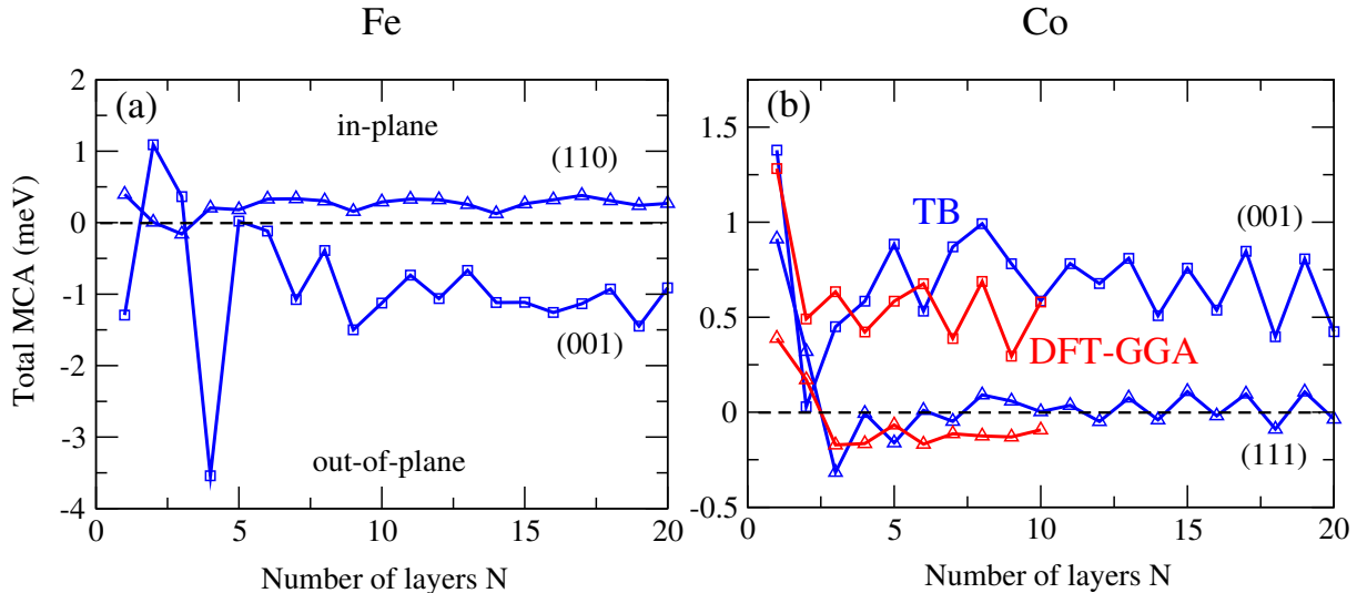
Figure 3.1: Total MCA per unit cell, E_{\perp}^{\text{band}} - E_{\parallel}^{\text{band}} , of N -atom-thick bcc-Fe and fcc-Co slabs as a function of the number of layers N . Squares and triangle ups are for two different orientations of Fe and Co slabs, respectively. In the case of fcc-Co slabs, TB calculations (blue) are compared with ab initio DFT-GGA calculations (red)
