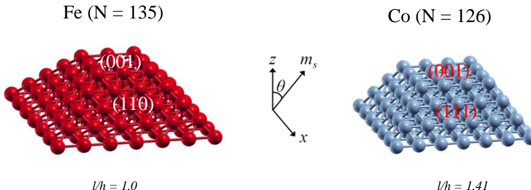
Figure 4.3: Examples of truncated-pyramid shaped Fe and Co nanocrystals studied in the present work. The crystals are made of bcc-Fe and fcc-Co with two types of facets : (001) and (110) for Fe and (001) and (111) for Co, respectively. Their possible size and shape is controlled by length-to-height ratio, l/h , kept to \sim 1.0 (Fe) and 1.41 (Co) which are close to experimental values, \sim 1.20 (Fe) [3] and \sim 1.48 (Co) [25]. The z axis was chosen to be normal to the pyramid base and the spin moment is rotated in the xz plane forming the angle \theta with the z axis.
