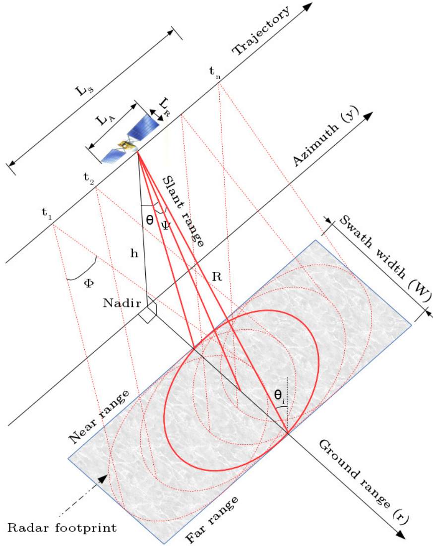
Figure 2.1: SAR acquisition.
