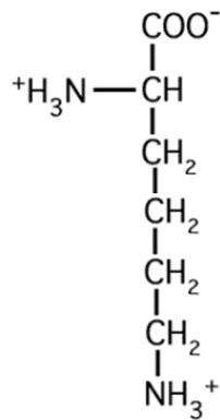
Figure 12.6 : Lysine
