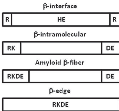
Figure 10. Schematic of the charge distribution in \beta -interactions. The amino acids are indicated using the single letter code. doi:10.1371/journal.pone.0032558.g010
