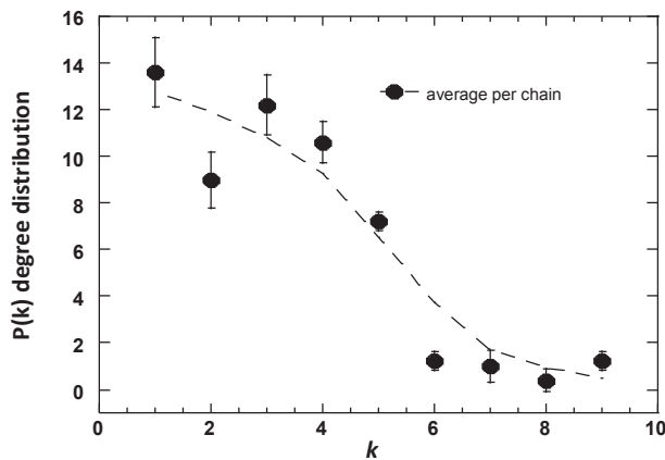
Figure 1: Degree distribution
