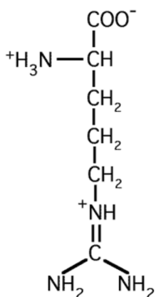
Figure 12.8 : Arginine
