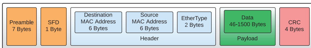
FIGURE 3.1: Ethernet Type II Frame format
