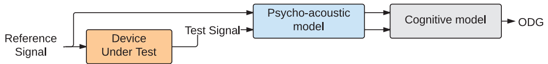
FIGURE 4.2: PEAQ principle
