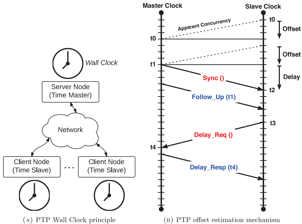
FIGURE 3.13: PTP principle
