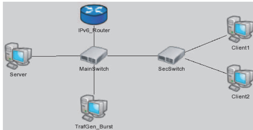
FIGURE 3.23: OmNet++ Simulation Topology.
