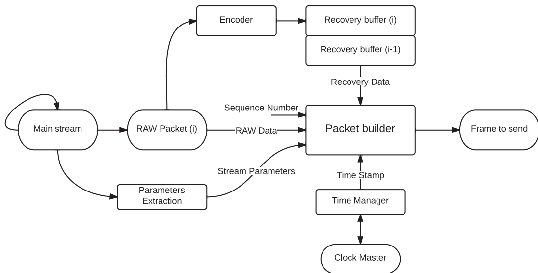
FIGURE 3.15: Packet building mechanism
