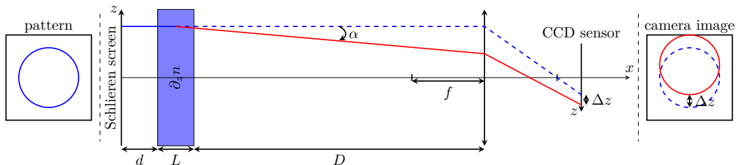
Figure 2.6: Schematics of the Schlieren visualization setup. The rays of light generated from luminous screen traverse a pattern (a circle in this example). The camera of focal length f and CCD sensor, is focused on the Schlieren screen. The stratified fluid between the screen and the camera shifts the position of the circle at the CCD sensor in \Delta z . Extracted from [7].
