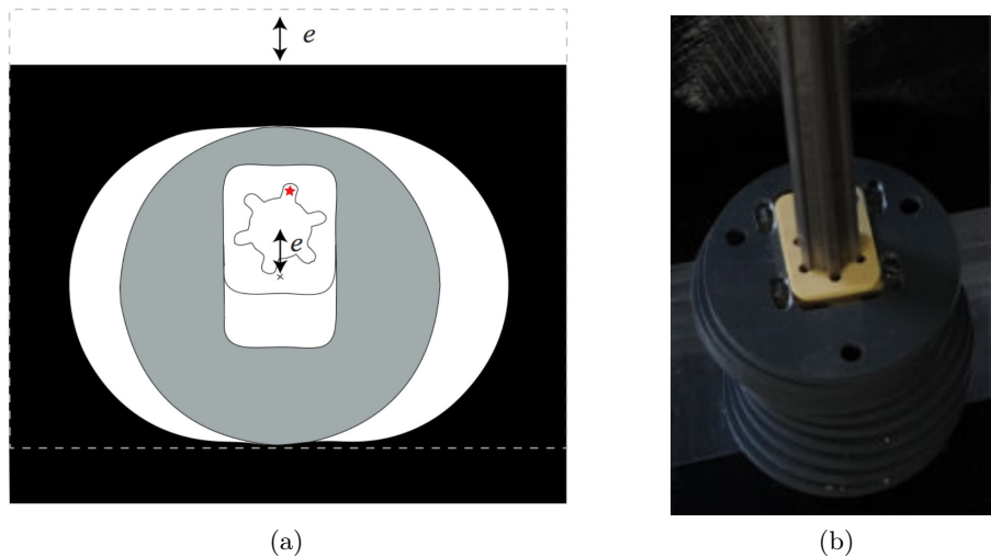
Figure 2.3: (a) Representation of the disc and plate system which transforms the rotation motion into a unidirectional translation. The white piece within the disc can be displaced to change the eccentricity e , and therefore, the translation amplitude of the black plate. (b) Image of discs piled over the camshaft (the discs are continuously shifted in phase). Extracted from [6, 7].
