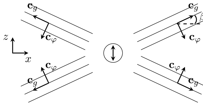
Figure 1.1: The four possible configurations of internal wave beams created by an oscillating body at fixed frequency.
