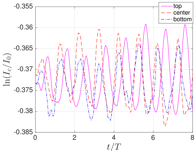
Figure 5.10: Oscillation of the concentration of particles in the column. \ln(I_c/I_0) as a function of time, measured for the regions indicated with three squares in figure 5.9(a).
