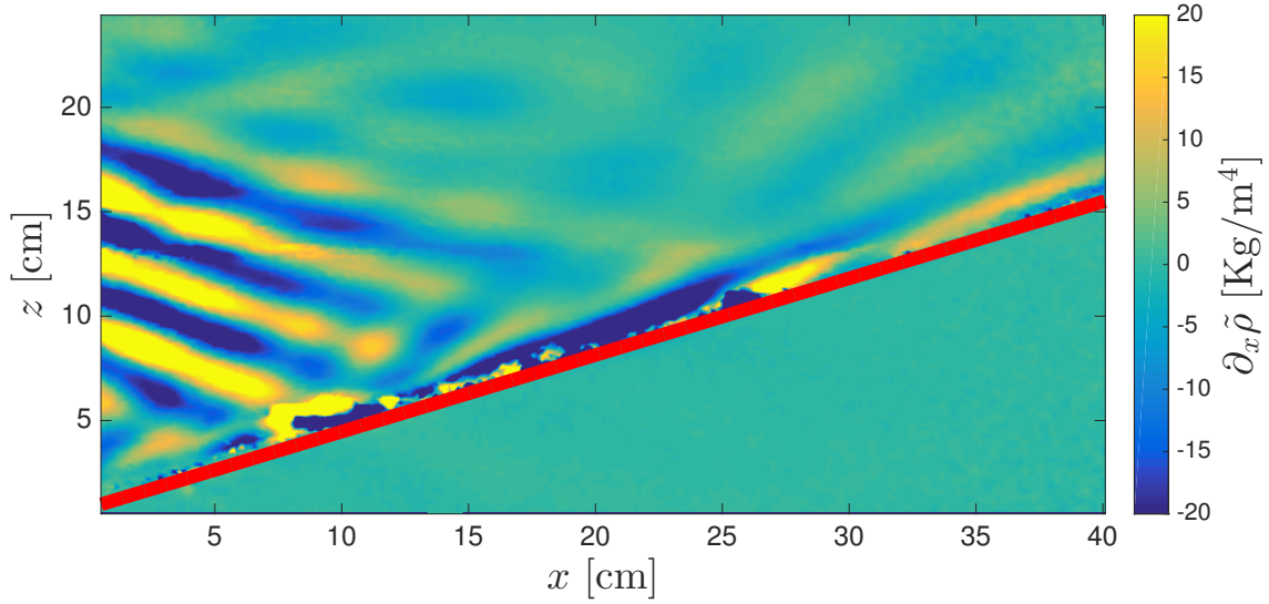
Figure 3.19: Snapshot of the wavefield of a plane wave propagating from left and reflecting over an oblique slope (indicated with a red line).
