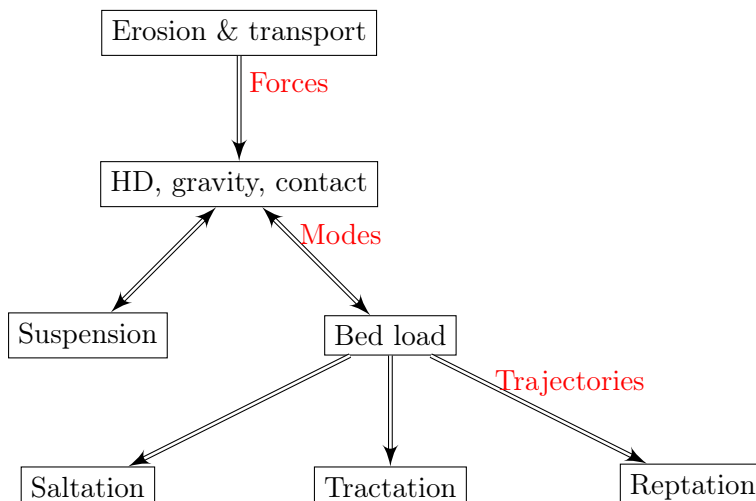
Figure 3.2: Diagram of the different types of granular transport separated by modes and trajectories, which respond to a particular combination of the relative hydrodynamic, gravity and contact forces acting over an individual grain.
