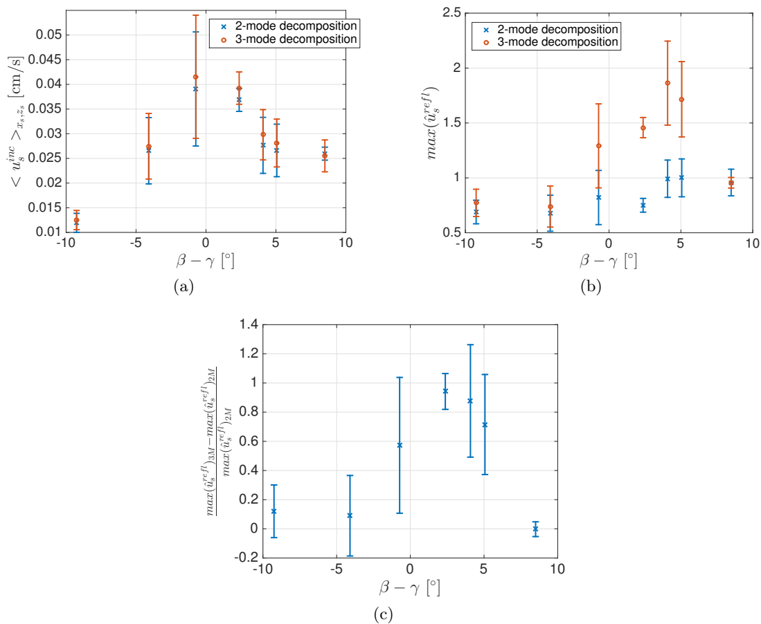
Figure 4.15: (a) u_s^{inc} as a function of \beta - \gamma for two- and three-mode decomposition (b) \max(\hat{u}_s^{refl}) as a function of \beta - \gamma for two- and three-mode VMD decomposition. (c) Normalized difference for \max(\hat{u}_s^{refl}) between two- and three-mode decomposition.
