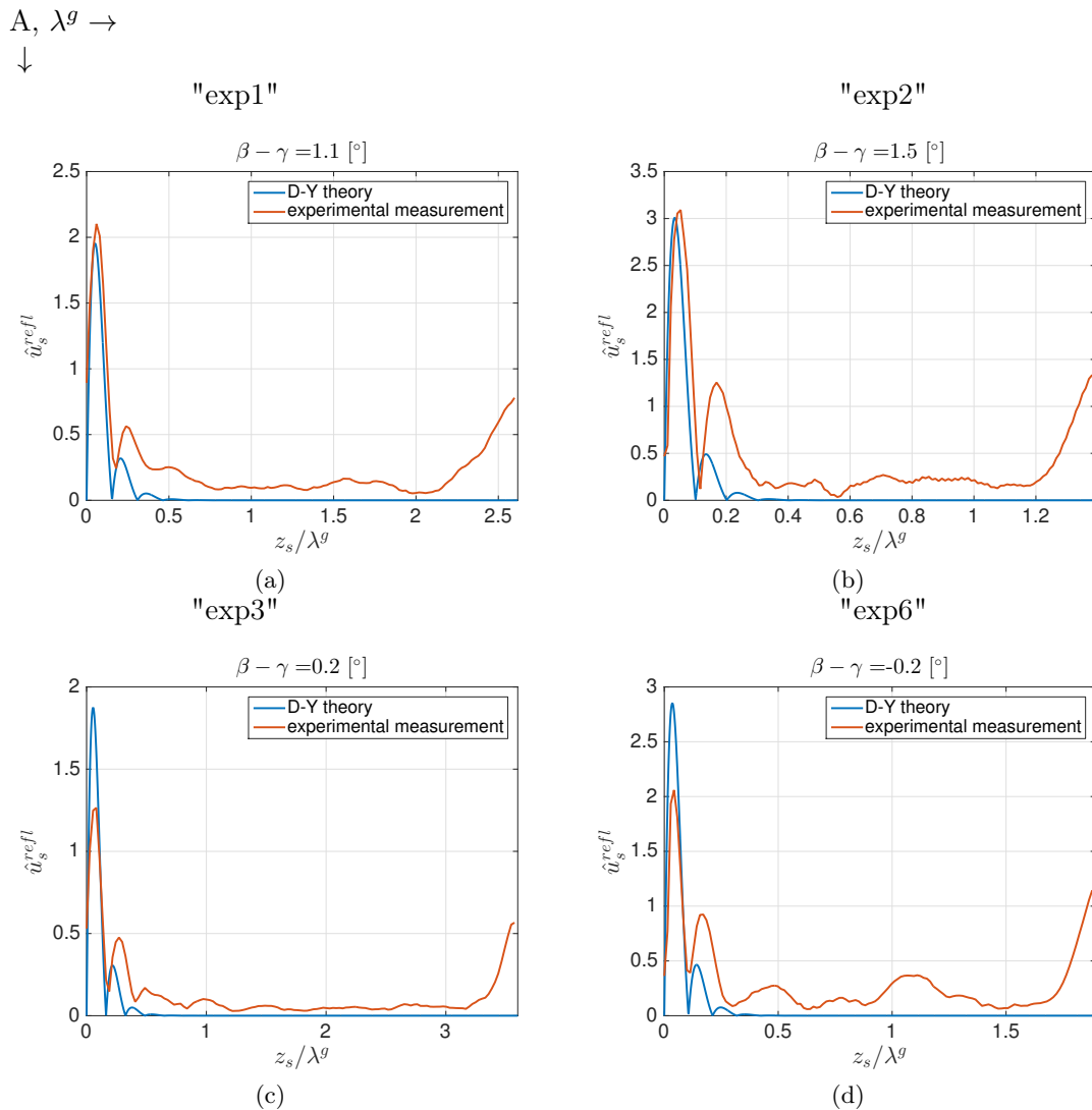
Figure 4.17: \hat{u}_s^{refl} as a function of z_s/\lambda^g for experiments (order in increasing Re number): (a) "exp1", (b) "exp2", (c) "exp3" and (d) "exp6". The experiments present different set of parameters A and \lambda^g , and at the top left it is indicated in which sense these two parameters increases.
