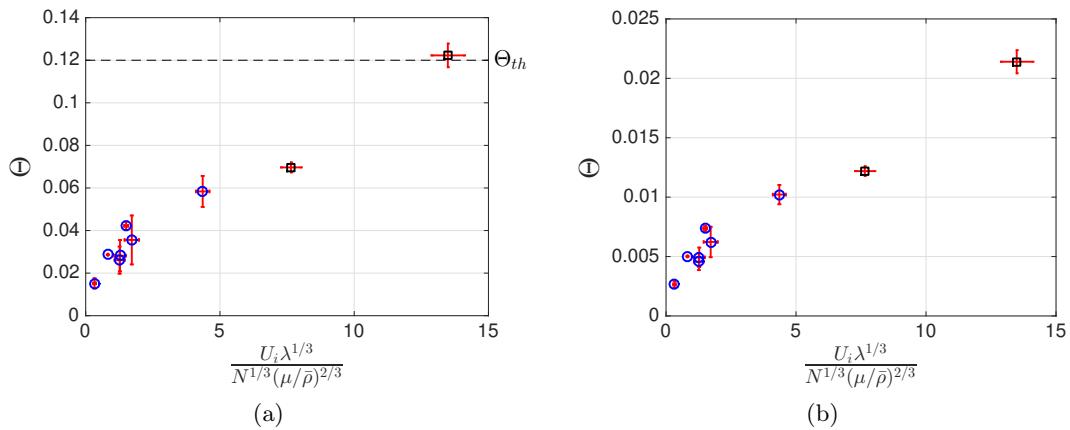
Figure 4.24: Shields number \Theta as a function of \frac{u_s^{inc} \lambda^{1/3}}{\nu^{2/3} N^{1/3}} for all experiments presented in table 4.1, computed for hollow glass particles (a) and Polystyrene particles (b). The experiments for which the forcing is performed with plane waves are indicated with circles (○), whereas the squares (□) indicate the experiments performed with vertical mode.
