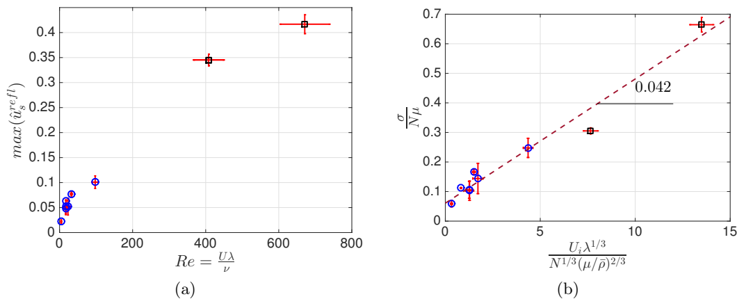
Figure 4.23: \max(\hat{u}_s^{refl}) obtained for the most critical reflection of each experiment (smallest |\beta - \gamma| ), as a function of the Re number (a). Dimensionless shear stress \frac{\sigma}{N\mu} for the most critical reflection as a function of \frac{u_s^{inc} \lambda^{1/3}}{\nu^{2/3} N^{1/3}} (b), with a dashed line is plotted the linear regression performed to the experimental results. The experiments for which the forcing is performed with plane waves are indicated with circles (o), whereas the squares ( \square ) indicate the experiments performed with vertical mode.
