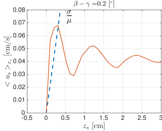
Figure 4.18: \langle u_s \rangle_{x_s} as a function of z_s for positions close to the boundary slope (located at z_s = 0 ). With a dashed blue line is indicated the slope of the first peak from which the shear stress \sigma is estimated. The experiment used here to illustrate how \sigma is obtained is "exp3".
