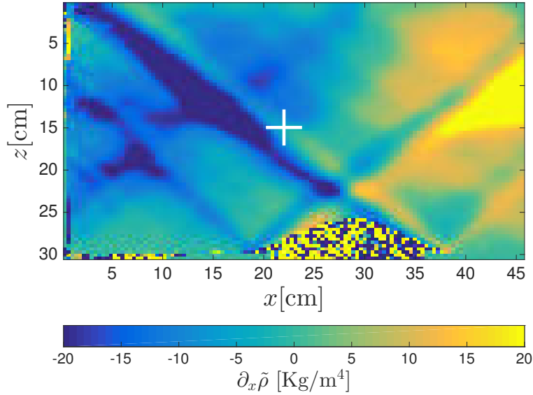
Figure 3.13: Snapshot of the wavefield generated by a vertical profile mode for t/T = 300 . The mountain of particles is centered at 27 cm from the wave generator, and acts as a source of waves. A white cross indicates the position where the time evolution of the wavefield is taken.
