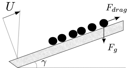
Figure 3.4: Schematics showing the forces acting over a individual grain located in a bed over an inclined slope underneath an horizontal stationary flow.
