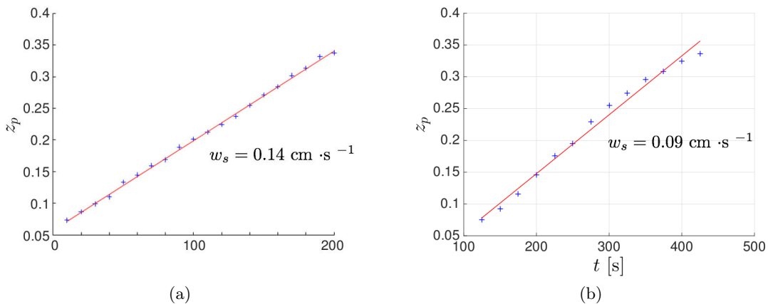
Figure 5.5: Depth of the particles front z_p as a function of time, for (a) a stratification with buoyancy frequency N = 0.8 \text{ rad}\cdot\text{s}^{-1} and (b) for N = 1.1 \text{ rad}\cdot\text{s}^{-1} . The line shows the result of a linear regression.
