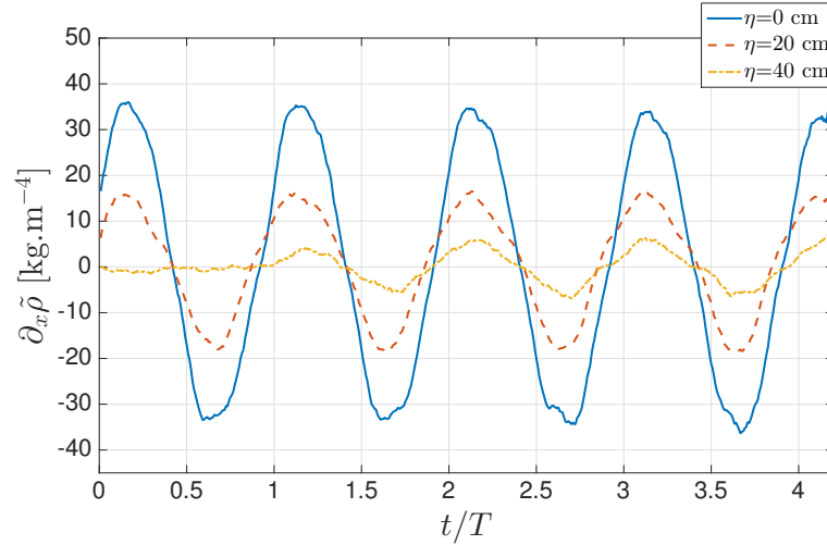
Figure 5.7: \partial_x \tilde{\rho} as a function of time of the internal plane waves for three points of the segment OP , illustrated in figure 5.6. The distance from O is indicated in the legend. The signal with smallest amplitude corresponds to the wavefield at the right side of the column.
