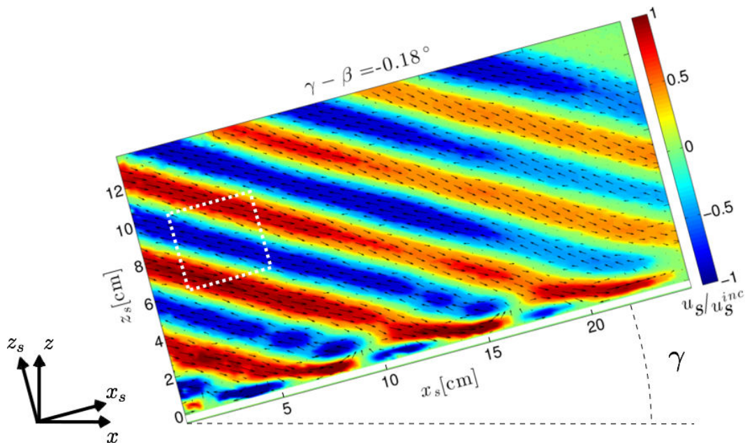
Figure 4.3: Snapshot of the normalized velocity field at t/T = 15 . The plot is tilted similarly to the experiment in order to illustrate the inclination of the slope \gamma = 16^\circ . x , z and x_s , z_s coordinates are indicated. The slope boundary is located at z_s = 0 . The background color indicates the u_s velocity component normalized by the along-slope component of the incident velocity u_s^{inc} = 0.1 cm/s, and arrows represent the velocity field. The incident wave is coming from left to right, and the generator is located 30 cm from the center of the image. This experiment corresponds to the case "exp3" indicated in table 4.1.
