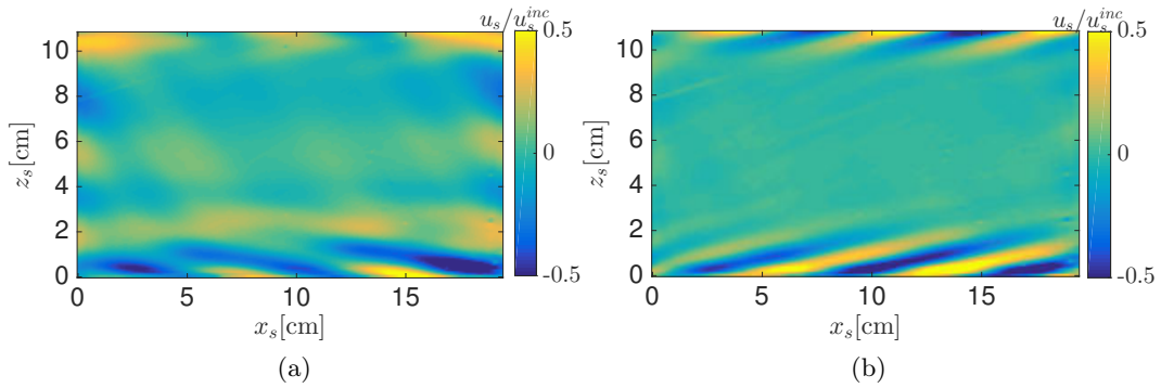
Figure 4.13: Normalized velocity field of experiment "exp4" corresponding to the downward (a) and the upward mode (b) of the reflected wave obtained through three-mode VMD decomposition. For this experiment \beta - \gamma = -0.7^\circ .
