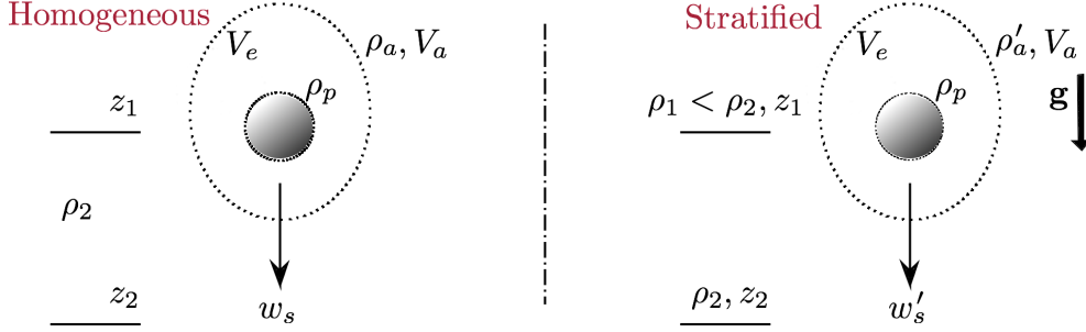
Figure 3.6: Sketch of a particle in sedimentation. On the left side of the sketch, the particle is in a homogeneous fluid with density \rho_2 . On the right, the particle is in a stratified fluid in which density increases with depth, going from \rho_1 at the top to \rho_2 below ( \rho_1 < \rho_2 ). To indicate the entrainment of fluid in the boundary of the particle a dotted circle is drawn around the particle.
