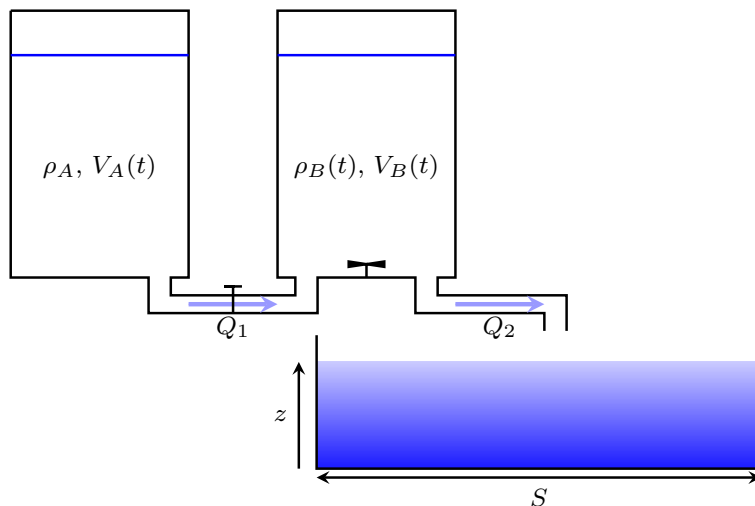
Figure 2.1: Schematics of the double bucket method for the generation of a linear stratified density profile. Extracted from [7].
