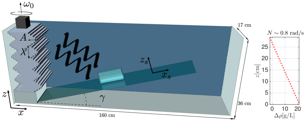
Figure 4.2: Sketch of the experimental setup. On the left of the tank is the wave generator (plane waves). A slope is introduced in the tank. Coming from the generator, the internal waves propagate from up-left to down-right as illustrated. The field of view is represented with a tilted rectangle over the slope. The control parameters are indicated in the sketch: A , \lambda^g and \omega_0 of the plane waves generator, and the angle of the slope \gamma . The two systems of coordinates are indicated: x , z and x_s , z_s . On the right is plotted an experimental measurement of the density (crosses) as a function of the water depth.
