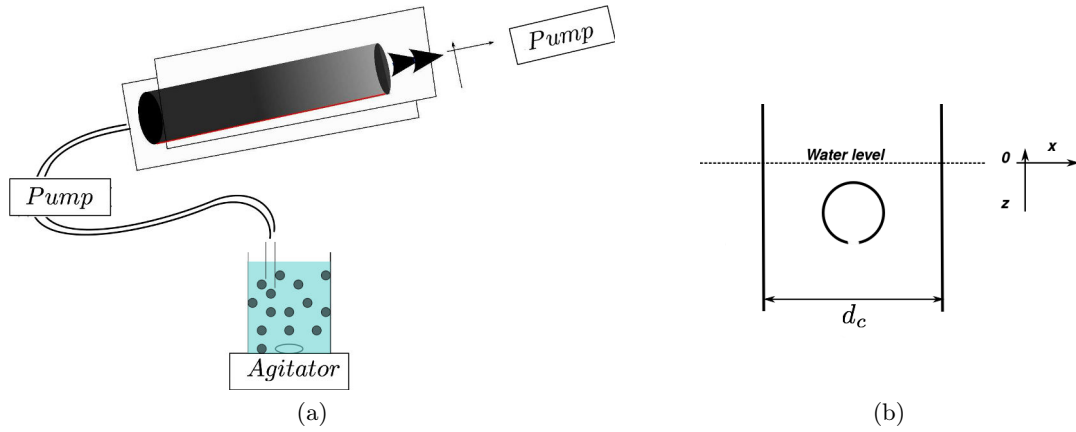
Figure 5.2: Diagram of the particle injector. Figure (a) shows how the particles are mixed prior to the injection, (b) shows a front view of the copper tube immersed in the water and contained between two PVC plates.
