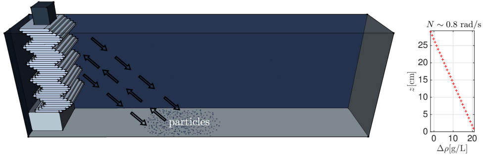
Figure 3.8: Schematics of the experimental setup used to study particle transport by internal gravity waves. The internal waves are generated at the side of the tank thanks to a wave generator. The particles are deposited at the bottom boundary in the region where the internal waves will pass through. On the right is plotted an experimental measurement of the density (crosses) as a function of the water depth.
