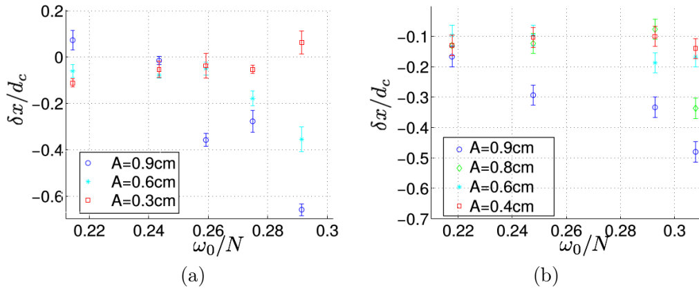
Figure 5.18: Displacement of the column \delta x/d_c as a function of \omega_0/N , where d_c is the size of the column. (a) The wave beam propagates downward. (b) The wave beam propagates upward. For this experiment N = 0.85 \text{ rad}\cdot\text{s}^{-1} .
