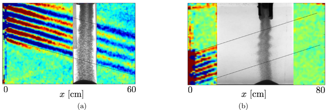
Figure 5.11: View of the wavefield and column of sedimentation particles for two configurations of the wave beam. (a) The wave beam is generated in the upper-left corner and propagates downwards. (b) The wave beam is generated in the lower-left corner and propagates upwards.
