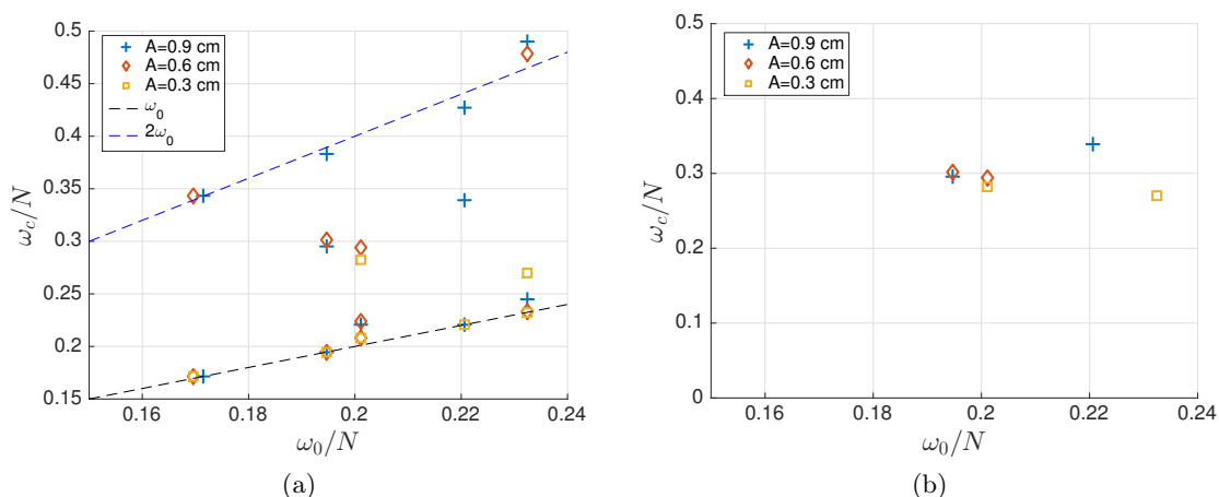
Figure 5.13: Main frequencies present in the spectral content of the column oscillation as a function of \omega/N , where N = 0.85 \text{ rad}\cdot\text{s}^{-1} . The experiment is repeated for different amplitudes of the generator, that is, A = 0.3 \text{ cm} , A = 0.6 \text{ cm} and A = 0.9 \text{ cm} . (a) Shows all the main frequencies found in the spectrum. (b) shows only the frequencies that are not present in the wave spectrum.
