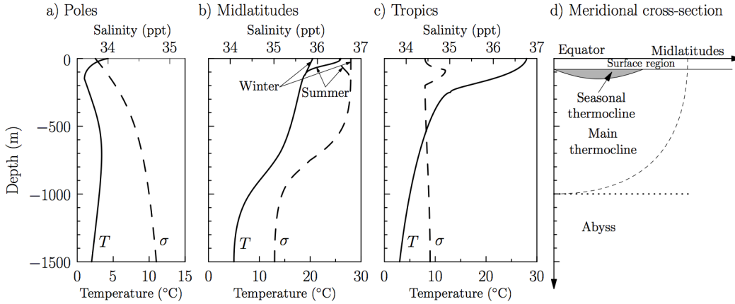
Figure 1.6: Schematic representation of the stratification profile for temperature T (solid line) and salinity \sigma (dashed line) of the ocean for decreasing latitudes (a), (b) and (c) respectively. The main layers as a function of latitude are indicated in (d). Extracted from [67]
