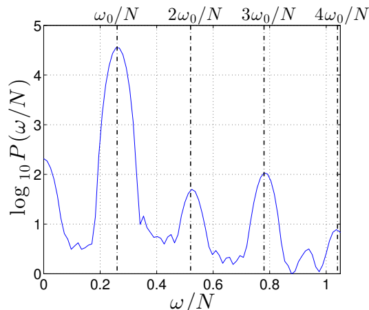
Figure 4.4: Power spectrum density P(\omega/N) of u_s for a critical reflection of the experiment corresponding to figure 4.3. The spectrum is taken from a set of points located in the left side of the field of view at approximately 8 cm from the slope (indicated with a white square in figure 4.3). This experiment corresponds to the case "exp3" indicated in table 4.1, in which \omega_0/N = 0.26 .
