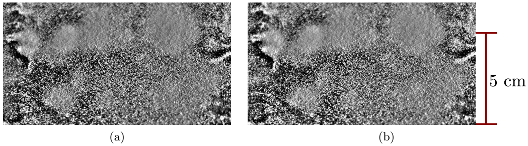
Figure 3.20: Image taken from above of a bed of particles located in an oblique slope, before internal waves are generated (a), and for t/T = 400 (b). No movements of grains is observed between these two moments.
