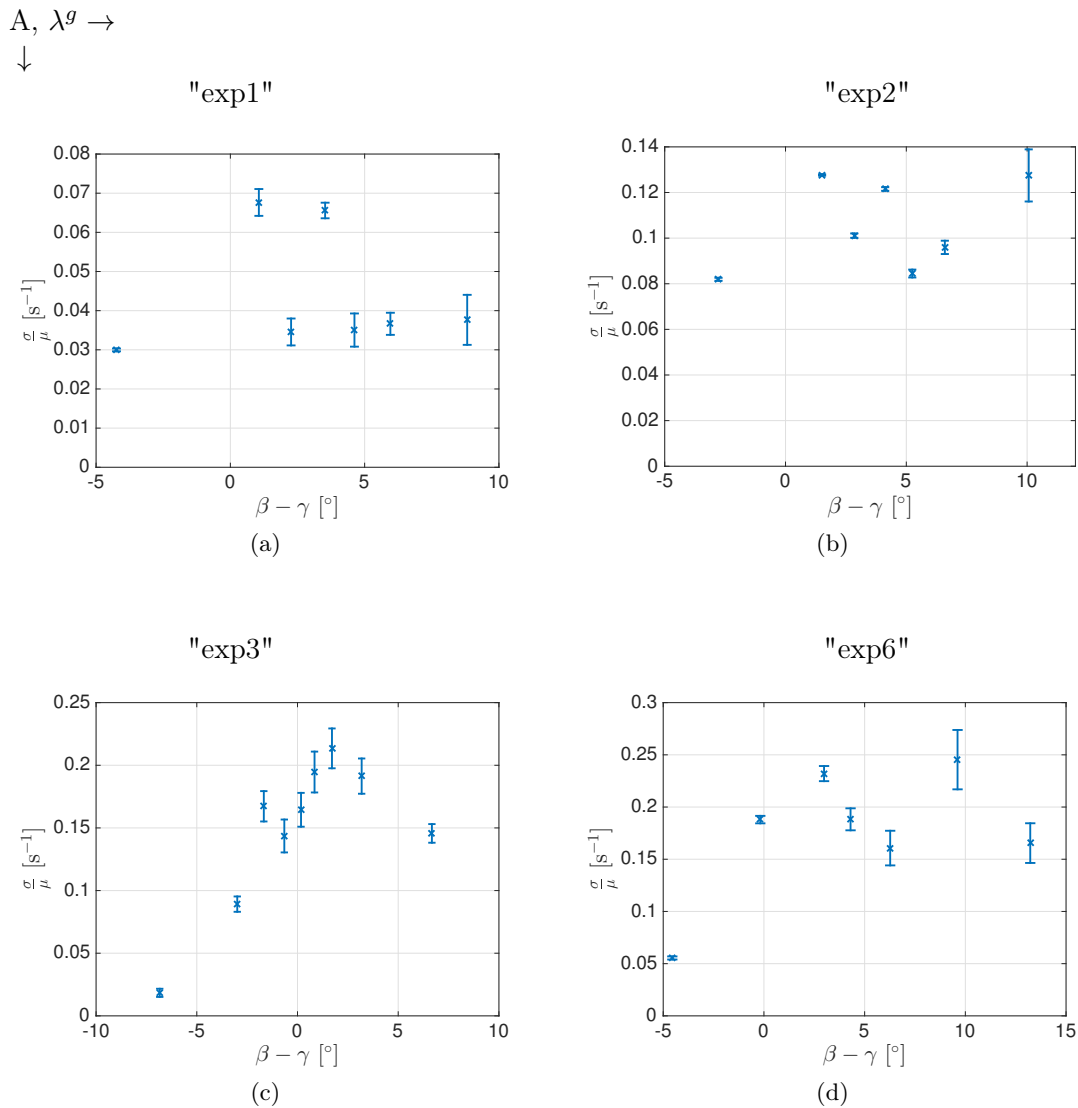
Figure 4.19: \sigma/\mu as a function of \beta - \gamma for experiments "exp1" (a), "exp2" (b), "exp3" (c) and "exp6" (d).
