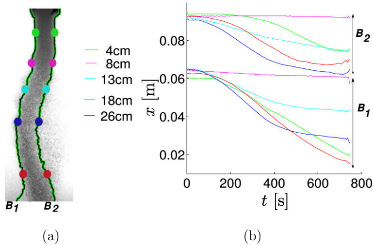
Figure 5.19: Evolution of the horizontal position of the boundaries for several vertical locations. (a) Shows the positions in the boundaries where the horizontal displacement is measured. (b) Evolution of the horizontal displacement of the boundaries for several vertical locations indicated in (a).
