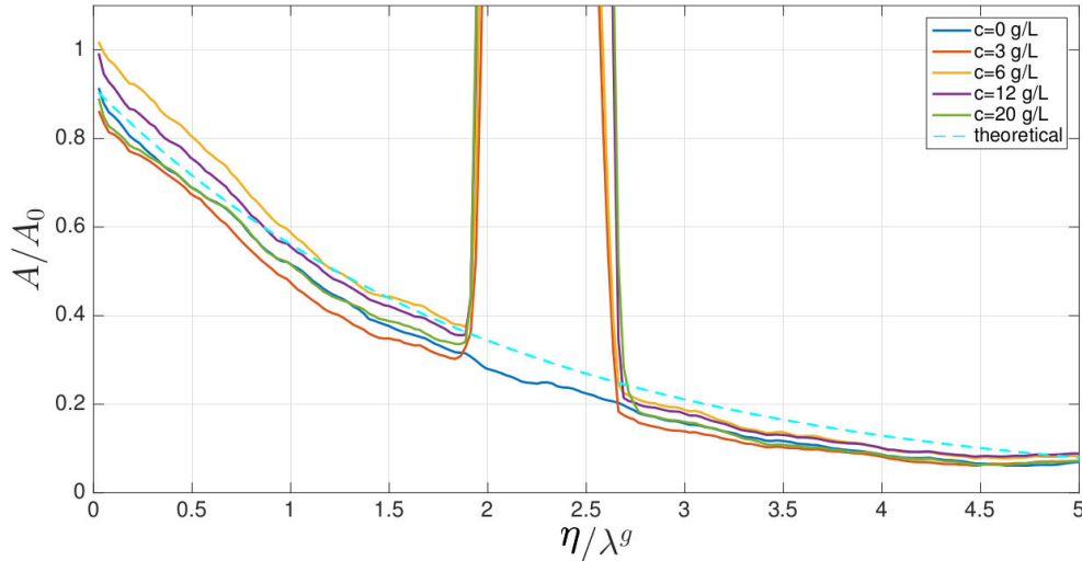
Figure 5.8: Normalized amplitude of the internal waves as a function of the position in the segment OP (indicated with a white dashed line in figure 5.6) for several concentrations c . In addition, the theoretical decay of the amplitude of the wave because of the viscosity is plotted.
