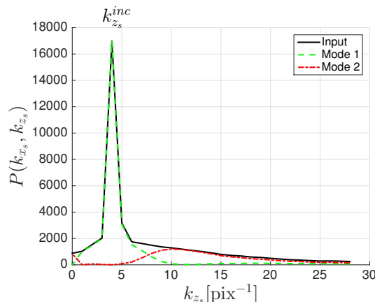
Figure 4.8: Profile along the k_{z_s} coordinate for k_{x_s} = k_{x_s}^{inc} of the three spatial spectrum plotted in figure 4.7.
