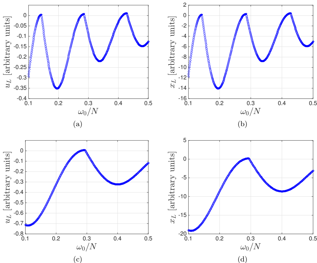
Figure 5.24: Horizontal velocity ((a) and (c)) and horizontal position ((b) and (d)) drift as a function of \omega_0/N . Figures (a) and (b) correspond to the experiment with buoyancy frequency N = 1.1 \text{ rad}\cdot\text{s}^{-1} . Figures (c) and (d) correspond to the experiment with buoyancy frequency N = 0.85 \text{ rad}\cdot\text{s}^{-1} .
