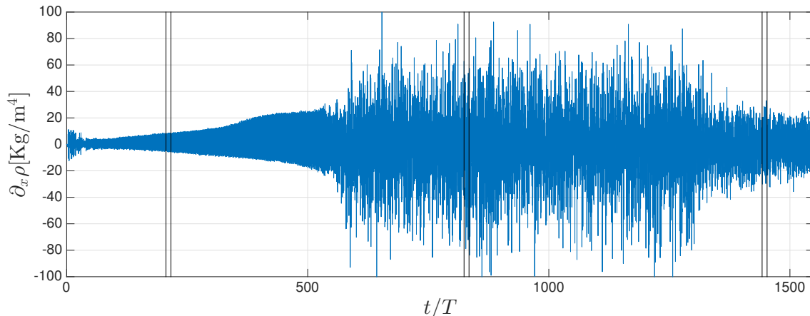
Figure 3.14: Time evolution of \partial_x \rho as a function of t/T . Three pair of vertical lines indicate time intervals that will be detailed in figure 3.15.
