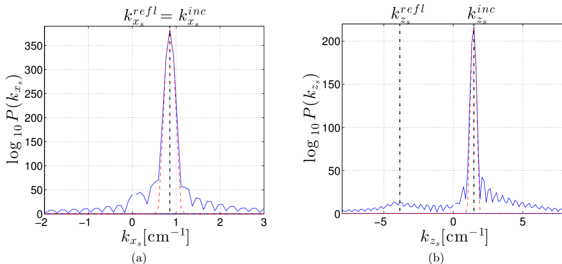
Figure 4.5: (a) Spatial spectrum (solid curve) for k_{x_s} . (b) Spatial spectrum (solid curve) for k_{z_s} ; the dashed line represents the spectrum filtered around the forced wavenumber \mathbf{k}^{inc} . With a dashed-dotted vertical line is indicated the experimental value of \mathbf{k}^{inc} and \mathbf{k}^{refl} . These spectra correspond to experiment "exp3" and \omega_0/N = 0.26 .
