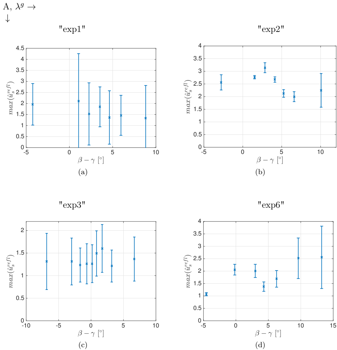
Figure 4.16: \max(\hat{u}_s^{refl}) as a function of \beta - \gamma for experiments (ordered by increasing Re number): (a) "exp1", (b) "exp2", (c) "exp3" and (d) "exp6". The experiments present different sets of parameters A and \lambda^g , and at the top left is indicated in which direction these two parameters increase.
