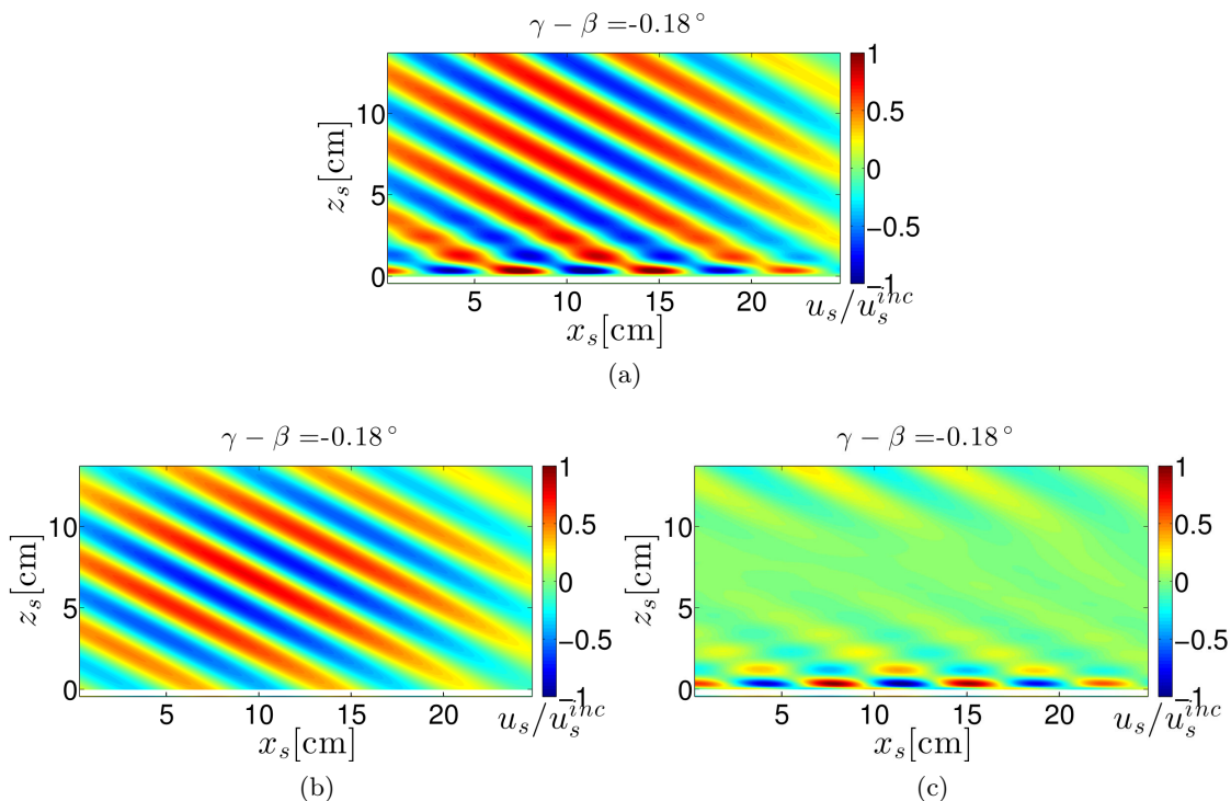
Figure 4.6: Snapshot of u_s/u_s^{inc} resulting from a filtering through Hilbert transform around: \omega_0 and k_{x_s}^{inc} (a); and around \omega_0 , k_{x_s}^{inc} and k_{z_s}^{inc} (b). (c) Result of the subtraction between velocity field u_s of (a) and (b). Note that the slope boundary is located at z_s = 0 .
