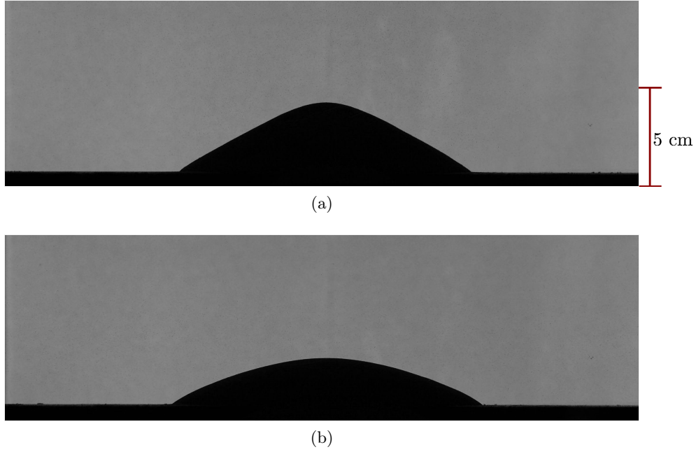
Figure 3.10: Front view of the mountain of particles for t/T = 0 (a), and for t/T = 4000 (b).
