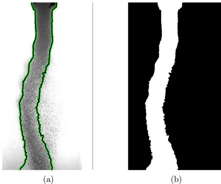
Figure 5.15: Example of the boundary detection algorithm for the column of sedimentation particles. (a) With a green line is indicated the localization of the boundaries. (b) Outcome of 2D matrix indicating where the column is located.
