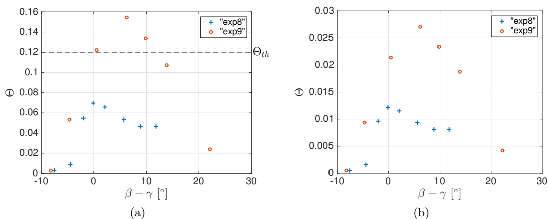
Figure 4.22: Shields dimensionless number \Theta as a function of \beta - \gamma for experiments "exp8" and "exp9". The Shields number is estimated for hollow glass particles (a), and for Polystyrene particles (b)
