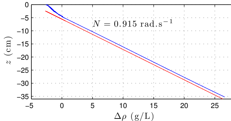
Figure 2.2: Depth as a function of \Delta\rho = \rho - 1000 \text{ g}\cdot\text{L}^{-1} . Density profile measured with a conductivity probe in blue and, in red the linear fit displaced 1 cm below. The buoyancy frequency N is computed from the linear fit.
