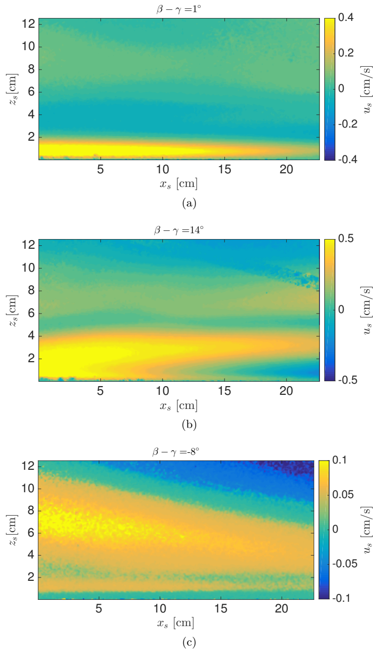
Figure 4.21: Snapshot of the velocity field u_s for a internal wave reflection generated with a vertical mode corresponding to experiment "exp9". Different frequencies (propagation angle \beta ) have been explored, \beta - \gamma = 1^\circ (a), \beta - \gamma = 14^\circ (b) and \beta - \gamma = -8^\circ (c).
