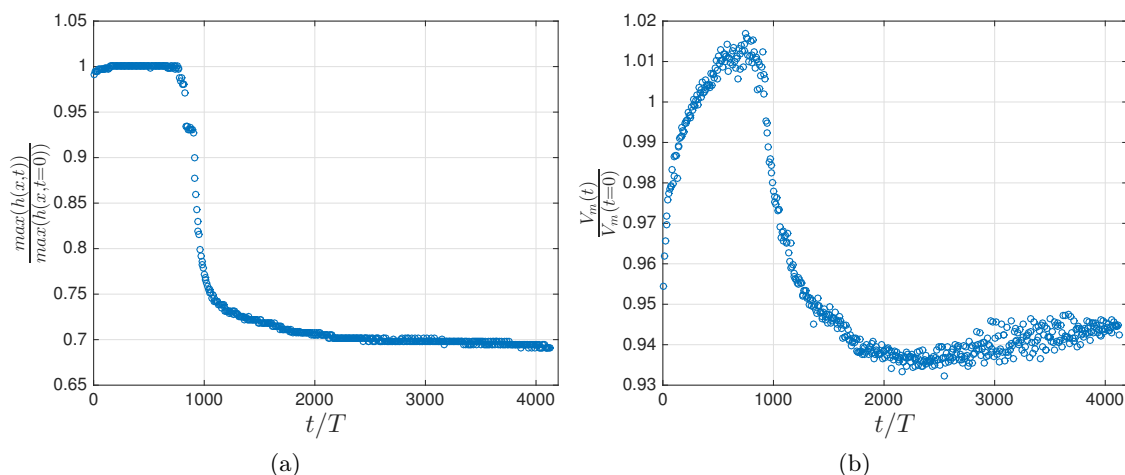
Figure 3.12: Evolution in time of: (a) the normalized maximum height of the contour, and (b) the normalized volume of the mountain.
