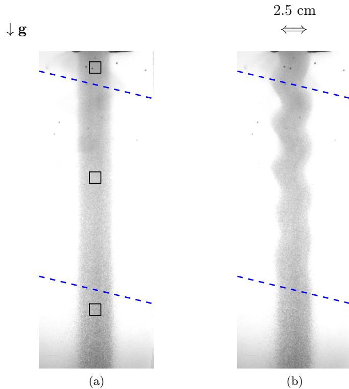
Figure 5.9: Front view of the column of sedimentation particles. (a) Snapshot at t/T = 0 , where no wave perturbations are present. (b) Snapshot of the column during the pass of internal plane waves through the column, after 100 periods. The wave beam is located between the two blue dashed lines. Three squares in (a) indicate the regions where the intensity evolution is measured.
