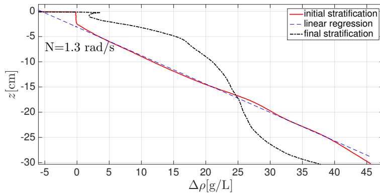
Figure 3.16: Measurements of the density profile, where \Delta\rho = \rho - 1000 g/L, for the initial state before internal waves are generated, and for t/T = 4000 . The linear approximation of the initial density profile is plotted with dashed line.
