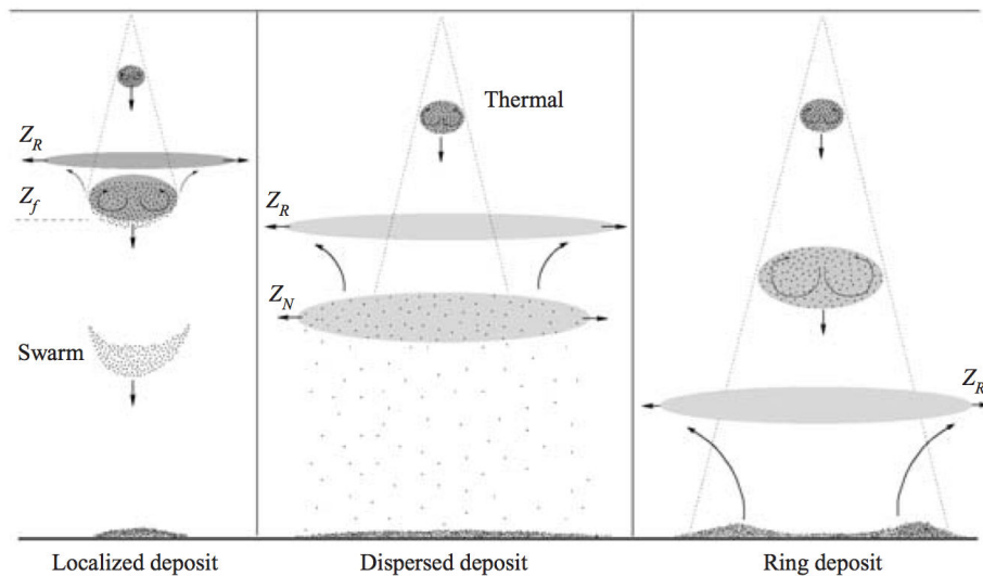
Figure 3.7: Particle cloud sedimentation. Three different scenarios are present, when the deposit is localized, disperse and in ring shape. Extract from Bush et al. [10]
