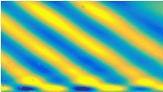
Wavefield of a focalization produced by an internal wave near-critical reflection over a sloped boundary.
