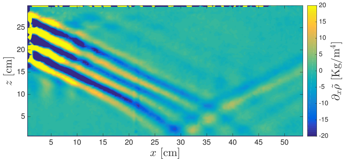
Figure 3.17: Snapshot of the wavefield of a plane wave propagating from left to right and reflecting on the bottom.
