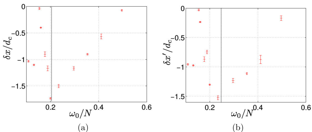
Figure 5.17: (a) Maximal displacement of the column \delta x/d_c as a function of \omega_0/N , where d_c is the size of the column. (b) The displacement of the column is corrected by a factor in consequence of the dependency of the internal wave amplitude with the frequency, that is, \delta x' = \delta x(1 - (\omega_0/N)^2)/\omega_0 . For this experiment A = 0.9 cm and N = 1.1 rad·s -1 .
