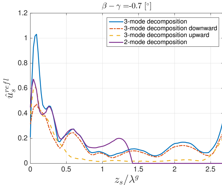
Figure 4.14: \hat{u}_s^{refl} as a function of z_s/\lambda^g estimated by two- and three-mode VMD decomposition, corresponding to experiment "exp4" and \beta - \gamma = -0.7^\circ . The upward and downward components of the three-mode VMD decomposition are also indicated.
