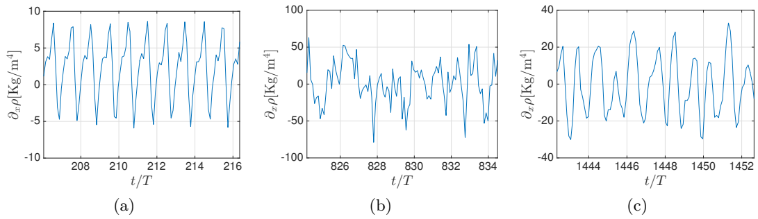
Figure 3.15: Time evolution of \partial_x \rho for three time intervals detailed with pairs of vertical lines in figure 3.14, (a) corresponds to the pair of lines on the left, (b) at the center and (c) on the right. Note the change in vertical scales between the three graphs.
