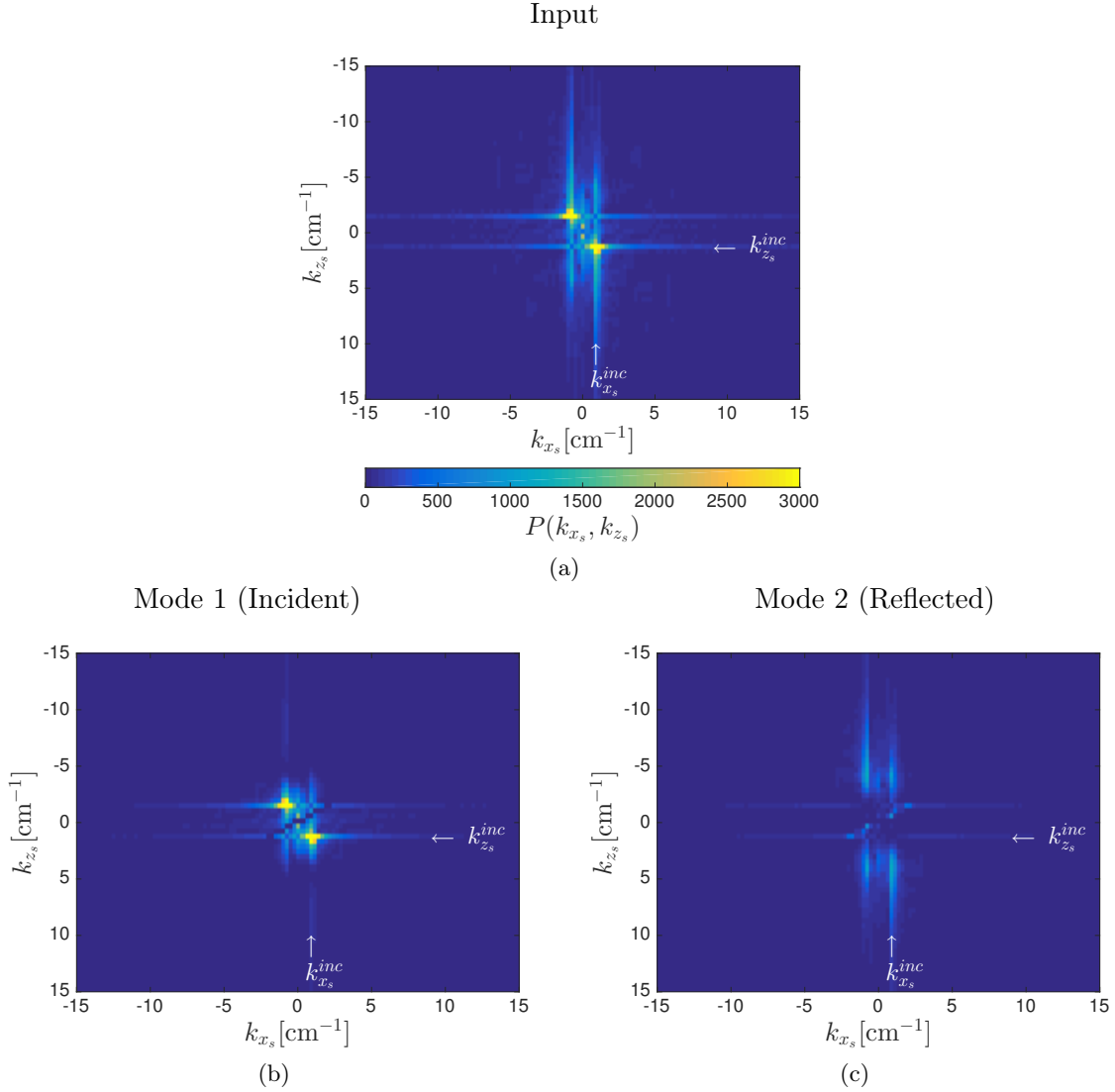
Figure 4.7: 2D spatial power spectrum P(k_{x_s}, k_{z_s}) of the velocity field corresponding to the experiment presented in figure 4.3. (a) Spectrum of a velocity field of incident and reflected wave together. (b) and (c) are Mode 1 and 2 obtained through 2D-VMD separation method associated to the velocity field of the incident and reflected wave respectively. k_{x_s}^{inc} and k_{z_s}^{inc} are indicated in the lower and right margin of each figure.
