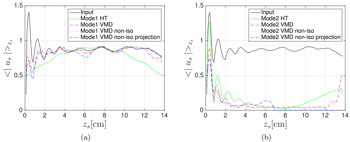
Figure 4.10: \langle |u_s(z_s)| \rangle_{x_s} for different spatial separation methods. (a) velocity field related to the incident wave (Mode 1). (b) velocity field related to the reflected wave (Mode 2). In both figures is plotted the profile of the Input. z_s = 0 represents the position of the slope.
