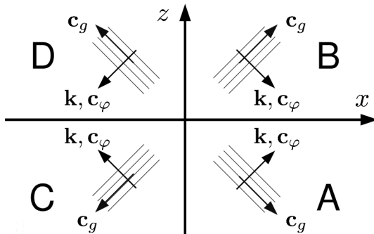
Figure 2.7: Illustration representing four possible waves generated from one pair of values (\omega, |\mathbf{k}|) , A, B, C and D.
