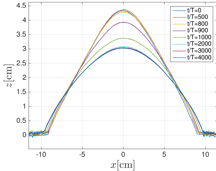
Figure 3.11: Height of the mountain h(x, t) for different instants.
