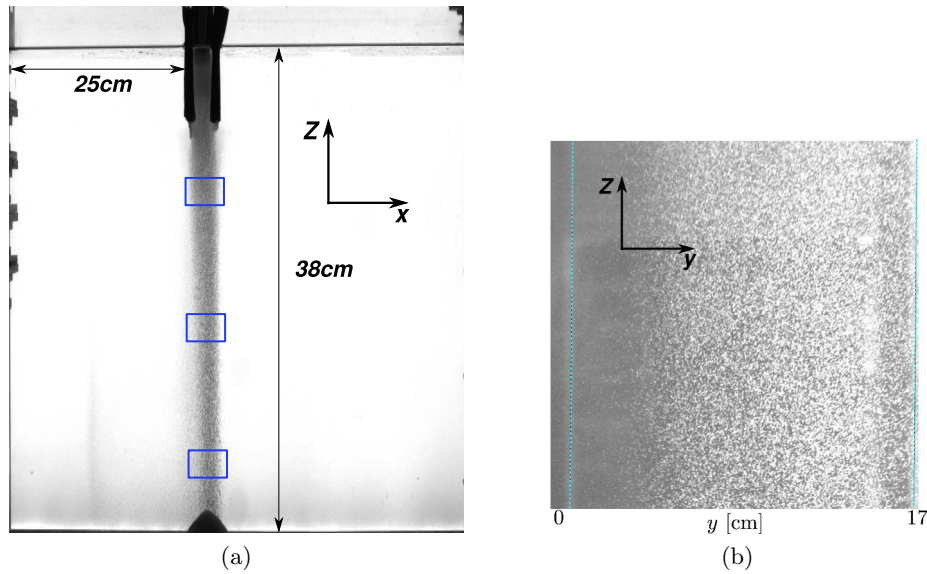
Figure 5.3: View of the column of particles in suspension in the stratified fluid. (a) Front view of the column. (b) Side view of the column. The fluid dragging the particles is injected at constant flow rate ( Q = 20 \text{ cm}^3 \text{ min}^{-1} ). The three blue squares in (a) illustrate where the variations of concentration will be measured.
