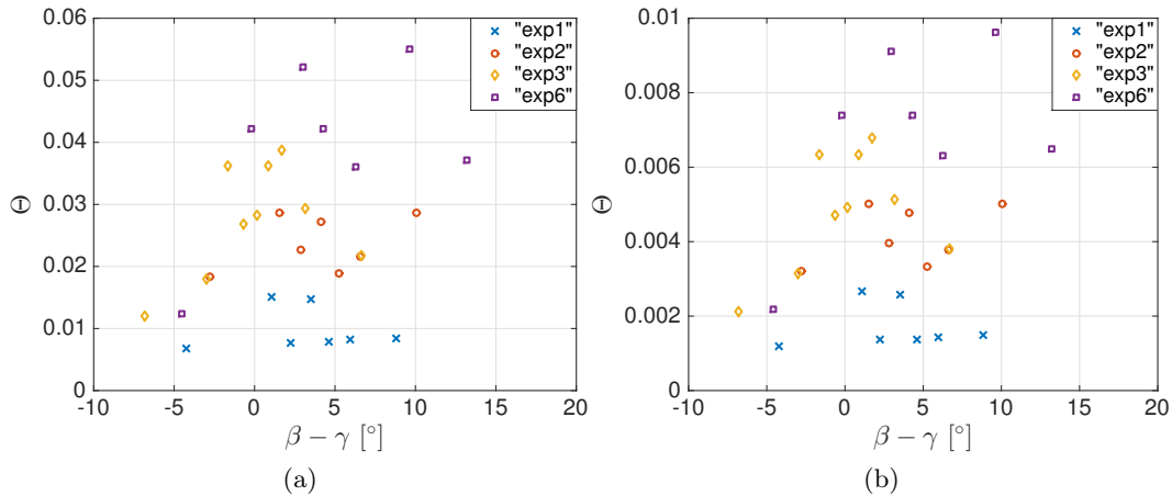
Figure 4.20: Shields dimensionless number as a function of \beta - \gamma for experiments "exp1", "exp2", "exp3" and "exp6". The Shields number is estimated for hollow glass particles (a), and for Polystyrene particles (b).
