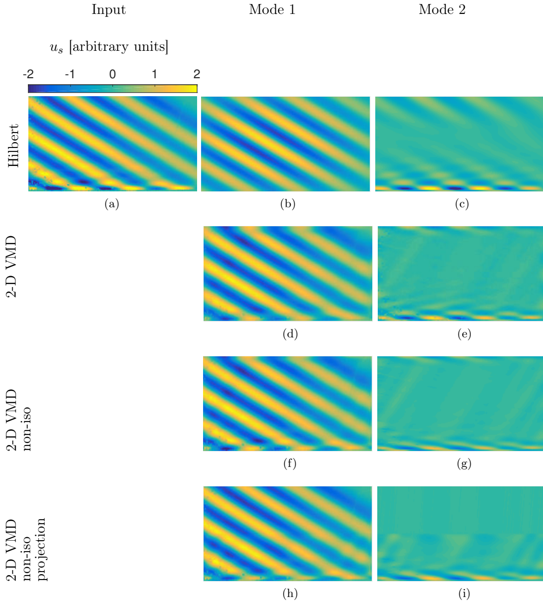
Figure 4.9: 2D images of the field of view for the experiment presented in figure 4.3. Abscissa and ordinate correspond respectively to the x_s and the z_s coordinates. Color scale indicates a scale proportional to u_s . (a) Velocity field filtered temporally at \omega_0/N = 0.26 that will be used as the input of the spatial separation methods. Figures (b), (d), (f) and (h) represent the Mode 1 (incident wave) obtained through respectively the Hilbert transform, VMD, VMD non-iso and VMD non-iso projection methods; whereas figures (c), (e), (g) and (i) represent the corresponding field for Mode 2 (reflected wave).
