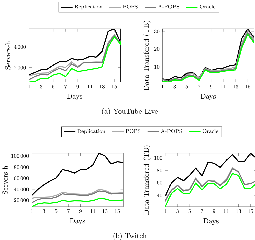
Figure 4.10: Approaches behavior upon time.
