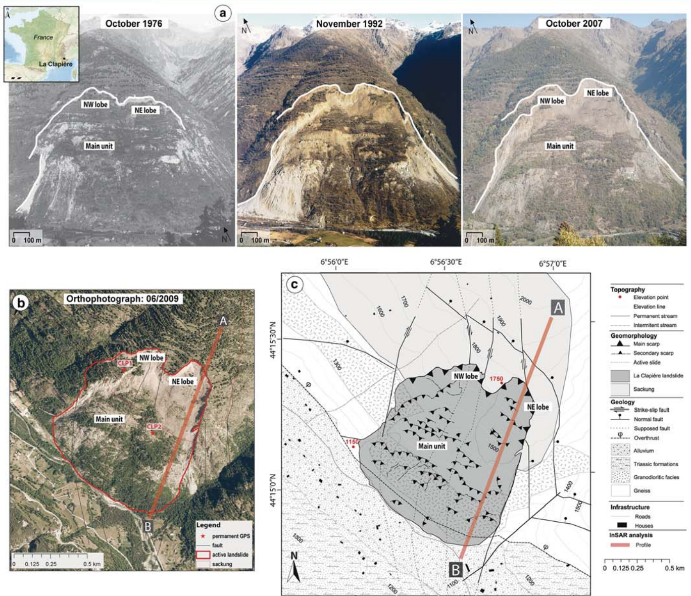
Fig. 1 Geomorphology of the La Clapière landslide. a Photographs of the La Clapière landslide in 1976, 1992 and 2007. b Orthophotograph of the landslide in 2009. c Morpho-structural map of the landslide.
