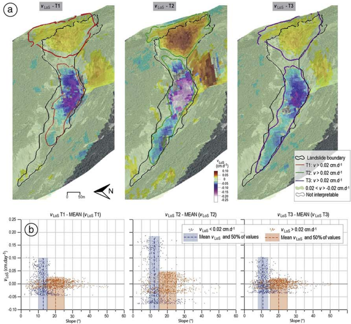
Fig. 13. InSAR displacement rates of the Poche landslide for three periods in 2007 and 2009. (a) Maps of v_{LoS} values ( cm \cdot d^{-1} ) at T1, T2 and T3. (b) Plots of v_{LoS} values as a function of slope angle ( ^{\circ} ). The velocity estimated at one pixel location is represented in relation to the average velocity observed in the subsidence zone ( v_{LoS} > 0.02 \text{ cm} \cdot d^{-1} , in orange) and in the transit zone ( v_{LoS} < 0.02 \text{ cm} \cdot d^{-1} , in blue).
