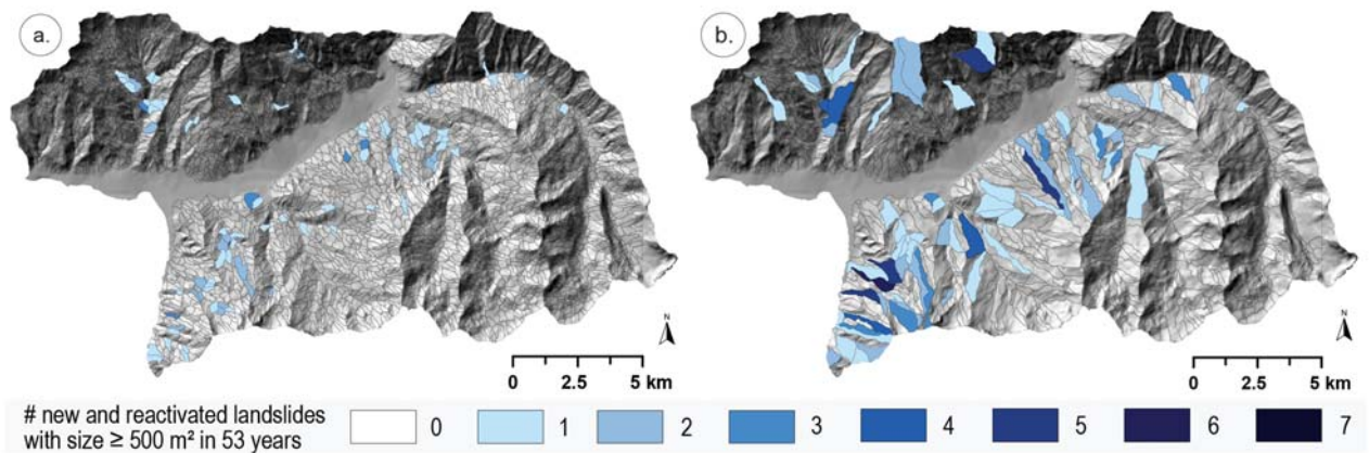
Figure 4-14: Number of new and reactivated landslides with a size evolution greater than 500 \text{ m}^2 over the time considered (i.e. 53 years). Calculation realised on mapping units affected by at least one new landslide or an old one with a size enlargement.
