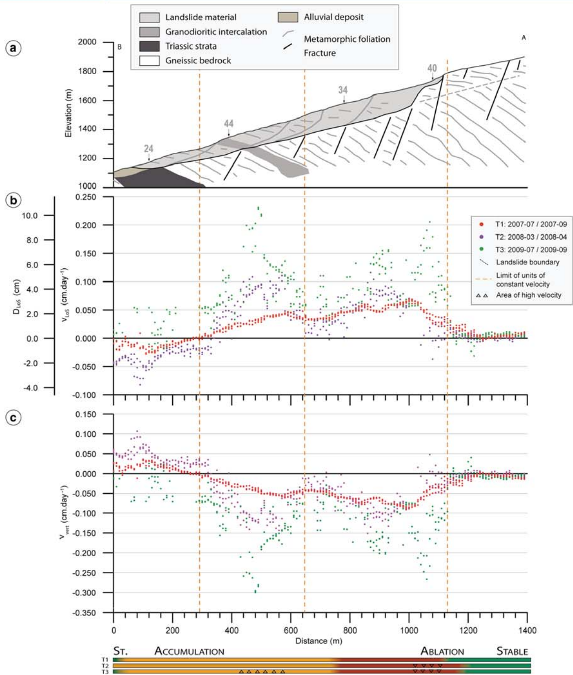
Fig. 10 Displacement (DLoS, DVert; cm), velocity (VLoS; cm day -1 ) observed at the La Clapière landslide from L-band ALOS/PALSAR SAR data. a Topography, lithology and geometry of the slip surfaces along a longitudinal cross section in the Eastern part of the landslide (A–B). The location of the 30-m-width profile is indicated in Fig. 9, and the landslide geometry is from Cappa et al. (2004). The displacement pattern is indicated by the theoretical vectors for each unit. b LOS displacements (DLoS) and velocity along profile A–B for the unwrapped interferograms T1, T2 and T3. c Vertical velocity (Vvert) along profile A–B for the unwrapped interferograms T1, T2 and T3. The colour bars indicate changes in the movement type (subsidence in red, accumulation in orange, stable slopes in green)
