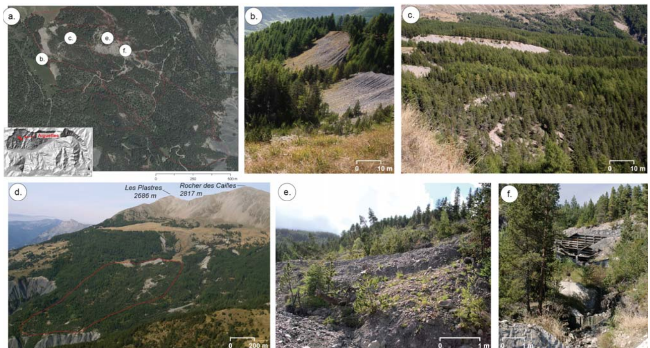
Figure 2-12: Morphology of Aiguettes landslide in the Riou-Bourdoux catchment. (a) Orthophotograph of 2009 locating the different slides and some features. (b) View to the southeast of the main scarp. (c) Ablation area of the
