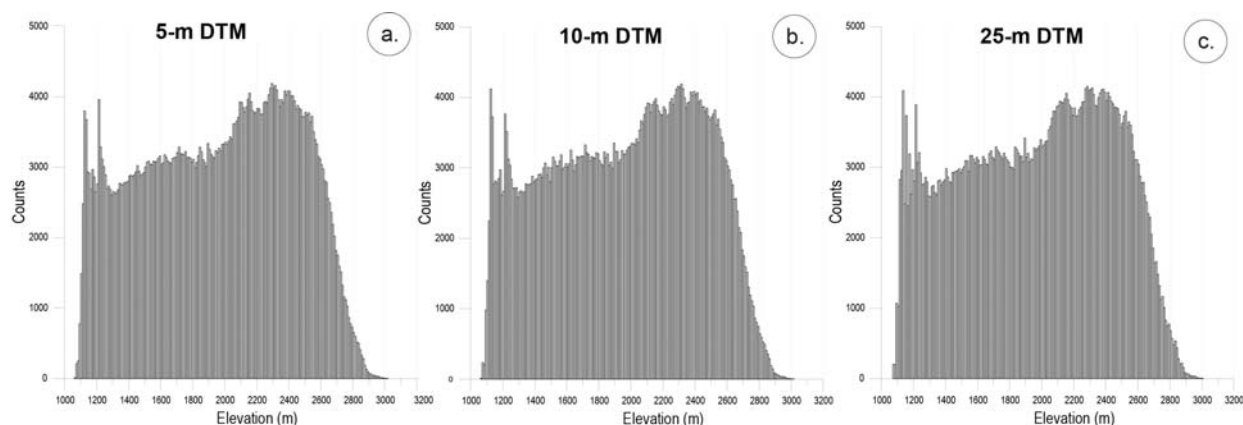
Figure 4-1: Histograms of elevation per elevation class for the DTMs at 5-m (a), 10-m (b) and 25-m (c) resolution
