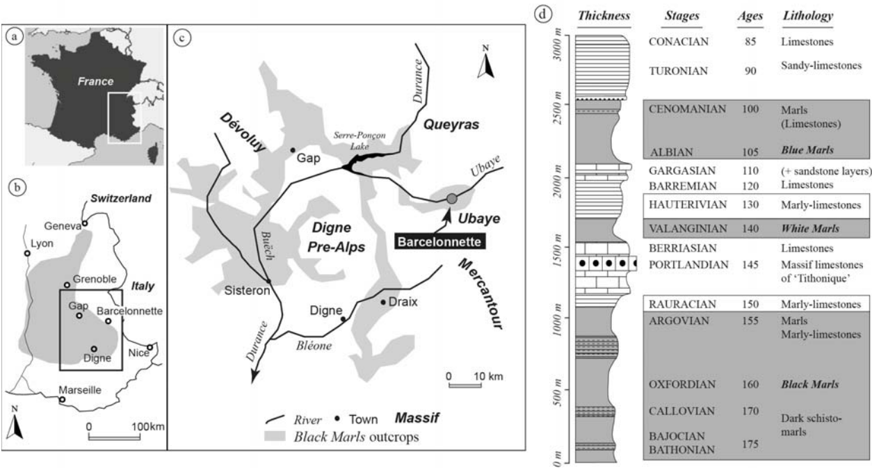
Figure 2-1: Location of the Ubaye Valley and extension of black marls facies in the South-East French Alps (a-c). Different types of black marls are represented in grey (b-c). Stratigraphy of the Dauphinois zone is shown in (d) (modified from Malet, 2003; Remaître, 2006).
