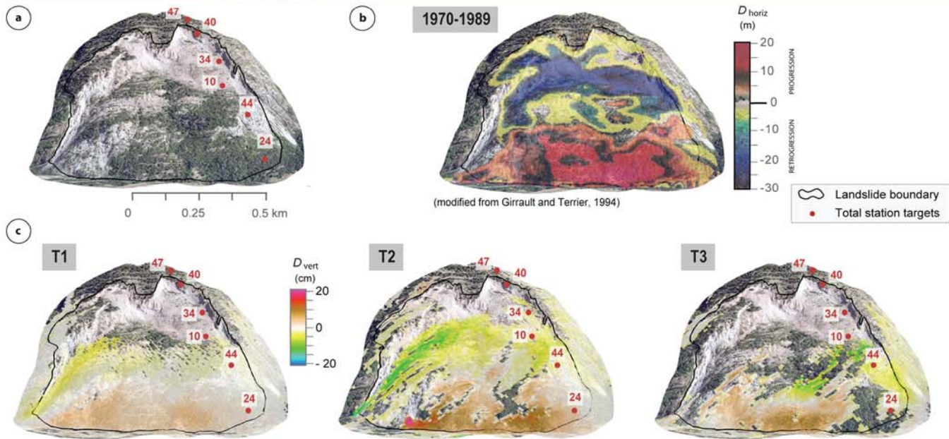
Fig. 11 Horizontal and vertical displacement fields of the La Clapière landslide. a Orthophotograph of the landslide in 2009. b Mean horizontal displacement field (dH) measured by comparison of digital surface models (DSM) between 1970 and 1989 (modified from Girault and Terrier 1994). c Vertical displacement field (dV) measured by InSAR at T1, T2 and T3. The landslide boundary is indicated in black and the targets by red dots
