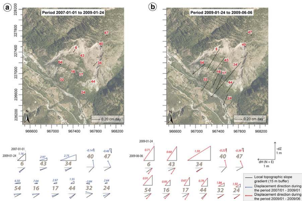
Fig. 7 Analysis of the geometry of the 3D displacement vectors for a period of low velocity ( < 0.2 \text{ cm day}^{-1} ; < 2009/01/24 ) and a period of high velocity ( > 0.2 \text{ cm day}^{-1} ; > 2009/01/24 ). a Map of 3D vectors for several targets for a period of low velocity. The ratio of vertical to horizontal displacement is indicated in blue for the period from 2007/01/01 to 2009/01/24. b Map of 3D vectors for several targets for a period of high velocity. The ratio of vertical to horizontal displacement is indicated in red for the period from 2009/01/24 to 2009/06/06. The horizontal displacement corresponds to the sum of the North (N) and East (E) components. The directions of displacement are compared to the local slope gradient
