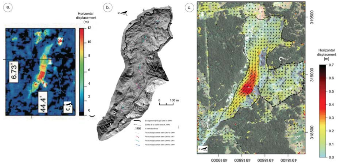
Figure 2-18: Displacement field of the Poche landslide. (a) Horizontal displacement for the period 09/19/2003–08/22/2004 derived from the correlation of SPOT5 images (Delacourt et al., 2007). (b) Horizontal displacement vector measured by comparing orthophotographs in 2000, 2004, 2007 and 2009 (Mazeau, 2013). (c) Horizontal displacement for the period 07/08/2012–05/10/2012 from terrestrial photogrammetry (Stumpf et al., 2014).
