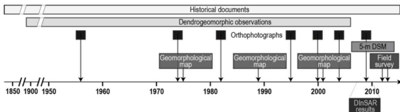
Figure 3-2: Timeline of the available observations.
