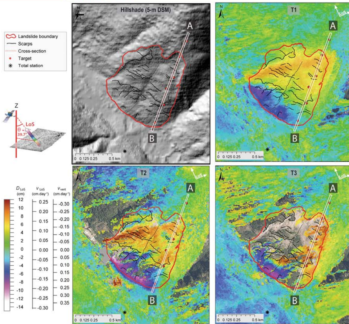
Fig. 9 Displacement (cm) and velocity (cm day -1 ) fields observed for the La Clapière landslide. The hillshade of a 5 m resolution digital surface model (year 2009) and the unwrapped interferograms for the periods T1, T2 and T3 are presented
