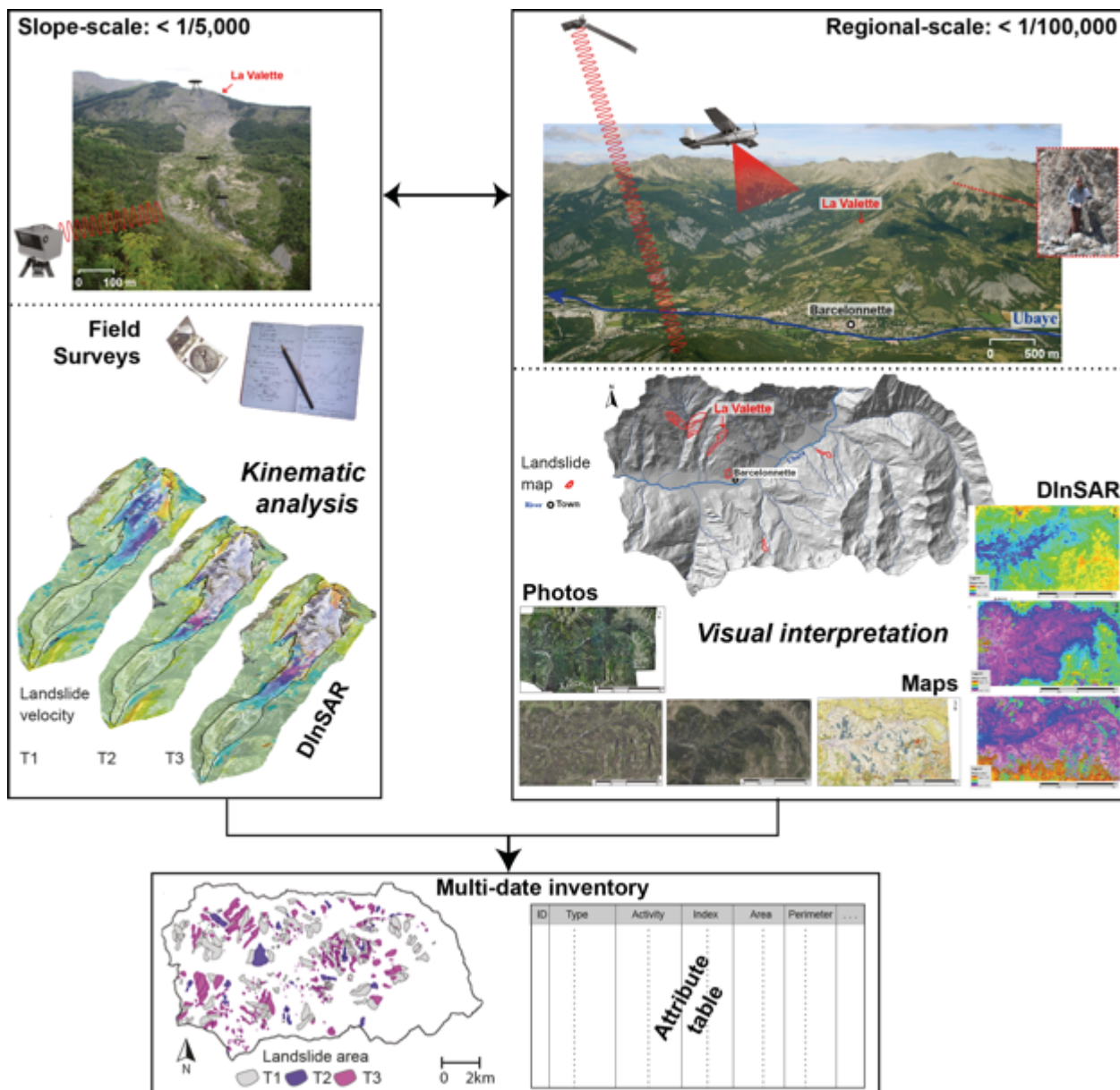
Figure 3-1: Combination of two analysis scales (slope, regional) for the creation of a multi-date landslide inventory.
