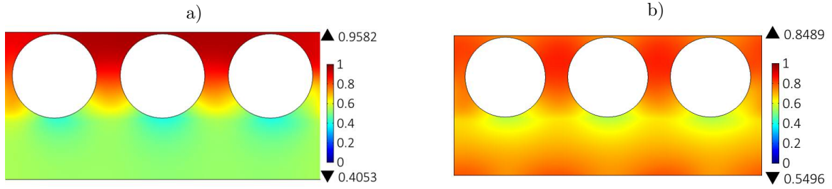
Figure 12: Pollutant concentration for c_0 = 1.43 \text{ mol.m}^{-3} after 30 cm along a) the single textile and b) multi-layer reactors
