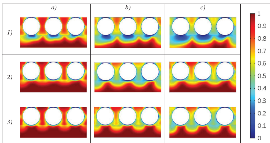
Figure 11: Pollutant concentration field ( c_A/c_0 ) at the RVE outlet. ( k_1 = 5 \times 10^{-3} m^3 \cdot mol^{-1} \cdot s^{-1} ); (a) after 10 cm along the UV textile; (b) after 20 cm along the UV textile; (c) after 30 cm along the UV textile; case 1: K = 1.8 \times 10^{-10} m^2 ; case 2: K = 5 \times 10^{-10} m^2 ; case 3: K = 8 \times 10^{-10} m^2 .
