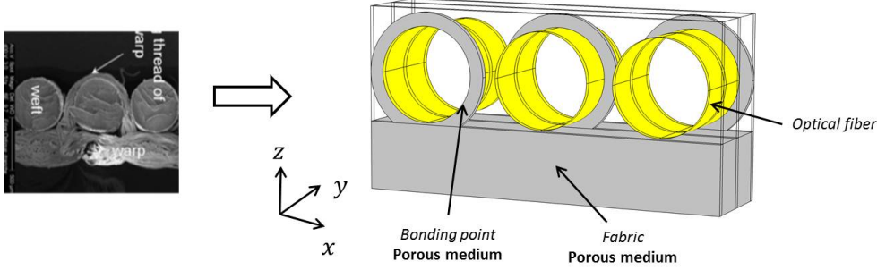
Figure 3: Representative Volume Element of the assembly of fabric and optical fibres
