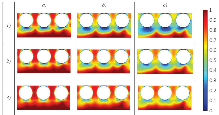
Figure 10: Pollutant concentration field ( c_A/c_0 ) at the RVE outlet. ( k_1 = 5 \times 10^{-3} m^3 \cdot mol^{-1} \cdot s^{-1} , K = 1.8 \times 10^{-10} m^2 ); (a) after 10 cm along the UV textile; (b) after 20 cm along the UV textile; (c) after 30 cm along the UV textile; case 1: U_0 = 1.3 \times 10^{-2} m \cdot s^{-1} ; case 2: U_0 = 2.6 \times 10^{-2} m \cdot s^{-1} ; case 3: U_0 = 3.9 \times 10^{-2} m \cdot s^{-1} .
