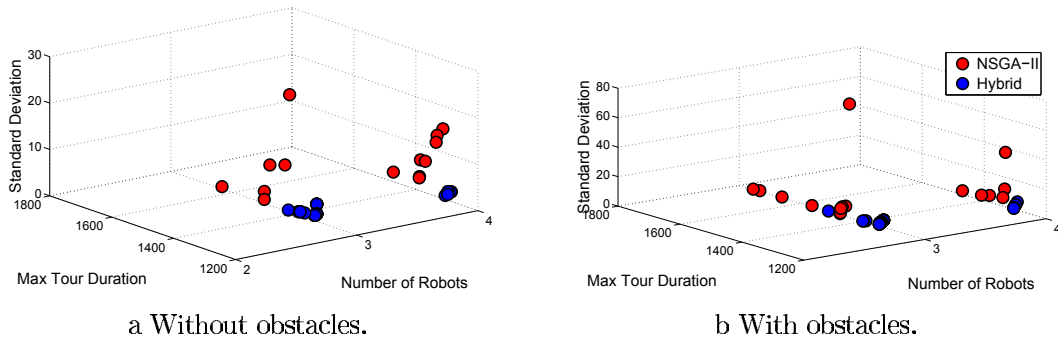
Figure 8.11: Pareto front obtained by 20 PoIs.
