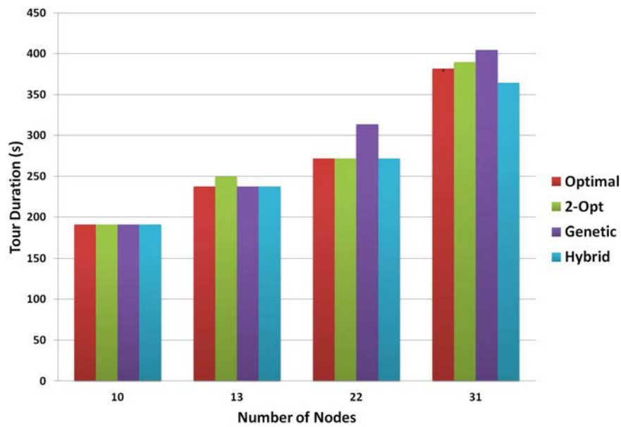
Figure A.3: Final solutions of Optimal, 2-Opt, Genetic and Hybrid for small configurations.
