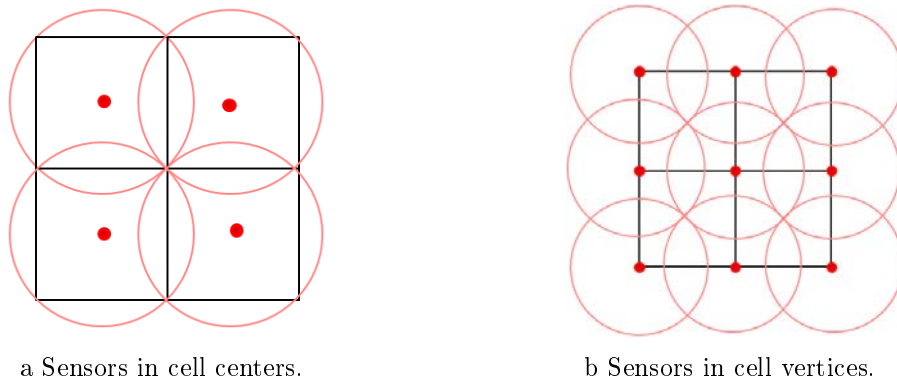
Figure 3.5: Grid Based Strategy.
