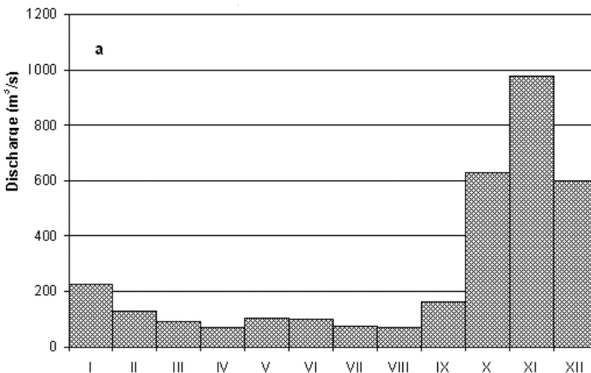
Figure 2.3 Average monthly flow at Nong Son station (Dang, 2009)
