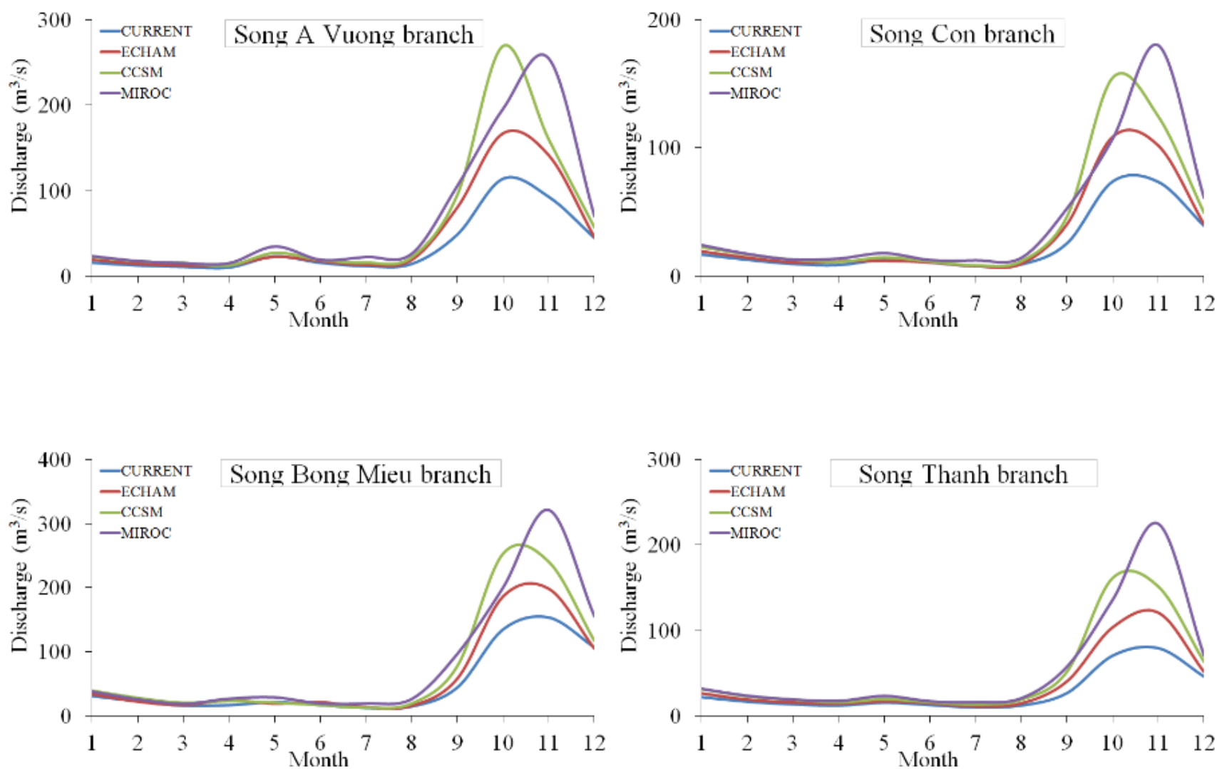
Figure 5.7a. Baseline and future stream flows at Vu Gia Thu Bon catchment.
