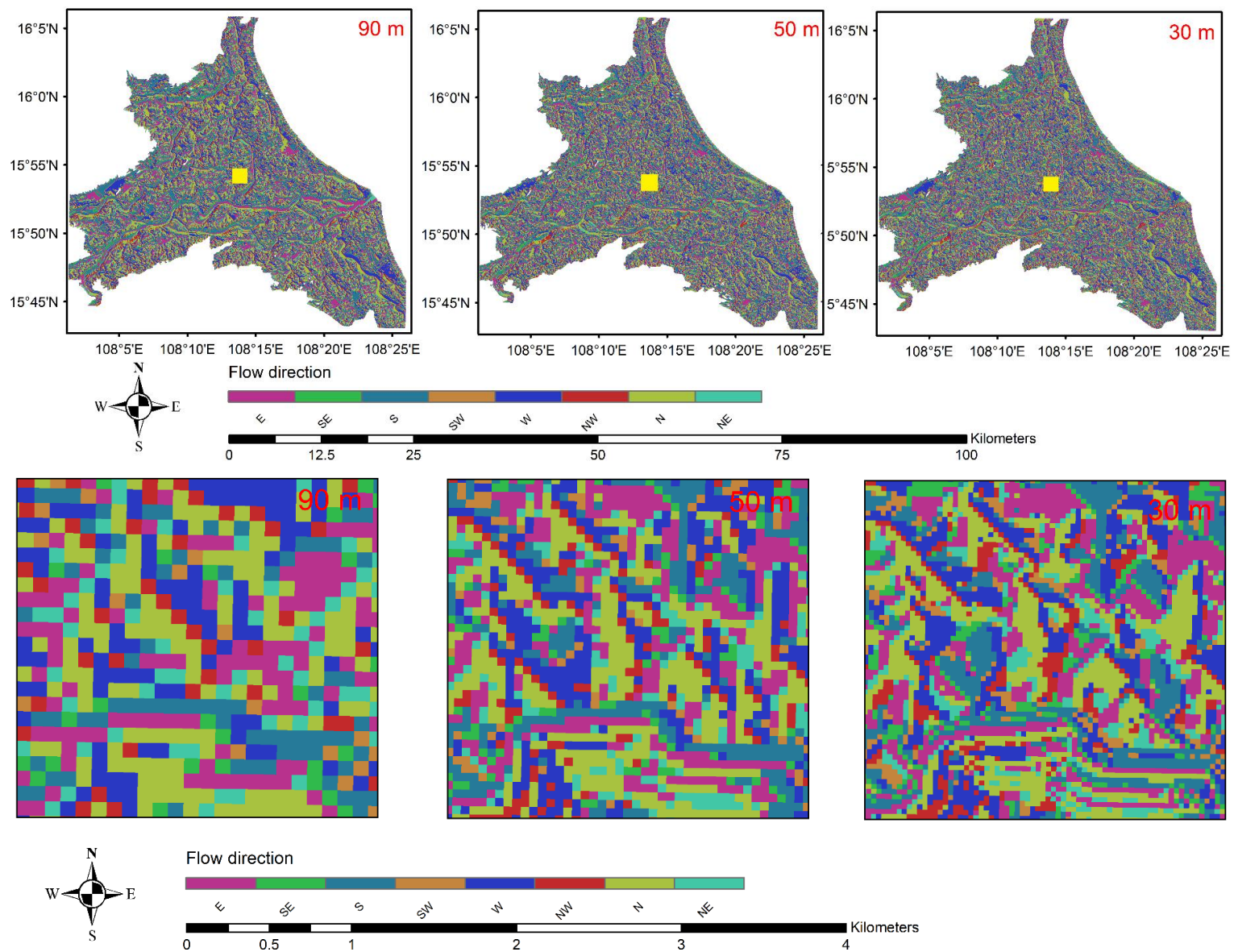
Figure 4.28. Flow direction distributed map against DEM resolution.
