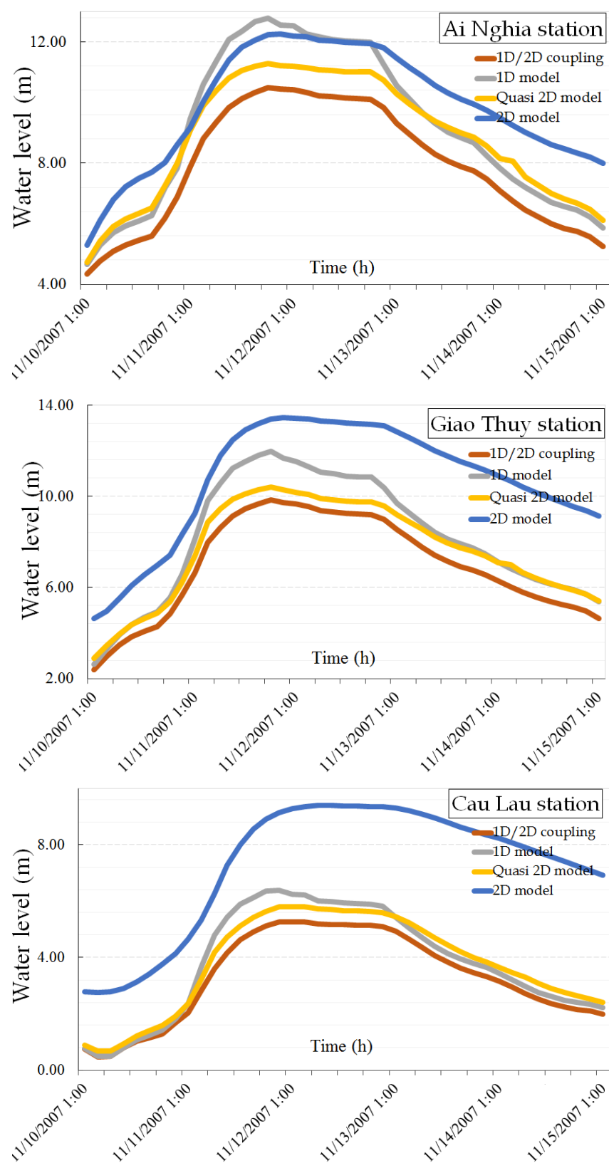
Figure 4.23. Hydrographs of water lever due to model structure.
