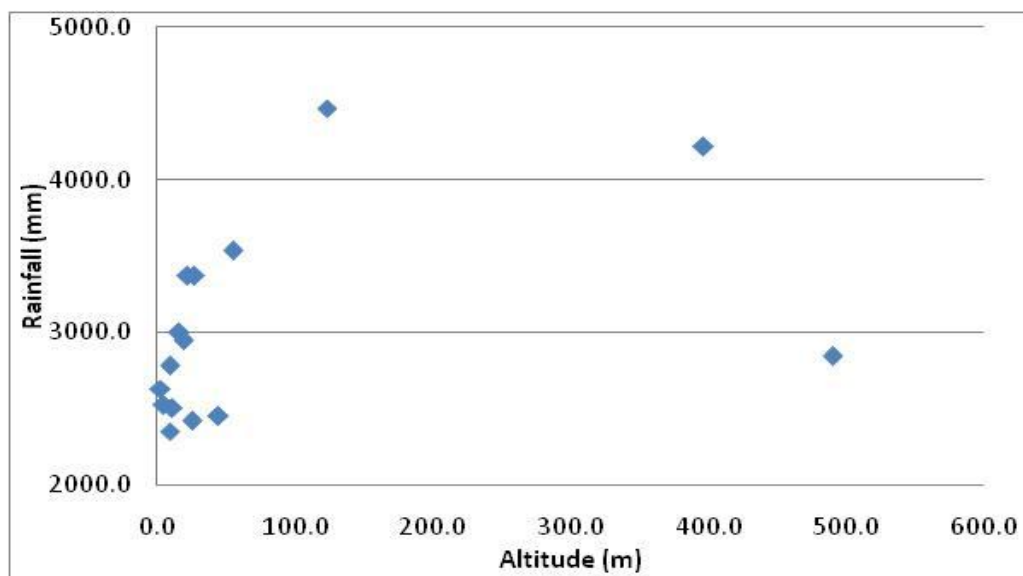
Figure 3.14. Correlation between annual rainfall and altitude at Vu Gia Thu Bon gauging stations.
