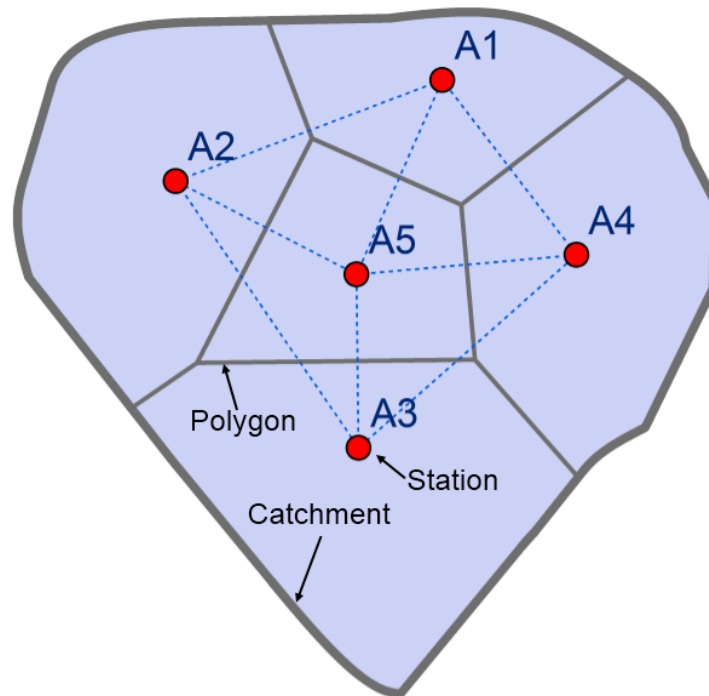
Figure 3.13 Thiessen polygon
