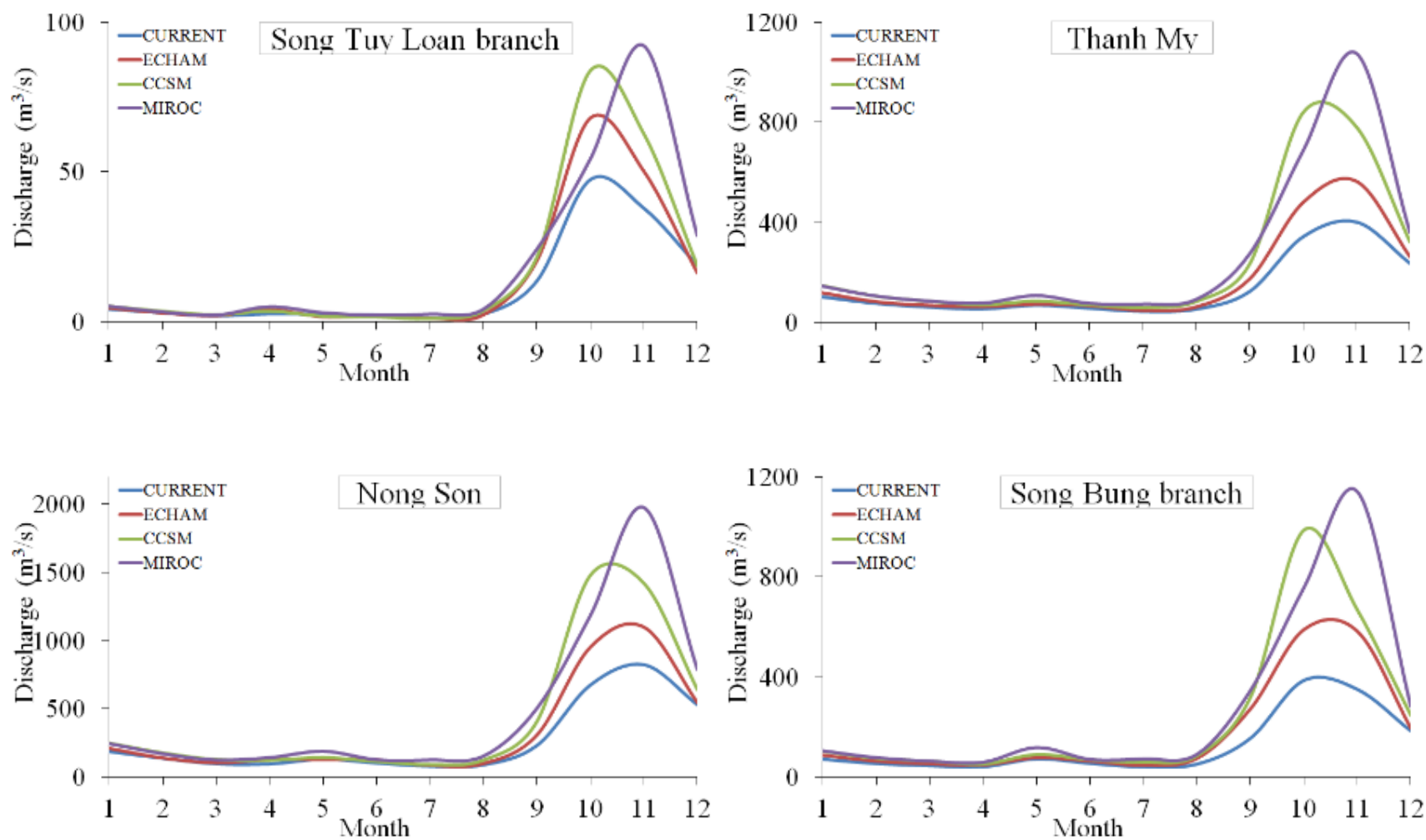
Figure 5.7b. Baseline and future stream flows at Vu Gia Thu Bon catchment.
