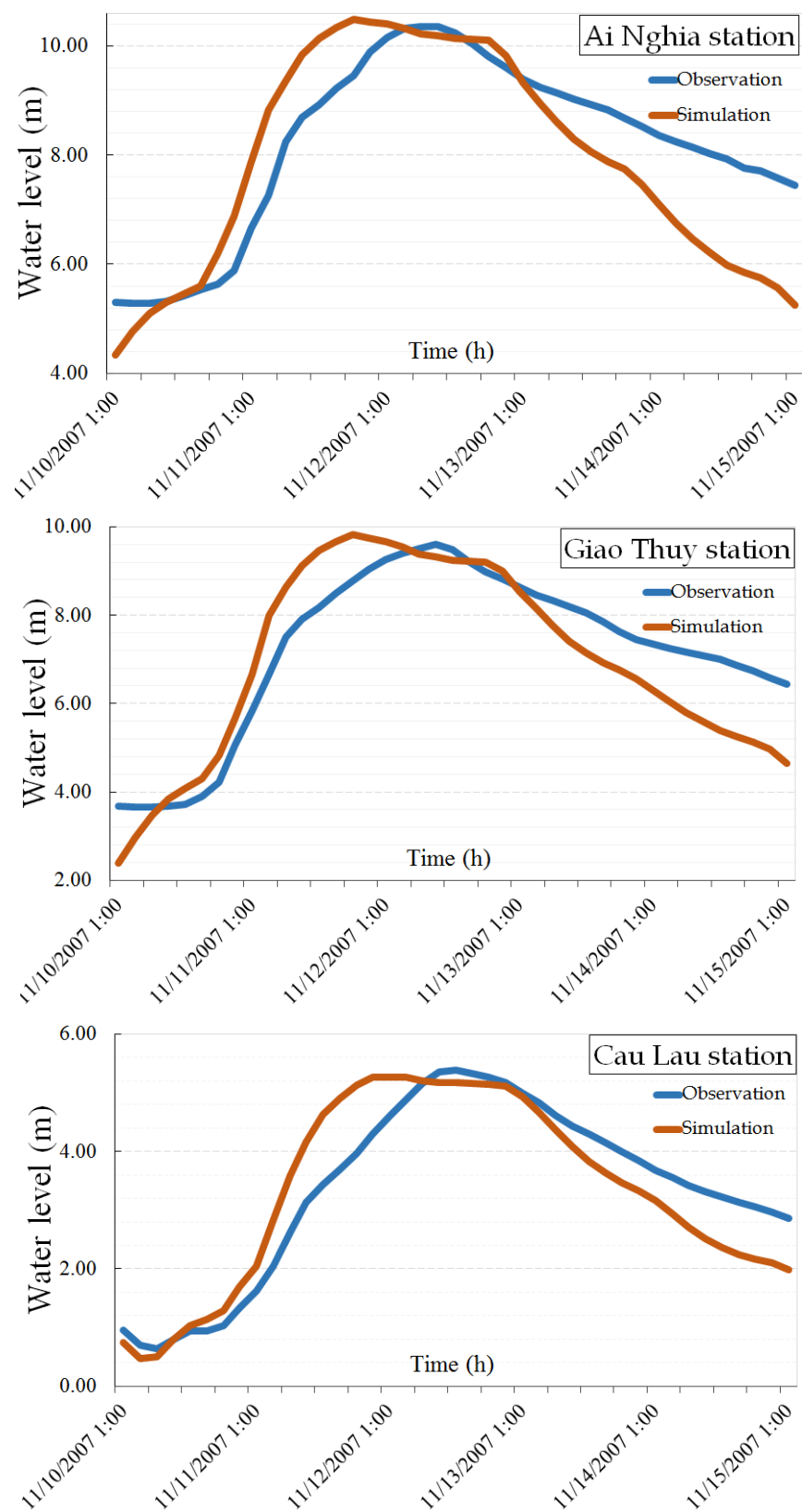
Figure 4.34. Model and observed hydrograph of water level.
