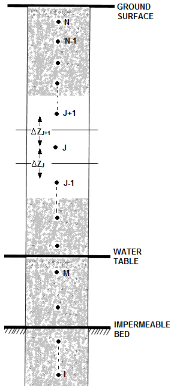
Figure 3.6. Vertical discretization in unsaturated zone. (DHI, 2012e)
