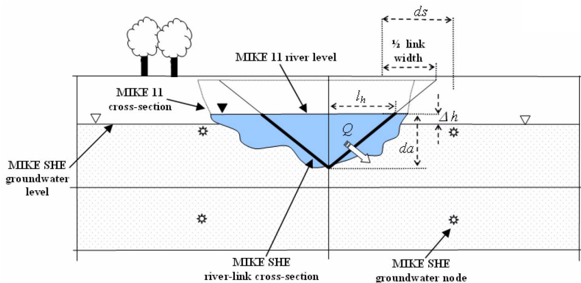
Figure 3.8. A typical simplified MIKE SHE River link cross section compared to the equivalent MIKE 11 cross section (DHI, 2012e).
