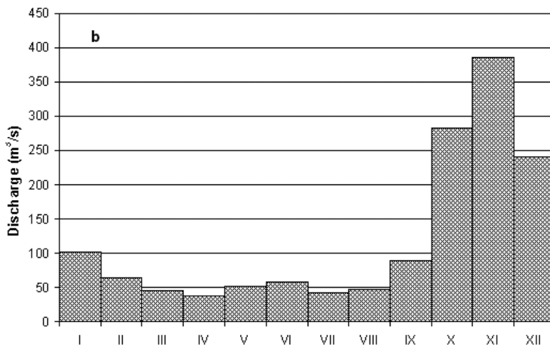
Figure 2.4 Average monthly flow at Thanh My station (Dang, 2009)
