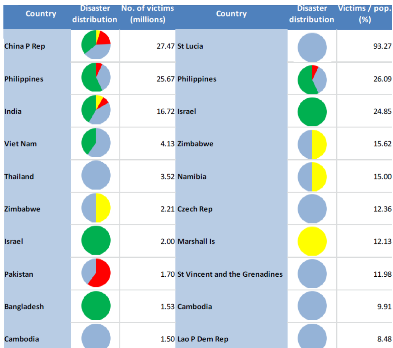
Figure 1.3 Top 10 countries by victims in 2013 and distributed by disaster type (Guha-sapir et al. , 2013)
