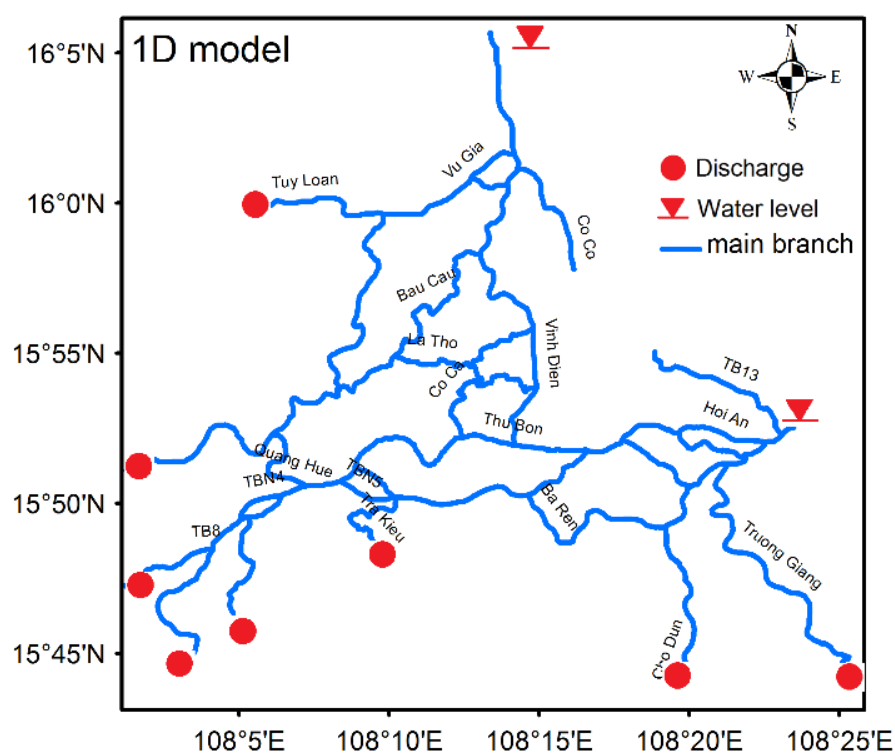
Figure 4.17. MIKE 11 (1D) model set up for Vu Gia Thu Bon river downstream.
