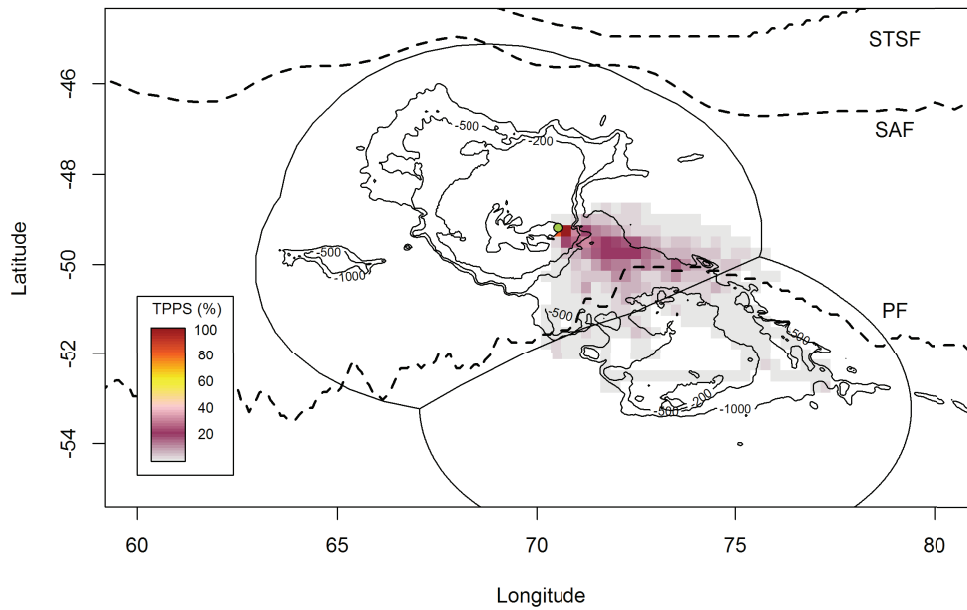
400 Fig.5 Standardised time spent per square from KIPPE tracking data. Contours of the 401 Kerguelen Plateau, Colony (green point) and Exclusive Economic Zones (solid lines) 402 and Front zones (dashed lines) are represented.
