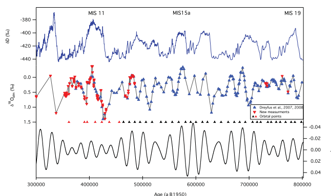
Fig. 1. EDC records between 300 and 800 ka on the EDC3 age scale. Top: water stable isotope ( \delta\text{D} ) record with labeling of selected interglacial periods (Jouzel et al., 2007). Middle: complete record of \delta^{18}\text{O}_{\text{atm}} , blue triangles from Dreyfus et al. (2007, 2008) and red triangles from this study. Bottom: precession parameter (here on a reverse y axis) obtained with the Analyseries software (Paillard et al., 1996), calculated using the Laskar et al. (2004) solution. Black points indicate the position of tie points between \delta^{18}\text{O}_{\text{atm}} and precession parameter signals from Dreyfus et al. (2007); the red ones are from this study (Table 1).
