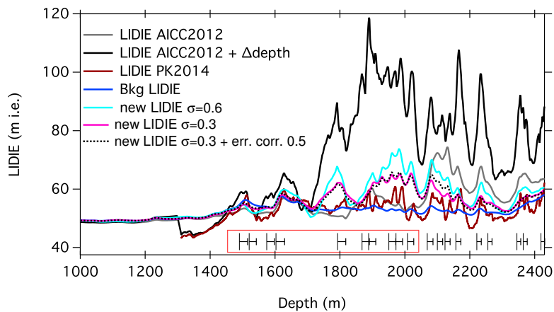
Figure 5. Comparison of NGRIP LIDIE over the glacial period. The LIDIE obtained when building the AICC2012 chronology (grey), the same as AICC2012 + \Delta depth markers deduced from Kindler et al. (2014) (black) and the LIDIE obtained from the \delta^{15}\text{N} data Kindler et al. (2014) are shown for comparison. The background LIDIE used as input is in dark blue. The output LIDIE after running Datice are also presented, in light blue when using the same error as in AICC2012 and in pink/black dotted line when reducing this error. The markers present at the bottom correspond to the \Delta depth markers implemented in Datice. The ones in the red box are new \Delta depth markers deduced from the data of Kindler et al. (2014).
