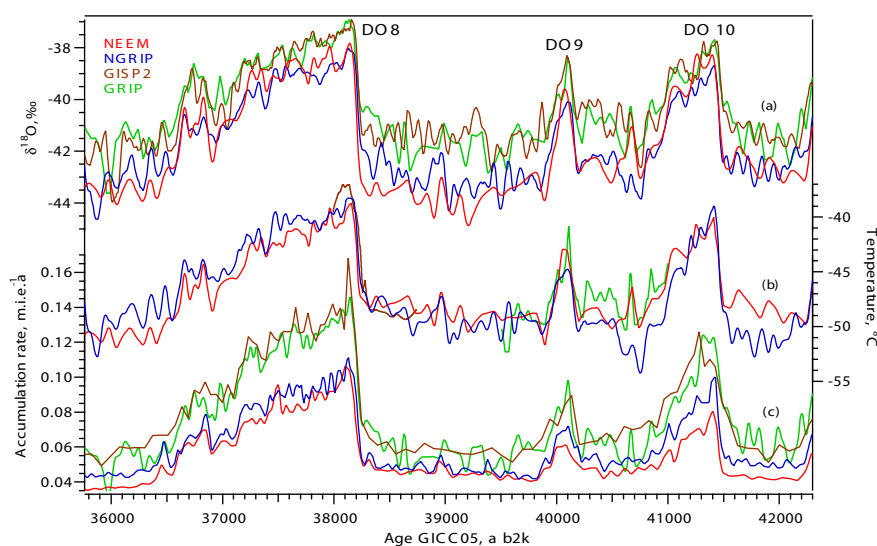
Fig. 4. NEEM (red), NGRIP (blue), GISP2 (brown) and GRIP (green) comparison. (a) Water isotopes, 50 yr running average, ‰ vs. VS-MOW. NEEM: this study. NGRIP: NGRIP members (2004). GISP2: Grootes et al. (1993). GRIP: Johnsen et al. (1992). (b) Temperature reconstruction, °C. (c) Accumulation rate reconstruction, \text{m.i.e.a}^{-1} .
