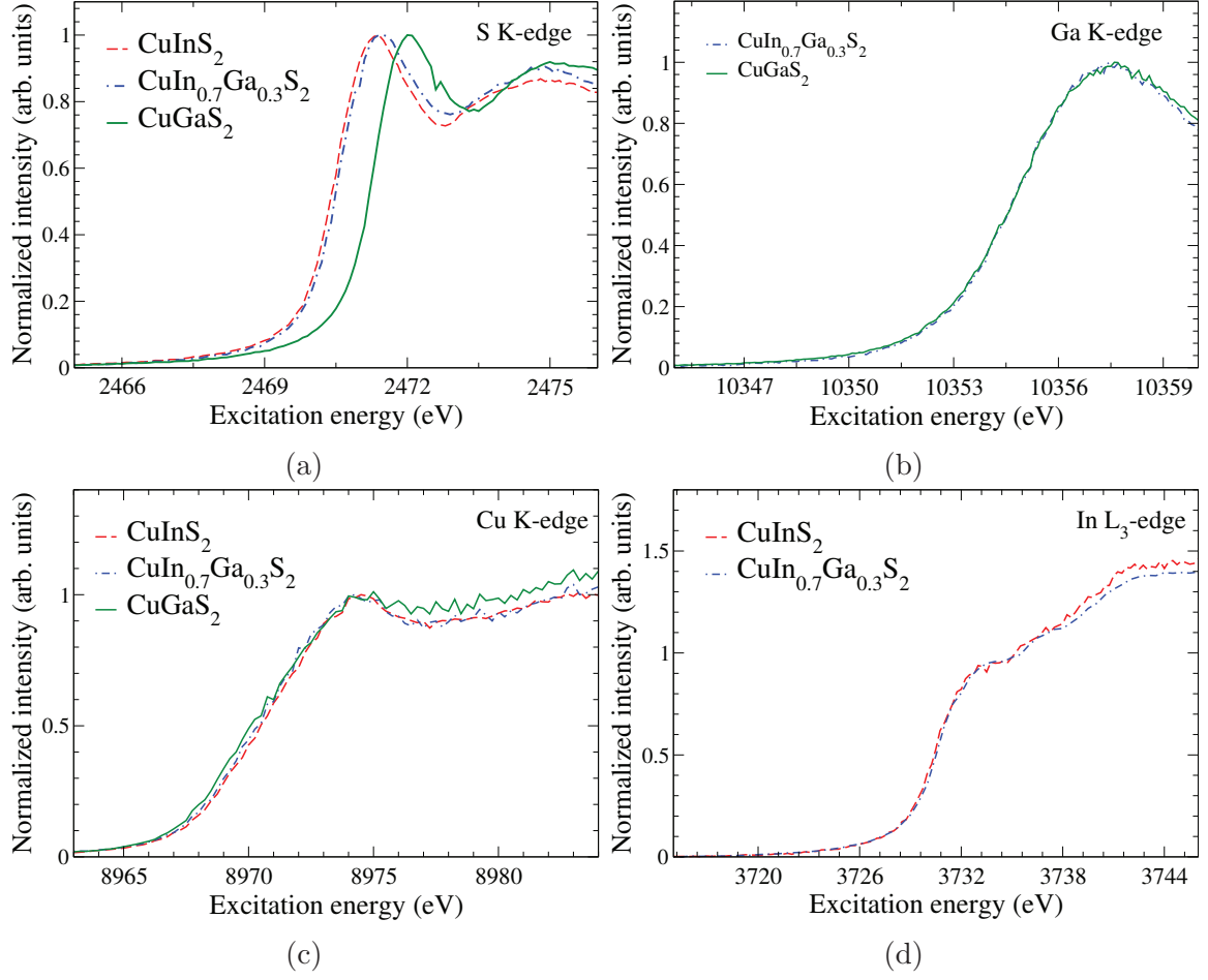
Fig. 3.8 Experimental results for samples of CuInS 2 , CuGaS 2 and CuIn 0.7 Ga 0.3 S 2 , from Reference [131]. a) Measured absorption K-edges of S, b) Measured absorption K-edges of Ga, c) Measured absorption K-edges of Cu, d) Measured absorption L 3 -edges of In
