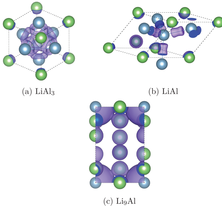
Fig. 2.15 Electronic density in the unit cell of \text{LiAl}_3 , \text{LiAl} , and \text{Li}_9\text{Al} . (aluminium, blue and lithium, green)
