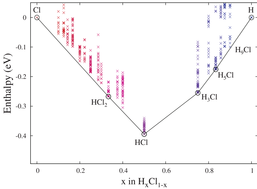
Fig. 2.16 Phase diagrams of the H-Cl system at 50 GPa (top) and 100 GPa (bottom).
