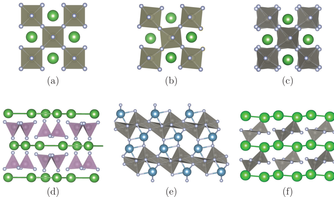
Fig. 3.5 The most relevant crystal structures obtained in our work: (a) the starting cubic perovskite structure (space group 221); (b) the orthorhombic perovskite structure (space group 62) of \text{LaReN}_3 and \text{YReN}_3 ; (c) the trigonal structure (space group 161) of \text{LaWN}_3 ; (d) The monoclinic structure (space group 15) adopted by \text{LaMoN}_3 , \text{LaTcN}_3 , \text{CaReN}_3 , \text{SrReN}_3 , \text{BaReN}_3 , \text{YWN}_3 , \text{LaCrN}_3 , \text{SrTcN}_3 , and \text{YTcN}_3 ; (e) The monoclinic structure (space group 12) adopted by \text{CaWN}_3 , \text{CaMoN}_3 , and \text{CaTcN}_3 ; (f) The monoclinic structure (space group 14) adopted by \text{BaWN}_3 and \text{LaTaN}_3 .
