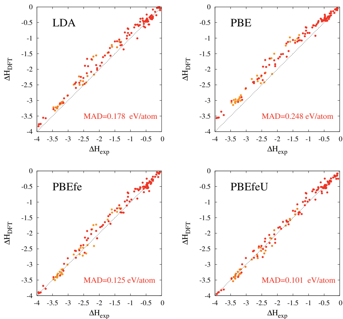
Fig. 4.6 Calculated versus experimental energies of formation in the control set for different exchange-correlation functionals. Orange dots correspond to ternary compounds. The MAD is indicated in each graph.
