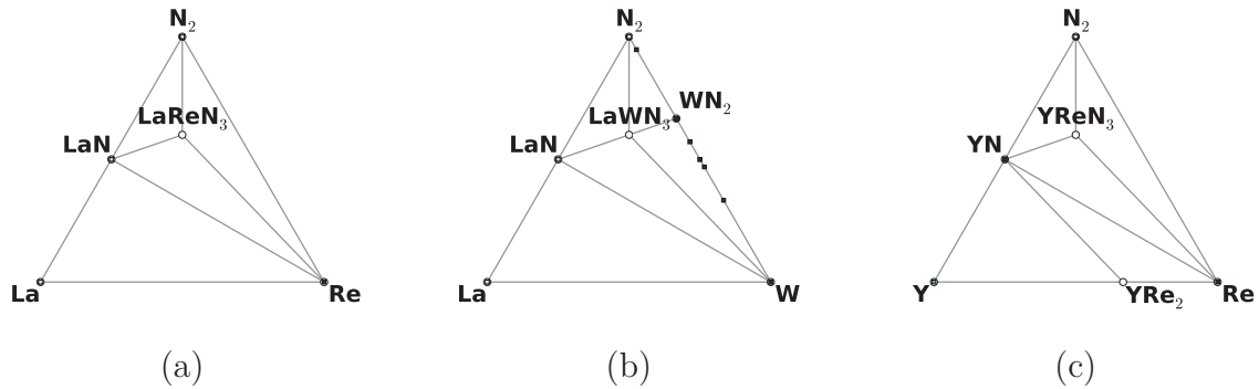
Fig. 3.6 Theoretical ternary phase diagrams for (a) \text{LaReN}_3 , (b) \text{LaWN}_3 , and (c) \text{YReN}_3 .
