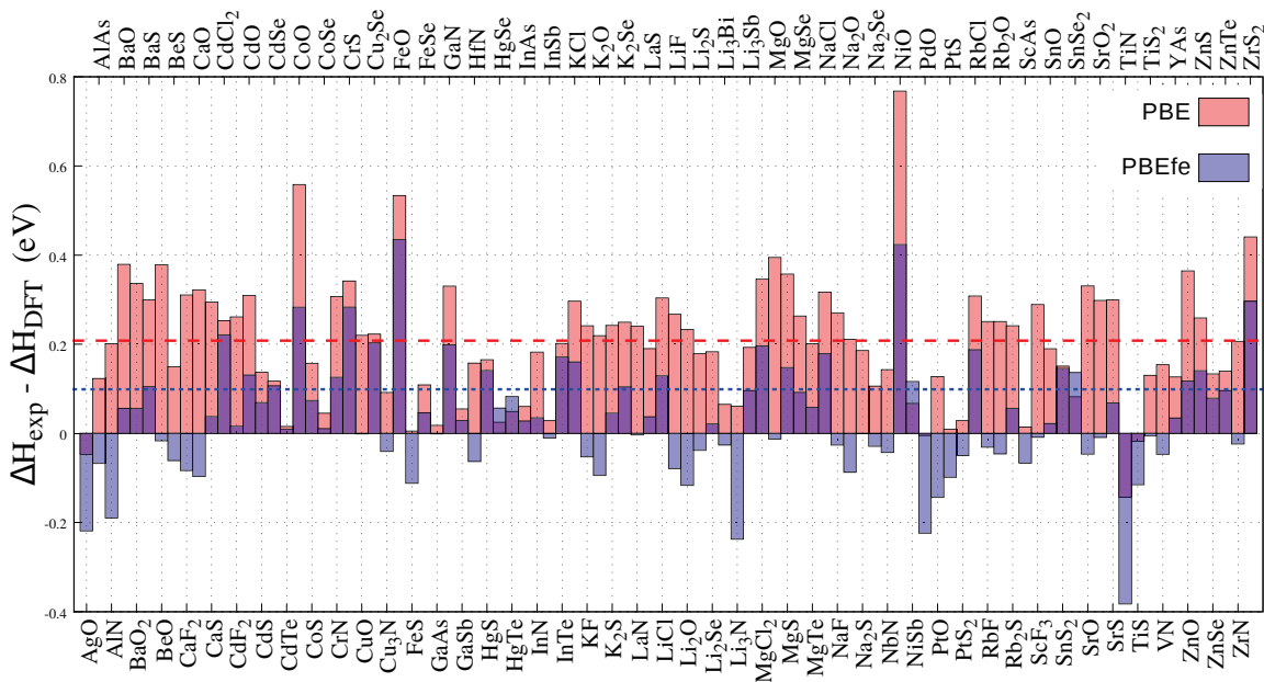
Fig. 4.2 Errors of the calculated energies of formation with the PBE and the PBEfe functionals. The orange long-dashed line represents the MAD of the PBE and the blue short-dotted line represent the MAD of PBEfe. Transparent colors have been used to show the orange bars when they are shorter than the corresponding blue one.
