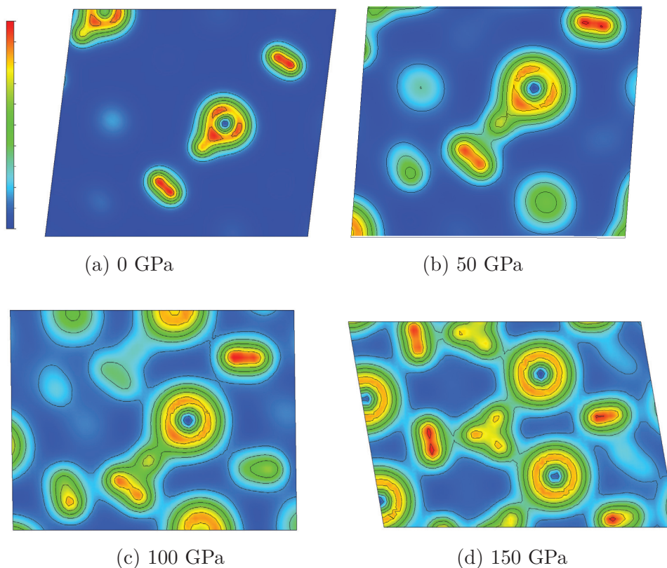
Fig. 2.21 Slices of the electronic density in the H 5 Cl cell at different pressures.
