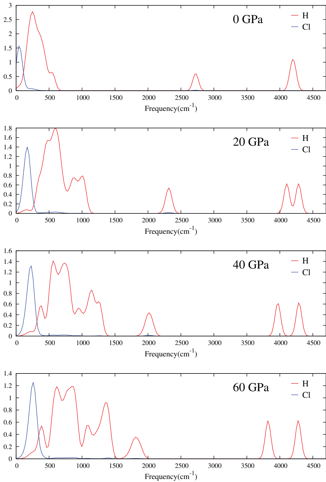
Fig. 2.18 Phonon density of states for the Cc phase of \text{H}_5\text{Cl} .
