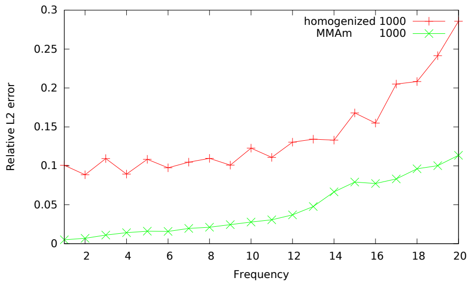
Figure 4.25: Homogenization vs MMam: 51 layers, 1000 m.s -1 contrast
