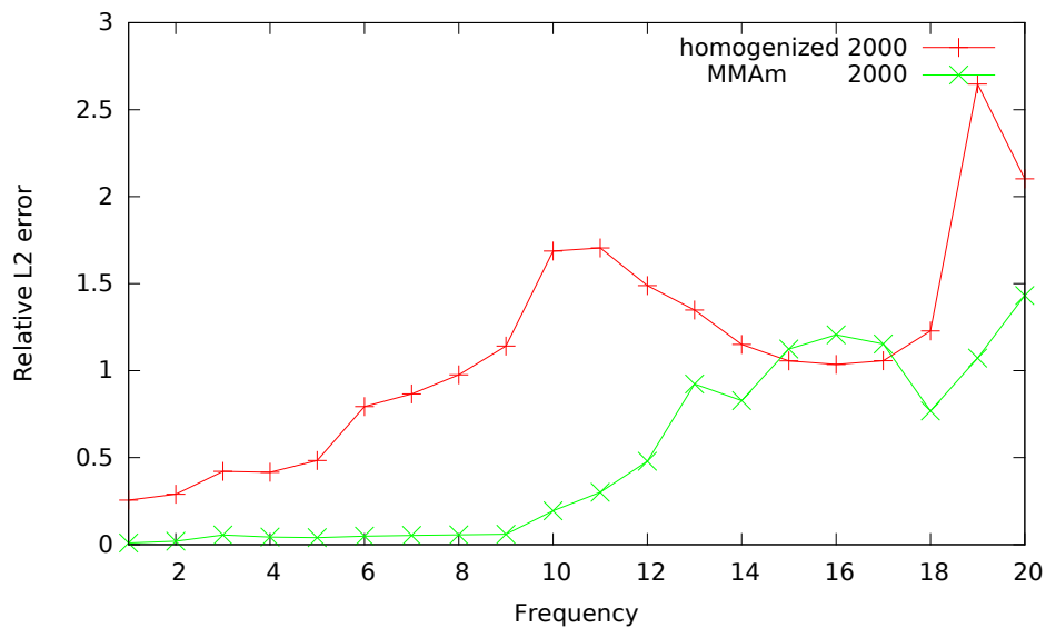
Figure 4.21: Homogenization vs MMAM: 21 layers, 2000 \text{ m.s}^{-1} contrast
