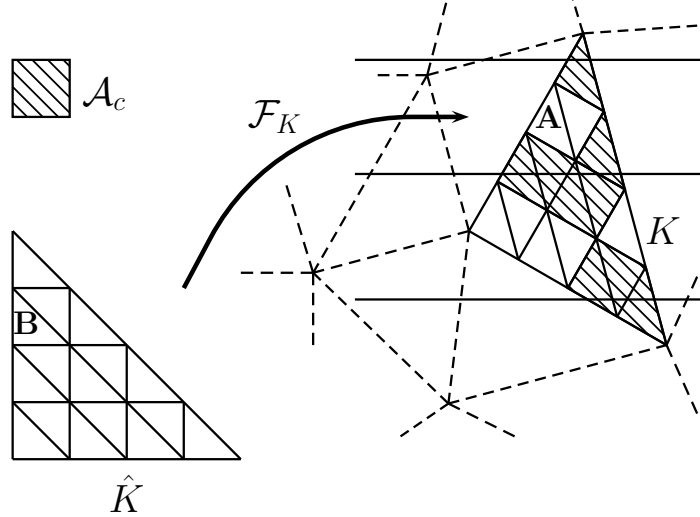
Figure 3.3: Mapping of the reference submesh
