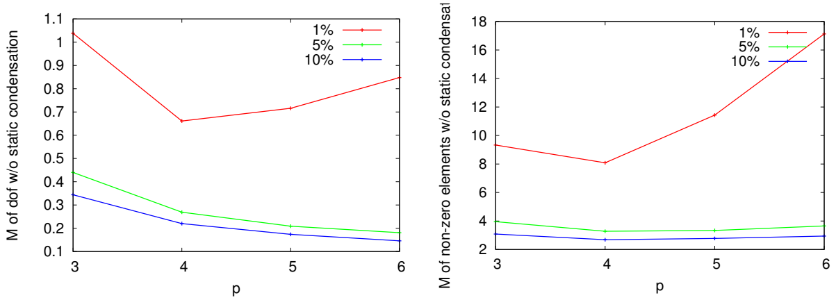
Figure 4.53: Number of degrees of freedom and non-zero elements in the linear system without static condensation for f = 20\text{hz}
