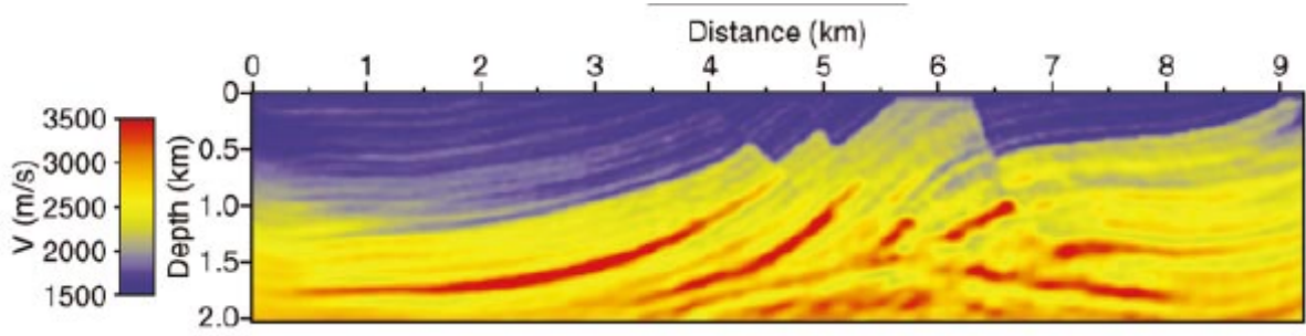
Figure 1.7: Output model from FWI
