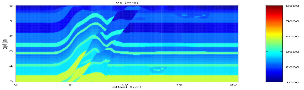
Figure 4.58: Overthrust S-velocity model
