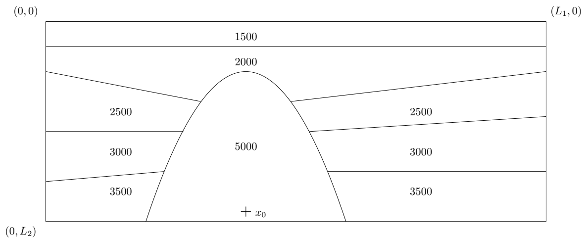
Figure 3.2: A velocity parameter with a salt body
