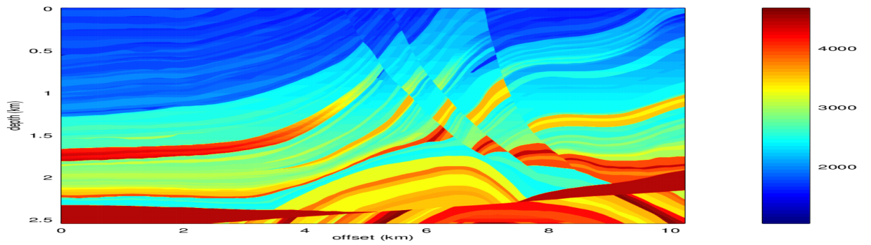
Figure 4.45: Marmousi II P-velocity model
