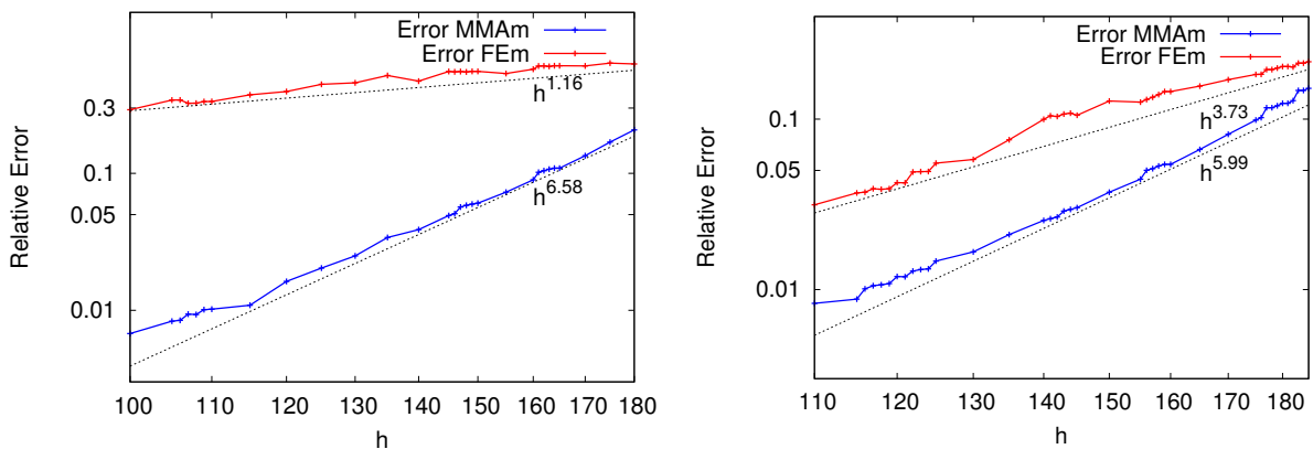
Figure 4.36: Convergence curves for p = 4 in the original (left) and smoothed (right) media
