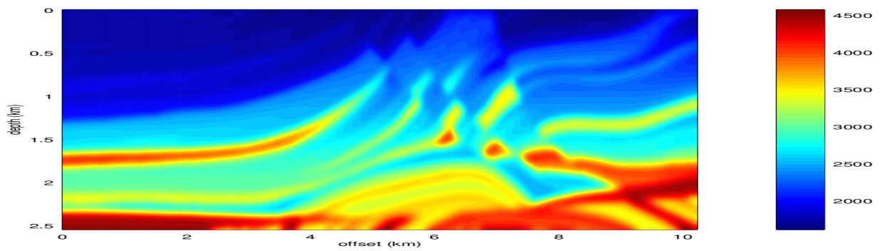
Figure 4.47: Marmousi II smoothed P-velocity model
