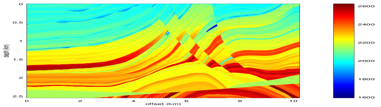
Figure 4.46: Marmousi II density model
