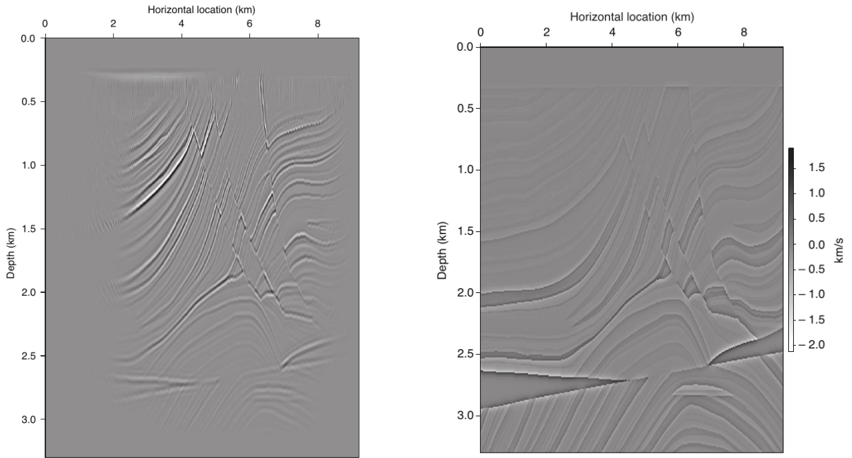
Figure 1.3: Output of the RTM (left) and true reflectivity (right)
