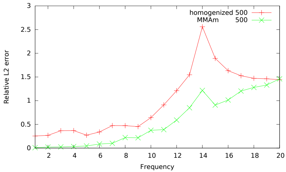
Figure 4.24: Homogenization vs MMam: 51 layers, 2000 m.s -1 contrast
