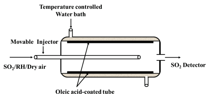
FigureS1. Schematic diagram of the flow tube reactor.
