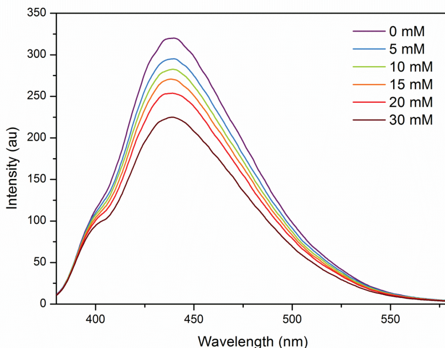
Figure III-2: Fluorescence emission spectrum of CPT in presence of different concentrations of NaBr ( \lambda_{ex}=350 nm, pH=7.1)
