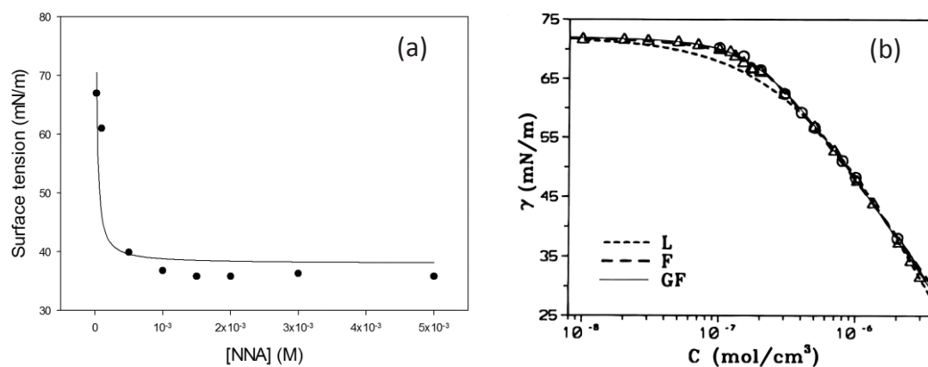
Figure II-10: Surface tension in function of bulk concentration for (a) nonanoic acid (adapted from Ciuraru et al., 2015) and (b) 1-octanol (Lin et al., 1997)
