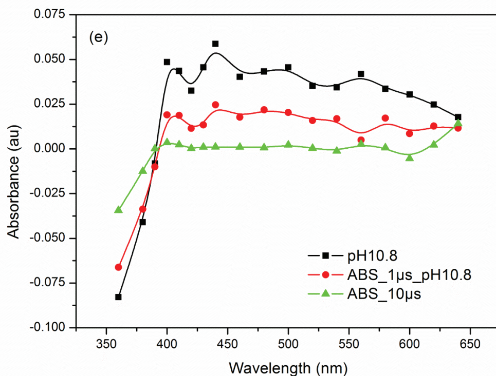
Figure III-S3: Transient absorption spectrum of triplet state CPT (0.1 mM) at different pH, recorded 450 ns, 1 \mu s and 10 \mu s after laser flash: (a) pH 6.1, (b) pH 7.3, (c) pH 8.2, (d) pH 9, (e) pH 10.8.
