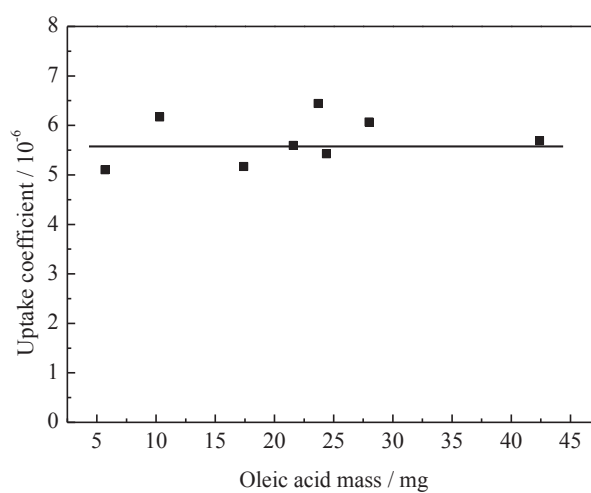
Figure S4. Dependence of uptake coefficient with oleic acid mass. Experimental Conditions: oleic acid mass = 5.7, 10.3, 17.4, 21.6, 23.7, 24.4, 28.0, 42.4 mg; RH = 3~4 %, \text{SO}_2 initial concentration = 2.0\sim 2.1 \times 10^{12} molecular \text{cm}^{-3} ; flow rate = 300 \text{mL min}^{-1} .
