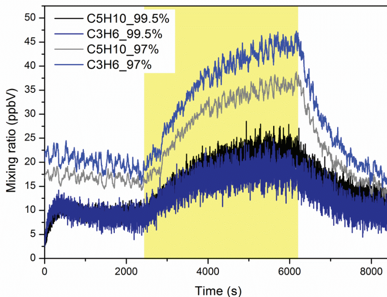
Figure VI-5: Time traces of two major compounds measured in the \text{H}_3\text{O}^+ ionization mode above an irradiated (1h) aqueous solution of 2 mM NA of 97% purity (brighter colors) and 99.5% purity (darker colors) with \text{N}_2 as carrier gas. The given concentrations are background corrected.
