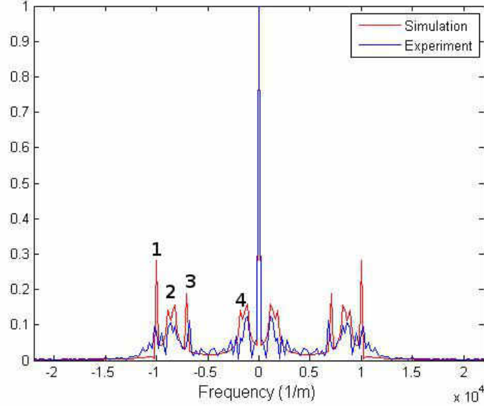
Fig. 7.31: FFT of the intensity distribution in simulation (red) and experiment (blue).
