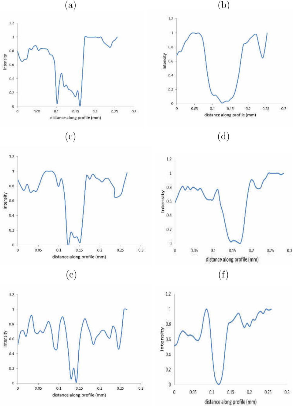
Fig. 5.7: Intensity profile of simulated reconstruction particle with 20\mu\text{m} diameter (a), 10\mu\text{m} diameter (c), and 5\mu\text{m} diameter (e). (b), (d), and (f) are the experimented intensity profile of 20\mu\text{m} , 10\mu\text{m} , 5\mu\text{m} particle, respectively.
