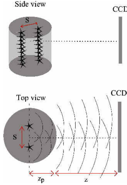
Fig. 7.5: Simulation set-up: side view and top view.
