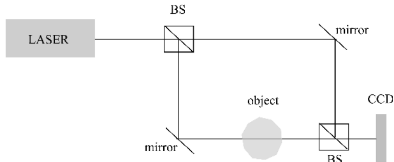
Fig. 1.12: DHI set-up.
