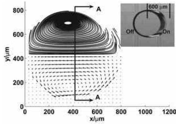
Fig. 1.4: The slab velocity field at z = 148\mu m inside a droplet is shown in the bottom half and its streamline is shown in the top half [20].
