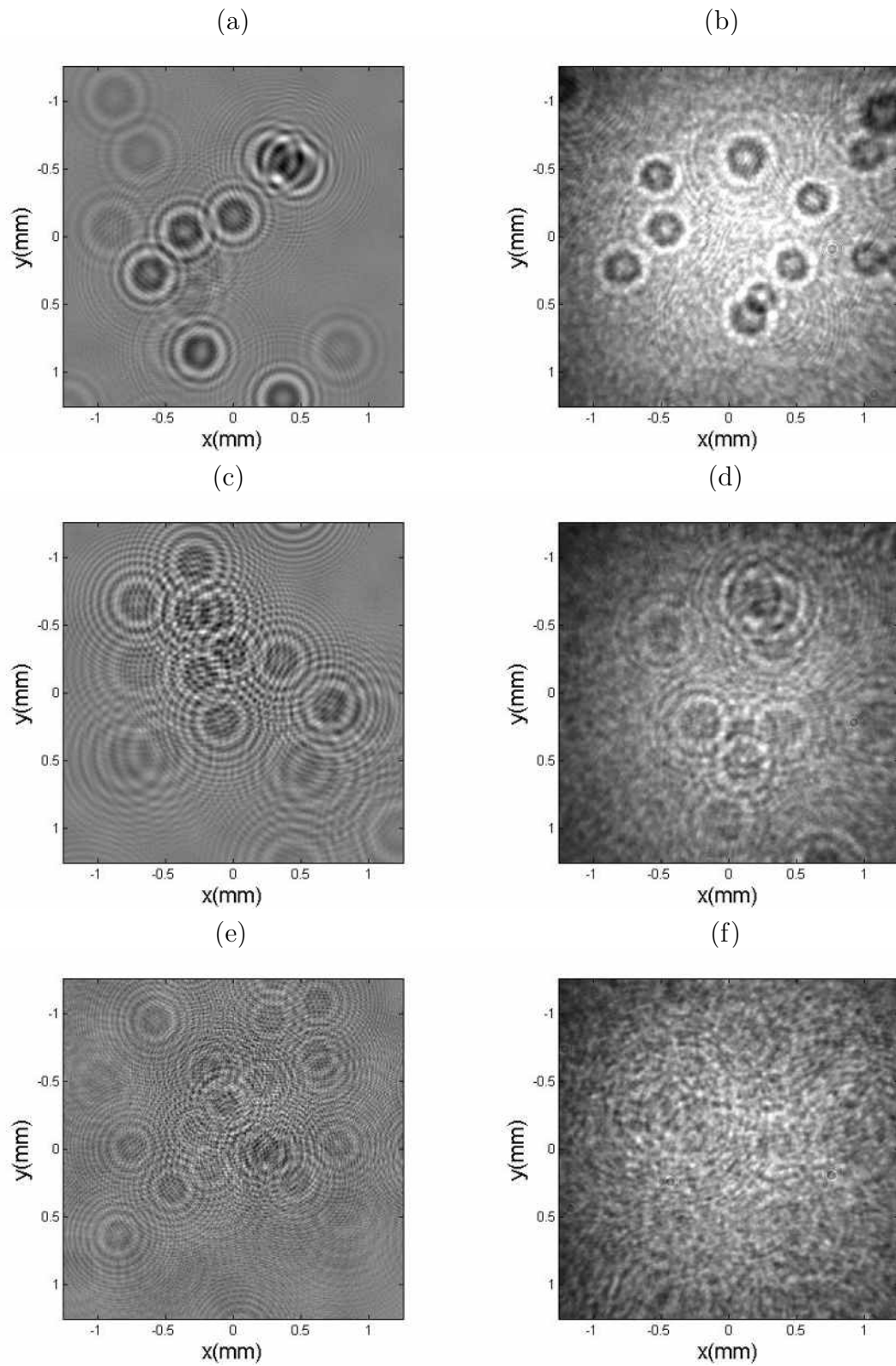
Fig. 5.3: Simulated hologram of 20 \mu\text{m} , 10 \mu\text{m} , and 5 \mu\text{m} particles are shown in (a),(c), and (e). Experimental holograma of 20 \mu\text{m} , 10 \mu\text{m} , and 5 \mu\text{m} particles are shown in (b),(d), and (f), respectively.
