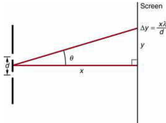
Fig. 7.4: Double slit interference*
