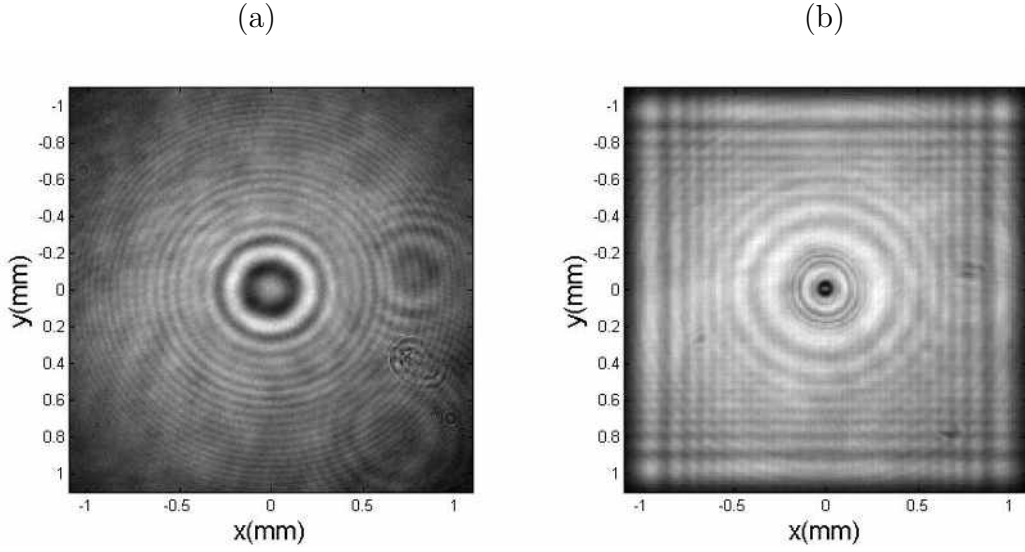
Fig. 3.23: (a) is the hologram of 20\mu m glass inclusion inside a droplet. (b) is the reconstruction image of (a) with fractional orders a_x = 0.8\pi/2 and a_y = 0.77\pi/2
