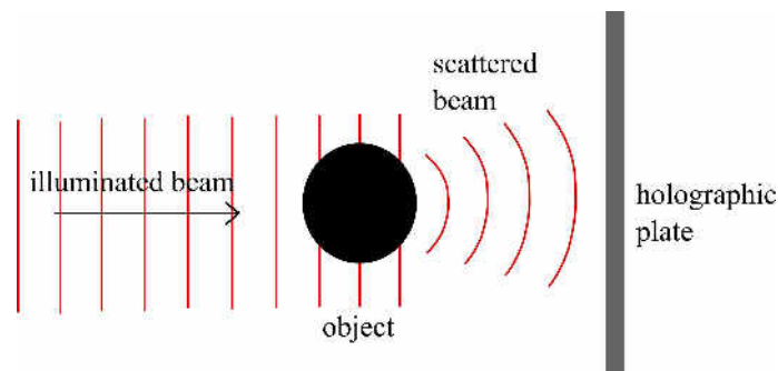
Fig. 1.9: Set-up of Gabor's hologram for recording.
