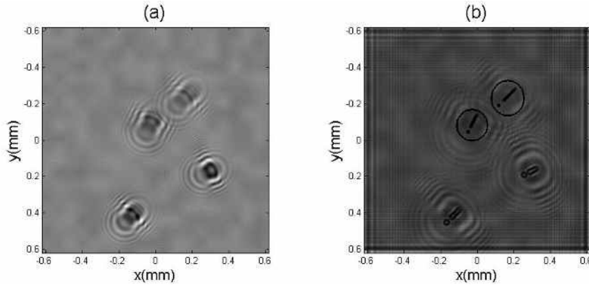
Fig. 6.4: Hologram recorded under a double exposure light source with 0.03\text{s} and 0.15\text{s} exposure time (a) and its reconstruction image (b) with fractional order \alpha = 0.67\pi/2 .
