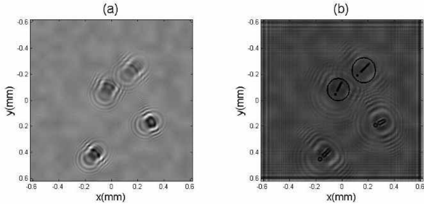
Fig. 6.4: Hologram recorded under a double exposure light source with 0.03\text{s} and 0.15\text{s} exposure time (a) and its reconstruction image (b) with fractional order \alpha = 0.67\pi/2 .
