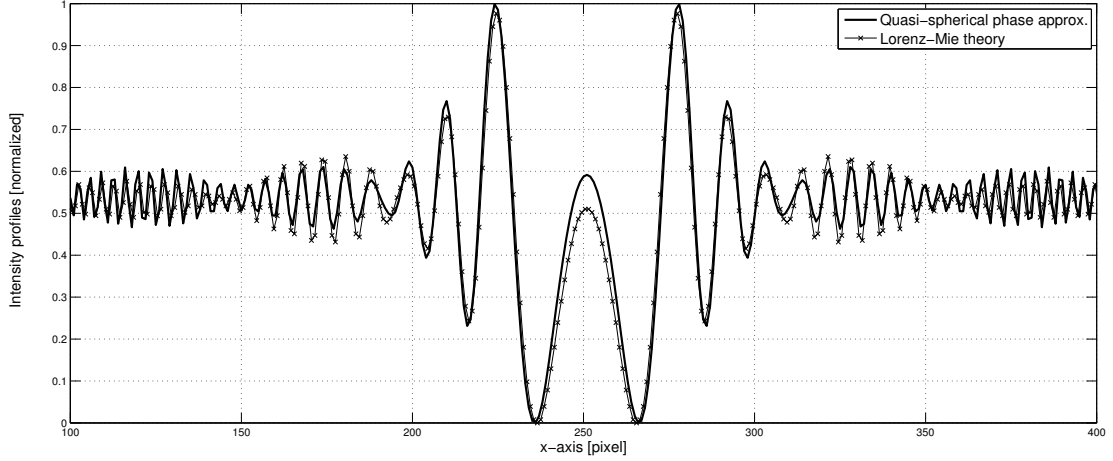
Fig. 3.16: Simulated intensity profile of a droplet with quasi-spherical phase approximation.
