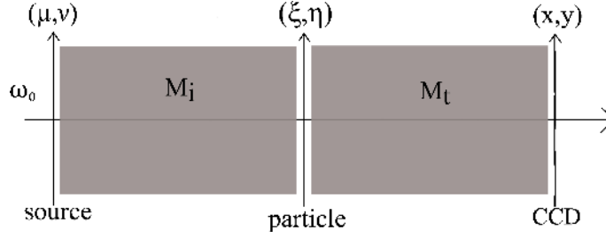
Fig. 3.1: In-line configuration of digital holography
