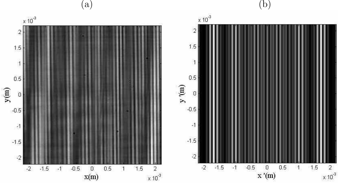
Fig. 7.29: Experimental interference pattern of quard-core pipe (a) and numerical interference pattern of quard-core pipe (b) without rotation.
