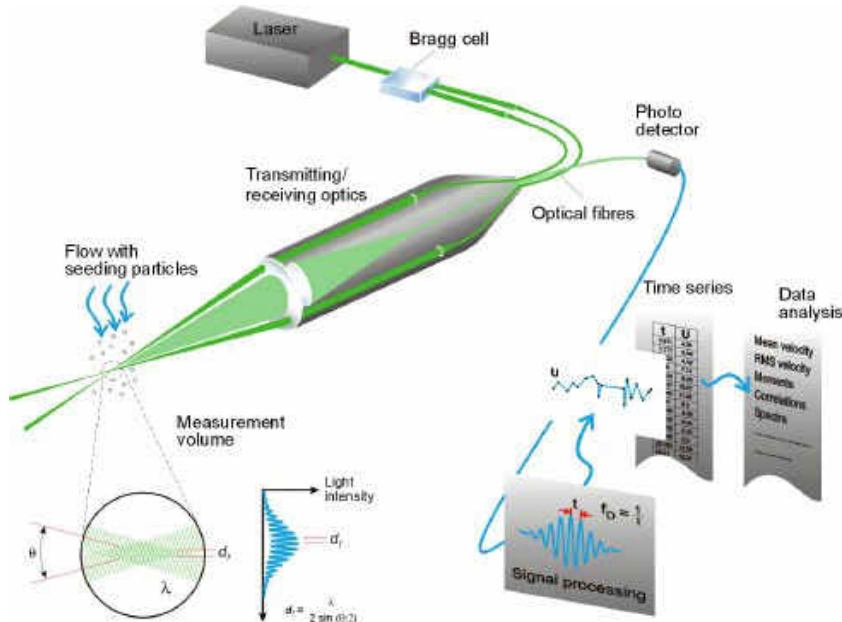
Fig. 1.5: Set-up of laser Doppler anemometry [29].
