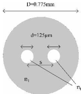
Fig. 7.6: Top view of pipe with indicated parameters.
