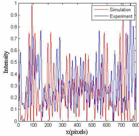
Fig. 7.30: Intensity profile of the interference fringes of simulation (red) and of experiment (blue).
