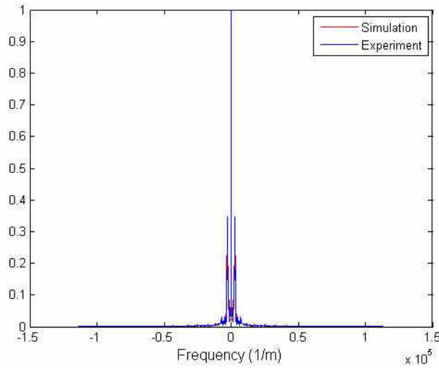
Fig. 7.25: FFT of the intensity profile in Fig. 7.24.
