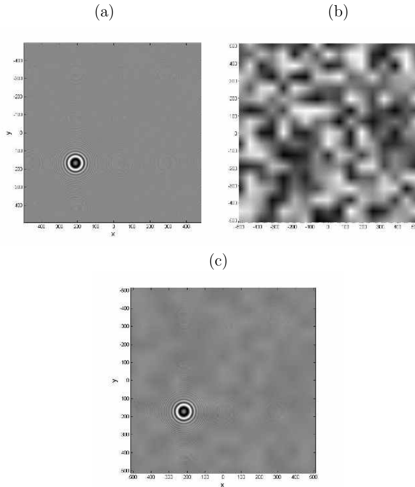
Fig. 4.25: (a) Hologram without any noise. (b) Generated noise. (c) Interpolated image between hologram in (a) and noise in (b).
