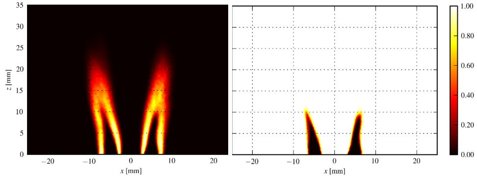
(b) Adiabatic simulation. (left) Normalized mean volumic heat release. (right) Mean binarized OH molar fraction X_{OH}
