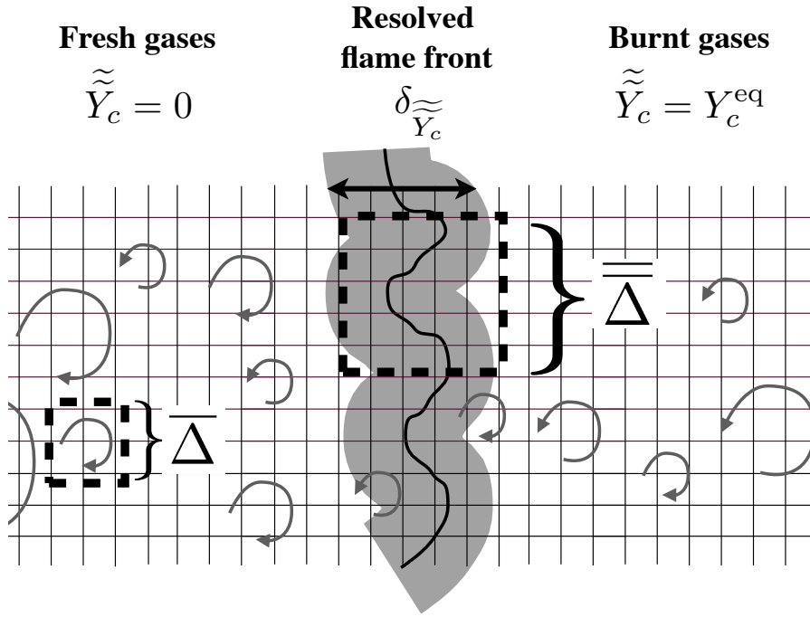
Figure 5.1: Filter size issues in premixed turbulent combustion LES.
