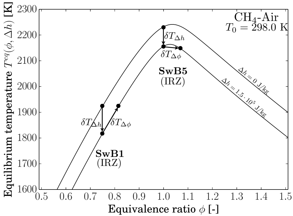
Figure 3.34: Equilibrium temperature function of fresh gas equivalence ratio \phi for adiabatic and non-adiabatic situations. CH 4 -Air fresh gas temperature is taken equal to T_0 = 298.0 K. Legend: upper curve: adiabatic ( \Delta h = 0 ); lower curve: non-adiabatic ( \Delta h = 1.5 \cdot 10^5 J/kg).
