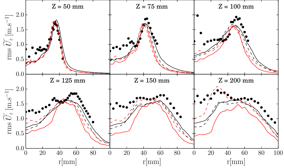
Figure 3.9: RMS of axial velocity at six distances Z from the pilot tube exit. Legend : — Adiabatic, Le \neq 1 . - - - Adiabatic, Le = 1 . — Non-adiabatic, Le \neq 1 . - - Non-adiabatic, Le = 1 . ●● TSF-A-r measurements.
