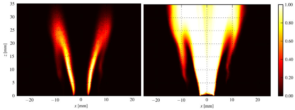
(c) Non-adiabatic simulation. (left) Normalized mean volumic heat release. (right) Mean binarized OH molar fraction X_{OH}
