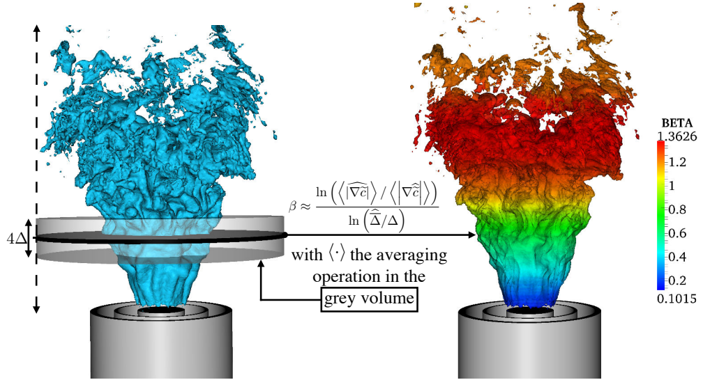
Figure 4.4: Instantaneous iso-surfaces of the filtered progress variable reaction rate \widetilde{\omega}_{Y_c} . (Left) Schematic view of the volume averaging operation needed for the dynamic estimation of the \beta parameter. (Right) The iso-surface is colored by the \beta parameter computed at a given instant using the dynamic procedure.
