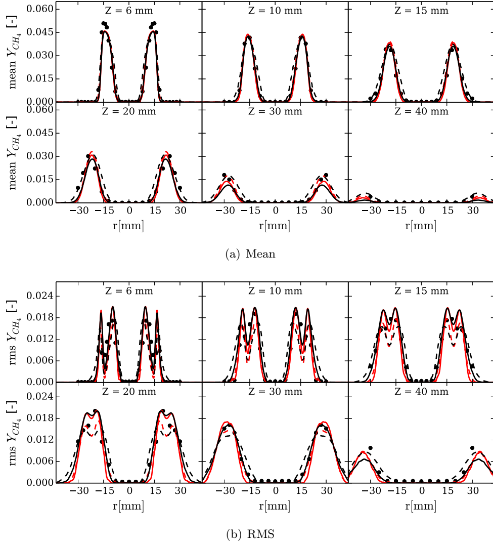
Figure 5.12: Radial profiles of \text{CH}_4 extracted from the LES of the PRECCINSTA burner using coarse (black lines) and fine (red lines) meshes. Legend: F -TACLES model ( \tilde{Y}_{\text{CH}_4} : - - -) ; F2 -TACLES ( \tilde{Y}_{\text{CH}_4} : —) ; Experiments ( \bullet \bullet ).
