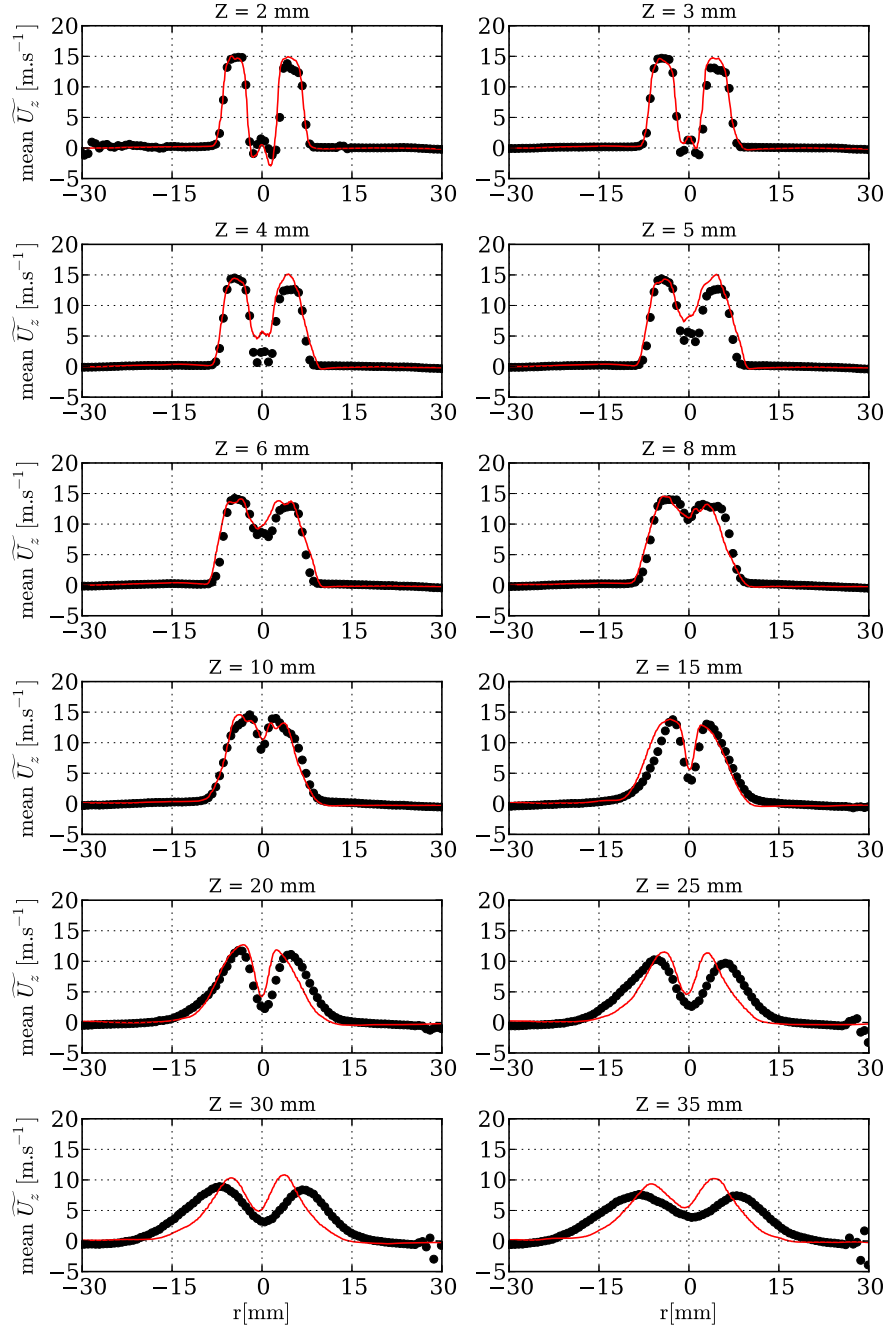
Figure 6.11: 1-D radial mean profiles of U_z axial velocity component at different axial positions Z in the longitudinal plane Y = 0 \text{ mm} . Red lines and black symbols correspond to LES calculations and PIV measurements, respectively.
