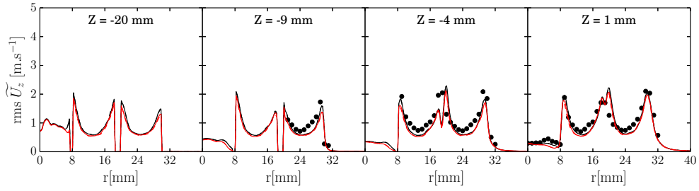
(b) RMS of axial velocity U_z
