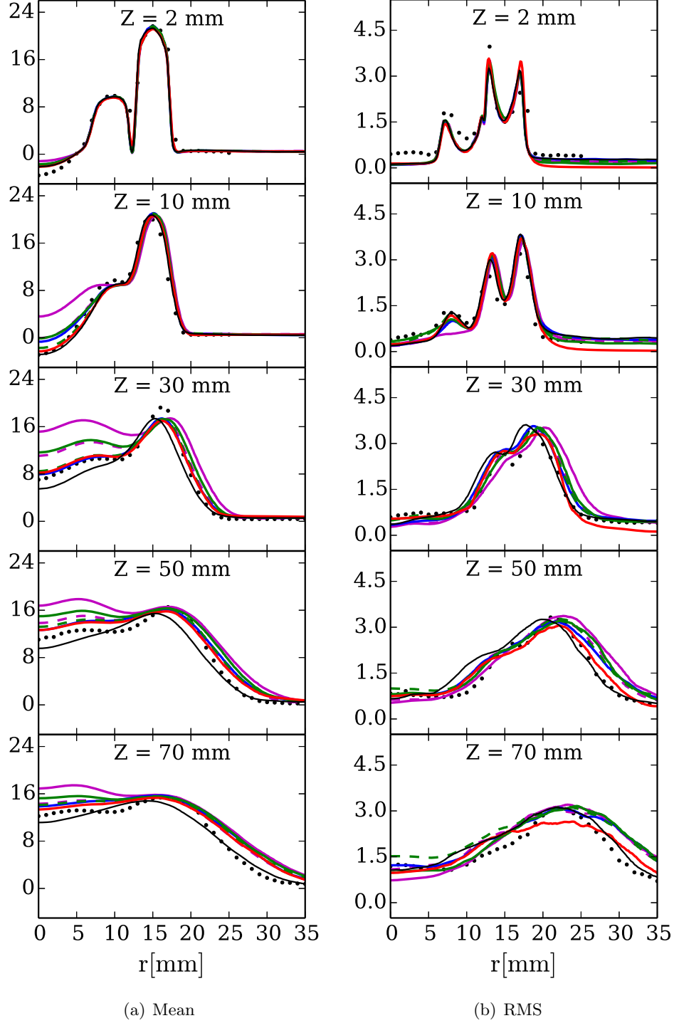
Figure 4.5: Radial profiles of mean and RMS of axial velocity \tilde{U}_z [ m.s^{-1} ] for the stratified case (SwB5). Legend: - - - SWB5-NAD-CH1; — SWB5-NAD-CH2; — SWB5-NAD-CO; — SWB5-NAD-B5; - - - SWB5-NAD-B3; — SWB5-NAD-BD; — SWB5-NAD-B0; • • Experiments.
