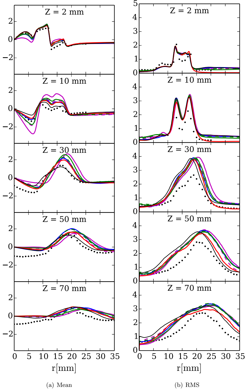
Figure 4.6: Radial profiles of mean and RMS of radial velocity \tilde{U}_r [ m.s^{-1} ] for the stratified case (SwB5). Legend: - - - SWB5-NAD-CH1; — SWB5-NAD-CH2; — SWB5-NAD-CO; — SWB5-NAD-B5; - - - SWB5-NAD-B3; — SWB5-NAD-BD; — SWB5-NAD-B0; • • Experiments.
