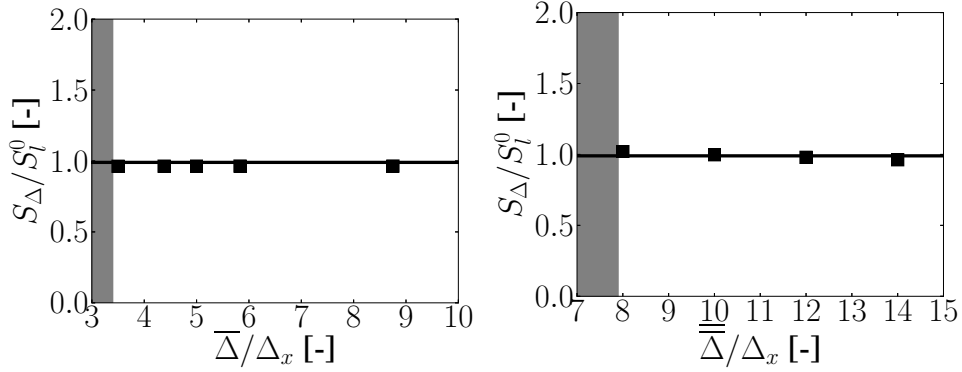
Figure 5.7: Left: S_{\Delta}/S_l^0 in terms of \overline{\Delta}/\Delta_x with \overline{\Delta} = 1.75 mm and \overline{\overline{\Delta}} = 7 mm. Right: S_{\Delta}/S_l^0 in terms of \overline{\overline{\Delta}}/\Delta_x with \overline{\Delta} = 1.75 mm and \Delta_x = 0.5 mm. Inside the grey surface, simulation where unstable and the predicted flame speed value was meaningless.
