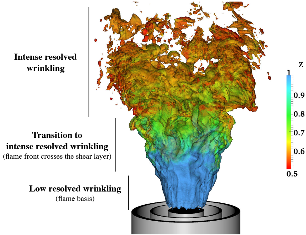
Figure 4.1: Instantaneous iso-surface of the filtered progress variable reaction rate \tilde{\omega}_{Y_e} colored by the resolved mixture fraction \tilde{z} for the non-adiabatic stratified computation of the SwB5 flame (SWB5-NAD-BD).
