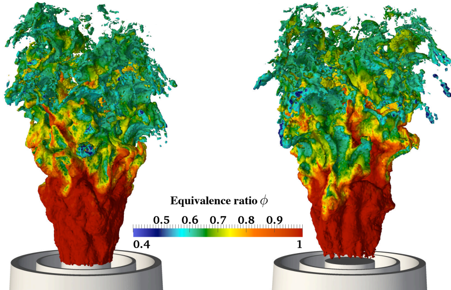
Figure 3.30: Isosurface of filtered progress variable reaction rate \tilde{\rho}\tilde{\omega}_{Y_c} = 0.5\tilde{\rho}\tilde{\omega}_{Y_c}^{max} colored by fresh gas equivalence ratio \phi for the stratified (SwB5) case. Left: Adiabatic computation (SWB5-AD). Right: Non-adiabatic computation (SWB5-NAD).
