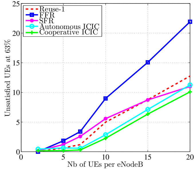
Figure 5.7: Unsatisfied UEs at 63% versus network load
