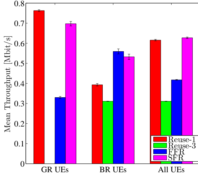
Figure 2.9: Mean Throughput per GR, BR, and all UEs
