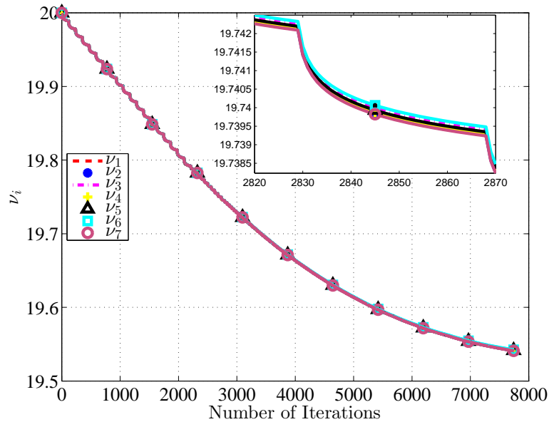
Figure 3.4: Lagrange prices \nu_i
