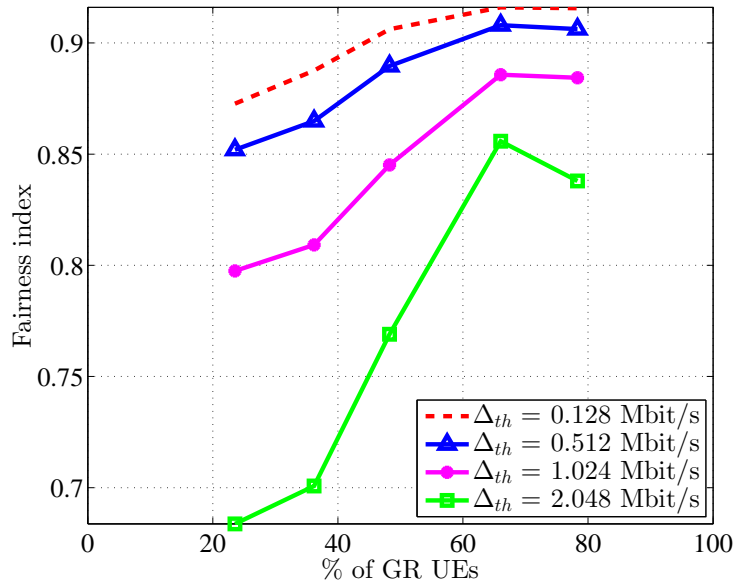
Figure 4.11: Fairness index versus UE distribution
