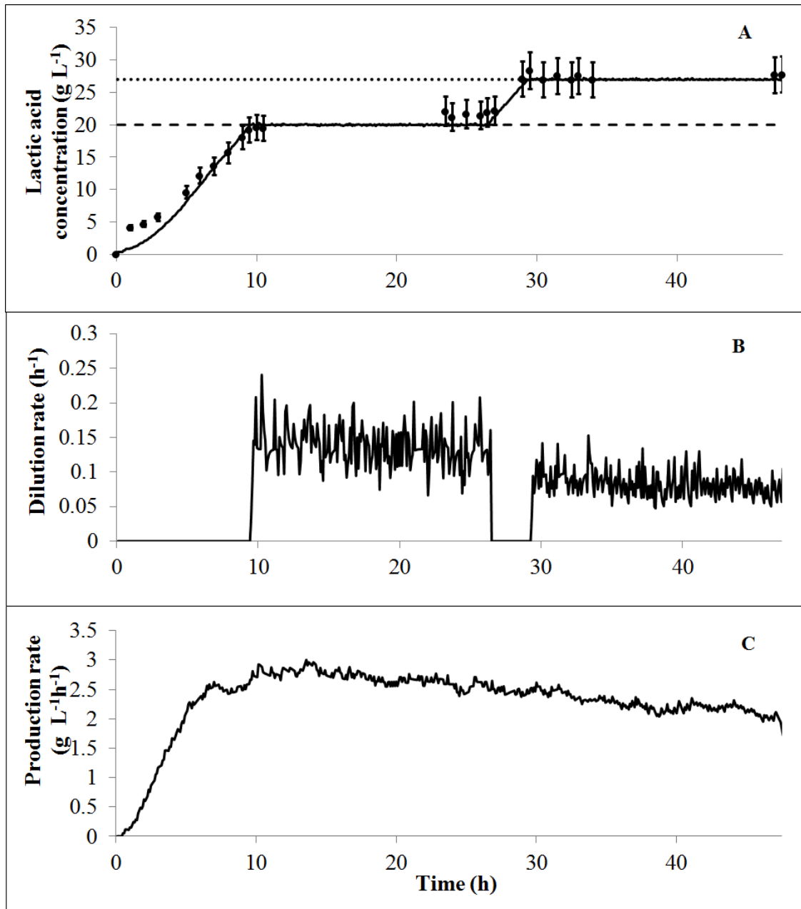
Figure 5.8. Adaptive control law experimental validation. A Lactic acid concentration evolution with time. Pref 1= 20g L -1 (— —), Pref 2= 27 g L -1 (.....), lactic acid concentration available (—) and lactic acid offline measurement (●). B Dilution rate evolution with time. C Estimated production rate.
