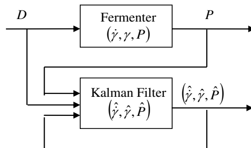
Figure 4.7 Kalman Filter structure for production rate estimation (linear model for \gamma ).
