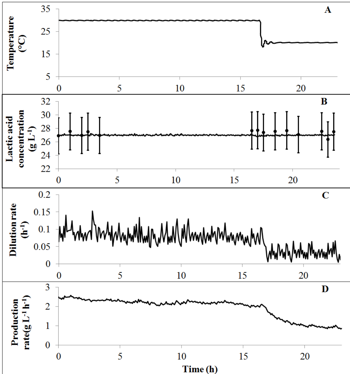
Figure 5.9 Adaptive control law robustness study. A Temperature disturbance. B Lactic acid concentration evolution with time. Pref \mu = 27 \text{ g L}^{-1} (.....), lactic acid concentration available online (—) and lactic acid offline measurement ( \bullet ). C Dilution rate evolution with time. D Estimated production rate.
