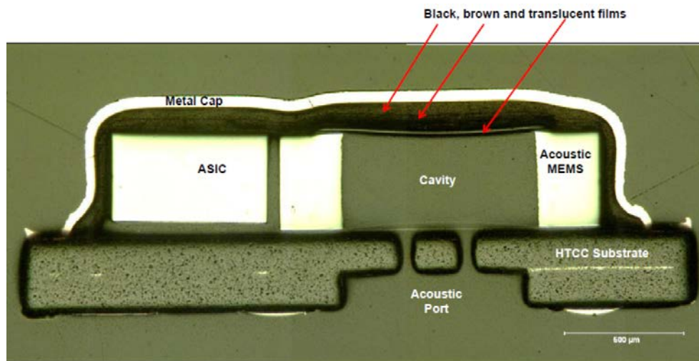
Figure 5.13: Cross-section of Epcos T4000 package [81].
