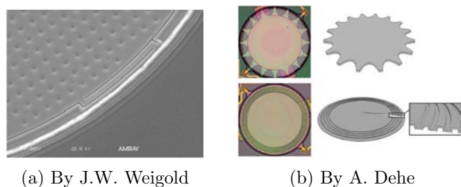
Figure 1.13: Different types of spring-suspended membranes.
