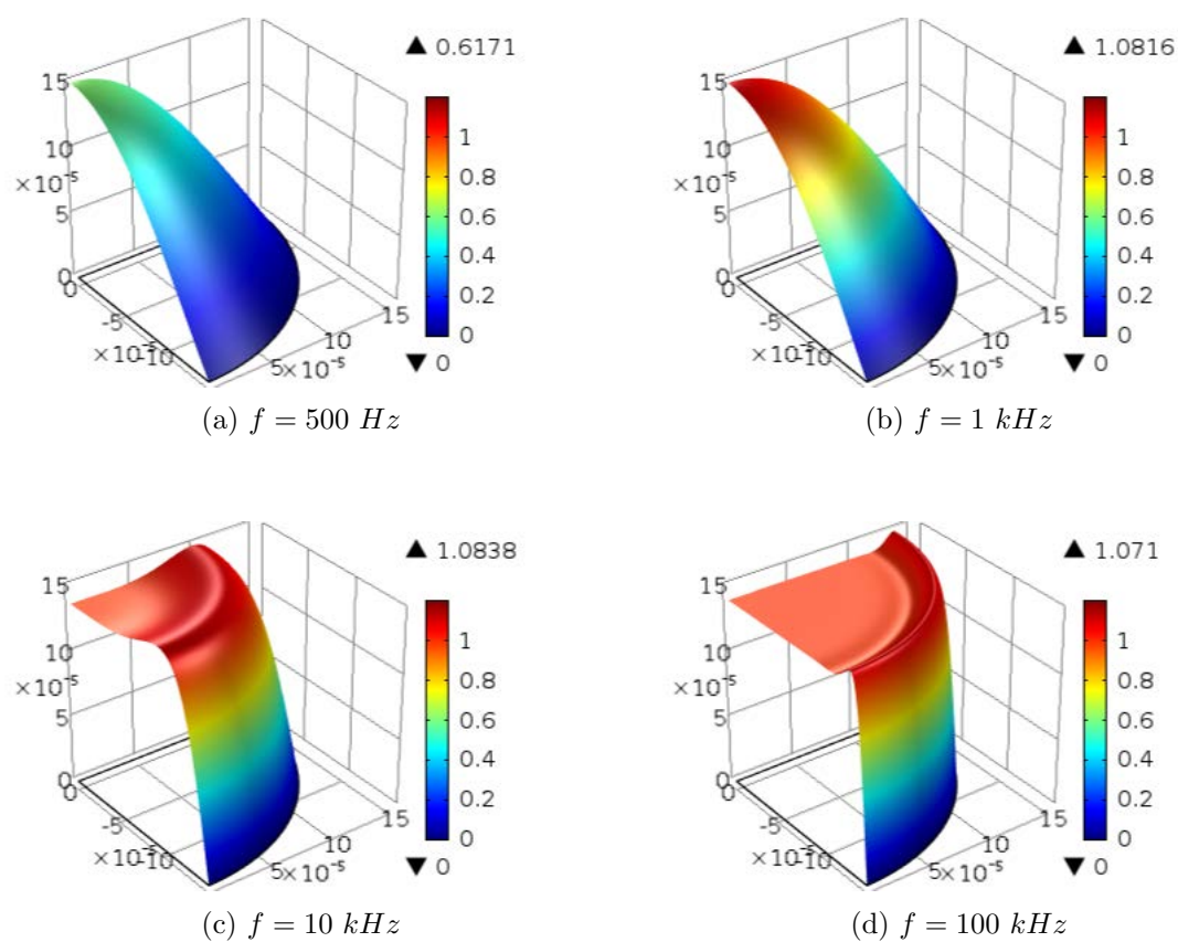
Figure 3.6: Evolution of the velocity shape function for circular vent with radius of 150 \mu\text{m}
