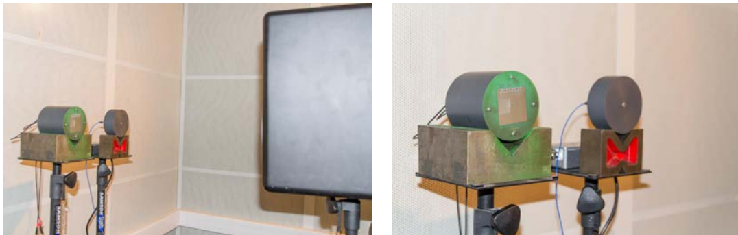
Figure 6.13: Experimental setup used in free-field investigations.
