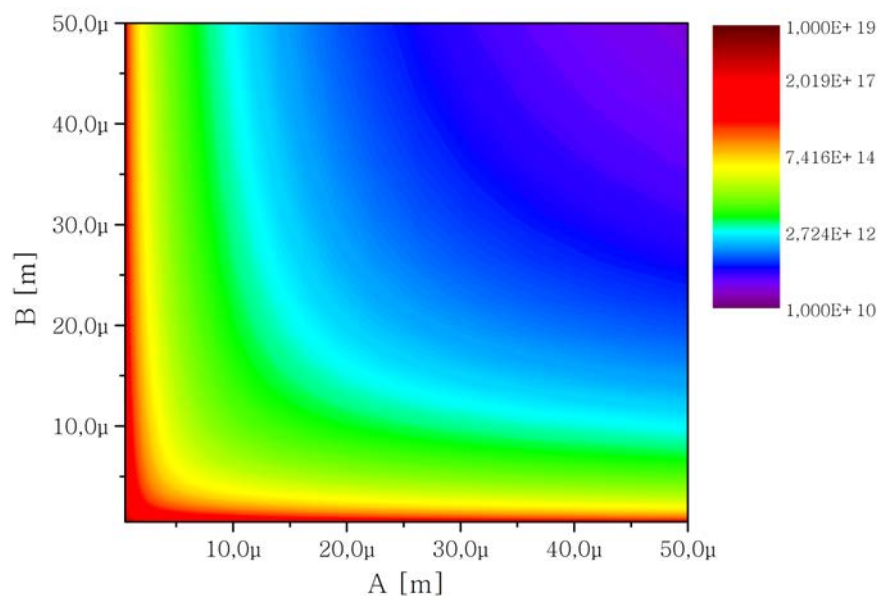
Figure 3.18: Acoustic resistance of the rectangular guide as a function its side length A and B . Color legend indicates the acoustic resistance with the units [\text{Pa}/(\text{m}^3/\text{s})] . The length L_r is set to 500 \mu\text{m} .
