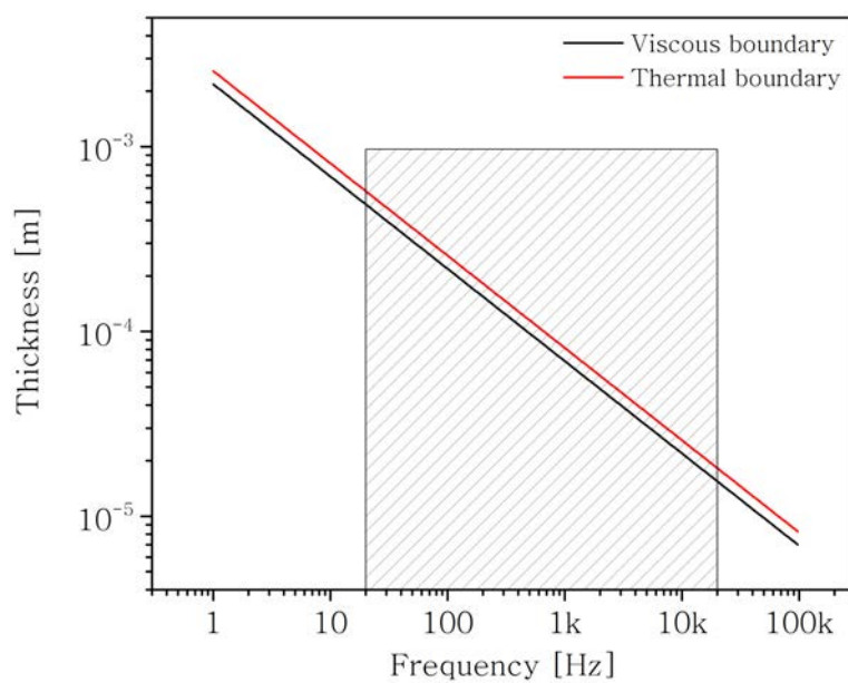
Figure 3.3: Viscous and Thermal boundary layers thicknesses as a function of frequency.
