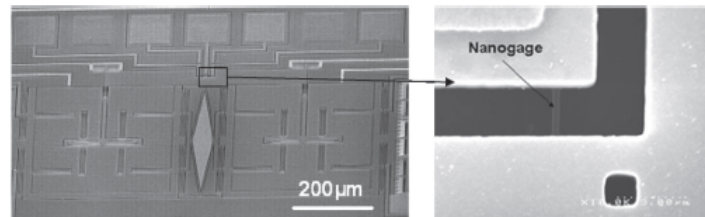
Figure 2.13: SEM image of gyroscope with zoom on nanogauge on the right side [52].
