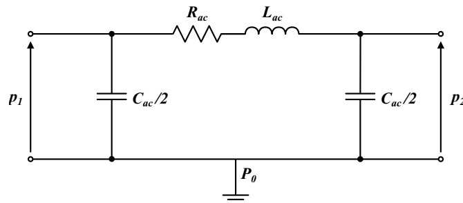
Figure 3.14: Electrical representation of two-port acoustic element.
