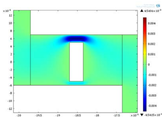
(c) Surface graph of velocity field at 1 kHz.
