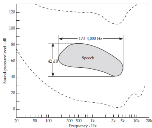
Figure 1.6: Auditory region according to F.A. Everest [12].
