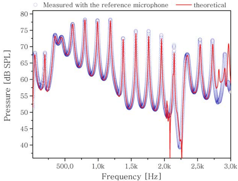
Figure 6.10: Comparison of experimental and identified data for impedance tube setup.
