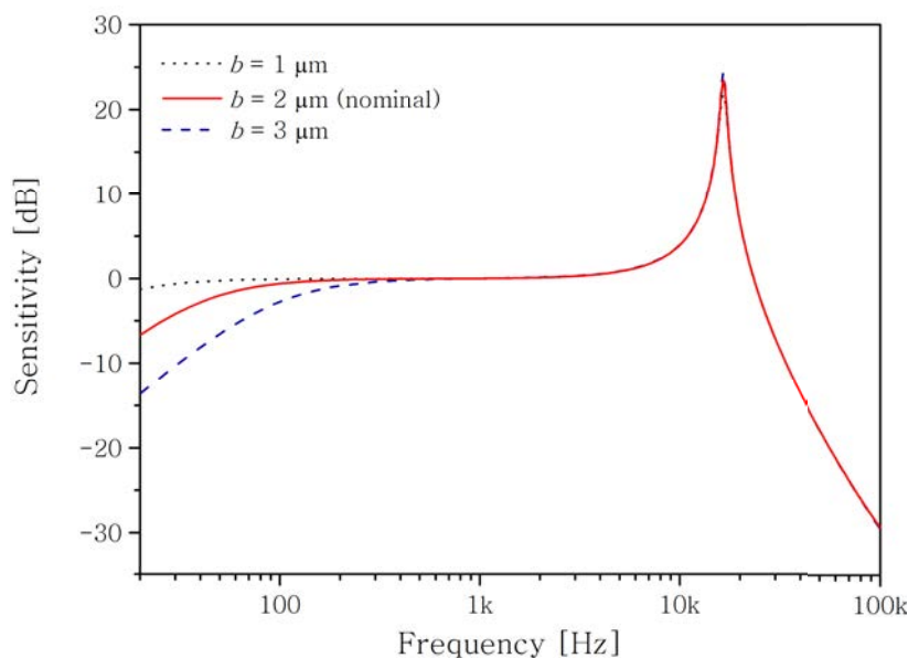
Figure 4.34: Comparison of normalized frequency response S(\omega)/S_0 of the microphone for different b parameters.
