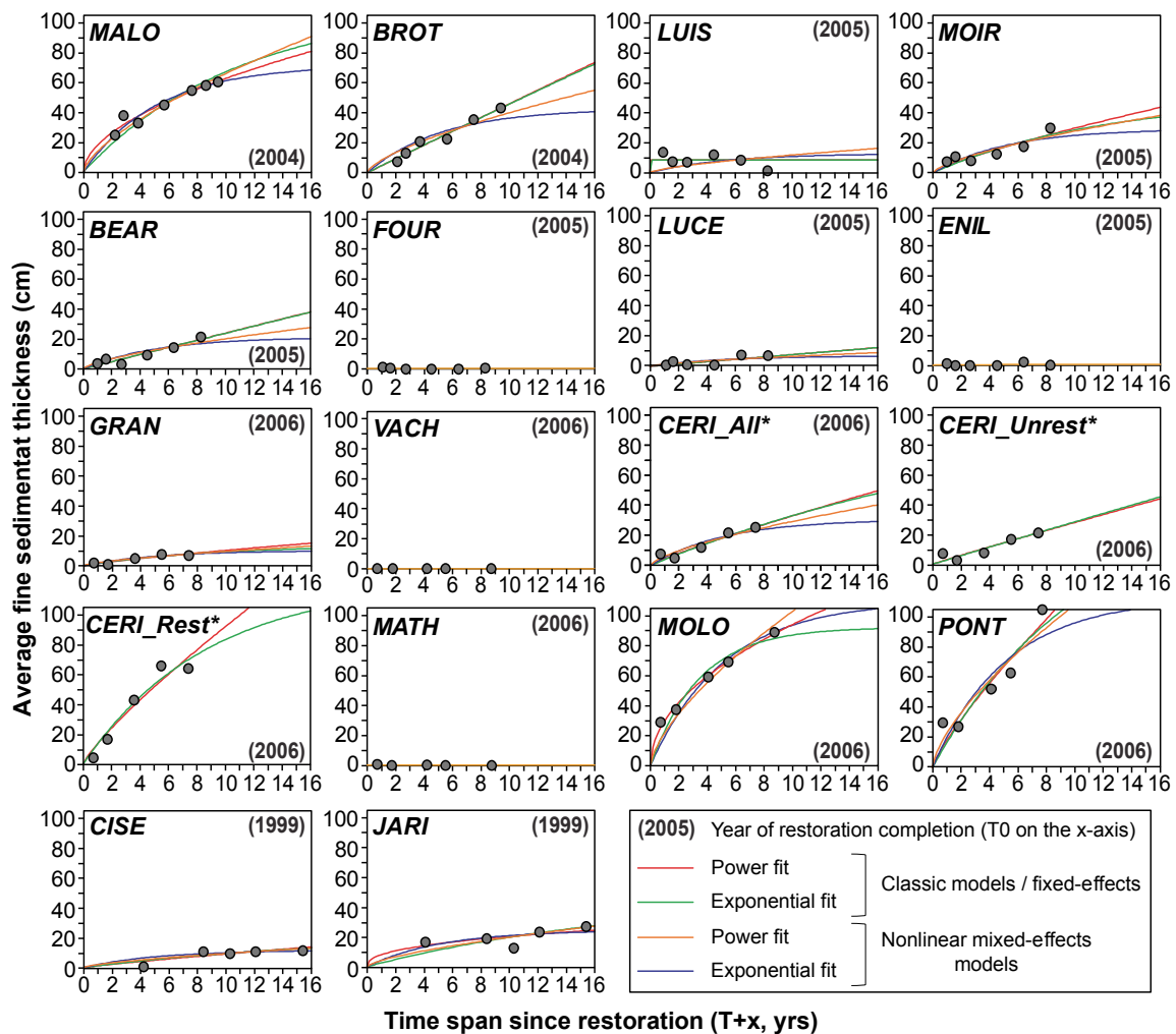
Figure 4.8. Statistical relationships linking the average fine sediment thickness observed in floodplain channels with the time since restoration ( i.e. from T_0 to T+\max ) according to four different models (see §3.3.1 for details). Raw data are available in Tables 4.1 & 4.2.
