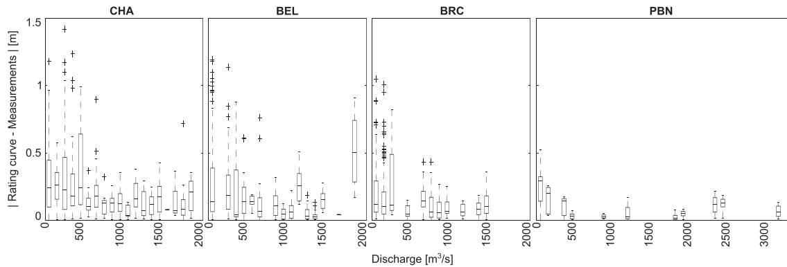
Figure 2. Variability of water levels around the fitted rating curves in the study reaches (from left: CHA, BEL, BRC, and PBN); all rating curves included
