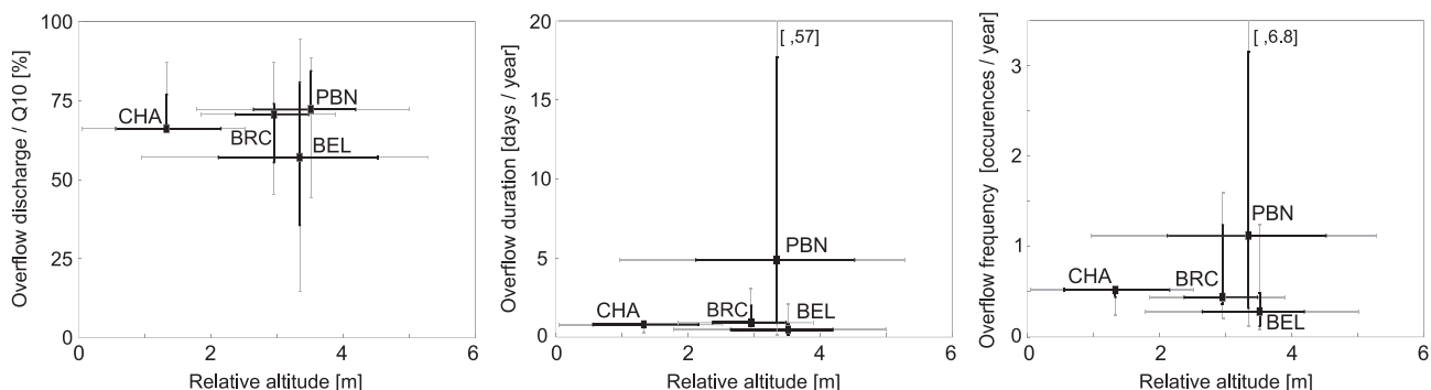
Figure 10. Boxplots linking relative altitude ( x -axis) with: (i) overbank flow discharge rated by Q10; (ii) overflow duration ( y -axis); and (iii) overflow frequency ( y -axis) for floodplain features flooded by the 10-year flood (permanent water bodies excluded) in all study reaches; the 10th, 25th, 50th, 75th and 90th percentiles are displayed. Grey lines refer to interdecile range, black lines to the interquartile range; the median corresponds to the centroid of the ‘double-cross’ displayed. Data were analysed for the period 1986–2010
