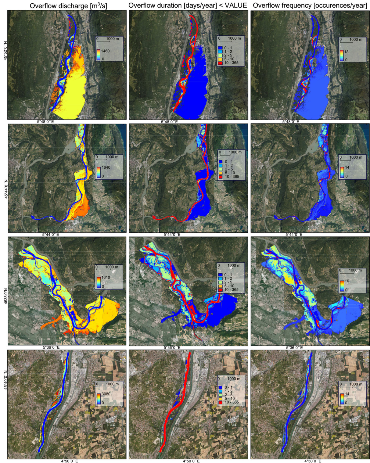
Figure 9. Spatial distribution of overflow discharge, duration, and frequency in study reaches (from above: CHA, BEL, BRC, and PBN). The area of interest corresponds to the 10-year flood extent (permanent water bodies excluded). The overflow frequency and duration are based on data for the period 1986–2010
