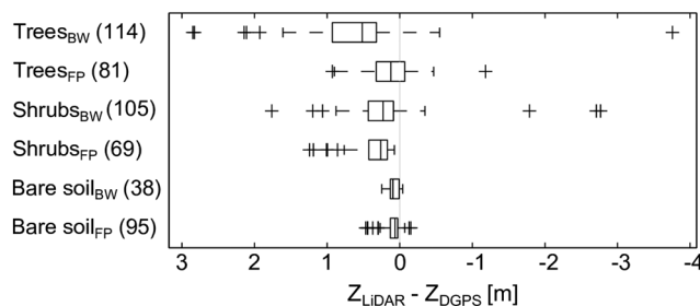
Figure 4. LiDAR accuracy in the floodplain (FP) and in backwaters plugs (BW) according to vegetation cover type, number of measurements marked in brackets
