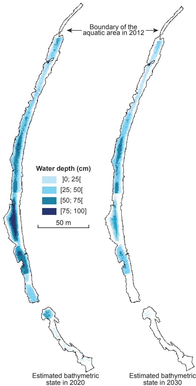
Figure 5.18. Simulated bathymetric states of the backwater in 2020 and 2030 for a discharge in the bypassed main channel of 50 \text{ m}^3 \cdot \text{s}^{-1} . Simulations are derived from the application of sedimentary models for each sub-reach (see Figure 5.11) on the distribution of water depths derived from the bathymetric map of March 2012 (see Figure 5.14).
