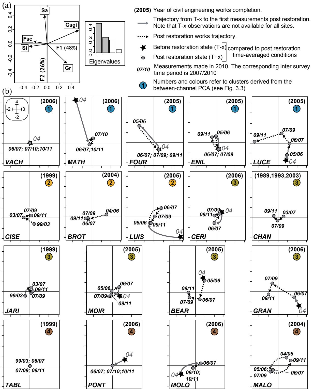
Figure 3.4. Results of the within-channel PCA. (a) Scores of sedimentological variables (proportion of gravel (Gr), sand (Sa) and silt (Si) plots; Fsc: relative length covered by fine sediments; Gsgi: grain size gradient index - a positive value indicates a downstream coarsening) and eigenvalues. (b) Survey scores for individual channels and associated dates. See Table 3.1 for channel codes.
