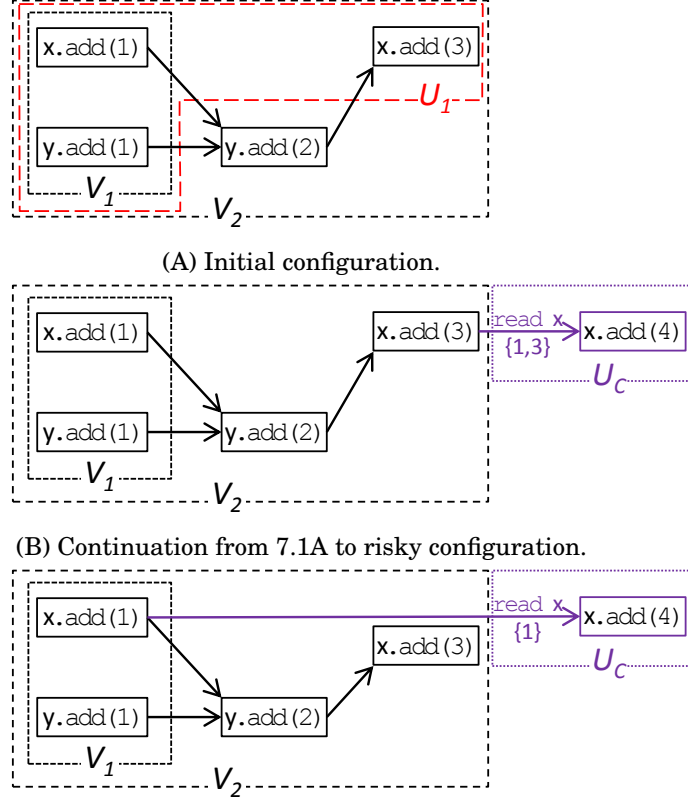
Figure 7.1: Example evolution of configurations for two DCs, and a client. x and y are sets; box = update; arrow = causal dependence (an optional text indicates the source of dependency); dashed box = named database version/state.
