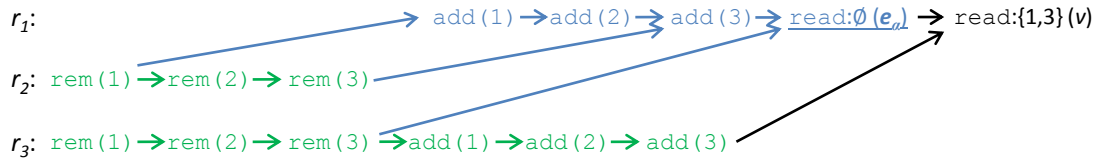
(B) Witness abstract execution \text{abs}(C'_\alpha, \mathcal{V}^{\text{state}}) . Arrows indicate visibility. Arbitration is not shown.
