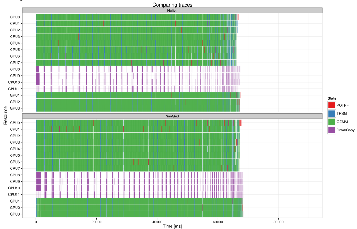
Figure 6.15: Comparing execution traces (native execution on top vs. simulated execution at the bottom) of the Cholesky application with a 72,000 \times 72,000 matrix on the Mirage machine using 8 cores and 3 GPUs as workers. Adding 8 cores, improved the performance by approximately 20% compared to the performances obtained in Figure 6.13.
