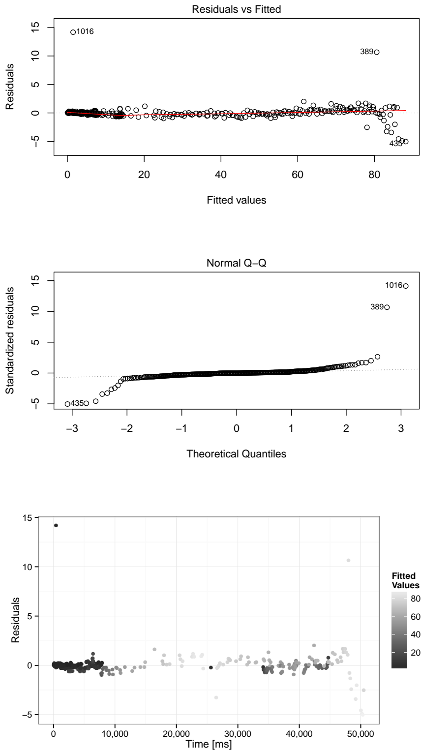
Figure 7.6: Analysing linear model for Panel kernel.
