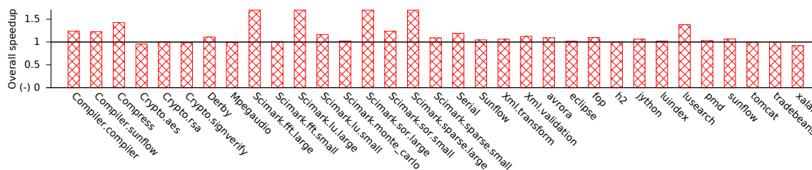
Figure 5.7 – Evaluation of applications with small heap (DaCapo and SPECjvm2008). Higher is better.
