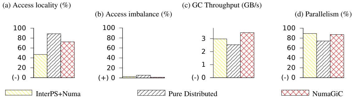
Figure 5.5 – Memory access locality versus parallelism. (-) = higher is better, (+) = lower is better
