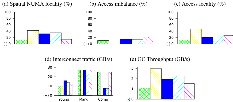
Figure 5.3 – Evaluation of the NUMA-friendly placement policies. (+) = lower is better, (-) = higher is better.
