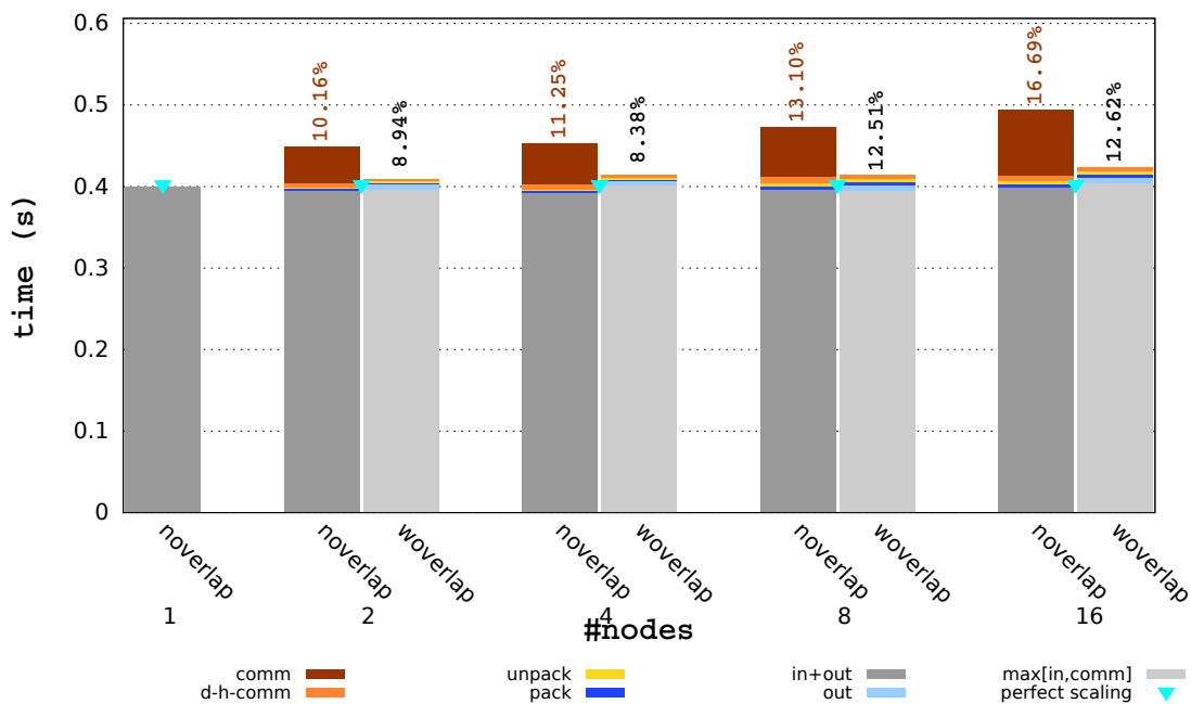
FIGURE 8.21: Performance impact of the communication-computation overlap on the seismic modeling application on the APU cluster , with the cgcc DPS. The weak scaling is considered. The \mathcal{V} dataset is used as input data. Each execution time is the average of 1000 of simulation iterations.
