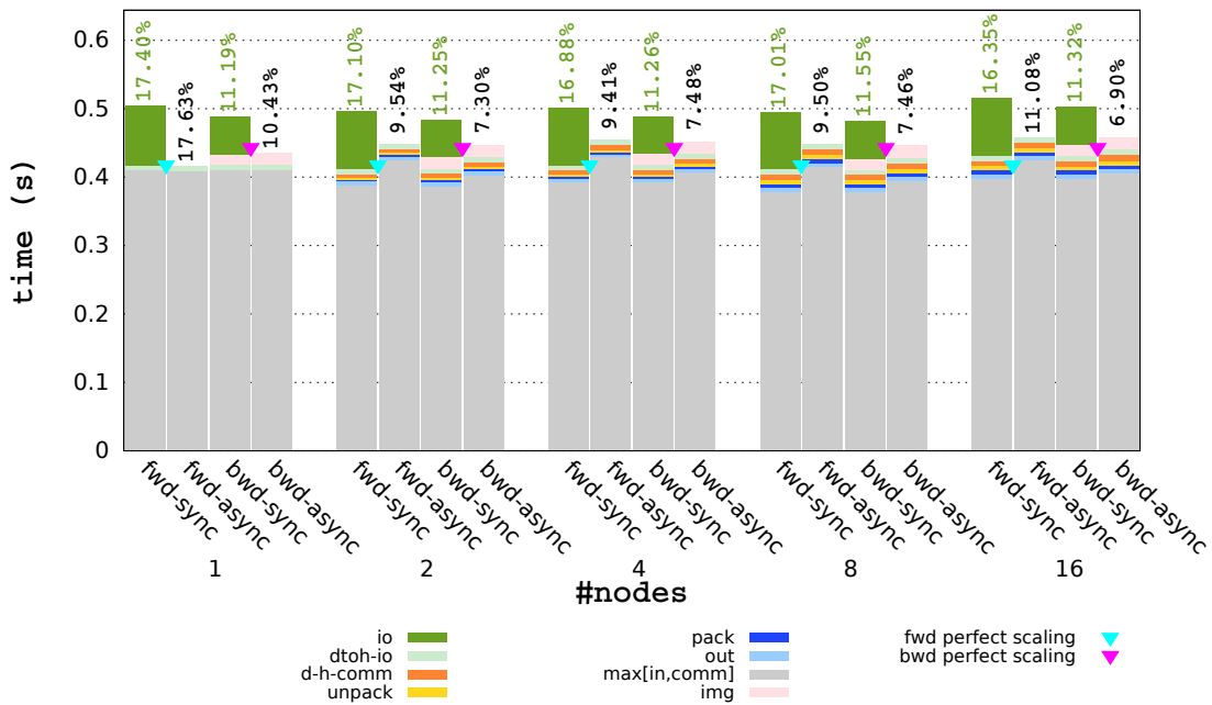
FIGURE 8.31: Performance impact of the asynchronous I/O on the seismic migration application on the APU cluster with the cggc DPS . The weak scaling is considered. The \mathcal{V} dataset is used as input data. Each execution time is the average of 1000 of simulation iterations.
