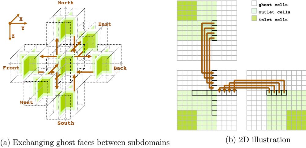
FIGURE 8.5: Exchanging ghost faces with immediate neighboring subdomains: the white cells represent the extra padding added to the compute grid and the light green (resp. the dark green) cells define the grid points whose computation depends on the surrounding subdomains (resp. the cells that can be updated locally). The axes orientation is an arbitrary choice used for the sole purpose to distinguish the MPI neighbors.
