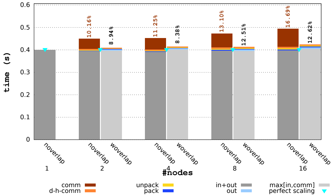
FIGURE 8.21: Performance impact of the communication-computation overlap on the seismic modeling application on the APU cluster , with the cggc DPS . The weak scaling is considered. The \mathcal{V} dataset is used as input data. Each execution time is the average of 1000 of simulation iterations.
