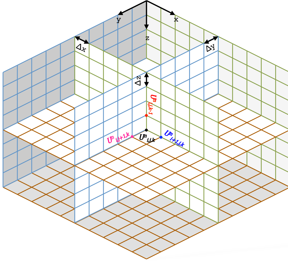
FIGURE 2.15: Space discretization of a 3D volume.
