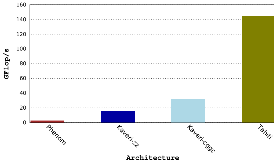
FIGURE 7.2: Comparison between the performance numbers of the seismic modeling OpenCL kernels obtained on the Phenom CPU , on the Kaveri APU and on the Tahiti discrete GPU . On the APU two data placement strategies are considered: cggc and zz .
