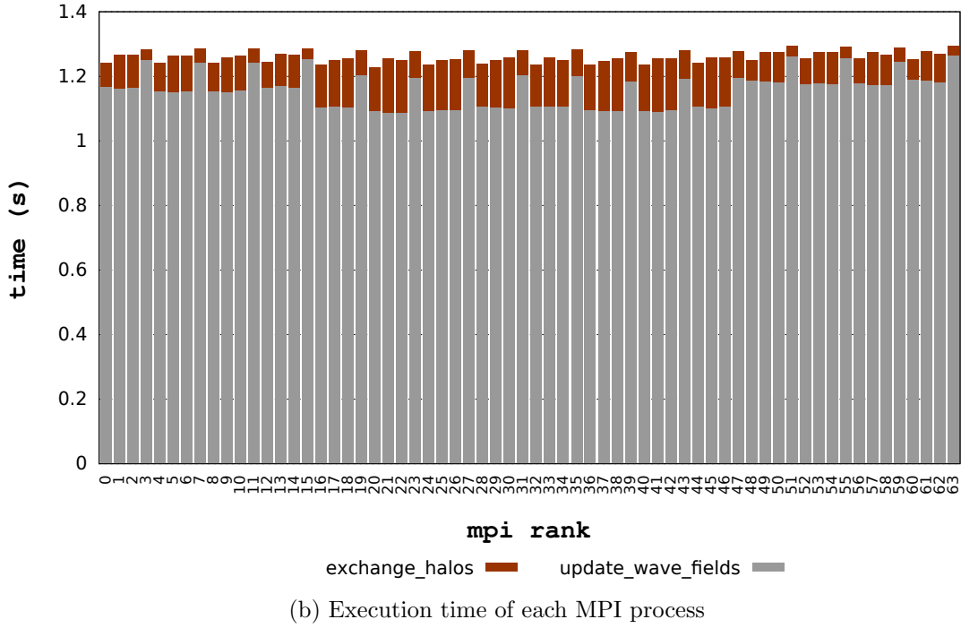
FIGURE 8.7: Demystification of the load imbalance due to the PML boundary condition, example on a 4x4x4 domain decomposition.
