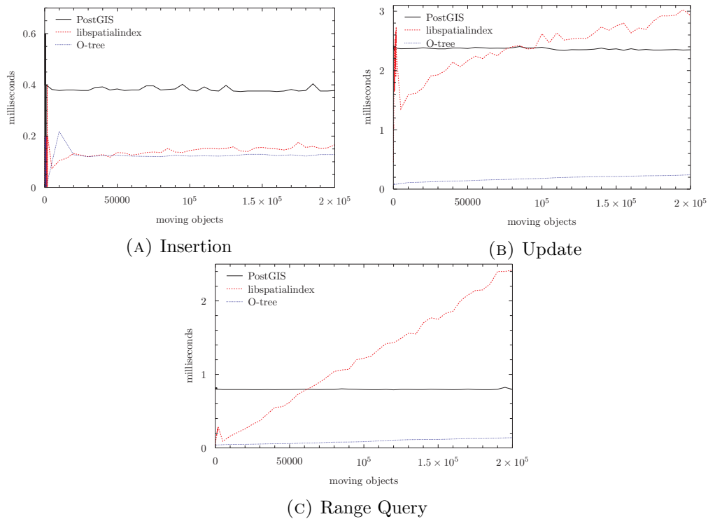
FIGURE 3.2: Performance for R-tree implementations
