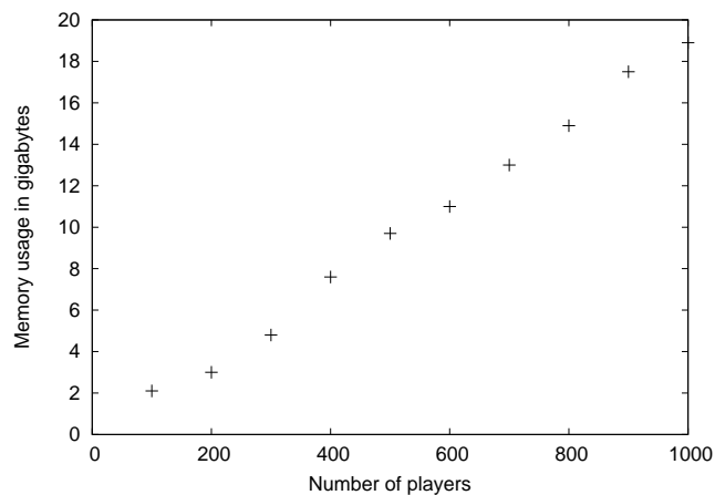
FIGURE 6.4: Memory usage
