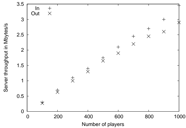
FIGURE 6.3: Throughput
