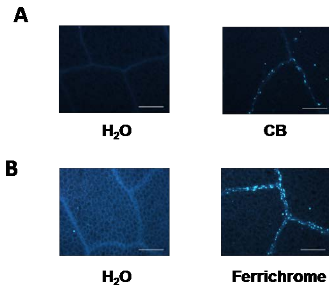
Figure S5: Chrysoabactin and ferrichrome trigger callose deposition. Leaves of hydroponically-grown Col-0 plants were infiltrated with 1 mM CB (A) or 1mM ferrichrome (B). Representative pictures of callose depositions detected with aniline blue staining in leaves 8 h after the indicated treatments are shown. Bar = 200 \mu m.
