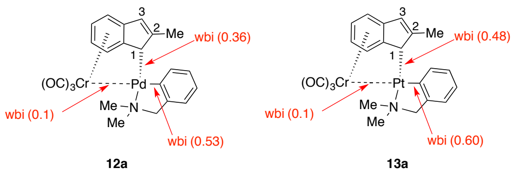
Figure 140: Inspection of the Wiberg bond indices for 12a and 13a .
