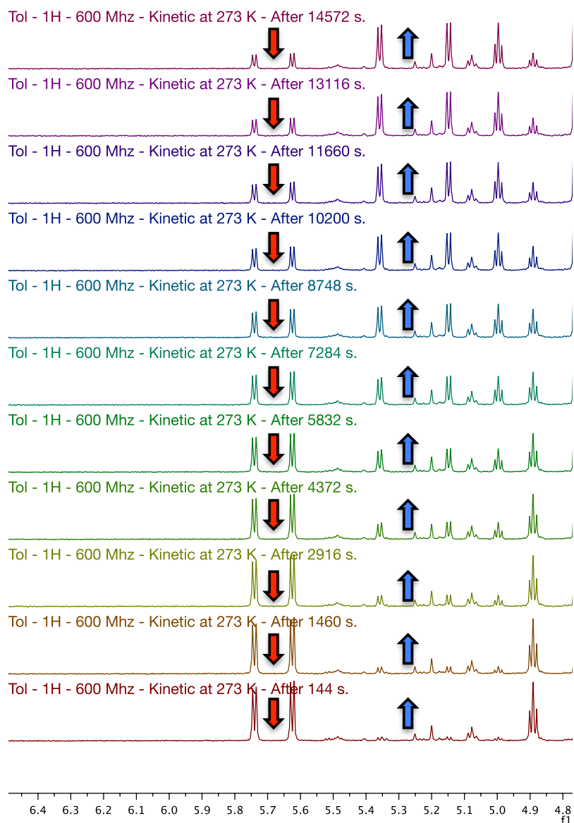
Figure 171: ^1\text{H} -NMR spectra in toluene at 273 K, showing the progressive disappearance of the signals associated to bimetallic 16a (red arrows) and the apparition of the signal of 17a (blue arrows).
