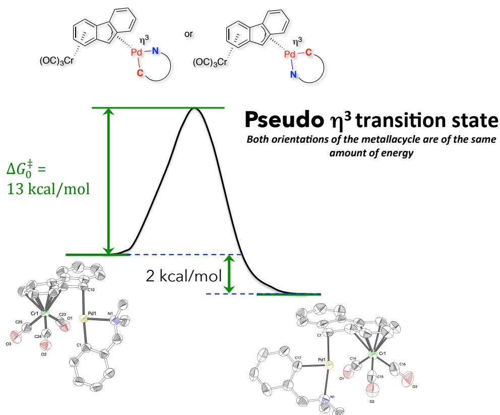
Figure 170: Illustration of the isomerization mechanism of 16a into 17a .
