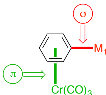
Figure 75: \sigma - \pi -bridged heterobimetallic complex.
