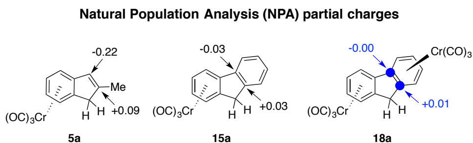
Figure 211: Natural partial charges (NPA) at C 2 and C 3 positions in 5a , 15a and 18a computed from gas phase singlet ground state geometries optimized at the ZORA-TPSS-D3(BJ)/all electron TZP level.
