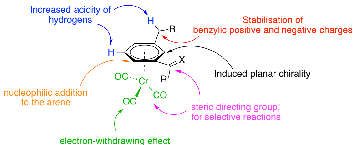
Figure 71: Summary of the main properties induced by the coordination of a Cr(CO) 3 unit to an arene ligand.
