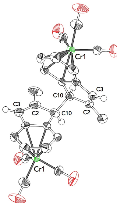
Compound 8d Space Group: C 2/c R-Factor (%): 4.62
