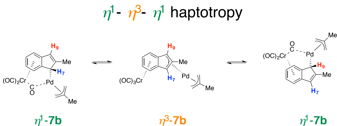
Figure 95: Supposed fluxional behavior of the Pd centre.
