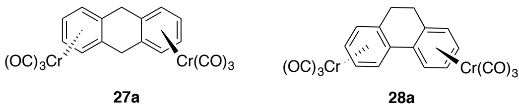
Figure 198: Other heteroditopic ligands tested in order to synthesize another tetrametallic complex.
