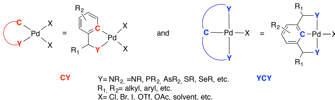
Figure 107: Structural definition of the palladacycles.
