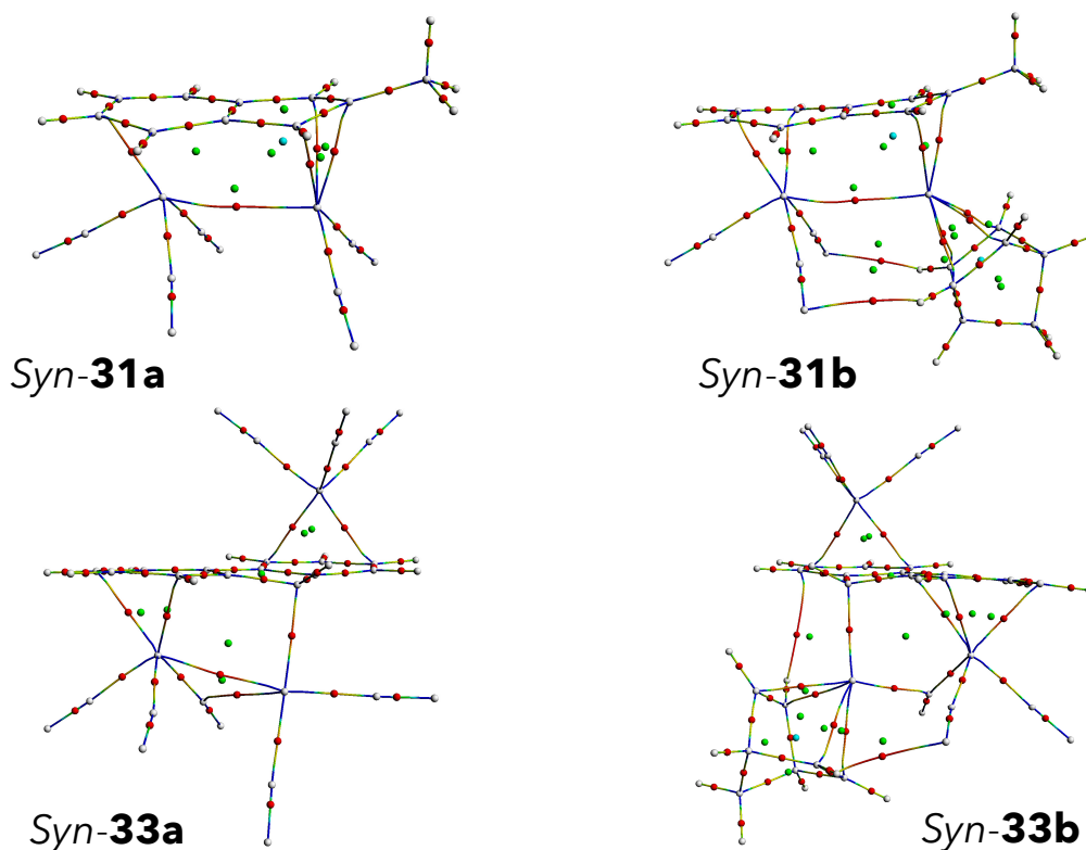
Figure 217: Atom-in-molecules analysis of the electron density topology for syn-31a , syn-31b , syn-33a and syn-33b . Red and green dots are associated to Bond (BCP) and Ring (RCP) Critical Points respectively. Grey spheres materialize the atomic critical points scaled by the associated density.
