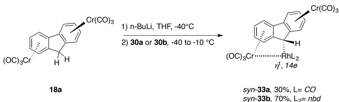
Figure 212: Formation of hemichelates syn - 33a and syn - 33b by sequential deprotonation and metalation of the benzylic position of 18a .
