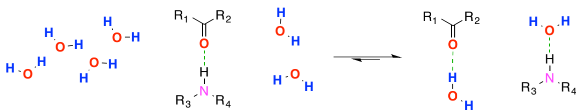
Figure 21: Competition of water molecules with other polar molecules in the establishment of non-covalent interactions.
