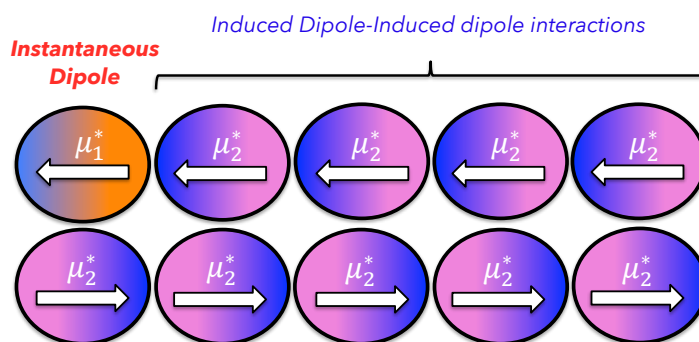
Figure 12: An instantaneous dipole on one molecule induces a dipole on another molecule, and then both dipoles interact to lower the energy.
