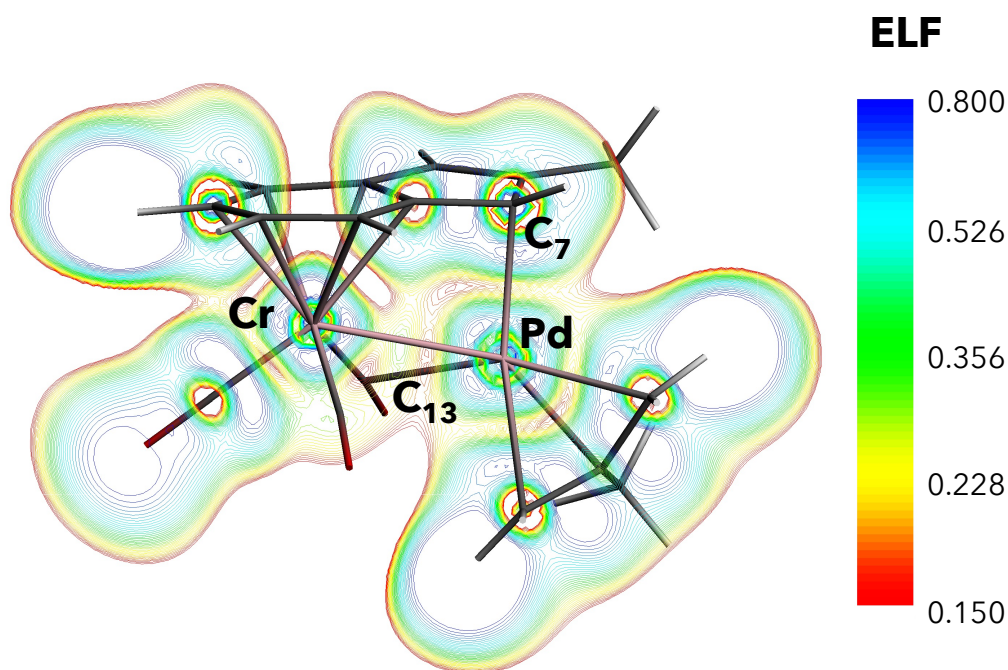
Figure 89: Contour plot of the ELF in 7b from a (ZORA) PBE0 (-dDsC)/all-electron-TZP gas phase minimum in the plane defined by Cr, Pd, and C 7 .
