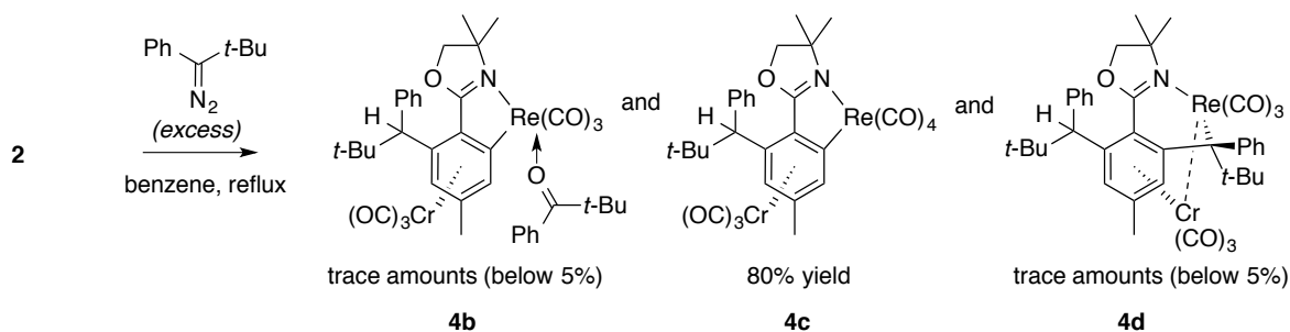
Figure 59: Reaction of 2 with (t\text{-Bu})(\text{Ph})\text{CN}_2 .
