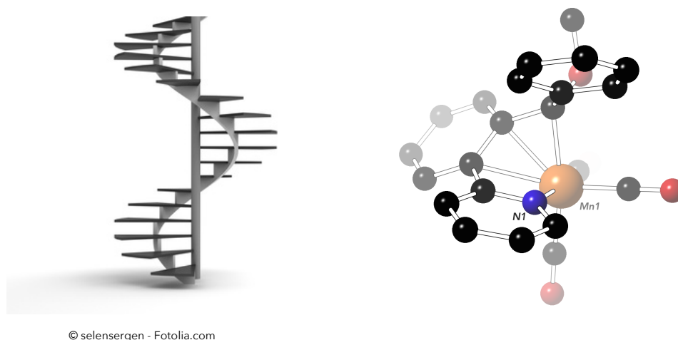
Figure 39: The geometrical analogy between a “spiralene” (right) and a “spiral staircase” (left). The manganese (I) centre sustains the helical molecular arrangement in a fashion similar to that of a pillar (in light grey) in a spiral staircase.
