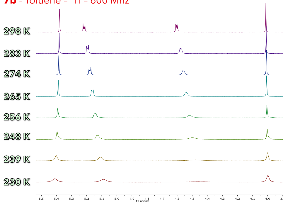
Figure 94: ^1\text{H} NMR variable temperature displaying the signal broadening upon decreasing the temperature.
