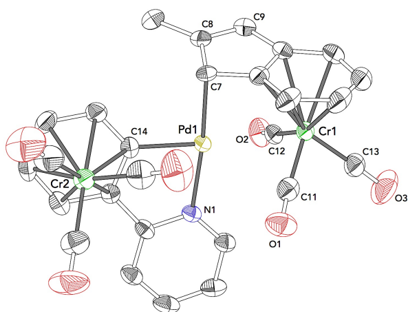
Compound 12g Space Group: Pbca R-Factor (%): 4.71
