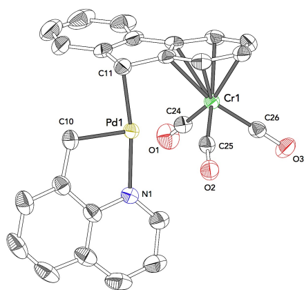
Compound 17j Space Group: Pbca R-Factor (%): 2.47
