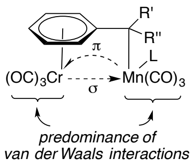
Figure 49: Lewis-type structure displaying the bonding interaction between the two metal centres.
