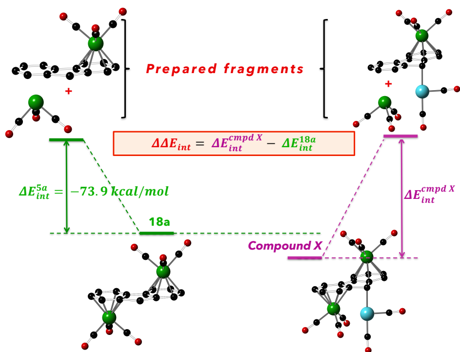
Figure 221: Considered fragments for the energy decomposition analysis.
