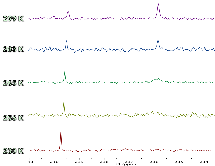
Figure 92: ^{13}\text{C} NMR variable temperature experiment displaying the evolution of the carbonyl signals of the \text{Cr}(\text{CO})_3 moiety.
