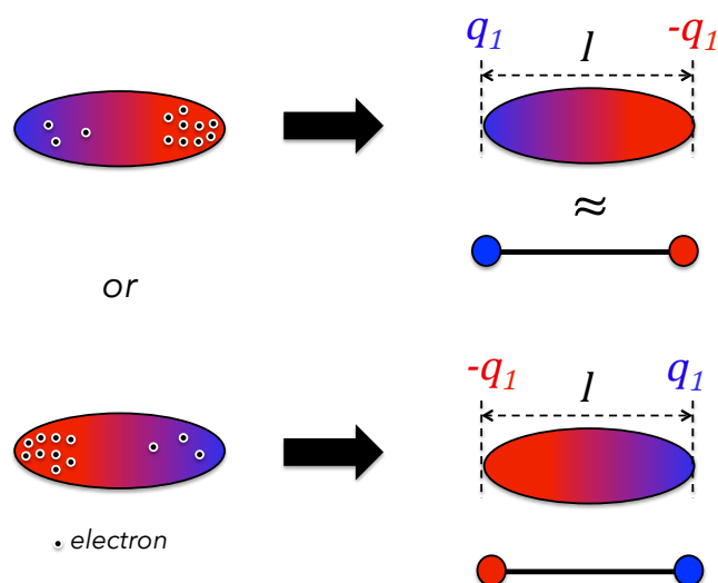
Figure 6: Illustration of the formation of dipoles through the movement of group of electrons.
