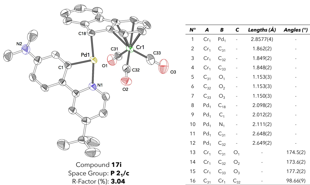
Figure 179: X-ray structure and selected interatomic distances of compound 17i .
