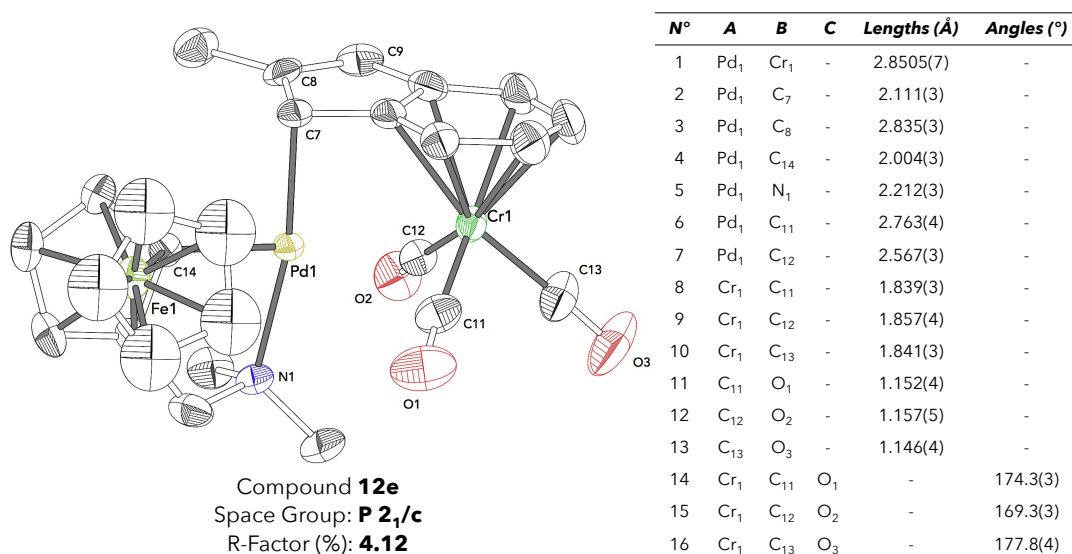
Figure 124: X-ray structure and selected interatomic distances of compound 12e .
