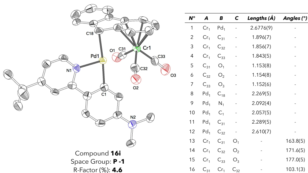
Figure 168: X-ray structure and selected interatomic distances of compound 16i .
