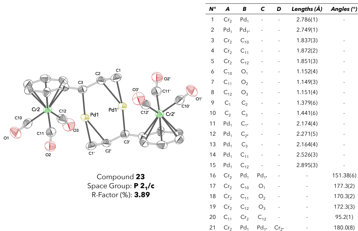
Figure 194: X-ray structure and selected interatomic distances of compound 23 .
