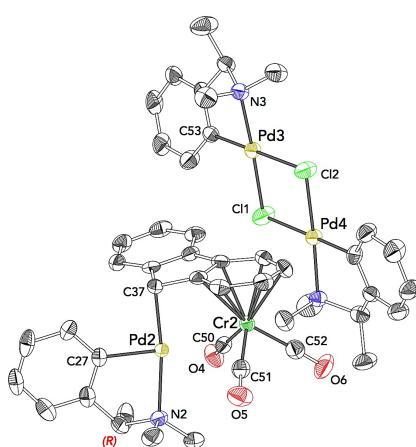
Compound (1R)- 17c Space Group: P 1 R-Factor (%): 3.07
