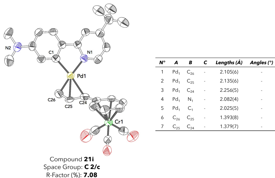
Figure 189: X-ray structure and selected interatomic distances of compound 21i .
