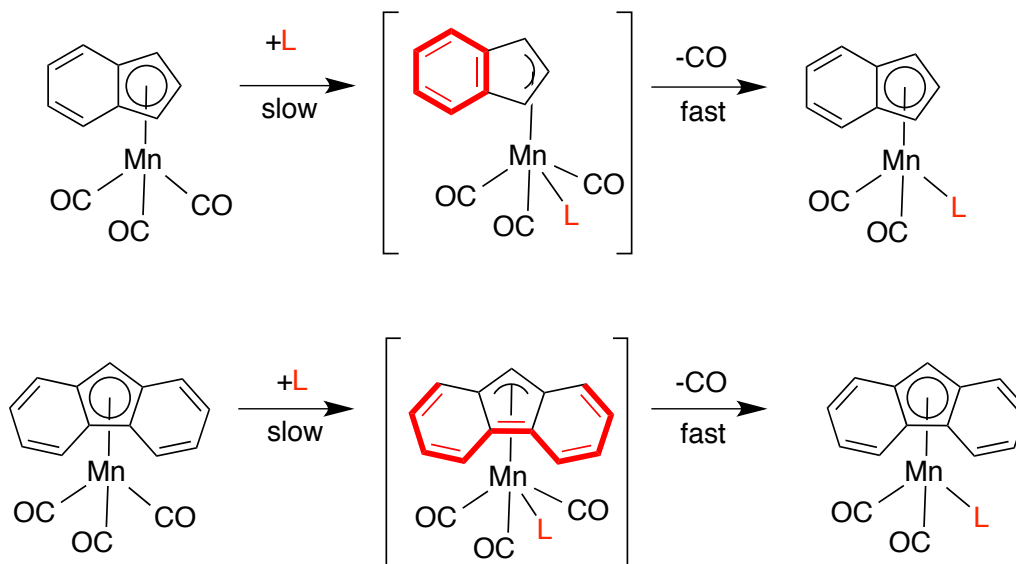
Figure 65: Substitution reactions on indenyl and fluorenyl Mn carbonyl complexes.
