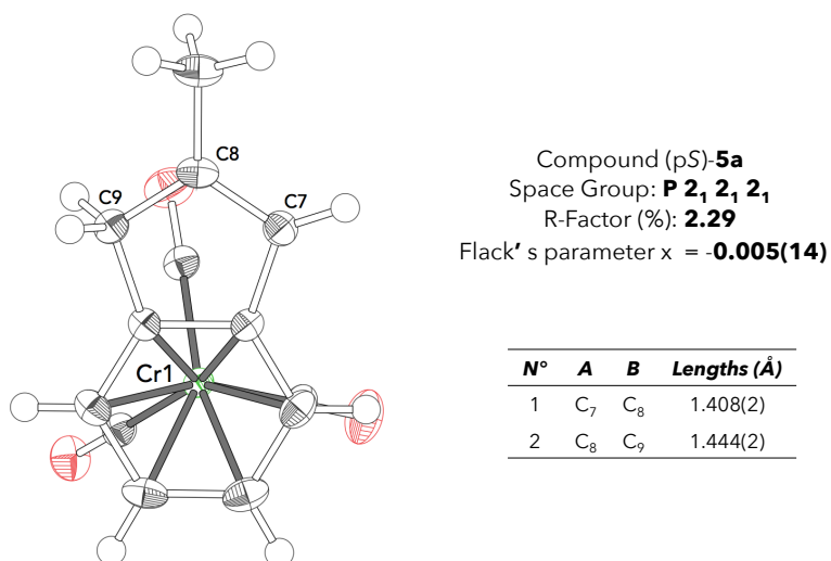
Figure 154: X-ray structure and selected interatomic distances of compound (pS)- 5a .
