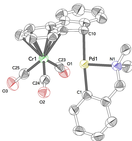
Compound 16a Space Group: C 2/c R-Factor (%): 4.66
