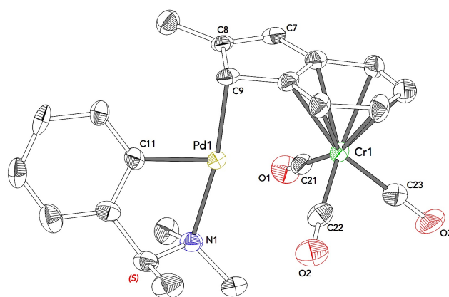
Compound (1S)- 12c Space Group: P 2 1 R-Factor (%): 4.04 Flack' s parameter x = 0.02(3)
