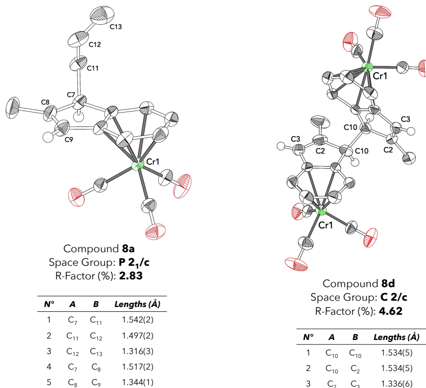
Figure 103: X-ray structure and selected interatomic distances of compounds 8a and 8d .
