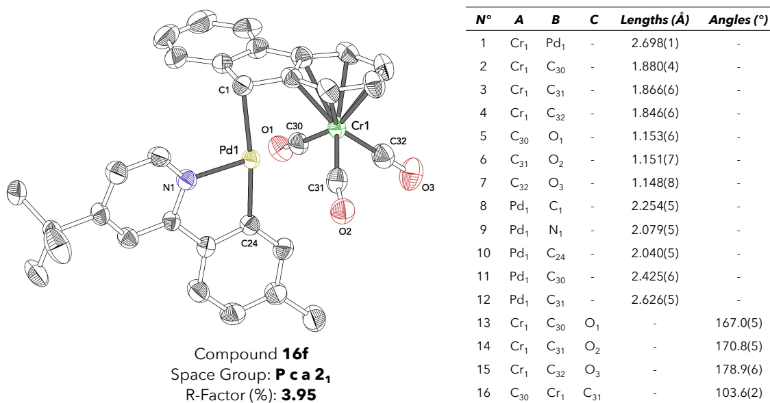
Figure 167: X-ray structure and selected interatomic distances of compound 16f .
