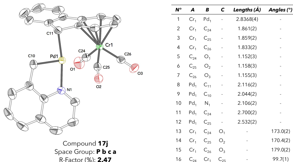
Figure 180: X-ray structure and selected interatomic distances of compound 17j .
