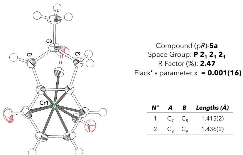
Figure 153: X-ray structure and selected interatomic distances of compound (pR)- 5a .
