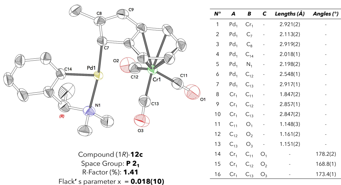
Figure 121: X-ray structure and selected interatomic distances of compound (1- R )- 12c .
