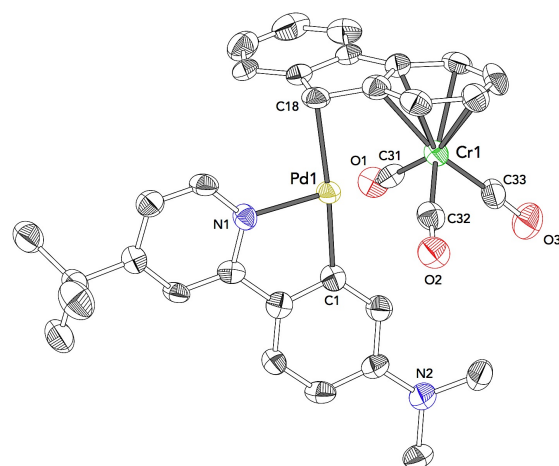
Compound 16i Space Group: P-1 R-Factor (%): 4.6
