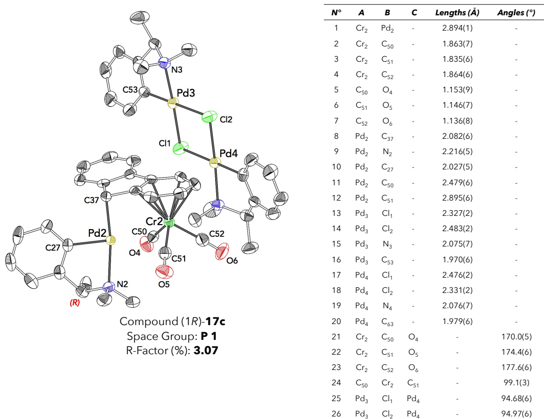
Figure 177: X-ray structure and selected interatomic distances of compound (1R)-17c .
