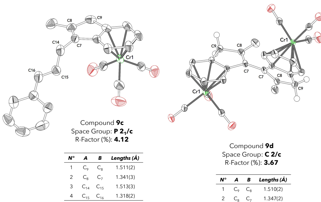
Figure 106: X-ray structure and selected interatomic distances of compounds 9c and 9d .
