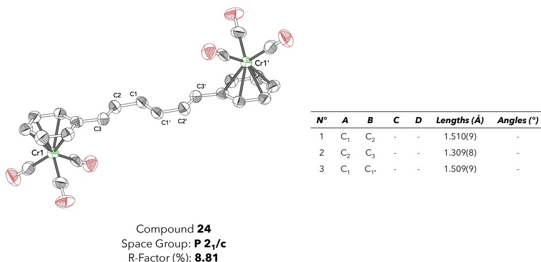
Figure 195: X-ray structure and selected interatomic distances of compound 24 .
