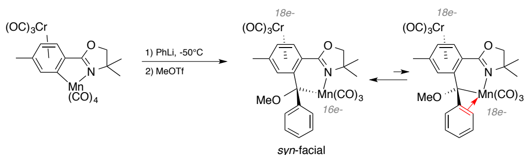
Figure 46: Formation of a mixture of two “pseudoconformers”. A syn -facial unsaturated 18-16 electrons isomer and a saturated 18-18 electrons isomer.
