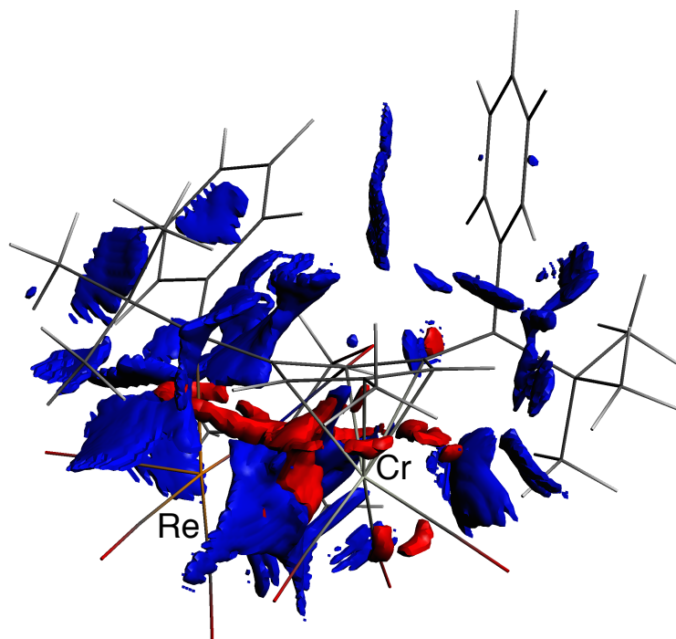
Figure 227: ADFview 2013 plot of NCI regions materialized by reduced density gradient isosurfaces (cutoff value s= 0.02 au, \rho= 0.05 ) coloured according to the signed density \lambda_2\rho (red and blue colours are assigned to negative and positive signs respectively) for the gas-phase singlet ground state geometry of 4d computed at the ZORA-PBE-D3(BJ)/all electron TZP level).
