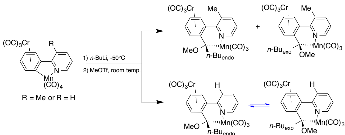
Figure 44: Formation of two isomeric spiralenes with a possible interconversion in the case of the more structurally flexible phenylpyridines.
