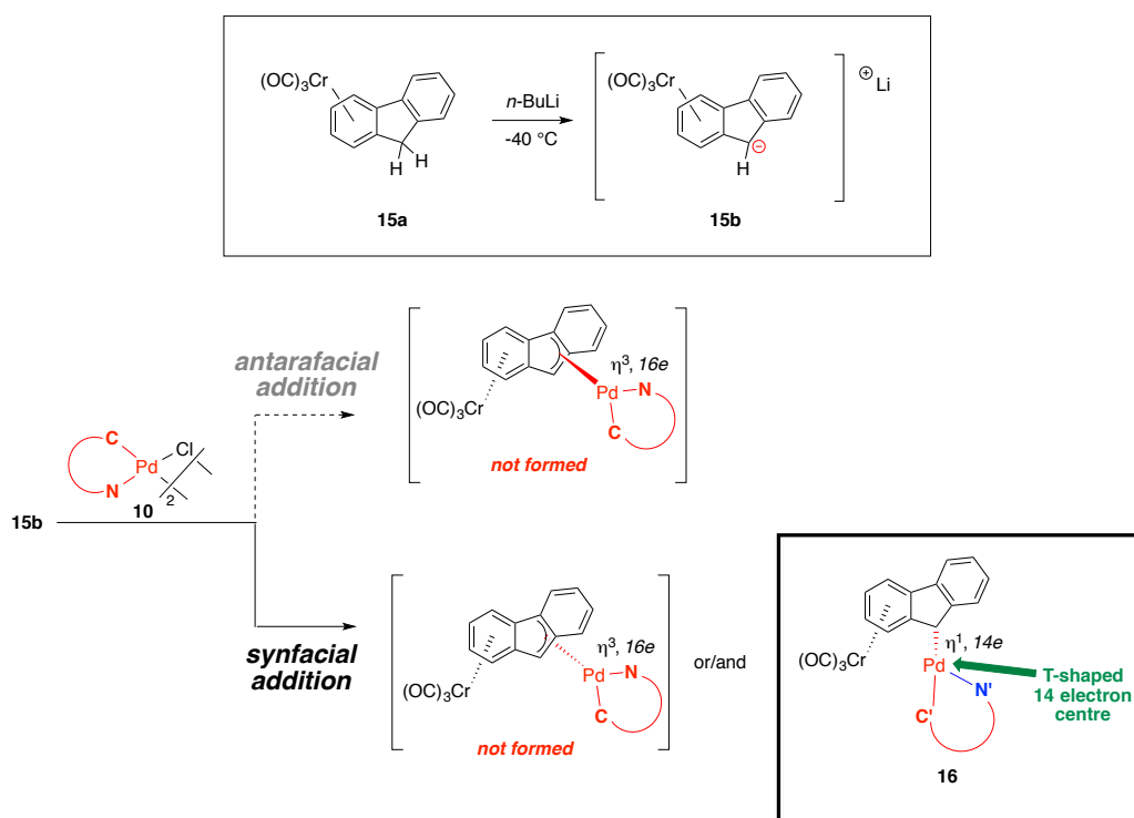
Figure 165: The ambiphilic character of anion 15b allows only one facial interaction with Pd metallacycles 10 , that is the syn -facial, leading exclusively to (\eta^1\text{-fluorenyl})\text{M} complexes, a new class of electron-unsaturated T-shaped \eta^1 -fluorenyl Pd complexes.
