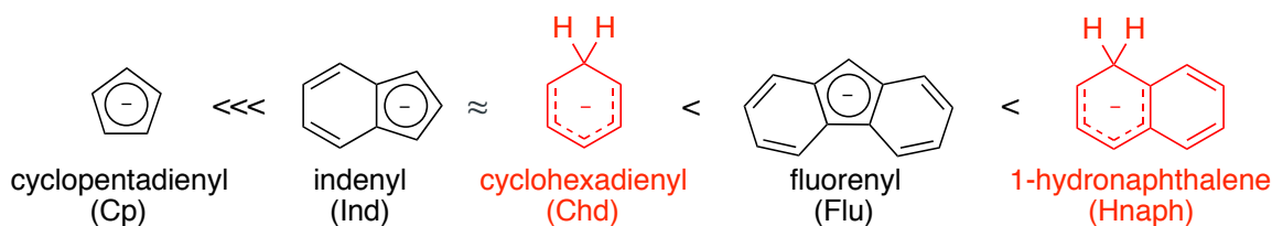
Figure 66: Ligand dependency of the reaction rates.
