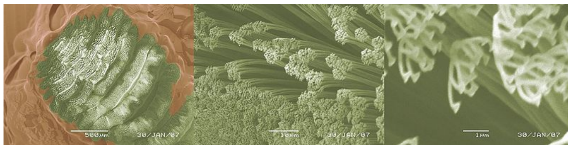
Figure 24: The foot of a Gecko, photograph taken by a scanning electron microscope - author: Oskar Gellerbrant; Public domain via Wikimedia Commons.
