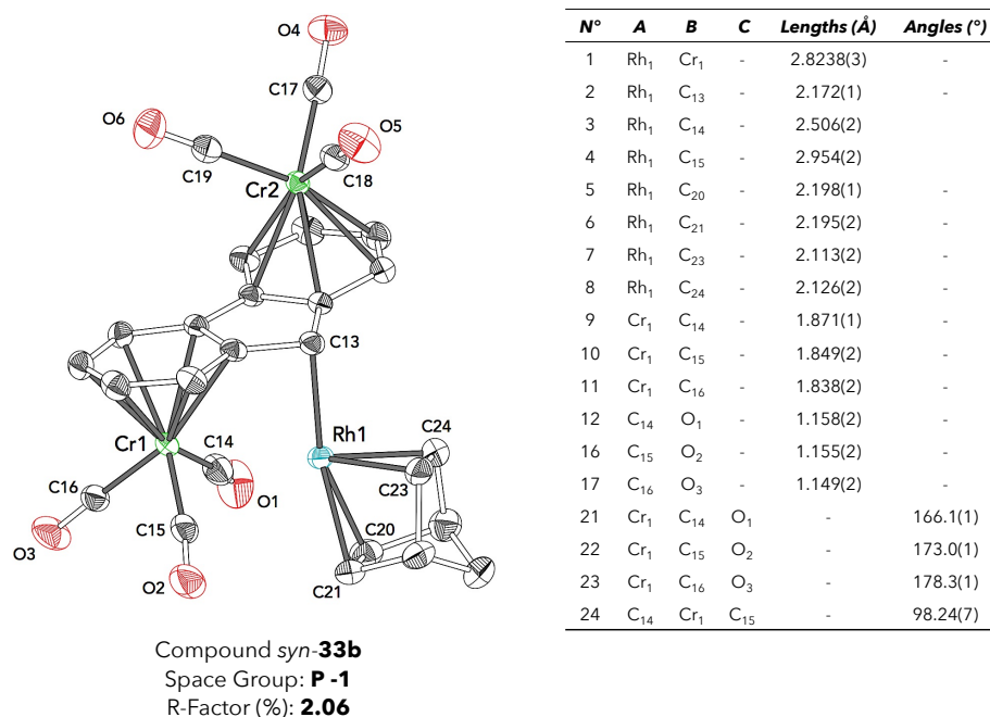
Figure 215: X-ray structure and selected interatomic distances of compound syn-33b .
