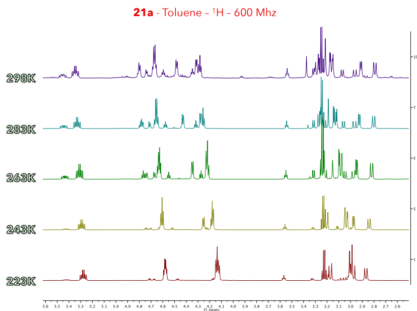
Figure 190: ^1\text{H} NMR variable temperature investigations at subambient temperatures revealing the simplification of the ^1\text{H} signals leading to the expected spectrum of 21a .
