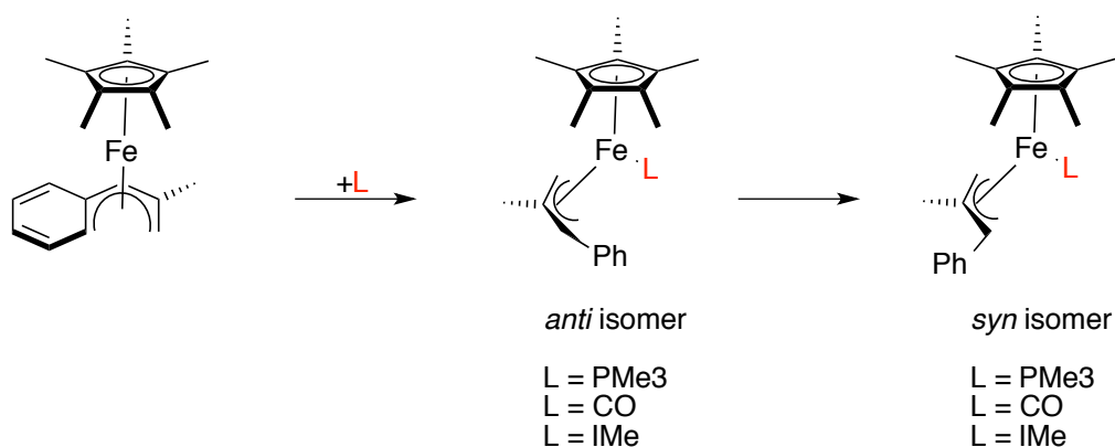
Figure 69: Hapticity switch of open indenyl ligand upon addition of a ligand L.
