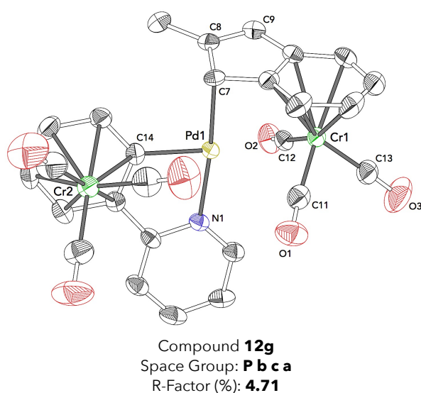
Figure 125: X-ray structure and selected interatomic distances of compound 12g .
