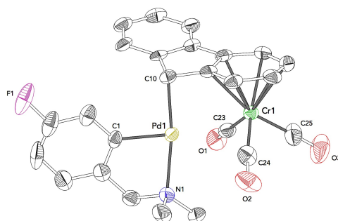
Compound 17b Space Group: P 2 1 /c R-Factor (%): 3.91
