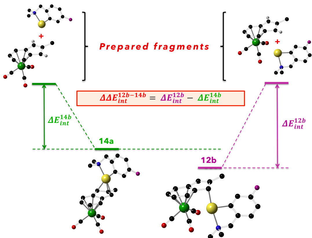
Figure 150: Considered fragments for the energy decomposition analysis.
