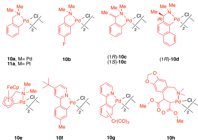
Figure 116: \mu -chloro-bridged palladacycles which were probed for their reactivity toward anion 5b .
