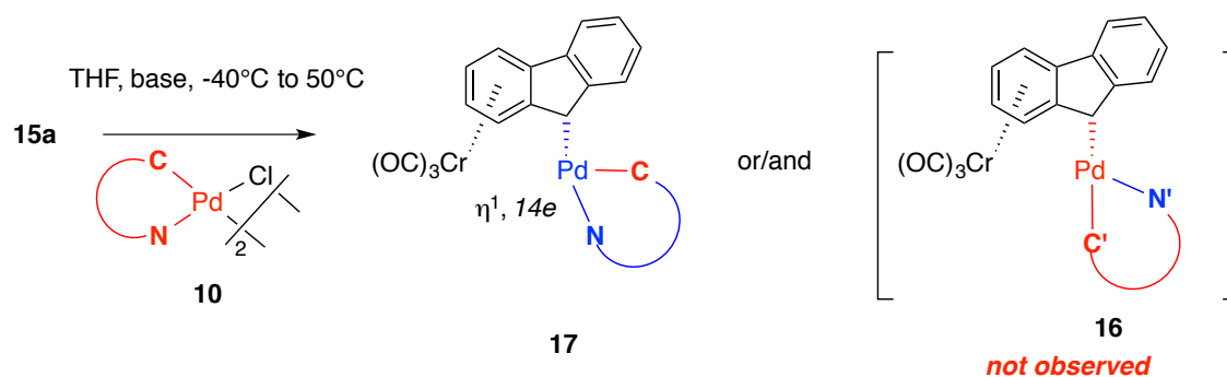
Figure 174: New experimental conditions used for the synthesis of compounds 17c , 17j .
