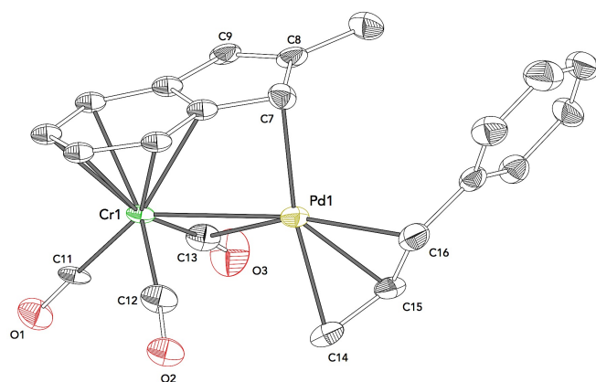
Compound 7c Space Group: P 2 1 /c R-Factor (%): 8.2
