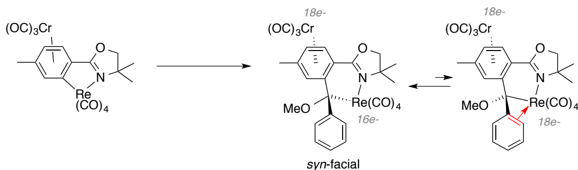
Figure 50: Expected formation of two “pseudoconformers”. A syn -facial electron-unsaturated 18-16 electrons isomer and an electron-saturated 18-18 electrons isomer.
