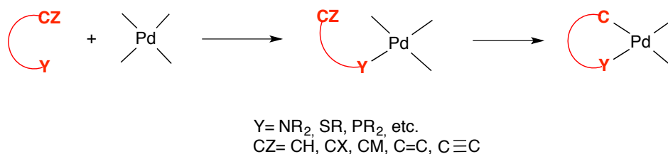
Figure 110: Methods for the generation of palladacycles.
