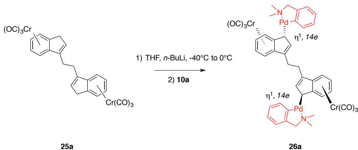
Figure 196: The ambiphilic character of the anion associated to 25a leads, upon reaction, to the formation of a new palladium hemicheate.
