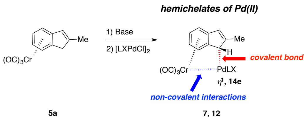
Figure 201: Formation of hemichelates of group 10 transition metals.
