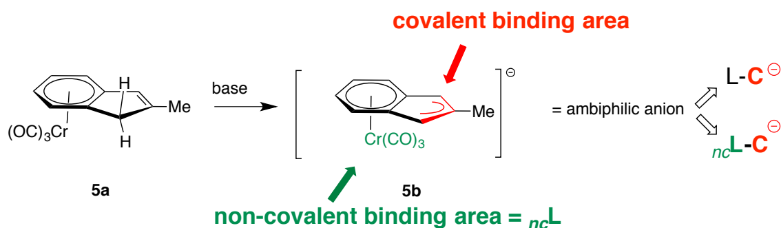
Figure 228: Ambiphilic character of anion 5b .
