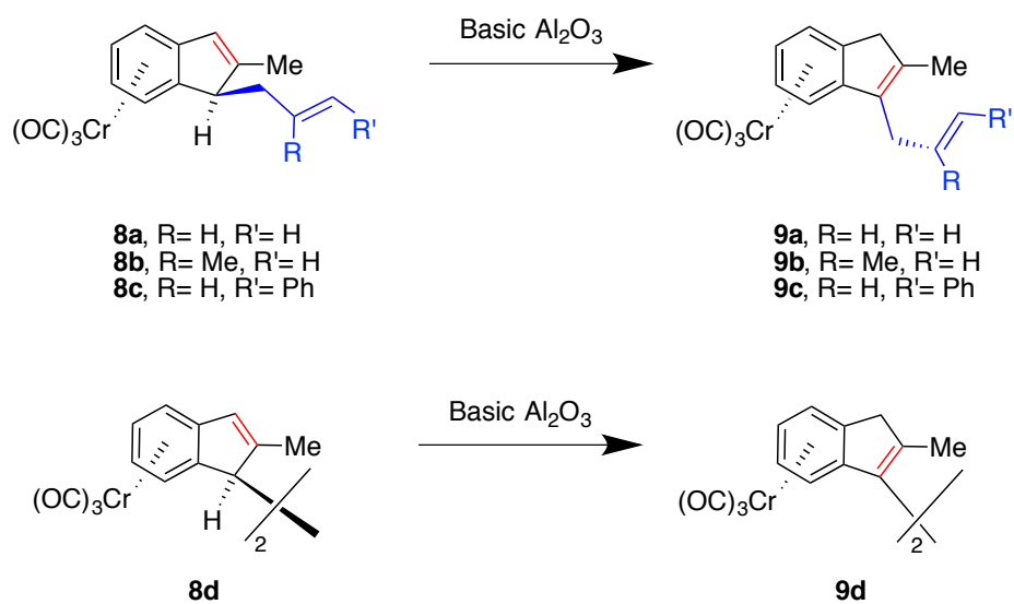
Figure 104: Basic activated alumina promotes the isomerization of 8a-d into the thermodynamically favoured isomers 9a-d .
