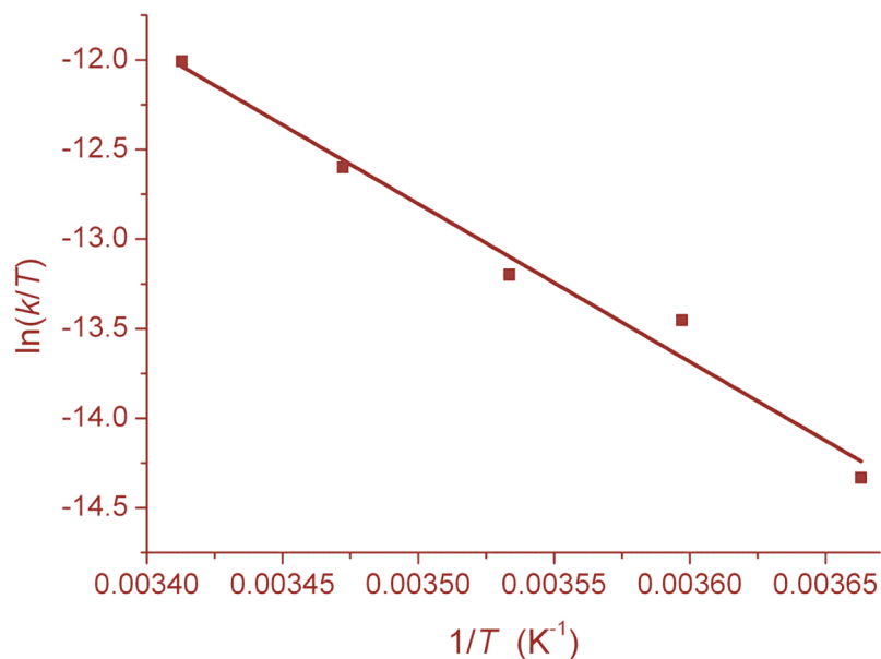
Figure 172: Eyring plot of \ln(k/T) vs T^{-1} (K -1 ) for the isomerization of 16a into 17a - 1 H NMR (600 MHz) line-shape between 273(1) and 293(1) K in toluene.
