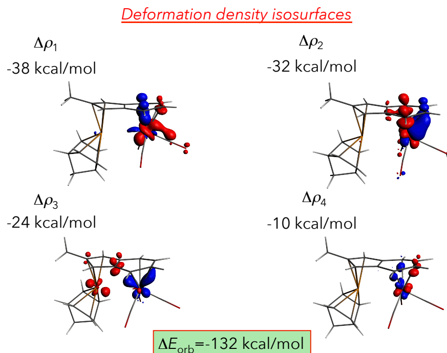
Figure 219: ETS-NOCV deformation densities \Delta\rho and the associated orbital interaction energies for the interaction of prepared \text{Cr}(\text{CO})_3 with the Rh-fluorenyl fragment of syn - 31a and syn - 31b . Red and blue-colored isosurfaces materialize regions where charge density depletion and build up occur respectively upon interaction of the two considered prepared fragments: electron density transfer operates from red-coloured areas to blue ones upon bonding. Density isosurface contour = 0.005 \text{ e/bohr}^3 .
