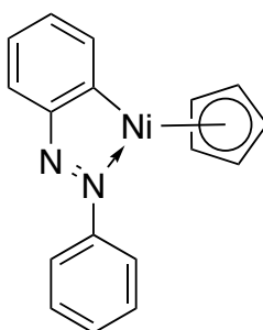
Figure 111: First metallacycle described by Kleinmann and Dubeck in 1963.
