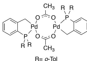
Figure 113: The first cyclopalladated catalyst precursor namely the tri- o -tolyl-phosphine complex.
