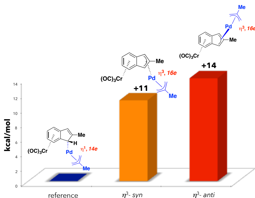
Figure 85: Energetic bias in favor of the \eta^1 mode in the syn -facial arrangement.
