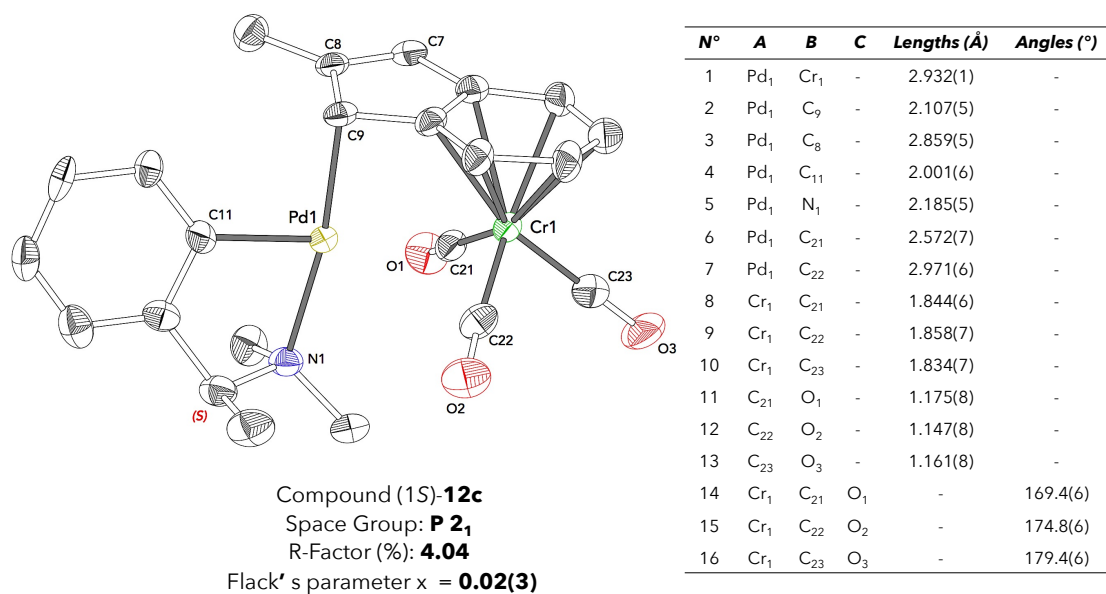
Figure 122: X-ray structure and selected interatomic distances of compound (1- S )- 12c .
