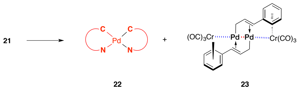
Figure 191: Compound 21 decomposes at room temperature into homoleptic compound 22 and a rare example of bis-Pd(I) bridged tetrametallic compound 23 .
