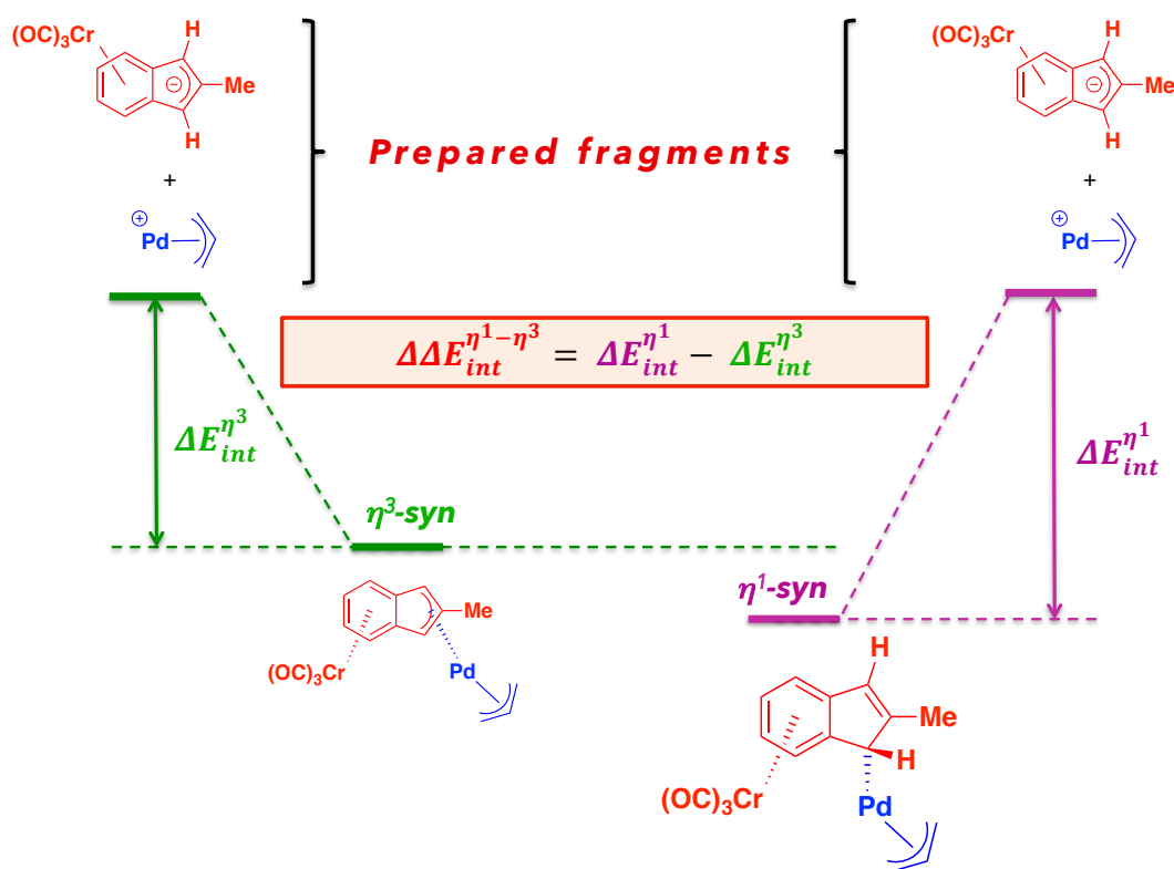
Figure 86: Considered fragments for the energy decomposition analysis.
