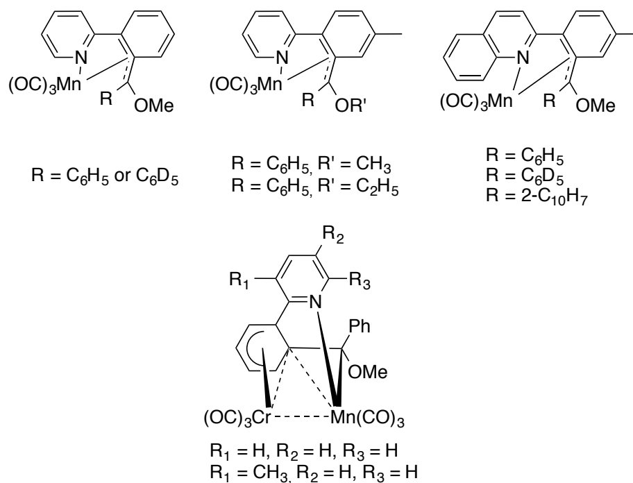
Figure 38: New classes of self-arranged helical chelated complexes.
