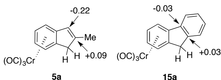
Figure 163: Natural partial charges (NPA) at C 2 and C 3 positions in 5a and 15a computed from gas phase singlet ground state geometries optimized at the ZORA-TPSS-D3(BJ)/all electron TZP level.
