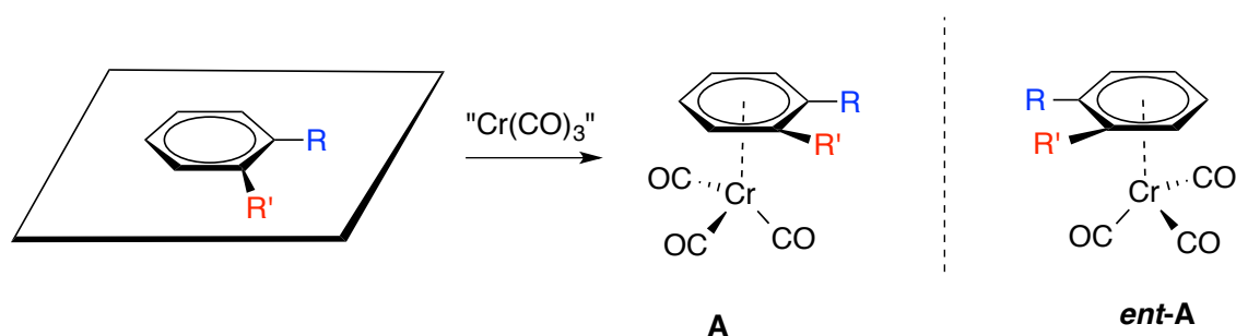
Figure 72: The coordination of a Cr(CO) 3 moiety to an arene results in a chiral compound.
