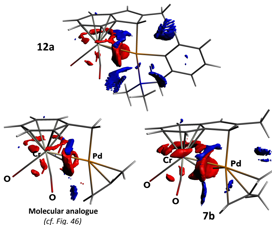
Figure 146: ADFview2013 plots of noncovalent interaction (NCI) regions materialized by reduced density gradient isosurfaces (cut-off value s = 0.02 au, \rho = 0.05 au) coloured according to the sign of the signed density \lambda_2\rho (red and blue colours are associated to negatively and positively signed terms) for gas-phase relaxed singlet ground state models of Pd-containing complexes 12a , 7b , and the molecular analogue reported by Kalinin et al. (cf. Figure 145 and CSDB refcode SOSTID). All calculations were performed with gas phase singlet ground state optimized geometries at the ZORA-PBE0-dDsC/all electron TZP level. Selected distances (in Å) for 7 : Cr–Pd, 2.698 (SOSTID 2.764); Pd–C benzyl , 2.119 (SOSTID 2.103); Pd–CCO, 2.370 (SOSTID 2.639).
