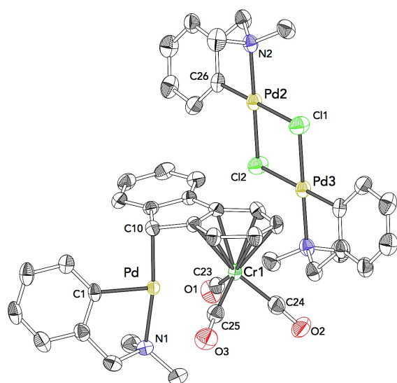
Compound 17a Space Group: P-1 R-Factor (%): 4.31
