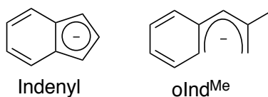
Figure 68: The indenyl and the open indenyl, oInd Me , ligands.
