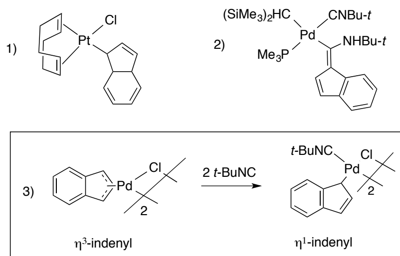
Figure 70: \eta -indenyl complexes of group 10 metals.
