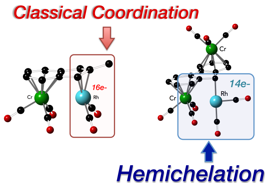
Figure 233: Illustration of the difference between the classical coordination and the hemichelation for Rh(I) derivatives.
