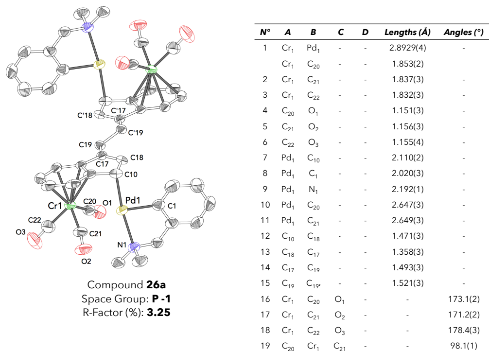
Figure 197: X-ray structure and selected interatomic distances of compound 26a .
