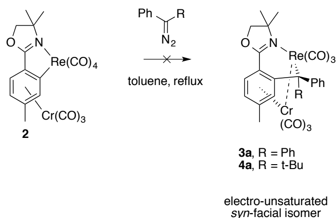
Figure 225: Expected formation of electron unsaturated heterobimetallic species.
