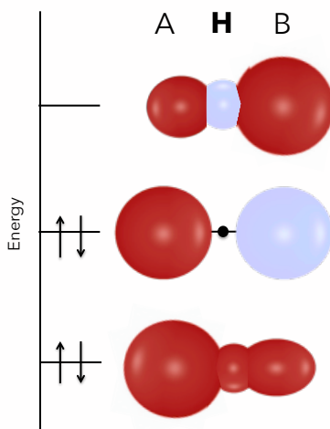
Figure 15: Molecular orbital interpretation of the formation of A-H...B . By starting from the three A, H, B orbitals, three new molecular orbitals can be formed. Only the two lower energetically orbitals are occupied, which may lead to a net diminution in energy compared with the separate AH and B species.
