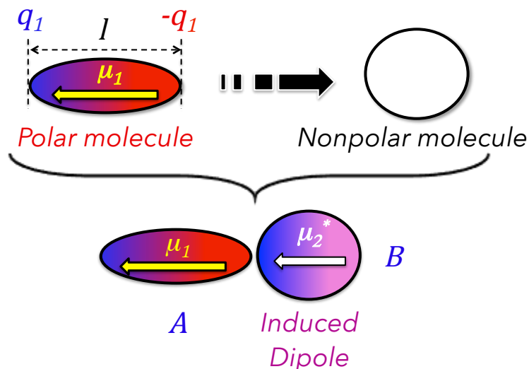
Figure 11: Illustration of the formation of an induced dipole by a polar molecule.
