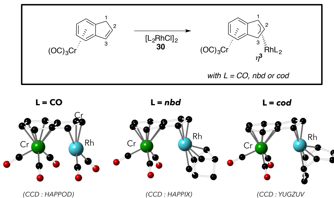
Figure 207: Cecon and coworkers demonstrated the syn -facial selectivity and \eta^3 coordination mode of the metal centre for some analogues.
