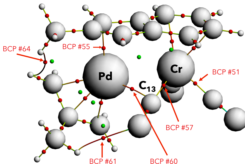
Figure 90: Atom-in-molecules analysis of the electron density topology for 7b . Red and green dots are associated to Bond (BCP) and Ring (RCP) Critical Points respectively. Grey spheres materialize the atomic critical points scaled by the associated density. Selected BCPs: #51, r = 0.1394 L_b = 0.1338 ; #55, r = 0.0856 L_b = -0.0444 ; #57, r = 0.1335 L_b = -0.1193 ; #60, r = 0.0493 L_b = -0.0290 ; #61, r = 0.00516 L_b = -0.00532 ; #64, r = 0.0407 L_b = -0.00348 . BCPs 55 and 60 correspond to the same type of closed shell interactions according to Popelier. BCP 61 does not fully fulfil the criteria for H bonding due to long interatomic distance. Worthy to note, there is no BCP in the Cr-Pd segment or in its immediate vicinity.
