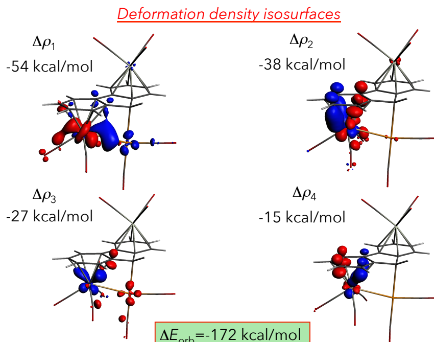
Figure 220: ETS-NOCV deformation densities \Delta\rho and the associated orbital interaction energies for the interaction of prepared \text{Cr}(\text{CO})_3 with the Rh-fluorenyl fragment of syn - 33a and syn - 33b . Red and blue-colored isosurfaces materialize regions where charge density depletion and build up occur respectively upon interaction of the two considered prepared fragments: electron density transfer operates from red-coloured areas to blue ones upon bonding. Density isosurface contour = 0.005 \text{ e/bohr}^3 .
