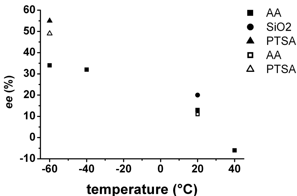
Figure 159: ee vs temperature (isolated yields span from 30 to 60 %), the negative value corresponds to a reversed enantioselectivity; filled and unfilled symbols are for reactions carried out with (1 S )- 12c , respectively. (Enantiomeric excess ee was calculated for reactions with (1 S )- 12c as follows: ee = 100 \times \frac{[pS-5a] - [pR-5a]}{[pR-5a] + [pS-5a]} where brackets express concentrations. For reactions with (1 R )- 12c the numerator becomes [pR-5a] - [pS-5a] ).
