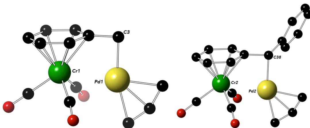
Figure 83: X-Ray structures of molecular analogues of 7a-c reported by Kalinin et al.
