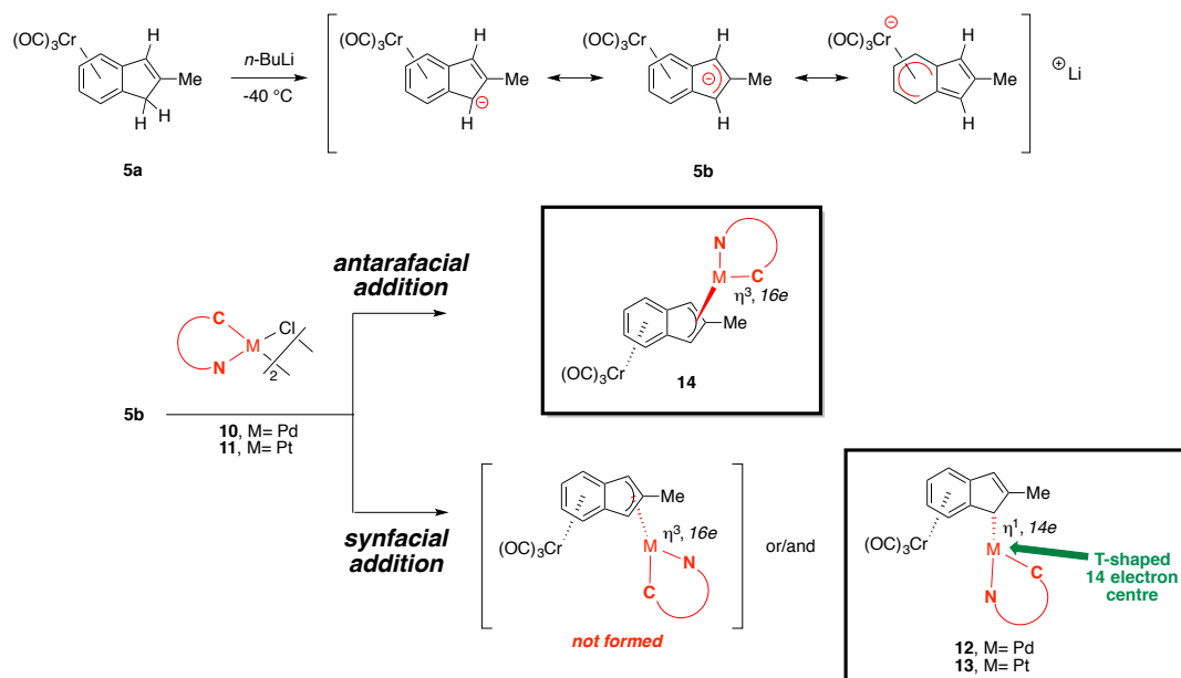
Figure 117: The ambiphilic character of anion 5b allows two facial interactions with Pd and Pt metallacycles 10 or 11 , that is, either the antara -facial leading to the (\eta^3\text{-indenyl})\text{M} complexes 14 or the syn -facial leading exclusively to (\eta^1\text{-indenyl})\text{M} complexes 12 and 13 , a new class of electron-unsaturated T-shaped \eta^1 -indenyl Pd/Pt complexes.
