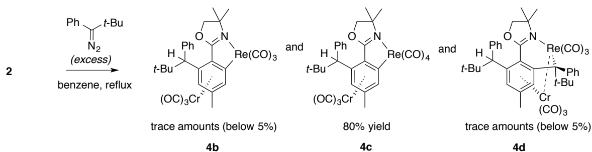
Figure 226: Reaction of 2 with ( t -Bu)(Ph)CN 2 .
