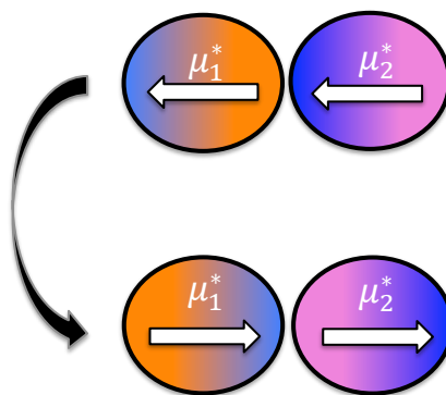
Figure 13: The two instantaneous dipoles are correlated, although they occur in different orientations at different instants.
