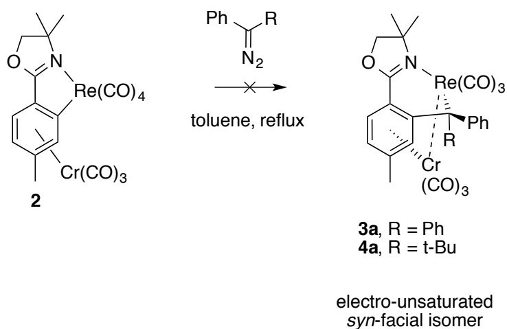
Figure 54: Expected formation of electron unsaturated heterobimetallic species.
