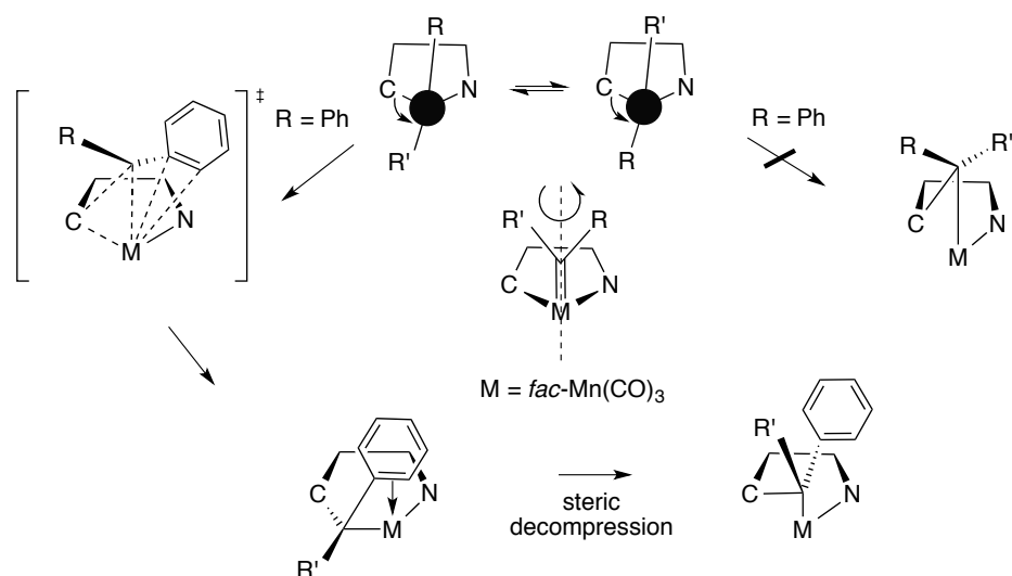
Figure 47: Origin of stereoselective formation of metallocarboranes species.
