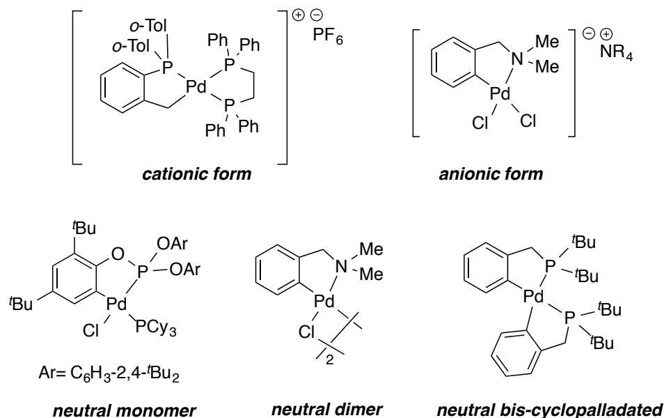
Figure 109: Different kind of CY species.
