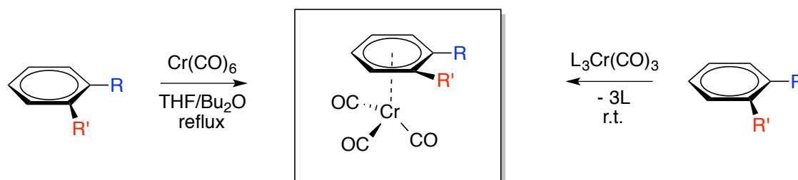
Figure 74: Pathways for the preparation of chromium arene complexes.
