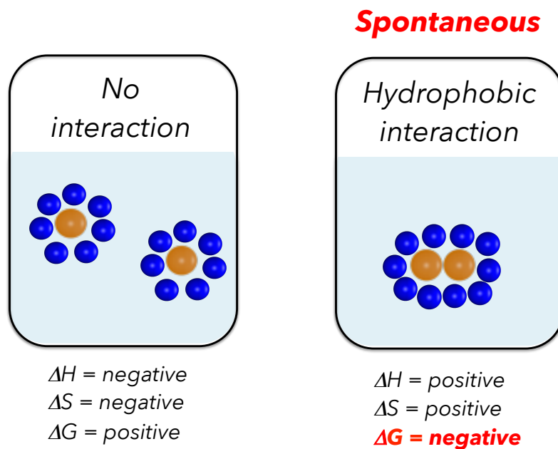
Figure 18: Illustration of the spontaneous process of the hydrophobic interaction.
