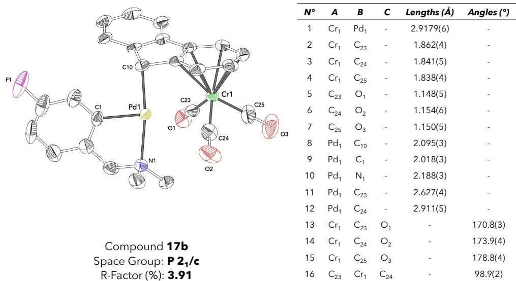
Figure 176: X-ray structure and selected interatomic distances of compound 17b .
