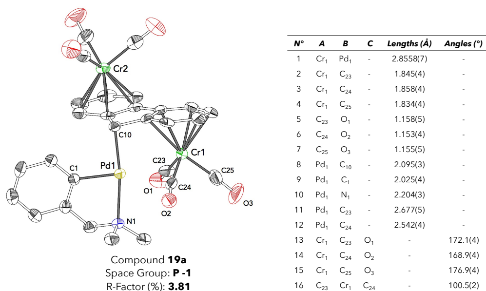
Figure 182: X-ray structure and selected interatomic distances of compound 19a .
