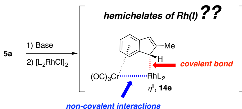
Figure 202: Expected formation of Rh(I) hemichelation by using 5a as an heteroditopic ligand.
