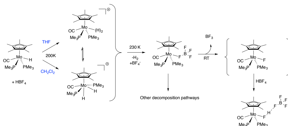
Figure 28: Overall reaction of Mo complex with \text{HBF}_4 . Published by Poli et al. 472 © 2014 American Association for the Advancement of Science
