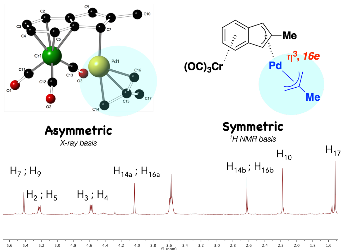
Figure 93: Contradictions between the ^1\text{H} NMR spectrum of an apparently symmetric molecule and the X-ray structure showing an asymmetric complex.
