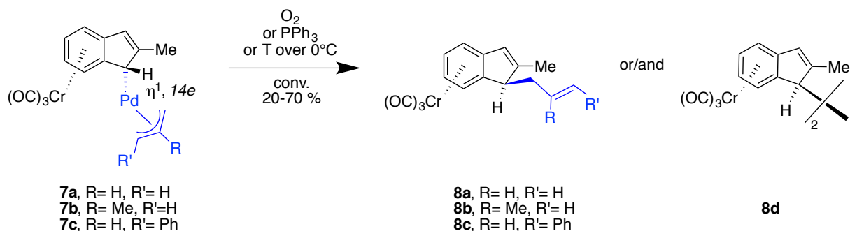
Figure 102: Decomposition pathway of 7a-c leading to the tricarbonyl( \eta^6 -2-methylindenyl)chromium moiety and the allyl ligand.
