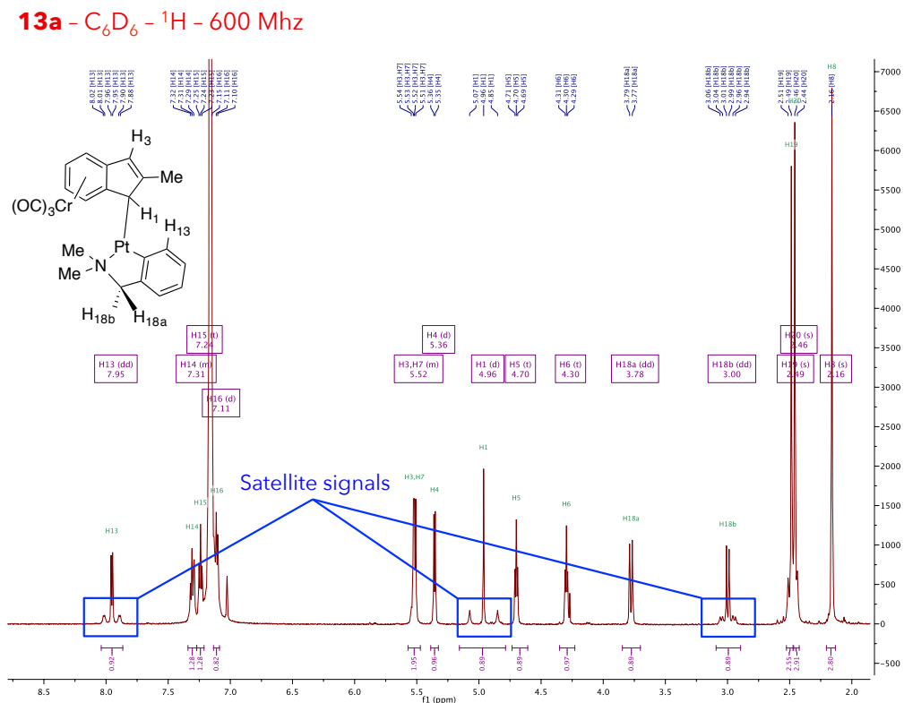
Figure 137: Typical satellite signals arising from the coupling of ^1\text{H} nuclei with the ^{195}\text{Pt} isotope in complex 13a .
