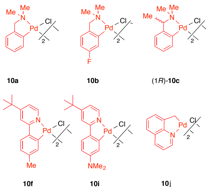
Figure 164: \mu -chloro-bridged palladacycles which were probed for their reactivity toward anion 15b .
