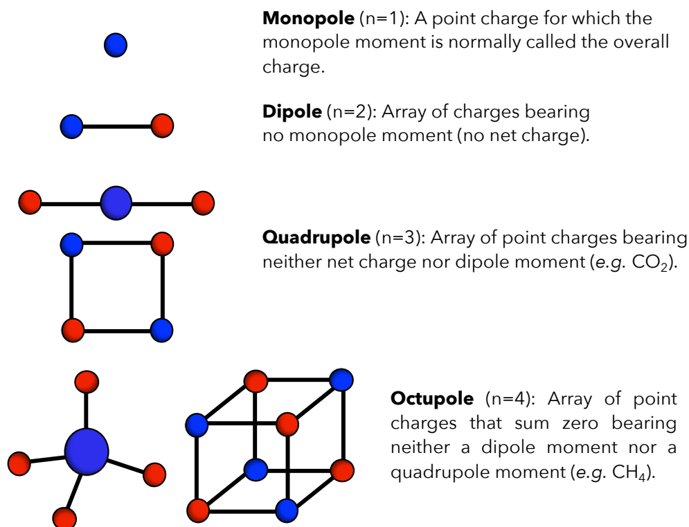
Figure 10: Illustration of typical charge arrays corresponding to electric multipoles.
