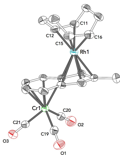
Compound anti - 32c Space Group: P-1 R-Factor (%): 3.99
