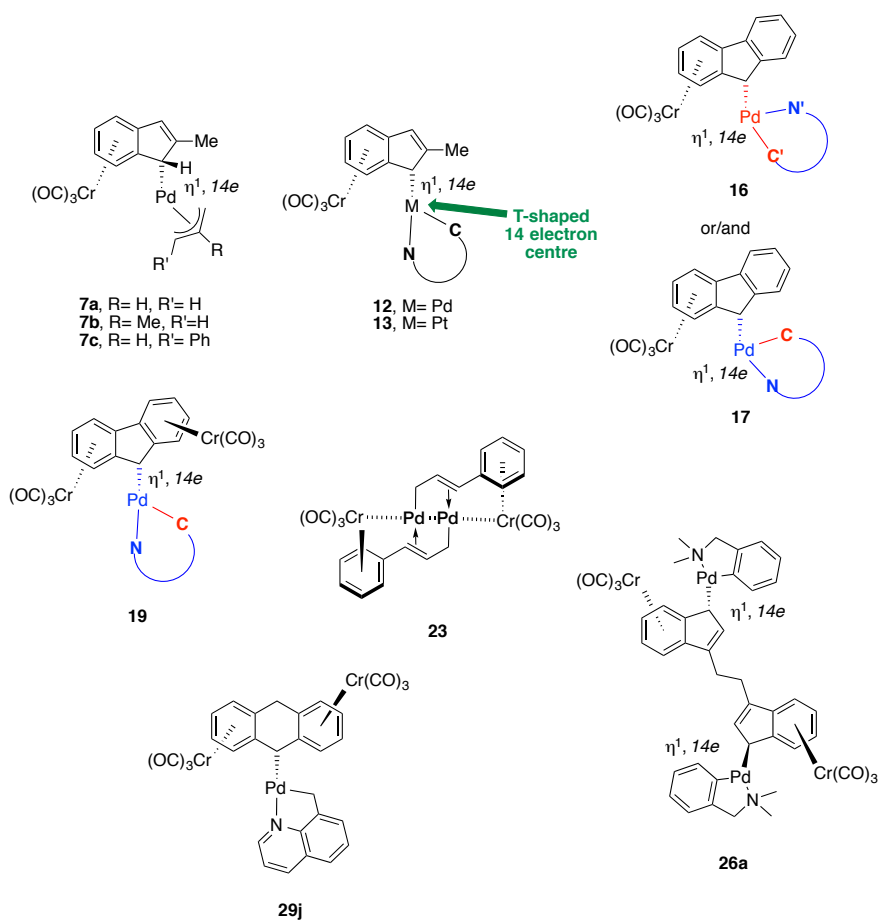
Figure 229: List of the coordinatively unsaturated Pd(II)/Pt(II) complexes synthesized.
