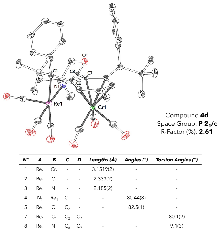
Figure 62: X-ray structure and selected interatomic distances of compound 4d .
