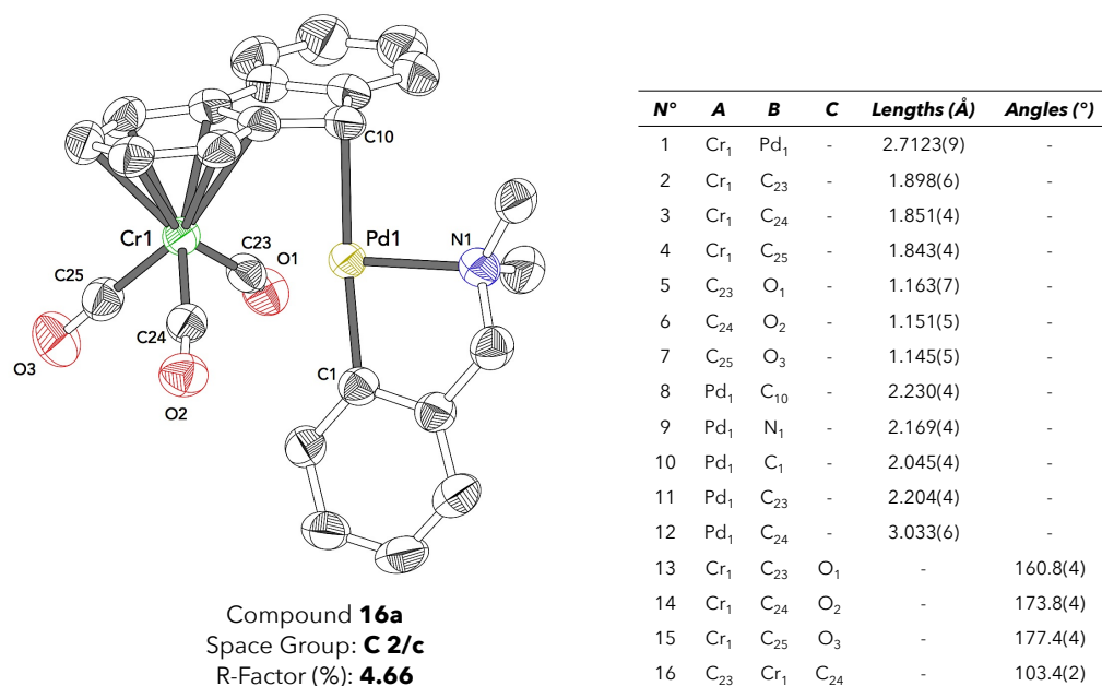
Figure 166: X-ray structure and selected interatomic distances of compound 16a .
