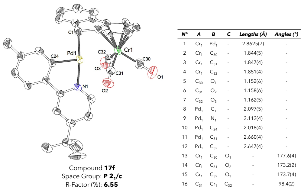
Figure 178: X-ray structure and selected interatomic distances of compound 17f .
