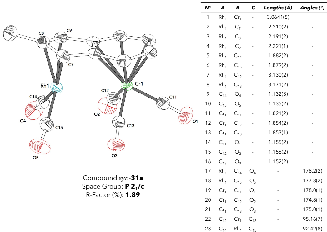
Figure 205: X-ray structure and selected interatomic distances of compound syn-31a .
