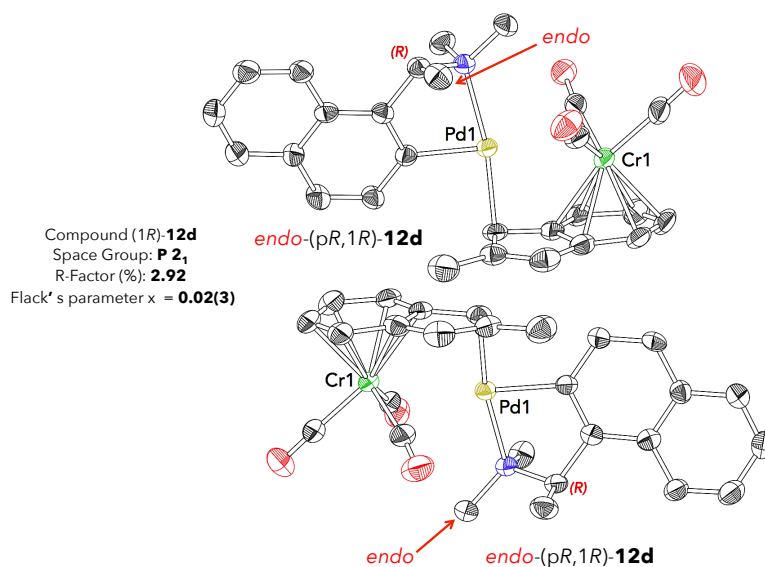
Figure 131: X-ray structure of compound ( 1R )- 12d containing only the endo diastereomer.
