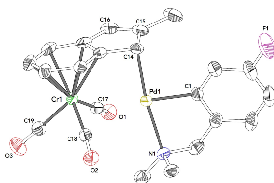
Compound 12b Space Group: P 2 1 /c R-Factor (%): 2.75
