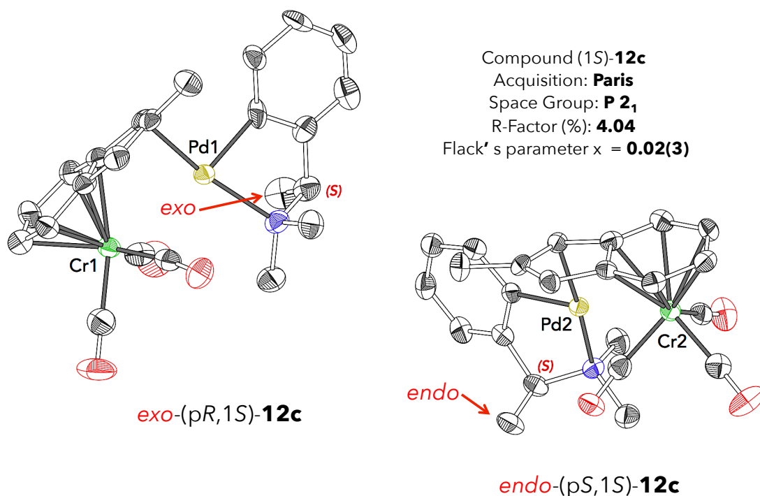
Figure 128: X-ray structure of compound (1-S)- 12c (acquisition performed in Paris).
