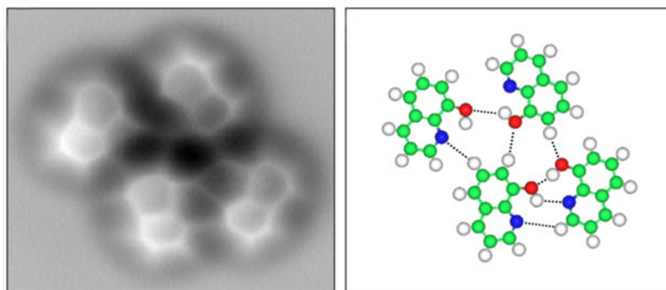
Figure 14: Hydrogen bonding visualized in 8-hydroxyquinoline using a non-contact AFM microscope at the National Centre for Nanoscience and Technology, China. Author: Royal Society of Chemistry (rsc.org), Public domain via Wikimedia Commons.
