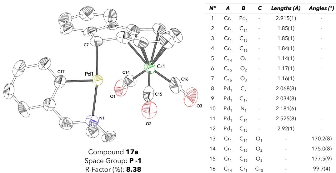
Figure 175: X-ray structure and selected interatomic distances of compound 17a .
