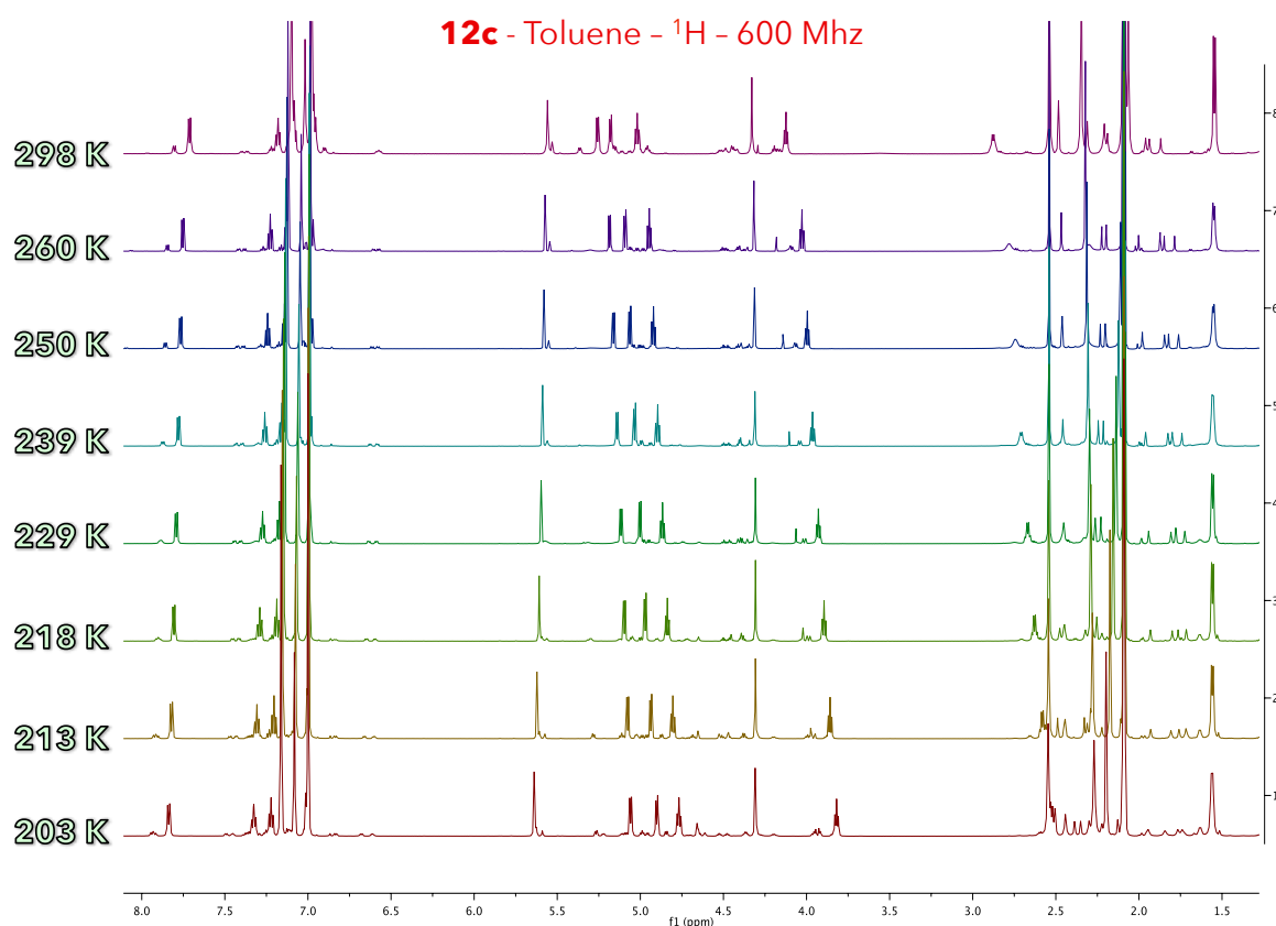
Figure 136: ^1\text{H} NMR variable temperature investigations of (1 S )- 12c at subambient temperatures did not reveal any significant line broadening of the signals of \text{H}_1 and \text{H}_3 upon cooling.
