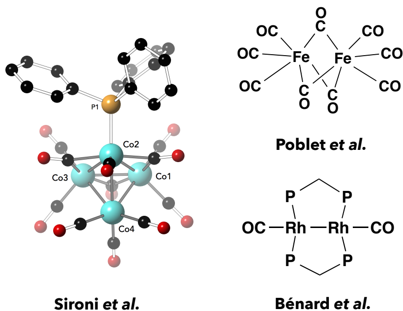
Figure 145: Other examples of carbonyl complexes.
