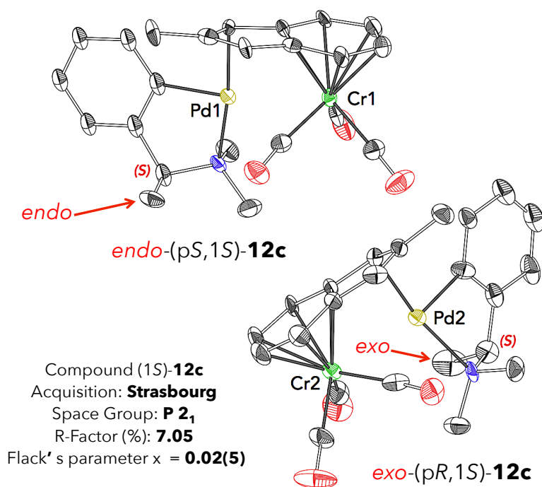
Figure 129: X-ray structure of compound (1-S)- 12c (acquisition performed in Strasbourg).
