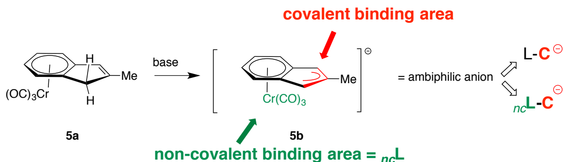
Figure 77: Ambiphilic character of anion 5b .
