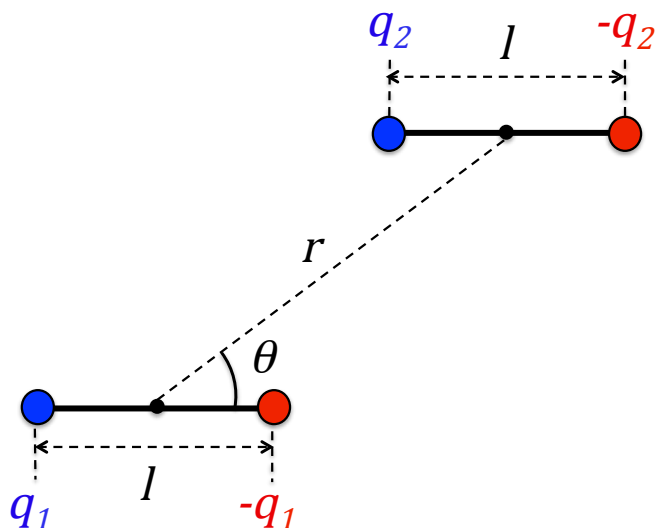
Figure 9: Consideration of the interaction between two parallel dipoles.
