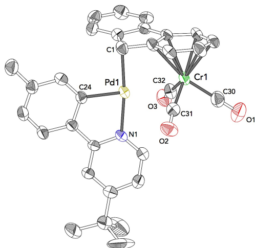
Compound 17f Space Group: P 2 1 /c R-Factor (%): 6.55
