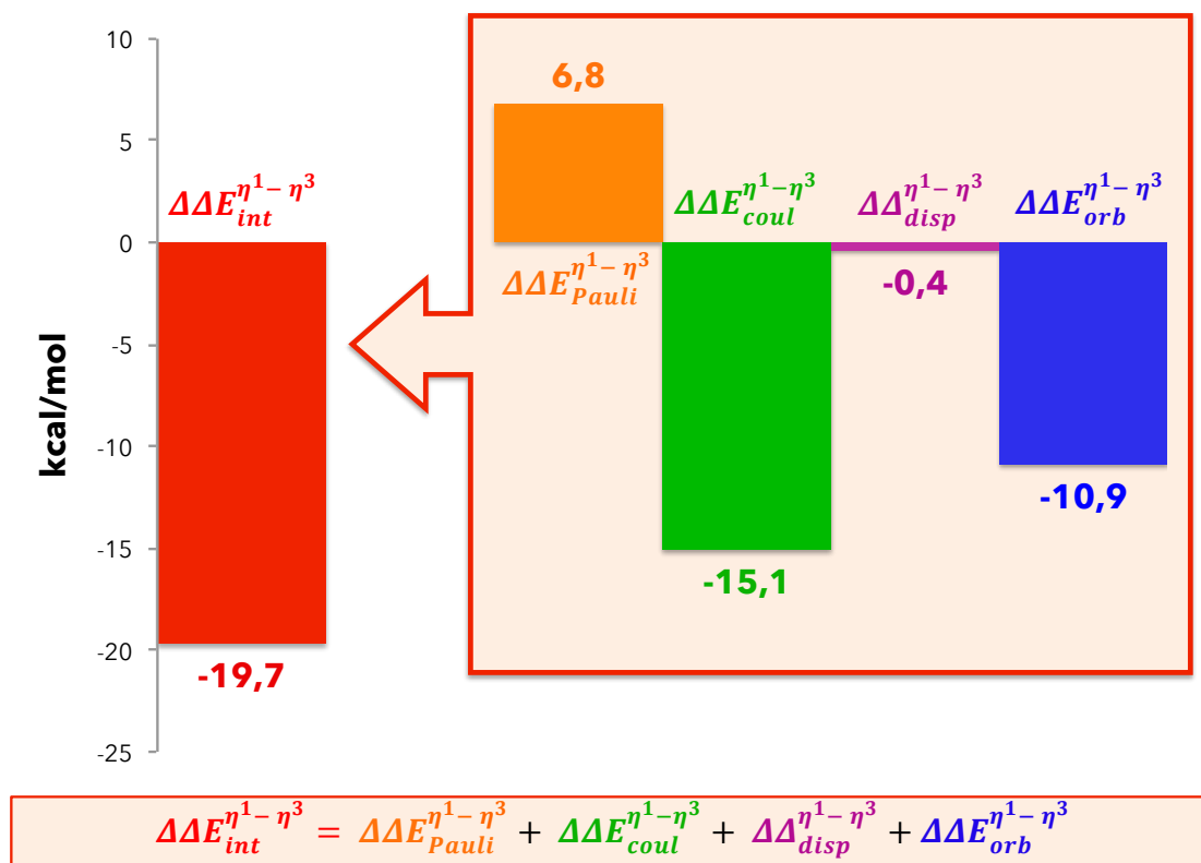
Figure 87: Contribution of each term in the stabilization of the \eta^1 coordination mode.
