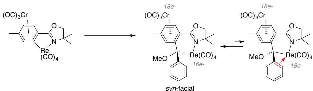
Figure 224: Expected formation of two “pseudoconformers”. A syn -facial electron-unsaturated 18-16 electrons isomer and an electron-saturated 18-18 electrons isomer.
