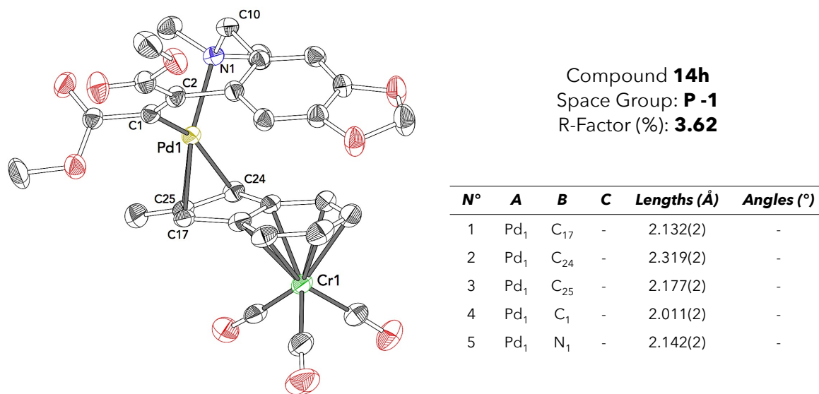
Figure 127: X-ray structure and selected interatomic distances of compound 14h .
