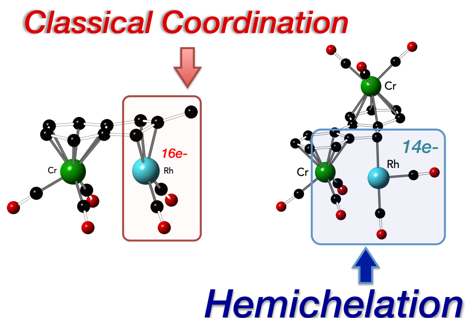
Figure 222: Illustration of the difference between the classical coordination and the hemichelation for Rh(I) derivatives.
