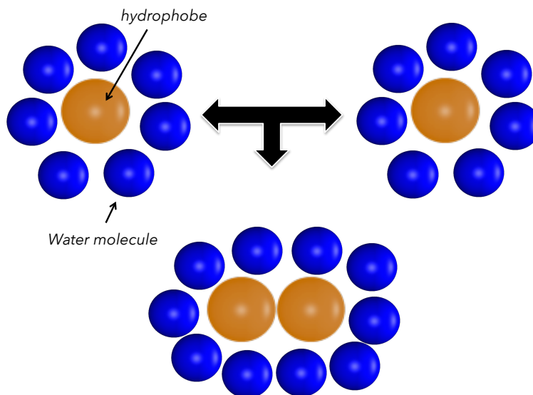
Figure 16: Illustration showing that when hydrophobes come together they will have less contact with the water molecules.
