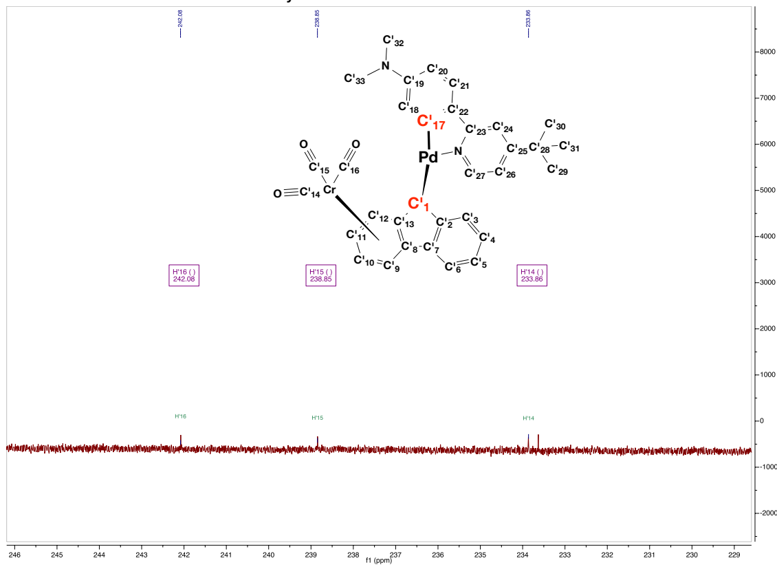
Tol – 13C – 126 Mhz – 293 K - Carbonyls.
