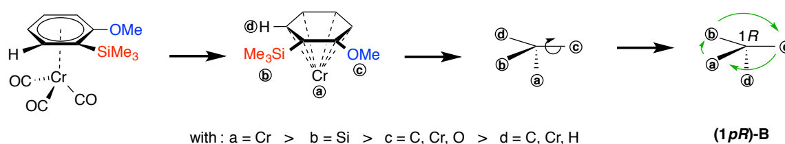
Figure 73: Example of stereochemical assignment of the chirality of a chromium arene complex.
