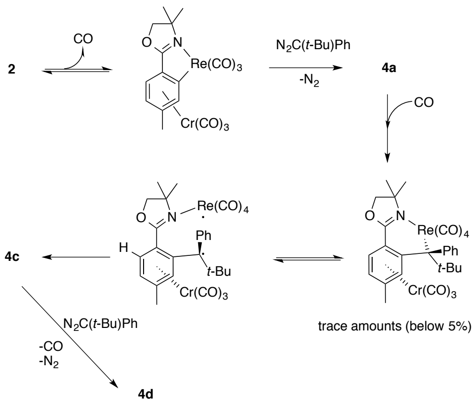
Figure 63: Mechanism rationalizing the double condensation of (t\text{-Bu})(\text{Ph})\text{CN}_2 .
