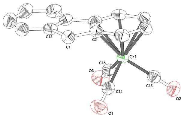
Compound 15a Space Group: P 2 1 2 1 2 1 R-Factor (%): 3.87
