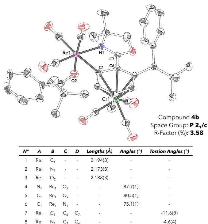
Figure 60: X-ray structure and selected interatomic distances of compound 4b .
