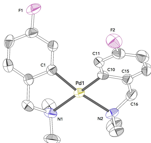
Compound 22b Space Group: P b c a R-Factor (%): 4.65
