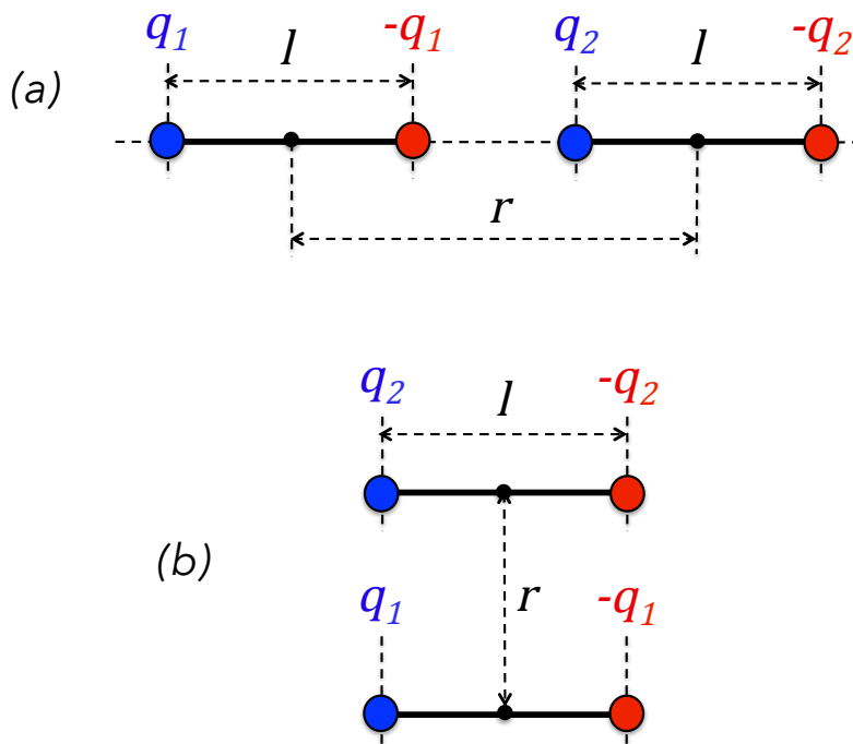
Figure 8: Consideration of the easiest manner of interaction between two dipoles.
