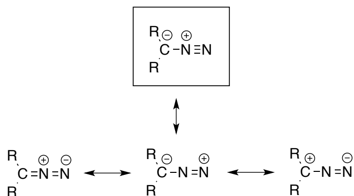
Figure 53: Charge delocalisation and mesomeric diazoalkane forms.
