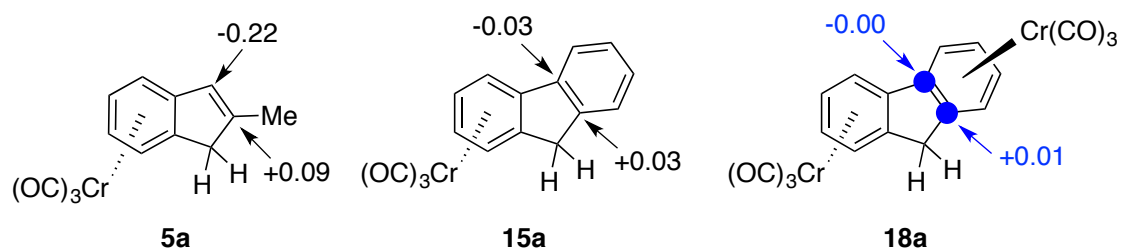
Figure 232: Natural partial charges (NPA) at C 2 and C 3 positions in 5a , 15a and 18a computed from gas phase singlet ground state geometries optimized at the ZORA-TPSS-D3(BJ)/all electron TZP level.
