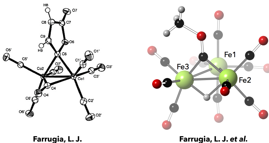
Figure 162: Examples of homometallic bridged transition metal carbonyl dimers described by Farrugia et al.
