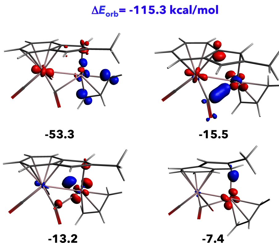
Figure 88: NOCV-ETS \Delta\rho^{\text{orb}} deformation densities computed at the (ZORA) PBE[-D3(BJ)]/all-electron TZP level for the interaction between closed-shell prepared fragments 5b and [(\eta^3\text{-allyl})\text{Pd}]^+ in \eta^1\text{-7a} with the associated orbital interaction energies (kcal/mol) with isosurfaces of 0.01 and 0.005 e/bohr 3 for the plots of highest orbital interaction energy and for the remaining three plots respectively. Blue and red colours are respectively associated with areas of electron density build-up and depletion upon interaction.
