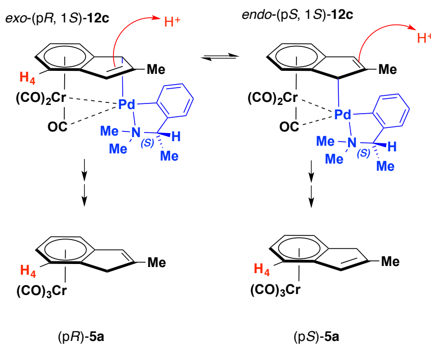
Figure 151: Kinetic quench of the putative endo-exo isomerization by proto-depalladation results from an exo -attack of H^+ at the indenyl, a pathway established by a reaction of 12a with CD_3CO_2D , which resulted into the predominant formation of exo deuterated rac - 5a at position 1.
