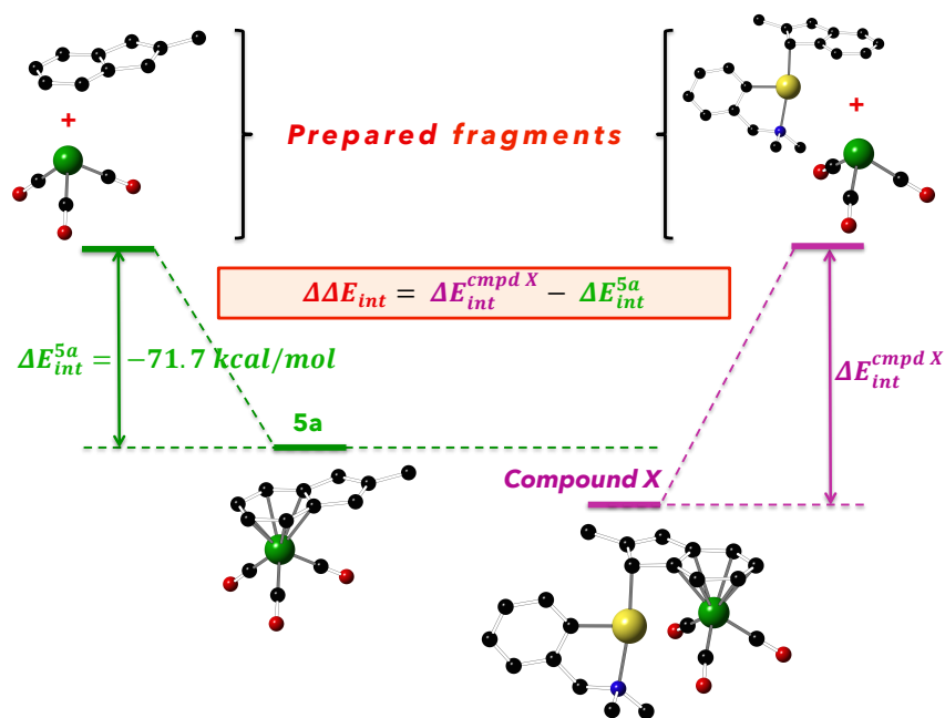
Figure 148: Considered fragments for the energy decomposition analysis.
