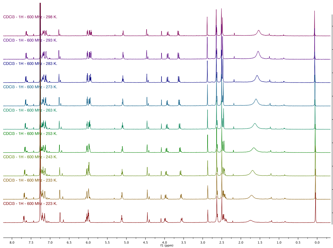
CDCl 3 - 1 H - 600 Mhz - Variable Temperature.
