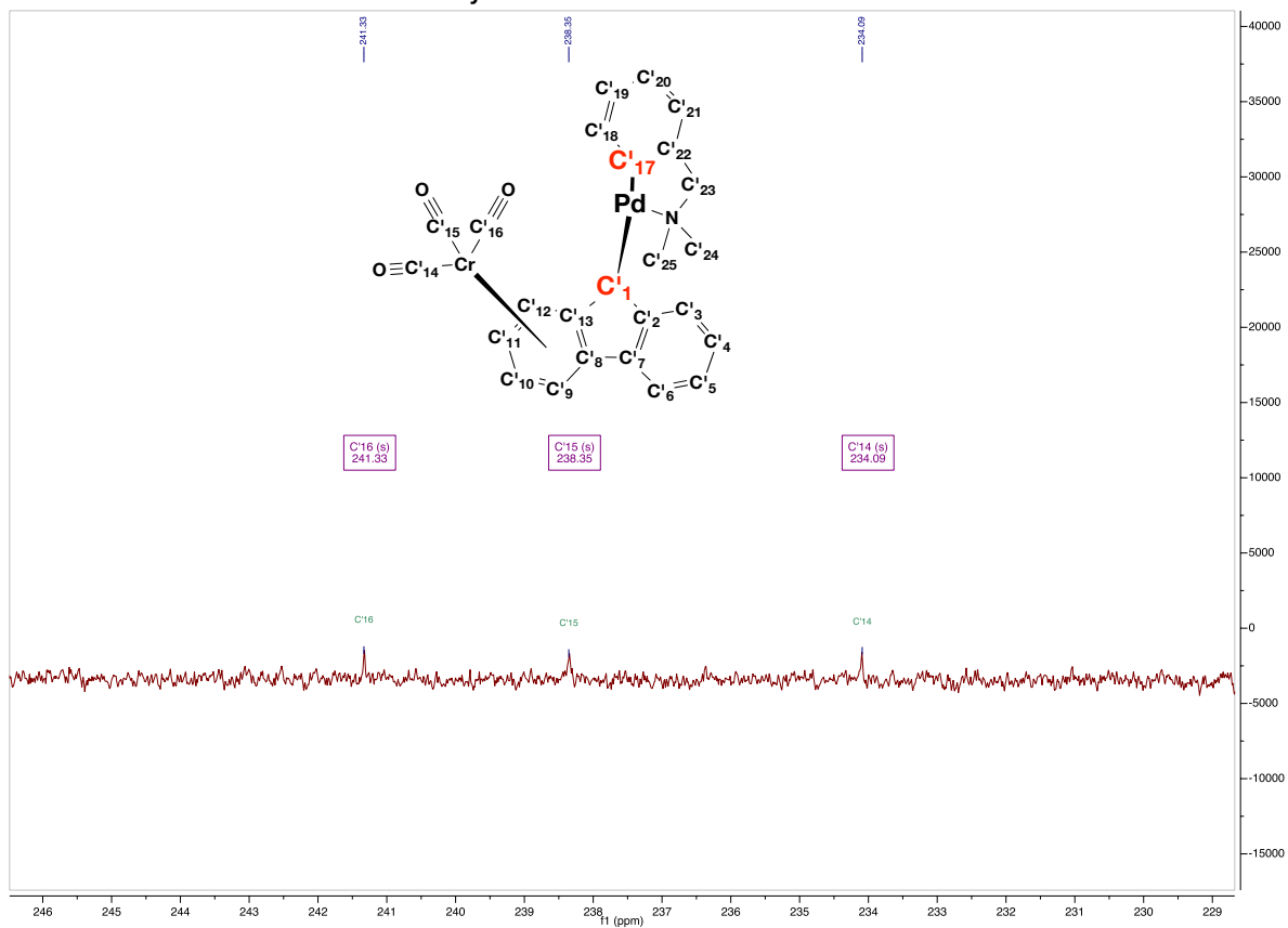
Tol - 13C - 126 Mhz - 223 K - Carbonyls.
