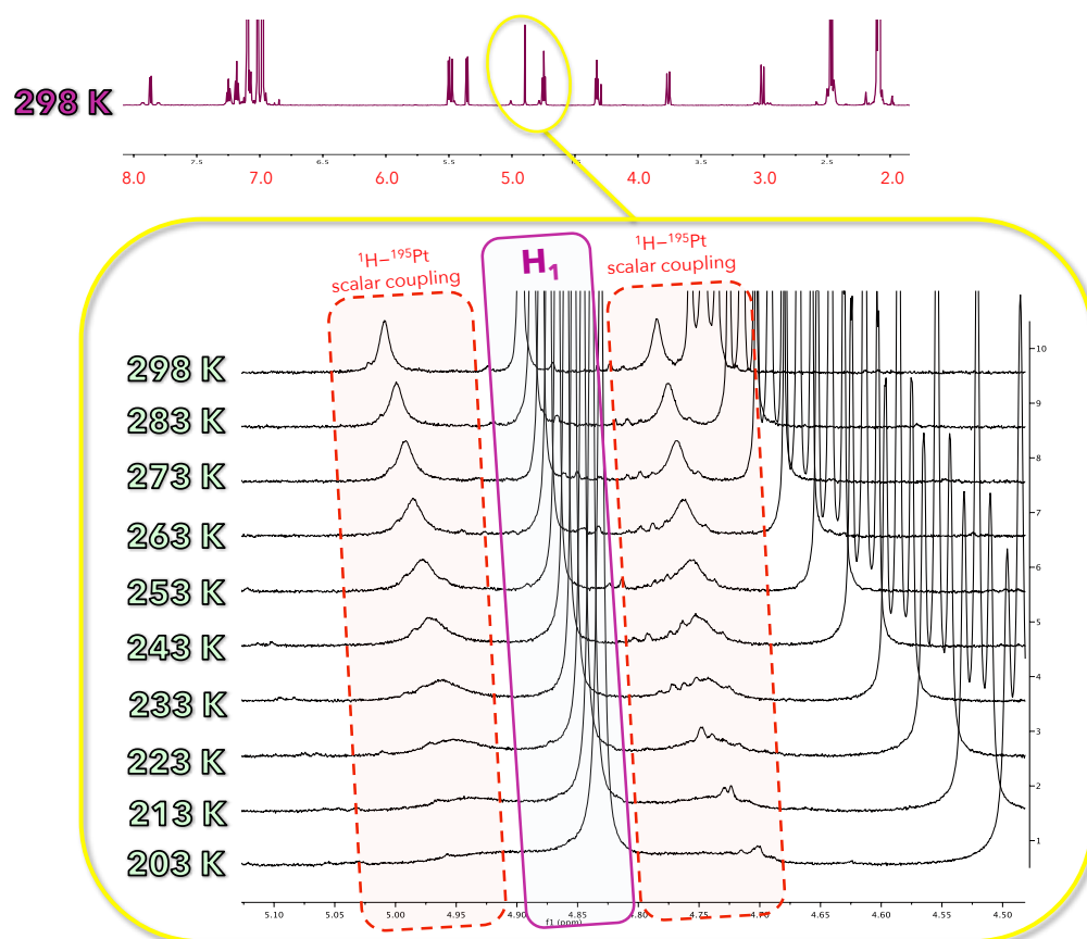
Figure 138: ^1\text{H} NMR variable temperature of 13a revealing the satellite signals broadening upon lowering the temperature of the NMR probe to eventually vanish at 213 K.
