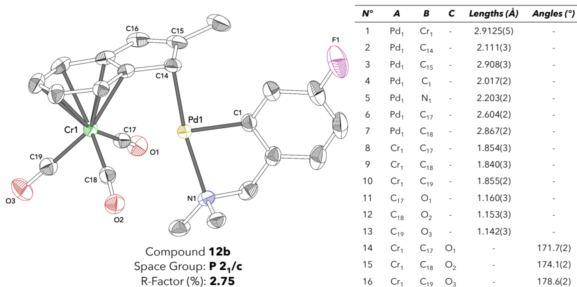
Figure 119: X-ray structure and selected interatomic distances of compound 12b .
