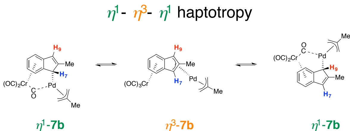
Figure 230: Supposed fluxional behavior of the Pd centre.
