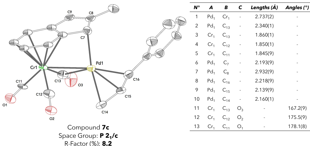
Figure 82: X-ray structure and selected interatomic distances of compound 7c .
