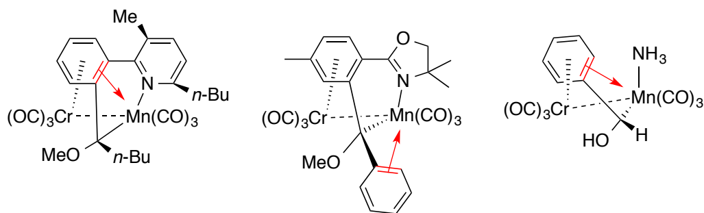
Figure 48: Some metallocenes molecules used in the theoretical study.
