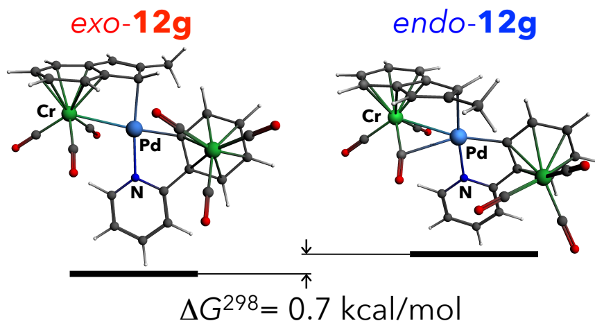
Figure 134: Gas-phase singlet ground-state geometries of the isoenergetic exo and endo - 12g diastereomers (ZORA-PBE-D3(BJ)/all electron TZP, T = 298.15 \text{ K} ).
