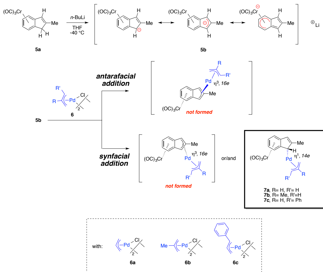
Figure 79: Synthesis of complexes 7a-c derived from 2-Methyl-1 H -indene.
