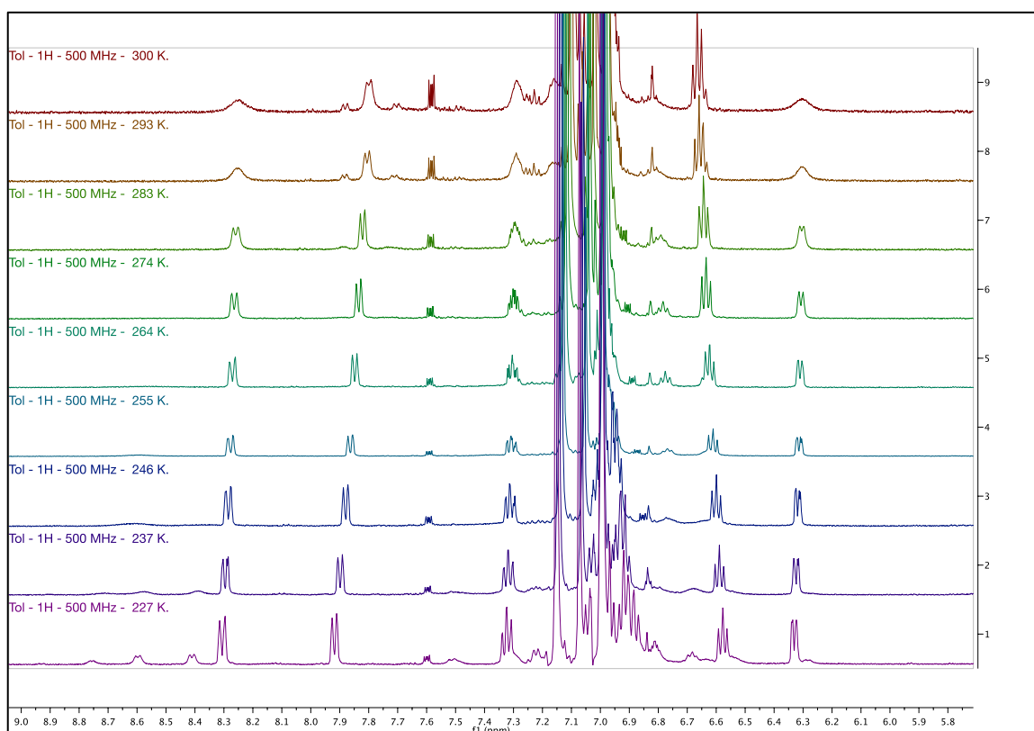
Figure 57: Variable temperature in deuterated toluene showing the partial decoalescence of the 2-bonded phenyl group.
