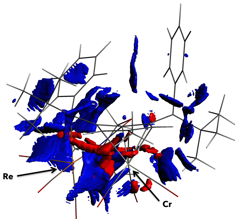
Figure 64: ADFview 2013 plot of NCI regions materialized by reduced density gradients isosurfaces (cutoff value s= 0.02 au, \rho= 0.05 ) coloured according to the signed density \lambda_2\rho (red and blue colours are assigned to negative and positive signs respectively) for the gas-phase singlet ground state geometry of 4d computed at the ZORA-PBE-D3(BJ)/all electron TZP level).
