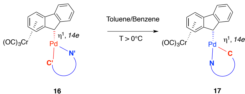
Figure 169: Isomerization process of 16 into 17 occurring in solution at temperatures over 0°C.
