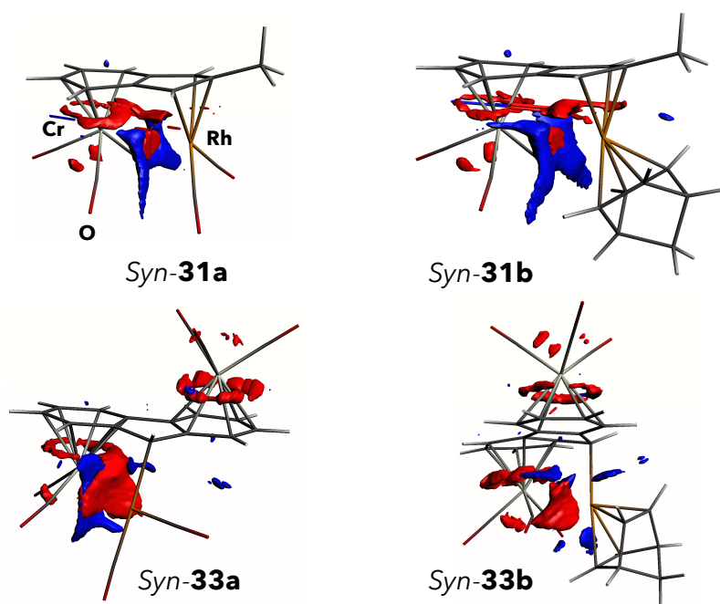
Figure 216: Plots of non-covalent interaction (NCI) regions materialized by reduced density gradient isosurfaces (cut-off value s= 0.02 a.u., \rho=0.05 a.u.) coloured according to the sign of the signed density \lambda_2\rho for gas-phase relaxed singlet ground state models of Rh-containing complexes syn-31a , syn-31b , syn-33a and syn-33b ; red and blue colours are associated to negatively (attractive) and positively (repulsive) signed terms respectively.
