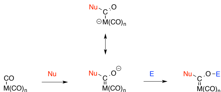
Figure 41: Fischer-type carbene intermediate mechanism.
