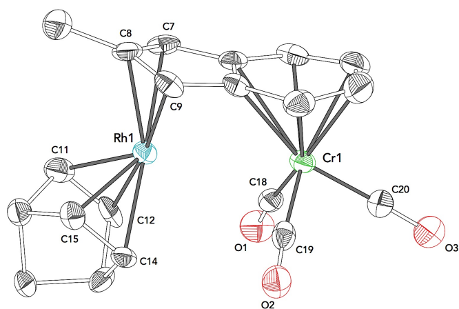
Compound syn-31b Space Group: C 2/c R-Factor (%): 4.82
