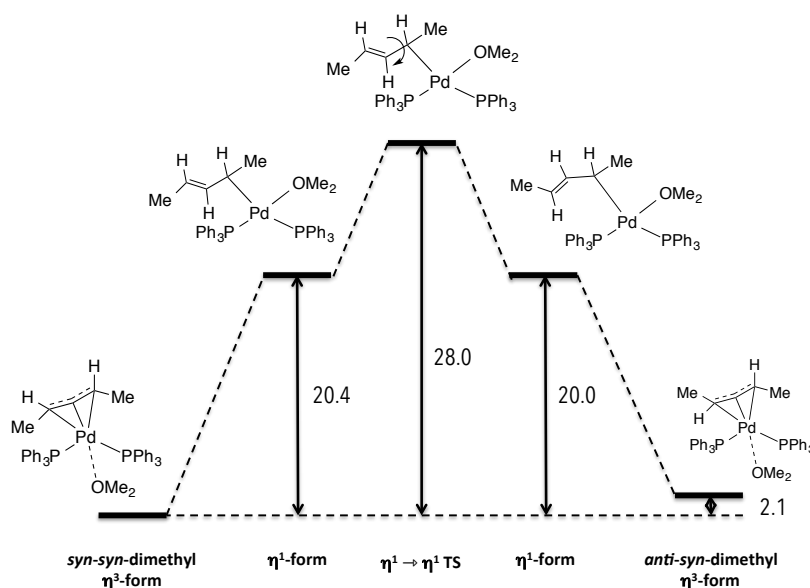
Figure 101: Diagram reproducing the \eta^3 \rightarrow \eta^1 \rightarrow \eta^3 isomerization process of ( \eta^3 -allyl)palladium complexes have been studied by Solin et al. 863 by applying density functional theory at the B3PW91(DZ+P) level.
