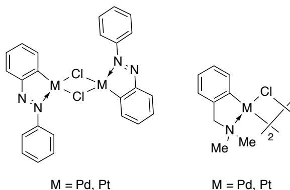
Figure 112: First palladium and platinum metallacycles described by Cope et al.
