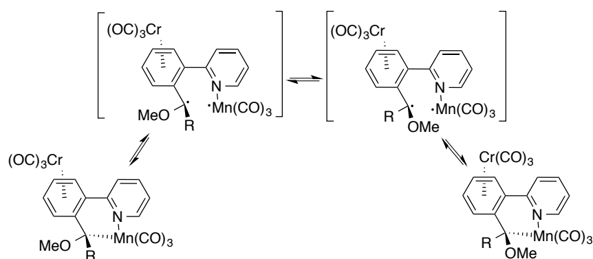
Figure 45: Interconversion between the two isomers with the probable mediation of biradical species.
