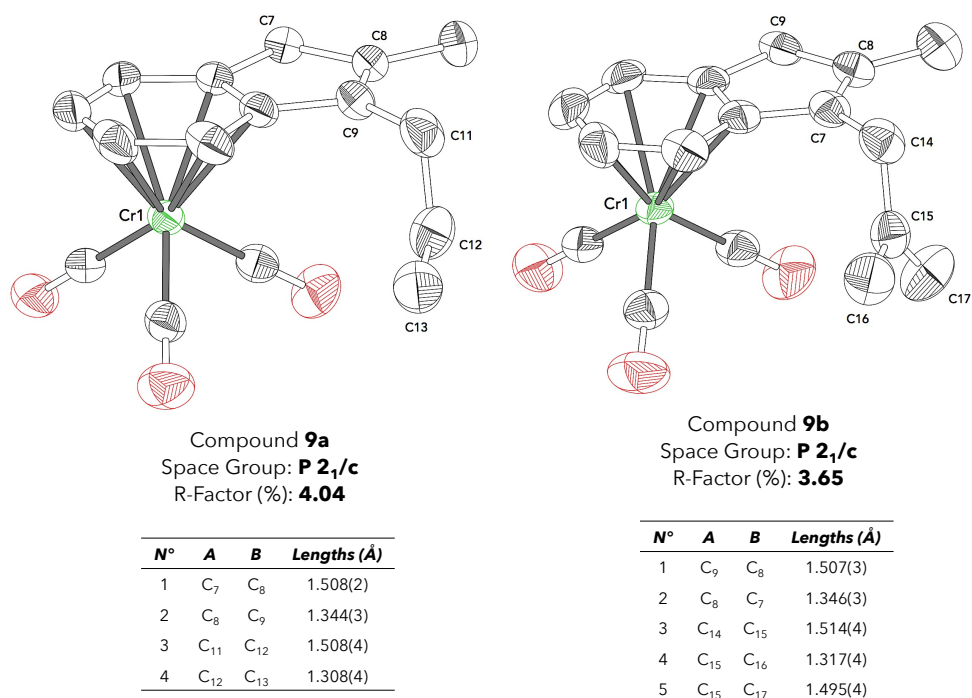
Figure 105: X-ray structure and selected interatomic distances of compounds 9a and 9b .
