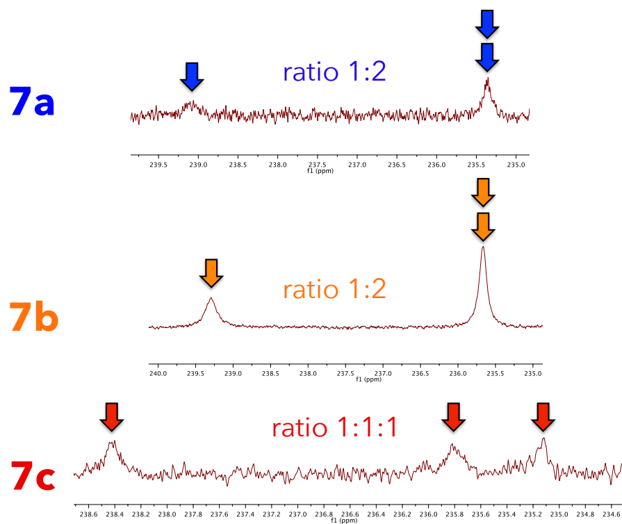
Figure 91: Multiple large ^{13}\text{C} NMR signals at room temperature for the carbonyls of the \text{Cr}(\text{CO})_3 moiety in the case of complexes 7a-c .
