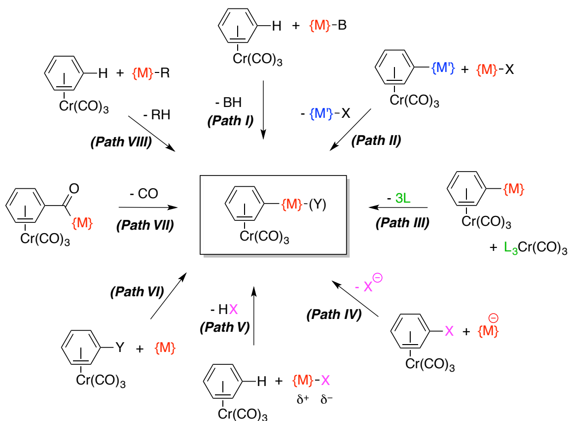
Figure 76: Summary of the different routes to prepare \sigma - \pi -bridged heterobimetallic complexes bearing a \text{Cr}(\text{CO})_3 unit.
