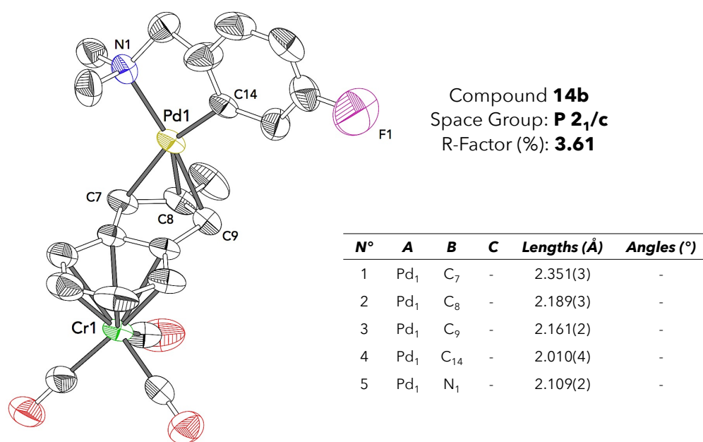
Figure 120: X-ray structure and selected interatomic distances of compound 14b .
