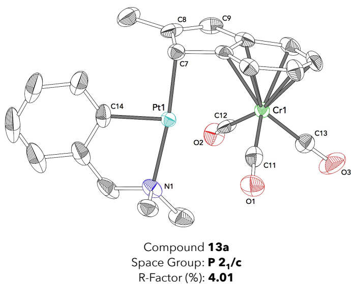
Figure 126: X-ray structure and selected interatomic distances of compound 13a .
