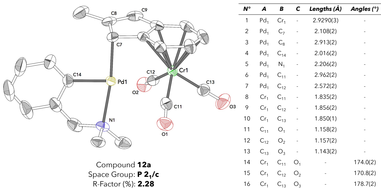
Figure 118: X-ray structure and selected interatomic distances of compound 12a .
