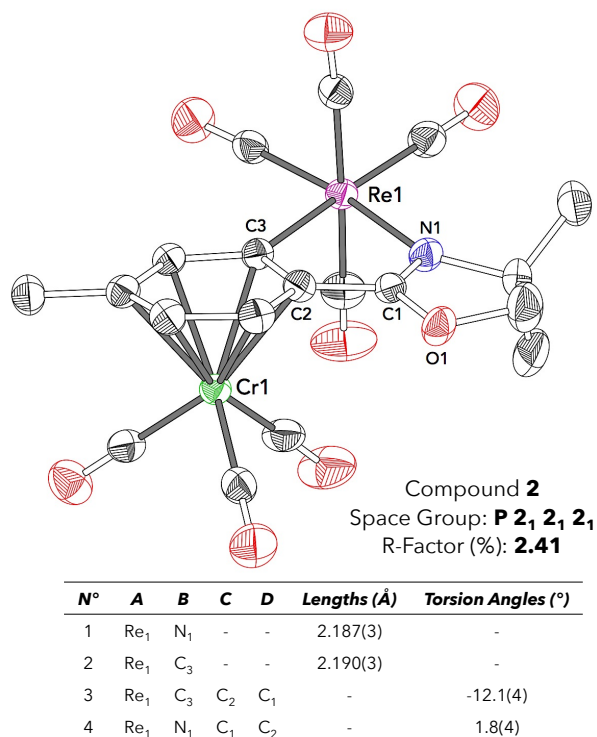
Figure 52: X-ray structure and selected interatomic distances of compound 2 .
