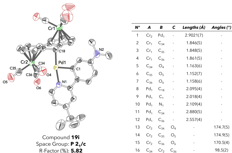
Figure 183: X-ray structure and selected interatomic distances of compound 19i .
