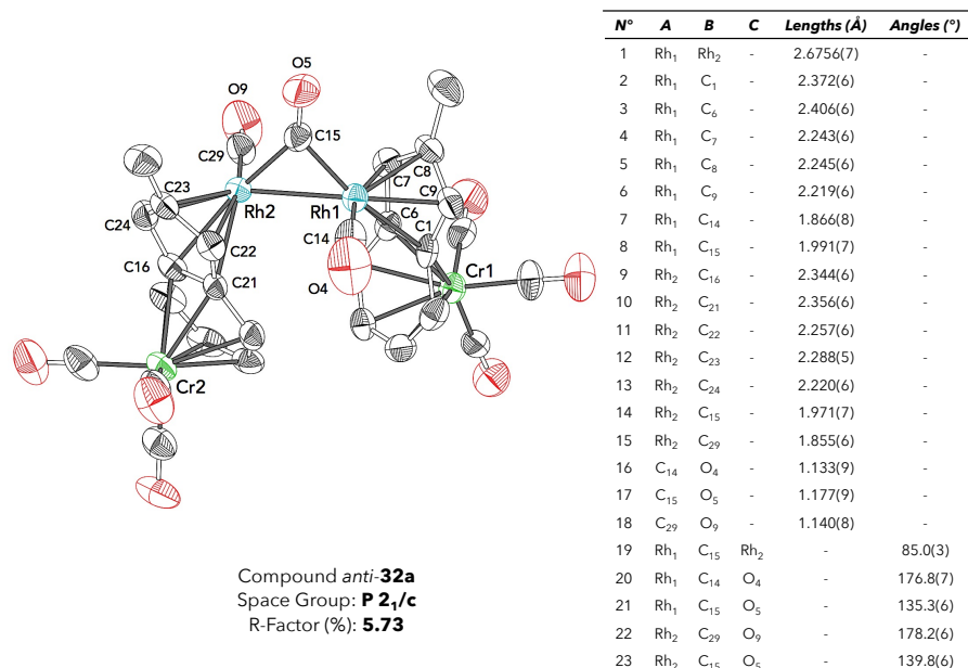
Figure 209: X-ray structure and selected interatomic distances of compound anti-32a .
