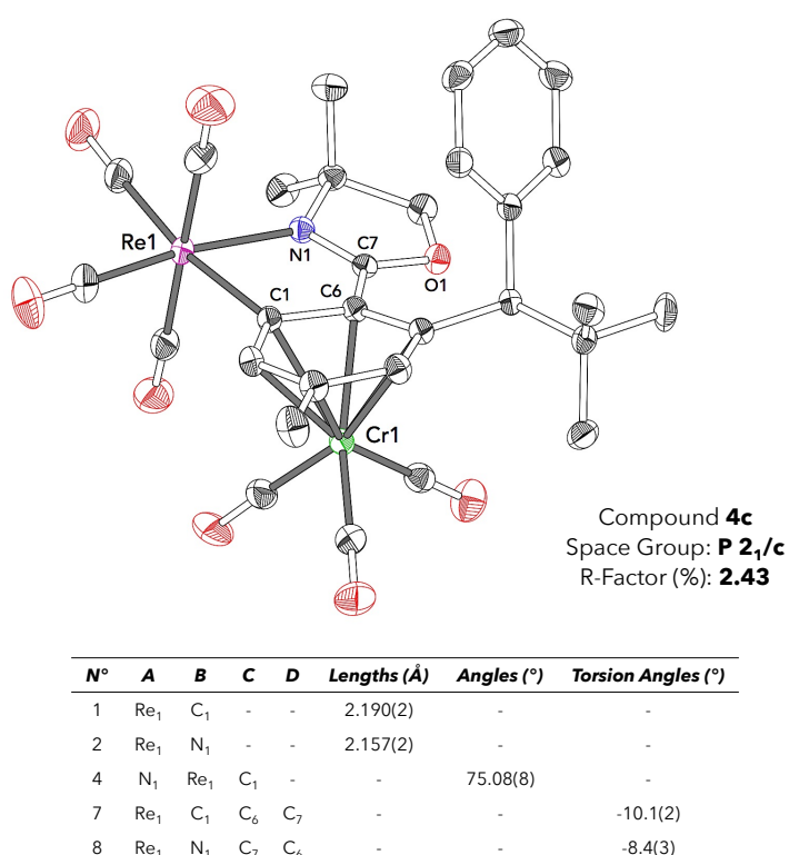
Figure 61: X-ray structure and selected interatomic distances of compound 4c .
