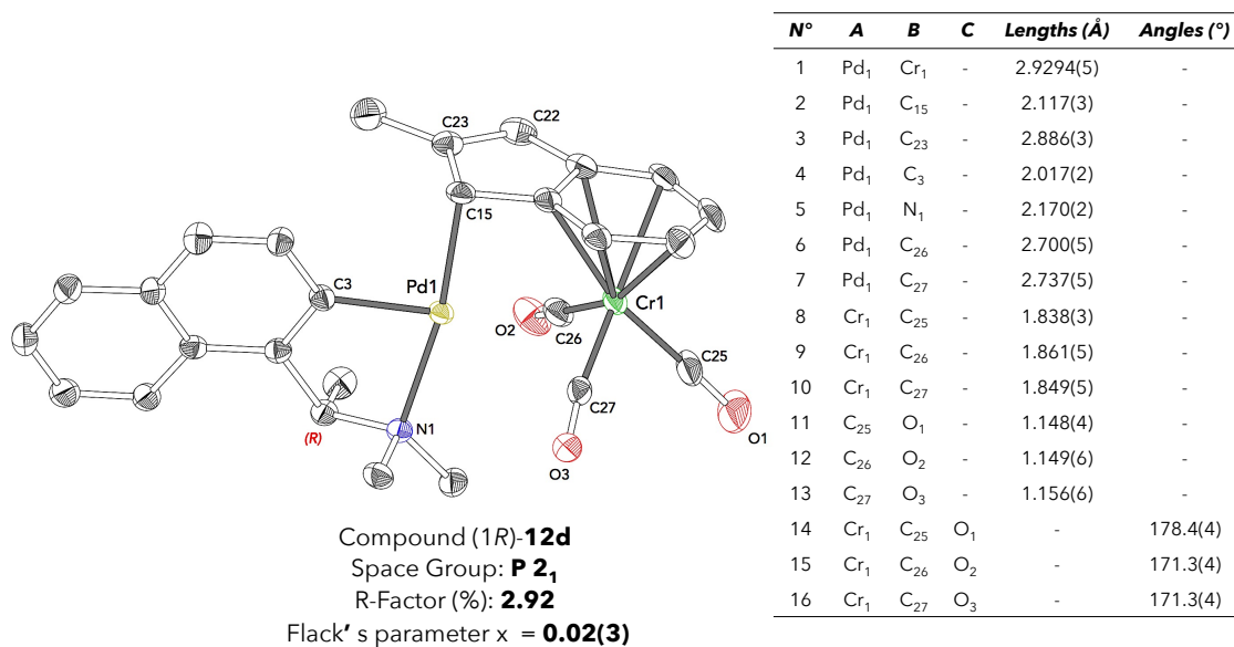
Figure 123: X-ray structure and selected interatomic distances of compound (1-R)-12d .
