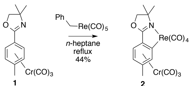
Figure 51: Formation of the cyclometallated 5-membered ring rhenium compound.
