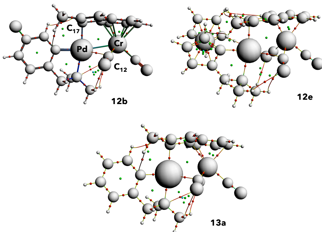
Figure 144: Atoms-in-molecule analysis of the electron density topology for 12b , 12e and 13a . Red and green dots are associated to Bond (BCP) and Ring (RCP) Critical Points, respectively. Grey spheres materialize the atomic positions scaled by their associated density.
