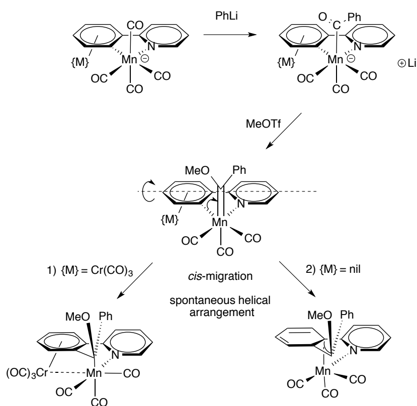
Figure 43: Synthesis of helical syn -facial heterobimetallic ( \eta^6 -aryl)benzyl and mononuclear \eta^3 -benzyl complexes.
