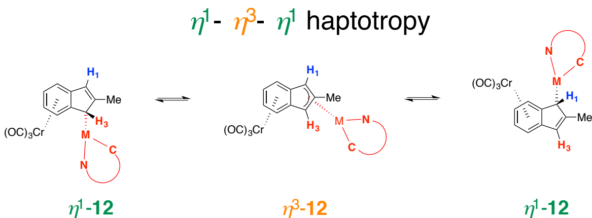
Figure 133: Assumed fluxional behavior of the Pd centre.
