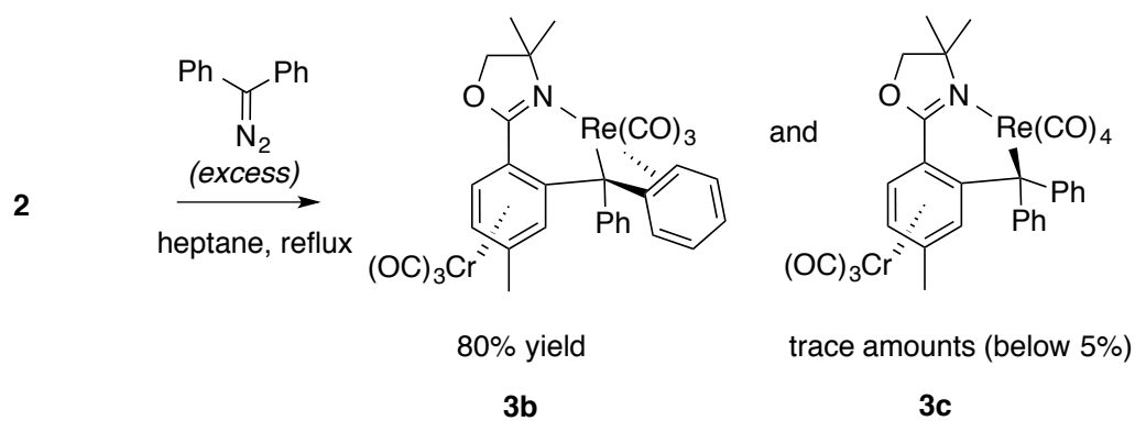
Figure 55: Reaction of 2 with \text{Ph}_2\text{CN}_2 .
