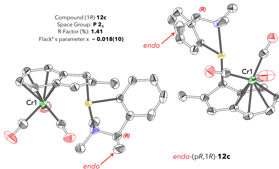
Figure 130: X-ray structure of compound ( 1R )- 12c containing only the endo diastereomer.
