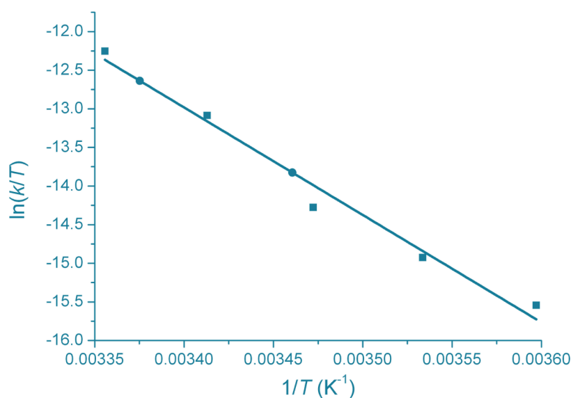
Figure 173: Eyring plot of \ln(k/T) vs T^{-1} (K -1 ) for the isomerization of 16b into 17b - 1 H NMR (600 MHz) line-shape between 278(1) and 298(1) K in toluene.
