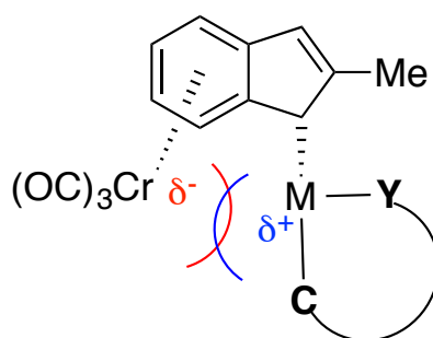
Figure 160: Reductionist representation of the stabilization by attractive Coulombic occlusion of the electron-unsaturated M centre (M = Pd, Pt) with a proximal large moiety (here Cr(CO) 3 ) on which charge density concentrates.
