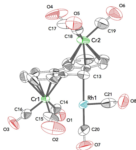
Compound syn-33a Space Group: P 2 1 R-Factor (%): 9.97
