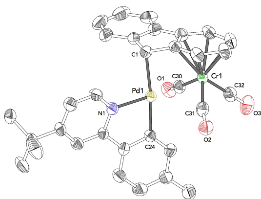
Compound 16f Space Group: Pca2 1 R-Factor (%): 3.95
