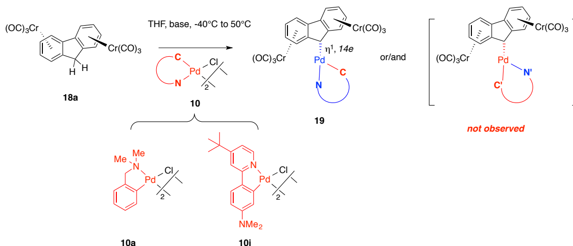
Figure 181: The ambiphilic character of anion 18b allows only one orientation for the metallacycle ( N-Pd-C ).
