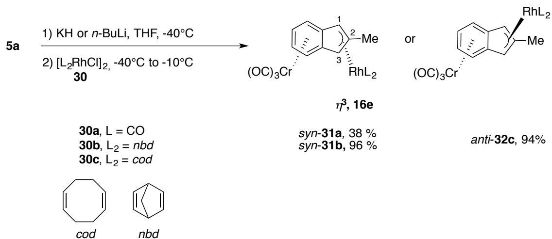
Figure 203: First approach for the synthesis of Rh(I) hemichelates.
