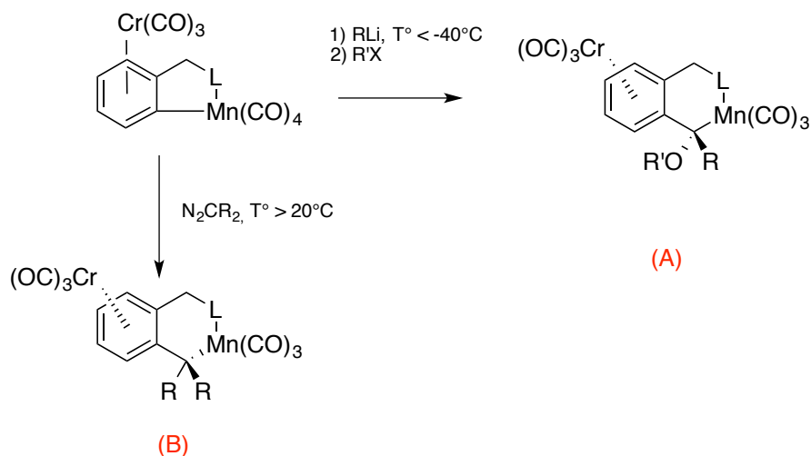
Figure 40: Two pathways for the synthesis of the metallospiralenes complexes.
