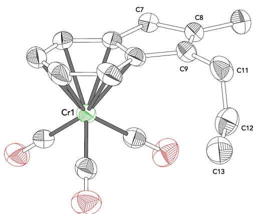
Compound 9a Space Group: P 2_1/c R-Factor (%): 4.04
