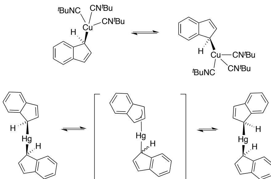
Figure 96: Fluxional behaviour of Cu(I) and Hg(II) derivatives.
