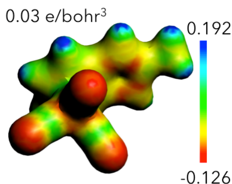
Figure 78: Map of Coulombic Potential of anion 5b showing the buildup of charge density at the double bond of the indenyl ligand and at the Cr(CO)_3 moiety.
