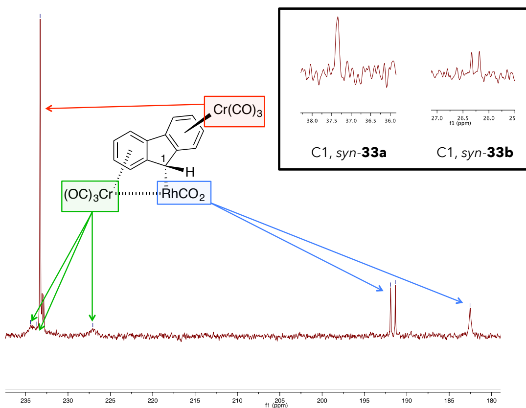
Figure 213: Most notable ^{13}\text{C} NMR spectral features for the Rh(I) hemichelates.
