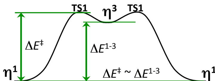
Figure 100: Diagram describing the mutual exchange between the indenyl benzylic positions assuming the \eta^3 \rightarrow \eta^1 barrier to be negligible.
