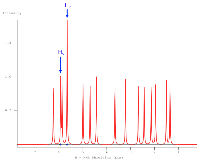
Figure 97: Theoretical ^1\text{H} NMR spectrum (ADFview 2012) calculated for \eta^1\text{-7b} at the COSMO(toluene)(ZORA)-SAOP/AE-TZP level from a ground state singlet geometry calculated at the COSMO (toluene) (ZORA)-PBE-D3(BJ)/AE-TZP. The two blue dots point the peaks arising from \text{H}_9 (left hand side peak) and \text{H}_7 (right hand side peak). The numbering is that of the experimental structure of 3b , \text{H}_7 is connected to \text{C}_7 , the carbon atom vicinal to the Pd centre.
