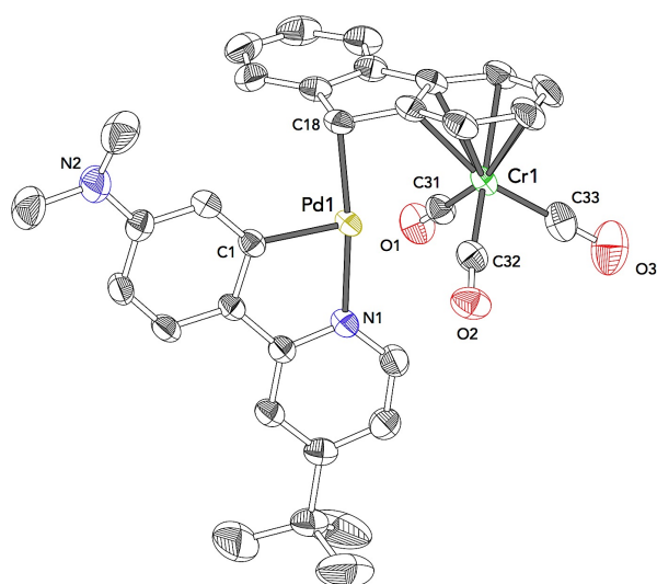
Compound 17i Space Group: P 2 1 /c R-Factor (%): 3.04
