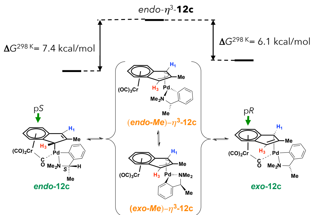
Figure 135: Putative mechanism of transposition of the palladacyclic unit in (1 S )- 12c modeled by DFT (COSMO toluene). Planar chiral configurations are assigned according to Schlägl's convention 922 giving priority n°1 to the Pd-substituted carbon position.
