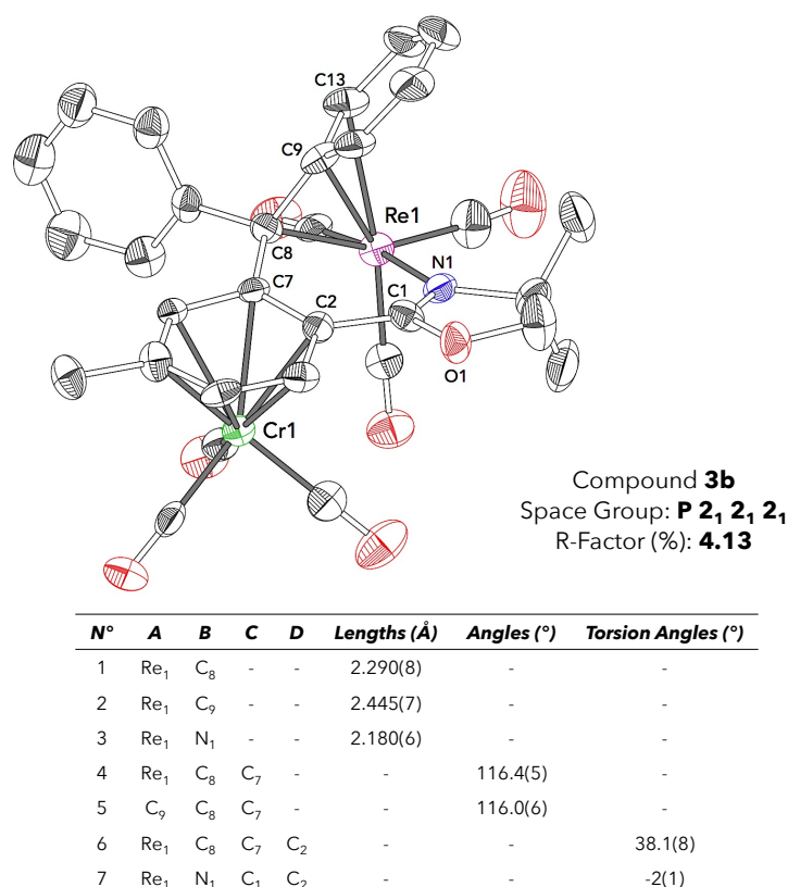
Figure 56: X-ray structure and selected interatomic distances of compound 3b .
