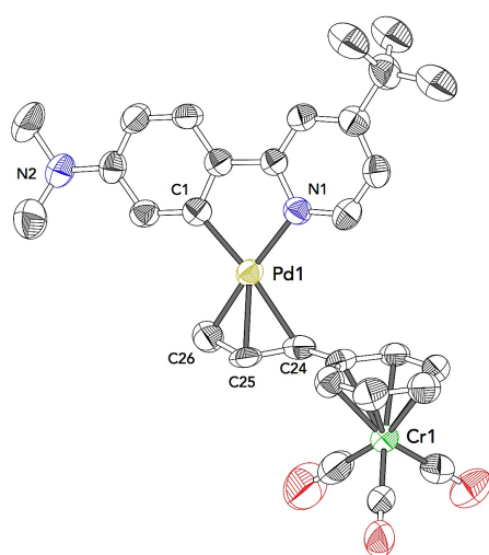
Compound 21i Space Group: C 2/c R-Factor (%): 7.08
