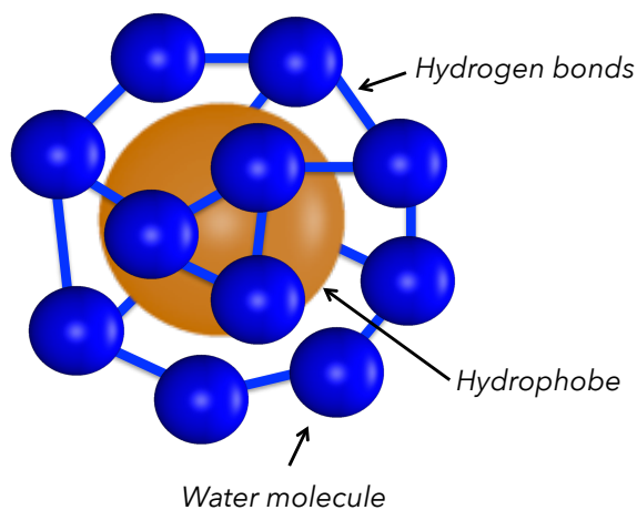
Figure 17: Illustration of water clathrates forming around the hydrophobe.
