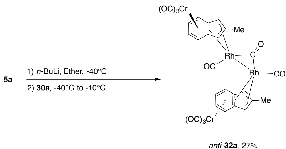
Figure 208: Formation of anti - 32a after a slight modification of the experimental conditions.
