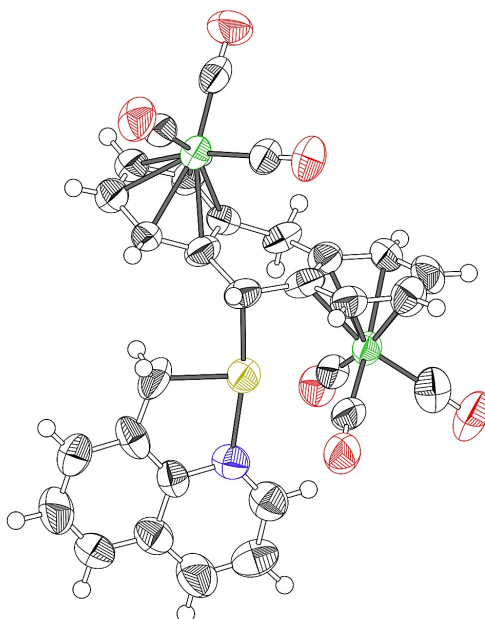
Figure 199: X-ray structure of the bimetallic obtained while trying to synthesize another tetrametallic complex 29j .
