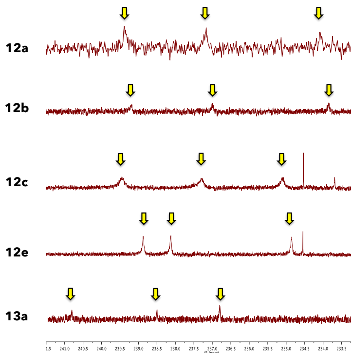
Figure 132: The ^{13}\text{C} NMR spectra of complexes 12 in d_6 -benzene present the typical signature of a rotation-hindered \text{Cr}(\text{CO})_3 moiety in an asymmetric local environment that is materialized by three broad signals at around \delta 239, 237, and 235 ppm.
