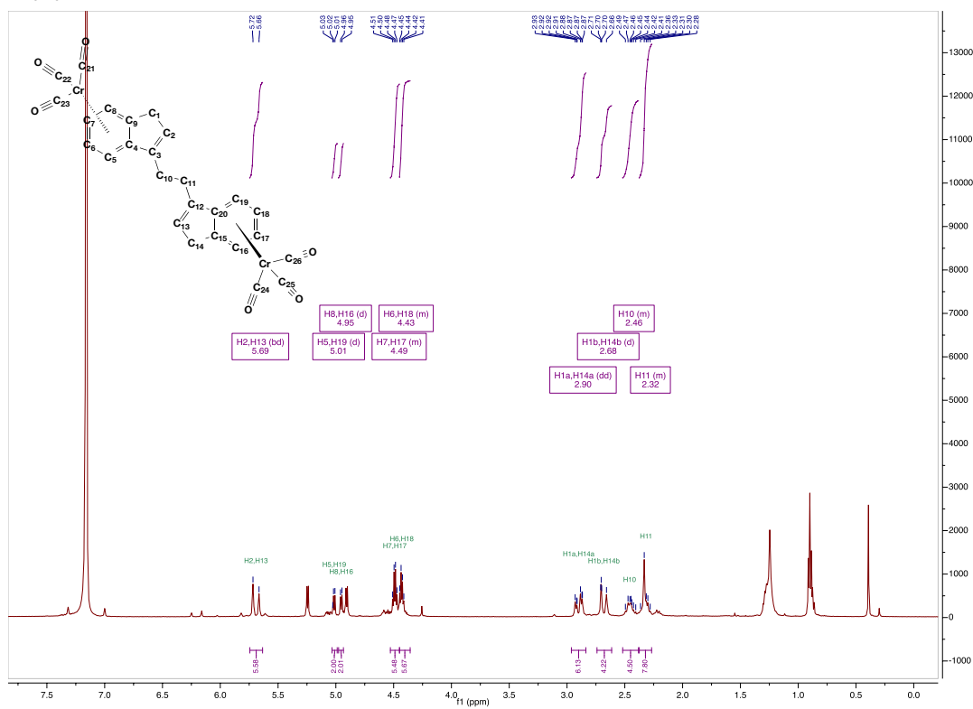
C_6D_6 - ^1H - 500 \text{ Mhz} - 293 \text{ K} - \text{isomer B.}
