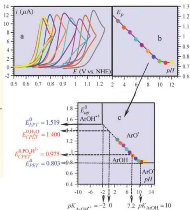
Figure IV-18: Some reaction pathways proposed in the literature for the redox mechanism of phenol and its derivatives like cresols (adapted from Costentin et al 2010).
