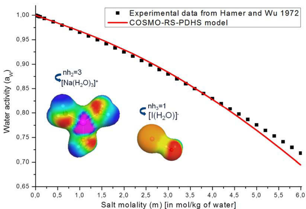
Figure III-44: Water activity results predicted by the COSMO-RS-PDHS model on the binary water -NaI, after hydrating the ions ( n_{h_2}=3 for Na^+ and n_{h_3}=1 for I^- ).
