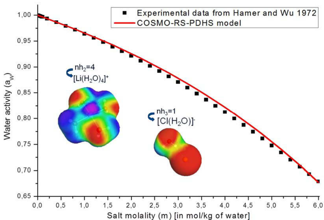
Figure III-18: Water activity results predicted by the COSMO-RS-PDHS model on the binary water-LiCl, after hydrating the ions ( n_{h_2}=4 for Li^+ and n_{h_3}=1 for Cl^- ). The COSMO-radii of atomic elements (Li, Cl, H and O) are given in Table III-6.
