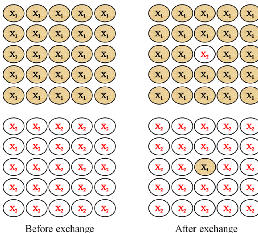
Figure I-4 : Physical significance of interchange energy.
