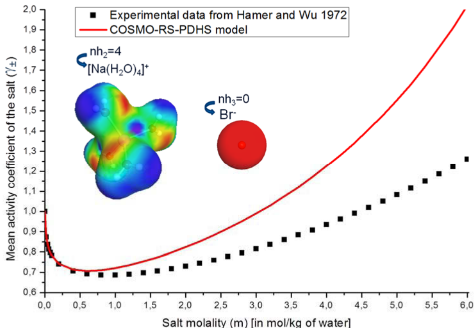
Figure III-43: \gamma_{\pm}^{(m)} results predicted by the COSMO-RS-PDHS model on the binary water -NaBr, after hydrating the ions ( n_{\text{H}_2}=4 for \text{Na}^+ and n_{\text{H}_3}=0 for \text{Br}^- ).
