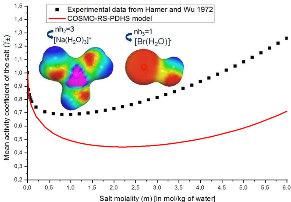
Figure III-42: \gamma_{\pm}^{(m)} results predicted by the COSMO-RS-PDHS model on the binary water -NaBr, after hydrating the ions ( n_{\text{H}_2}=3 for \text{Na}^+ and n_{\text{H}_3}=1 for \text{Br}^- ).
