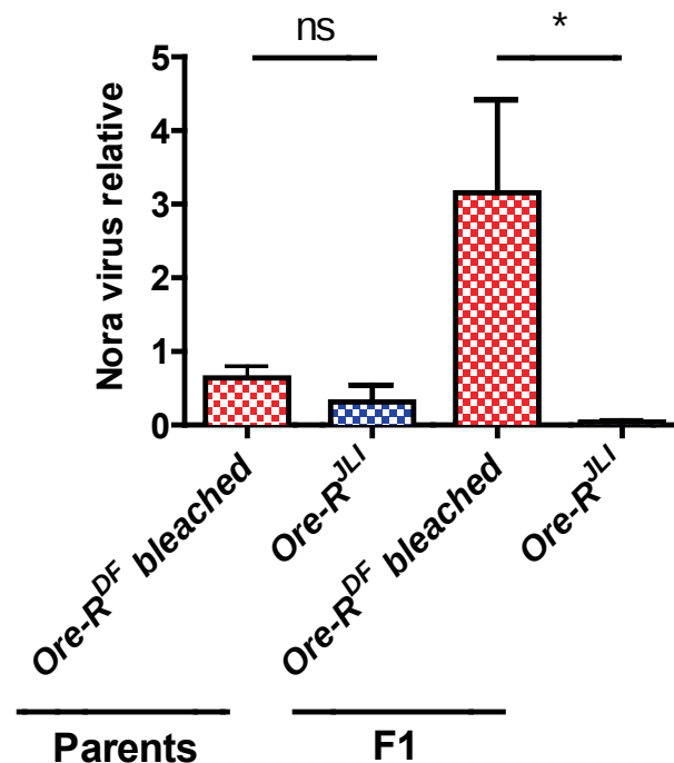
Figure 65. Ore-R DF flies are more sensitive to Nora virus infection compared to Ore-R JLI flies. Ore-R DF bleached flies and Ore-R JLI flies were contaminated with feces from Ore-R DF flies at 25°C for 5 days. Then, Nora virus RNA level was measured by qPCR in these flies and also in 4-8days flies from the first generation. Bar graphs represent the average standard deviation of 1 experiment.
