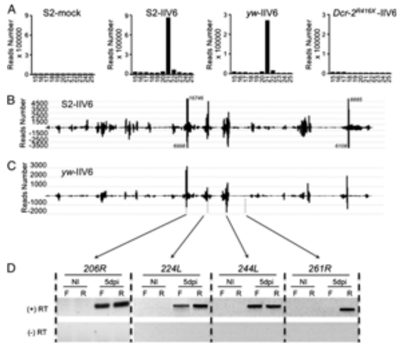
FIGURE 2. Virus-derived siRNAs in S2 cells and Drosophila adult flies infected by the DNA virus IIV-6. RNA was extracted 5 dpi from S2 cells infected by IIV-6 (MOI 0.01) and adult wild-type (yw) or mutant ( Dcr-2 R416X ) flies injected with IIV-6 (5000 PFU per fly). (A) Size distribution of the small RNAs matching the viral genome in S2 cells and adult flies of the indicated genotype. (B and C) Distribution of the 21-nucleotide siRNAs from the S2 cell (B) and yw adult fly (C) libraries along the IIV-6 genome. Each IIV-6-derived small RNA is represented by the position of its first nucleotide. The IIV-6-derived small RNAs matching the upper and lower strand of the DNA genome are respectively shown above (positive reads number) and below (negative reads number) the horizontal axis, which represents the 121482bp genome. In (B) , the number of reads for four peaks going off-scale is indicated next to them, in italics. (D) Strand-specific RT-PCR with primers corresponding to the annotated viral genes 206R , 224L , 244L , and 261R . The experiment was performed in the presence (+) or absence (–) of RT. NI, Noninfected; F and R, forward and reverse strand primer used for reverse transcription.
