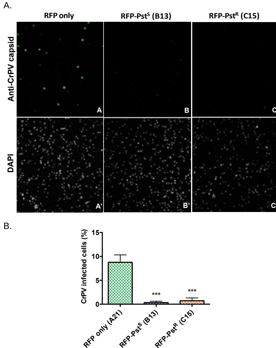
Figure 37. Overexpression of Pst S and Pst R decreases the number of cells infected by CrPV. A. Stable cell lines overexpressing RFP only (control, panels A and A' ), Pst sensitive (panels B and B' ) and resistant (panels C and C' ) versions tagged by RFP in N-terminal, were infected with CrPV (MOI 0.01) for 24h. Cells were stained with an antibody against CrPV capsid (anti-CrPV-4, panels A , B and C ). DAPI staining is represented in panels A' , B' and C' . Pictures were taken by confocal LSM700. B. CrPV infected cells were quantified using ImageJ. Bar graphs represent the average standard deviation of 9 pictures. Panels are representative of 1 experiment. Clones identifications are indicated in brackets.
