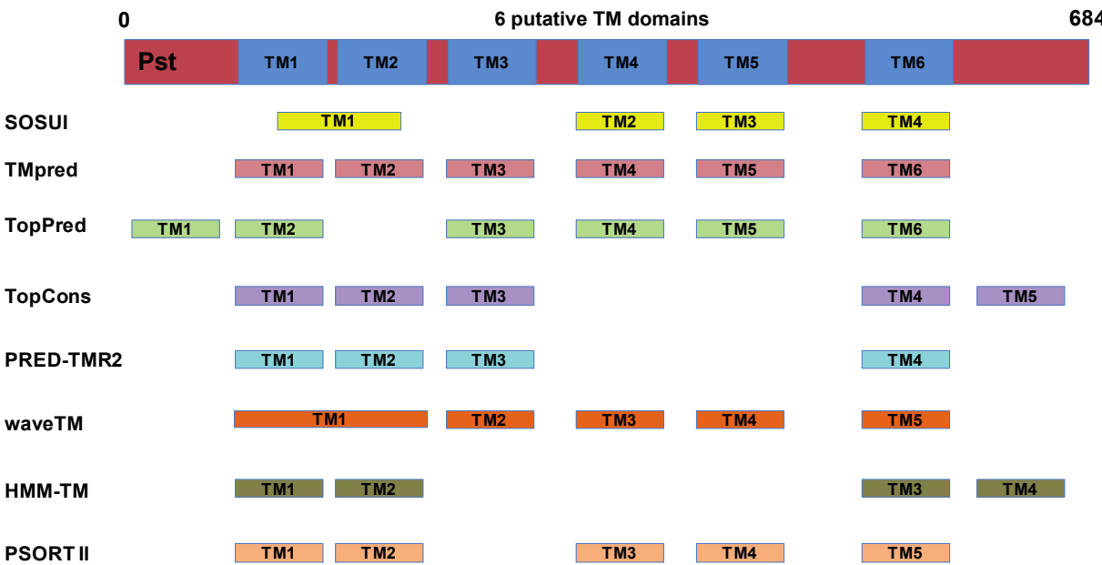
Figure 45. Prediction of 6 putative TM domains in Pastrel protein. Programs for TM prediction were used to identify the number of putative TM domains in Pastrel protein.
