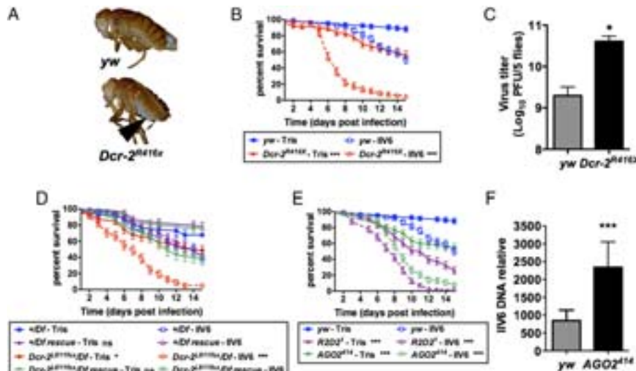
FIGURE 1. Dcr-2 is involved in host defense against the DNA virus IIV-6. (A) Upon injection of IIV-6 (5000 PFU) in wild-type ( yw ) and Dcr-2 416X mutant flies, typical blue paracrystalline structures appeared earlier in the abdomen (arrowhead) of the mutant flies. Representative individuals 10 dpi are shown. (B) Groups of 20 wild-type ( yw ) or Dcr-2 416X mutant flies were injected with IIV-6 or Tris, and survival was monitored daily. The difference between the wild-type and Dcr-2 mutant flies is statistically significant. (C) Viral titer in groups of five wild-type ( yw ) or Dcr-2 416X mutant flies was monitored 10 dpi. (D) Rescue of the hemizygous Dcr-2 416X for the IIV-6 susceptibility phenotype by a transposon expressing a wild-type Dcr-2 transgene. Dcr-2 416X hemizygous flies ( Dcr-2 416X /Df) are significantly more susceptible than Dcr-2 416X hemizygous flies complemented by a wild-type Dcr-2 transgene ( Dcr-2 416X /Df rescue). Df is Df(2R)BSC45, a deficiency that fully uncovers the Dcr-2 locus. All control and genomic rescued flies are in CantonS background. (E) Survival rate of wild-type ( yw ), R2D2 14 , and AGO2 114 mutant flies upon IIV-6 or Tris injection. (F) IIV-6 DNA load was determined by quantitative PCR in four groups of six flies of the indicated genotype at 10 dpi. For all panels, the data represent the mean and SD of at least three independent experiments, and the difference between controls and mutant flies is statistically significant. * p < 0.05, *** p < 0.001. All experiments are performed at 22°C (A, C, F) or 25°C (B, D, E).
