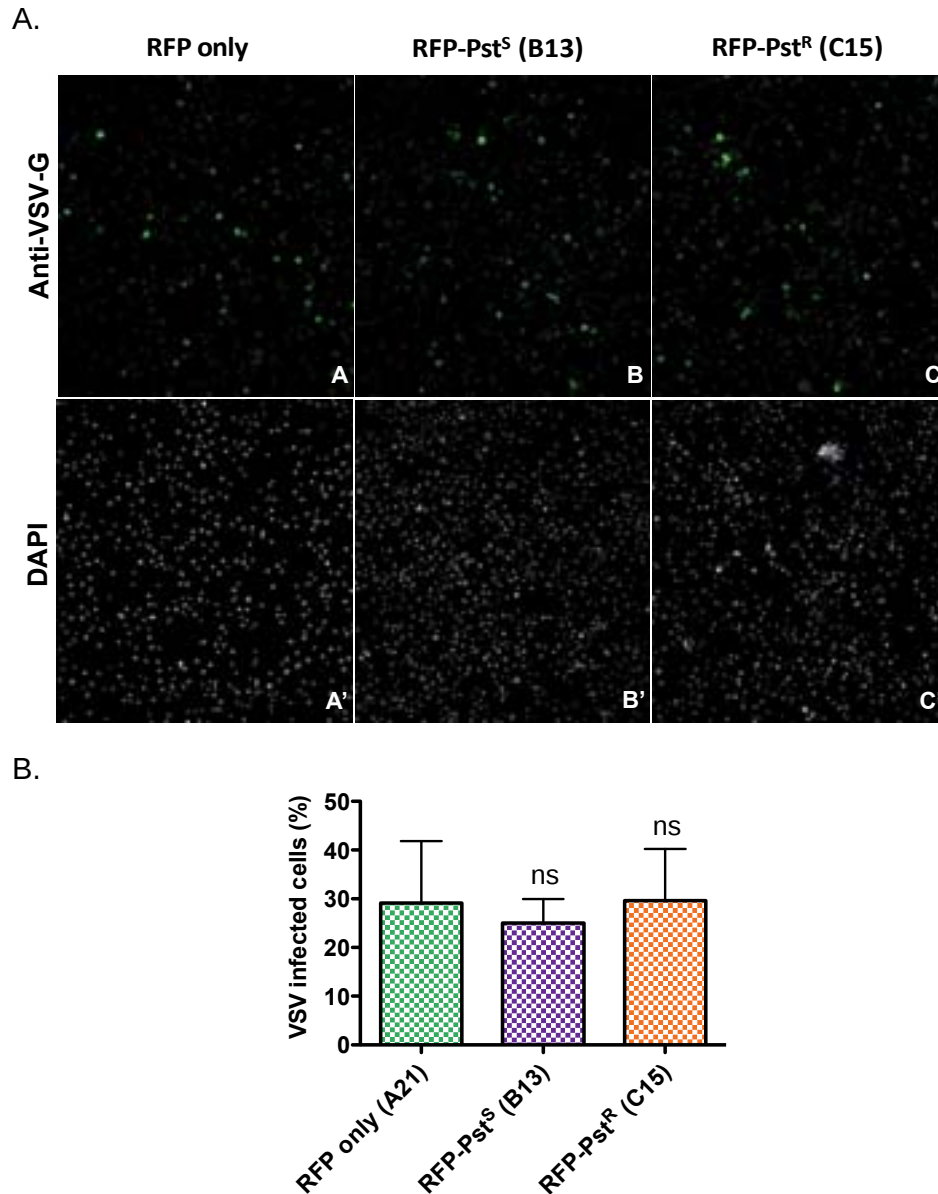
Figure 39. Overexpression of Pst S and Pst R does not affect the number of cells infected by VSV. A. Stable cell lines overexpressing RFP only (control, panels A and A' ), Pst sensitive (panels B and B' ) and resistant (panels C and C' ) versions tagged by RFP in N-terminal were infected with VSV (MOI 25) for 48h. Cells were stained with an antibody against glycoprotein (G) of VSV (anti-VSV-G-FITC, panels A , B and C ). DAPI staining is represented in panels A' , B' and C' . Pictures were taken by confocal LSM700. B. VSV infected cells were quantified using ImageJ. Bar graphs represent the average standard deviation of 9 pictures. Panels are representative of 1 experiment. Clones identifications are indicated in brackets.
