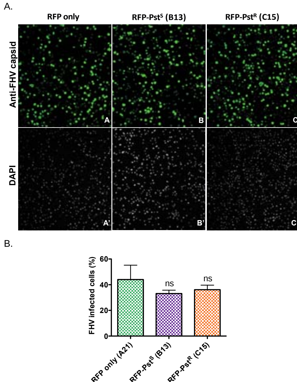
Figure 38. Overexpression of Pst S and Pst R does not affect the number of cells infected by FHV. A. Stable cell lines overexpressing RFP only (control, panels A and A' ), Pst sensitive (panels B and B' ) and resistant (panels C and C' ) versions tagged by RFP in N-terminal were infected with FHV (MOI 1) for 24h. Cells were stained with an antibody against FHV capsid (anti-FHV-5588, panels A , B and C ). DAPI staining is represented in panels A' , B' and C' . Pictures were taken by confocal LSM700. B. FHV infected cells were quantified using ImageJ. Bar graphs represent the average standard deviation of 4 pictures. Panels are representative of 1 experiment. Clones identifications are indicated in brackets.
