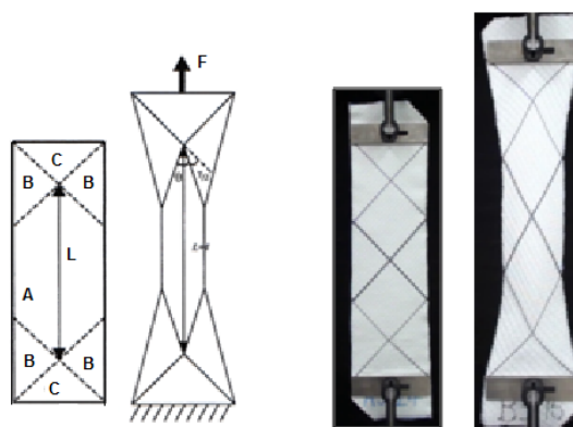
Figure 6. 15 : Bias Extension Test [78]
