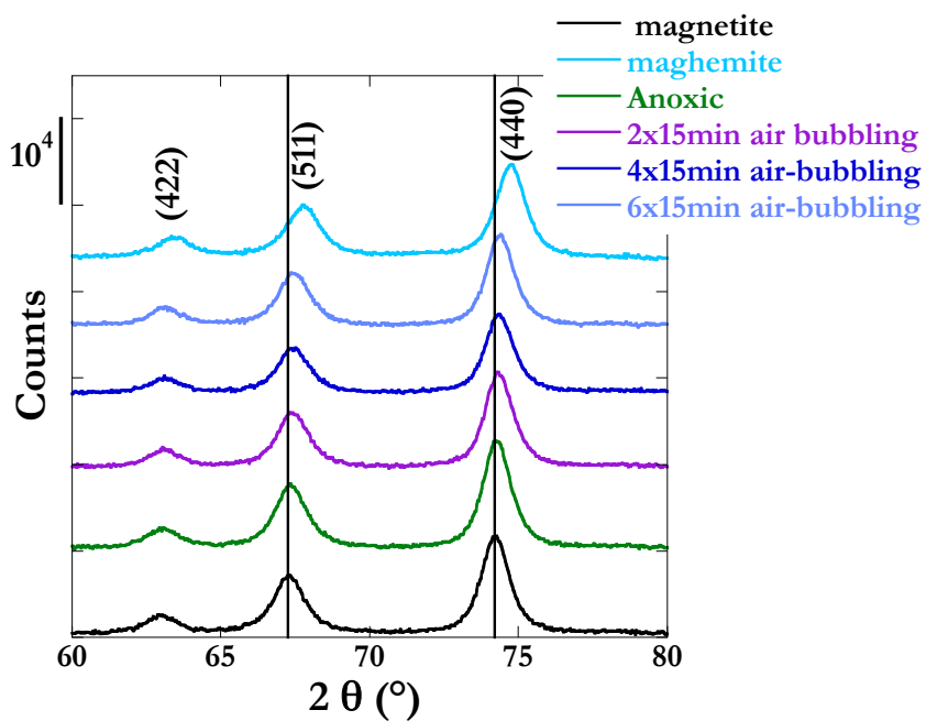
Figure SI-2 : Detailed high angle region of the powder XRD patterns obtained from the solid samples after reaction of nanoMt with NAL under oxic and anoxic conditions in the variable pH experiment. Data are compared with pure nanoMt (bottom, black line) and pure nanoMh (top, light blue), which indicates progressive oxidation of the nanoMt during the oxic experiment, as confirmed by XAS and colorimetric analyses (Figure IV.10).
