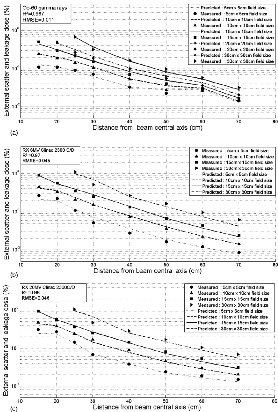
Figure 4. Variation, according to distance from the field center, of measured and calculated out-of-field doses at 10 cm depth in a water tank, for different field sizes (cm 2 ) and SSD set at 80 cm for cobalt treatment unit Alcyon II (a) and an SSD set at 100 cm for the Varian linear accelerators: Clinac 2300 C/D operated at 6 MV; (b) Clinac 2300 C/D operated at 20 MV RX; (c) and Novalis Tx operated at 6 MV (d). The doses are given as percentage of dose to dose at the depth of the maximal dose on the beam axis.
