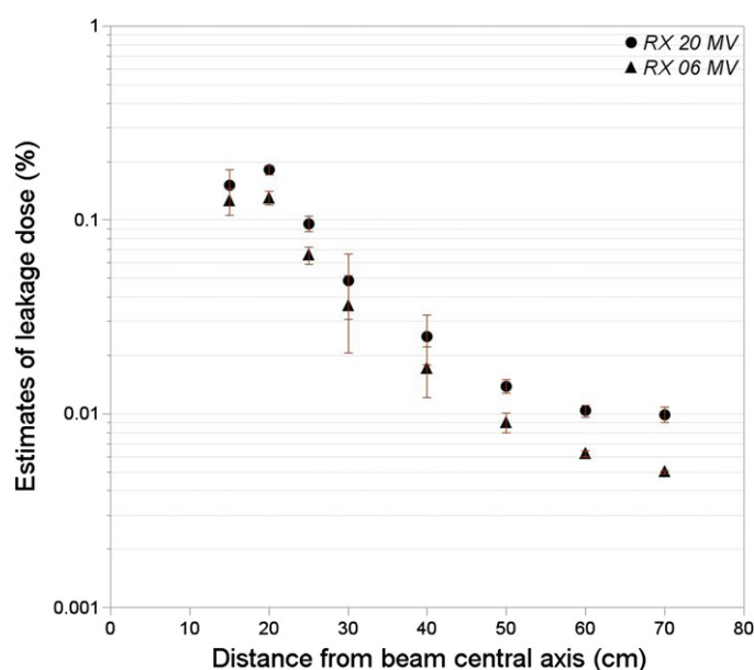
Figure 3. Estimates of leakage dose components (parameter \lambda(r, z, \varphi) , equation (3)) for the Varian linear accelerator Clinac 2300 C/D operated at 6 and 20 MV RX, respectively. The doses are given as percentages of the dose at the depth of the maximum dose on the beam axis.
