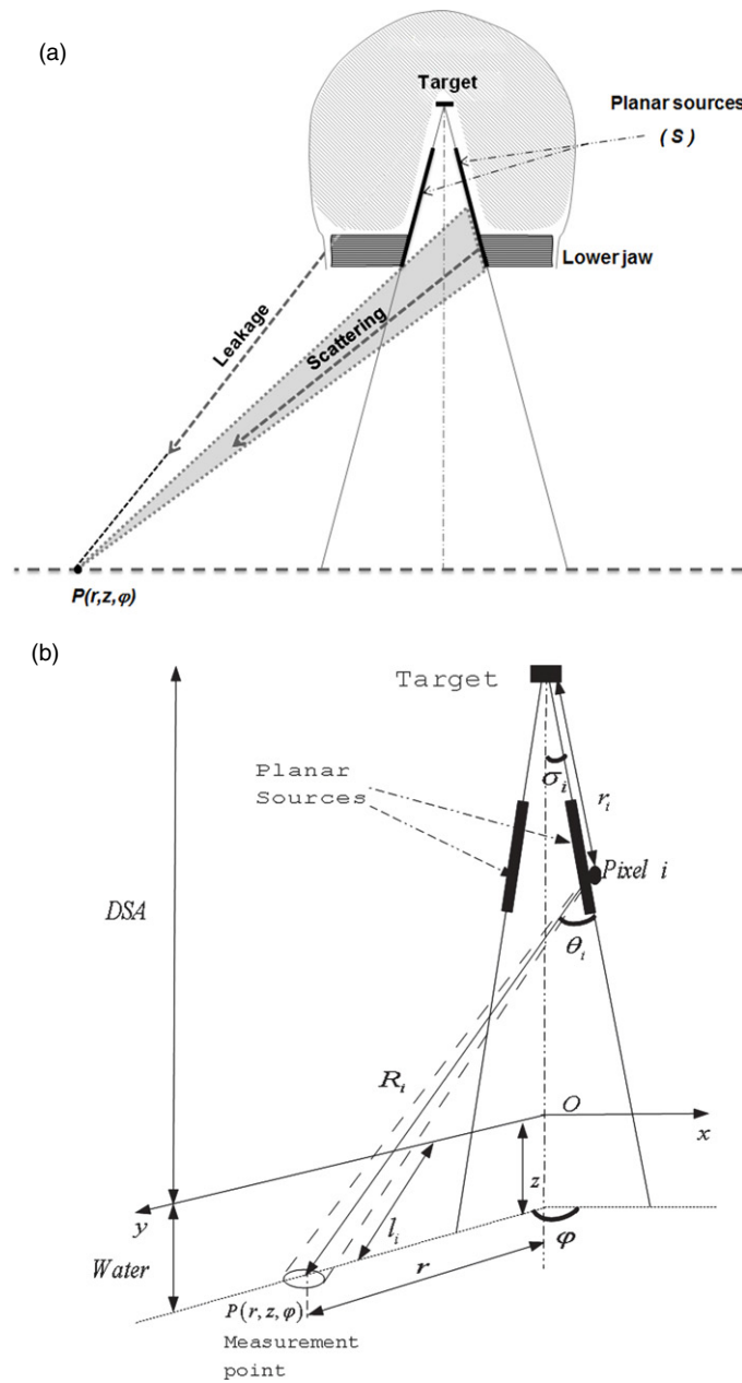
Figure 2. Basic principle of the multi-plane source model. (a) A schematic representation of the surface source S and of the linear accelerator head shielding and secondary collimator lower jaws is depicted and (b) indicates the geometric terms used in the final model formulation equation (7).
