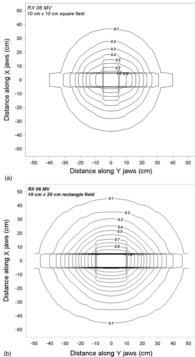
Figure 5. Calculated isodose for simple shaped fields (a) 10 \times 10 \text{ cm}^2 square field and (b) 10 \times 20 \text{ cm} rectangular field. Doses are given as percentage of the dose to the dose at the depth of the maximum dose on the beam axis. Calculations are made for Varian linear accelerator Clinac 2300 C/D operated at 6 MV RX.
