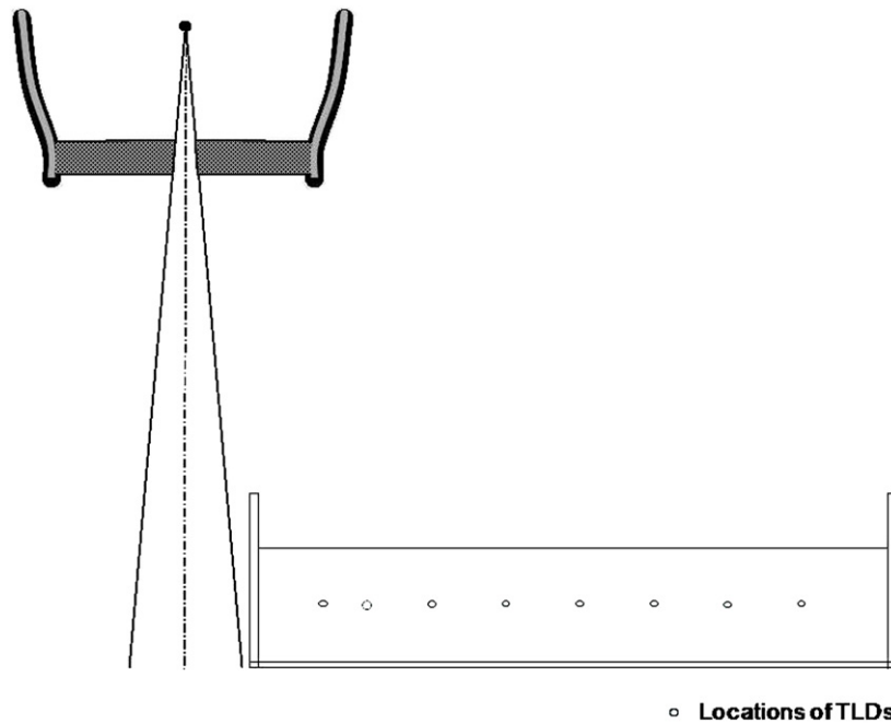
Figure 1. Experimental setup used to measure the dose reflecting the sum of the components related to external scattering and external leakage radiation, respectively.
