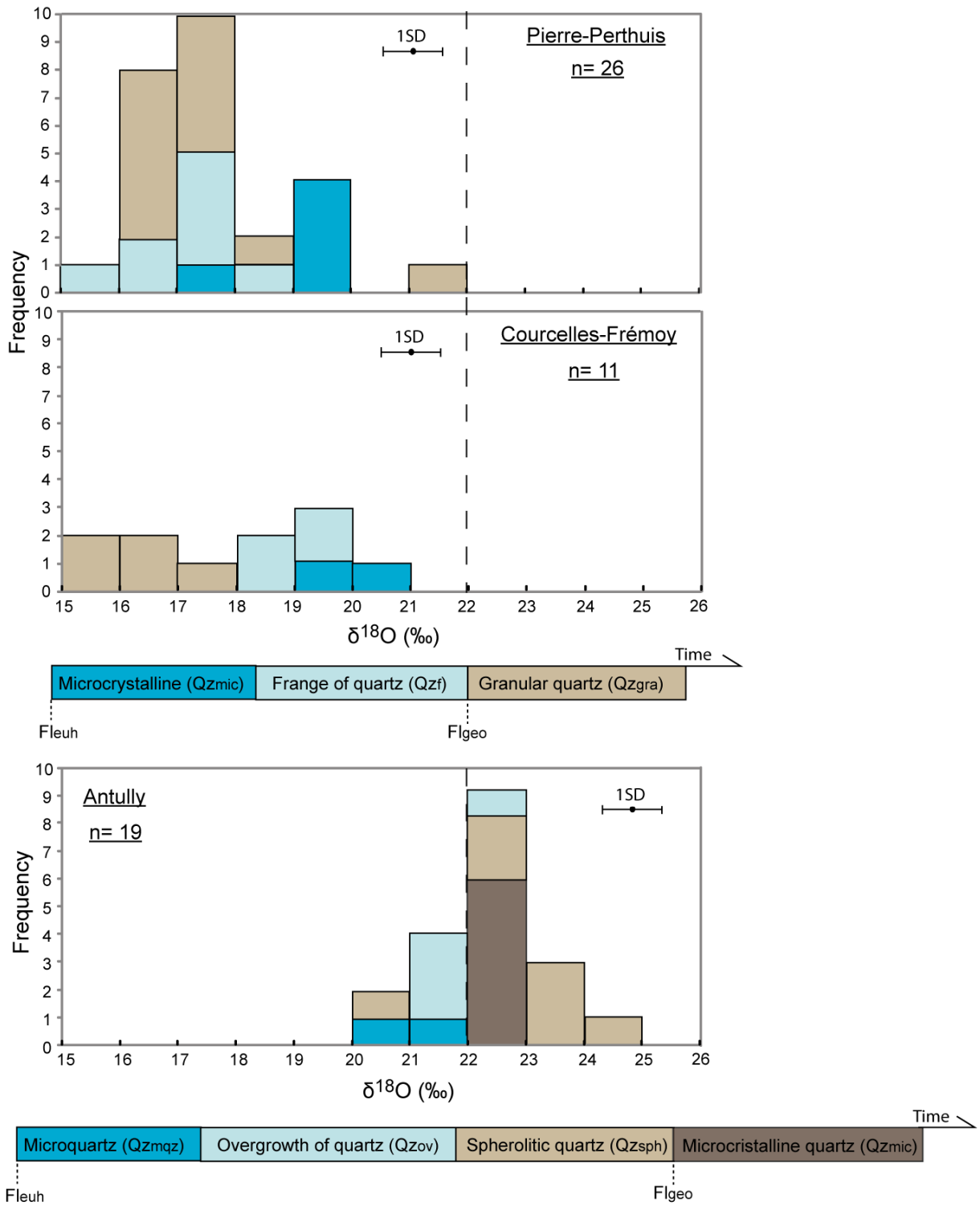
Figure 10: Distribution of \delta^{18}\text{O} (V-SMOW) in quartz stages from Pierre-Perthuis, Courcelles-Fré moy and Antully deposits
